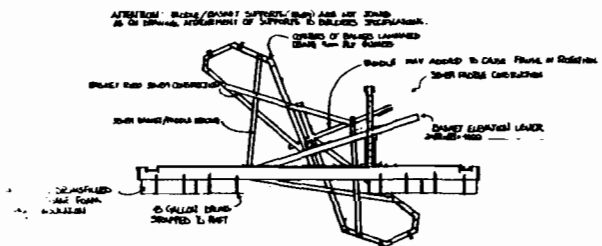
④ ELEVATION VIEW OF FISHWHEEL SCALE 1/50
