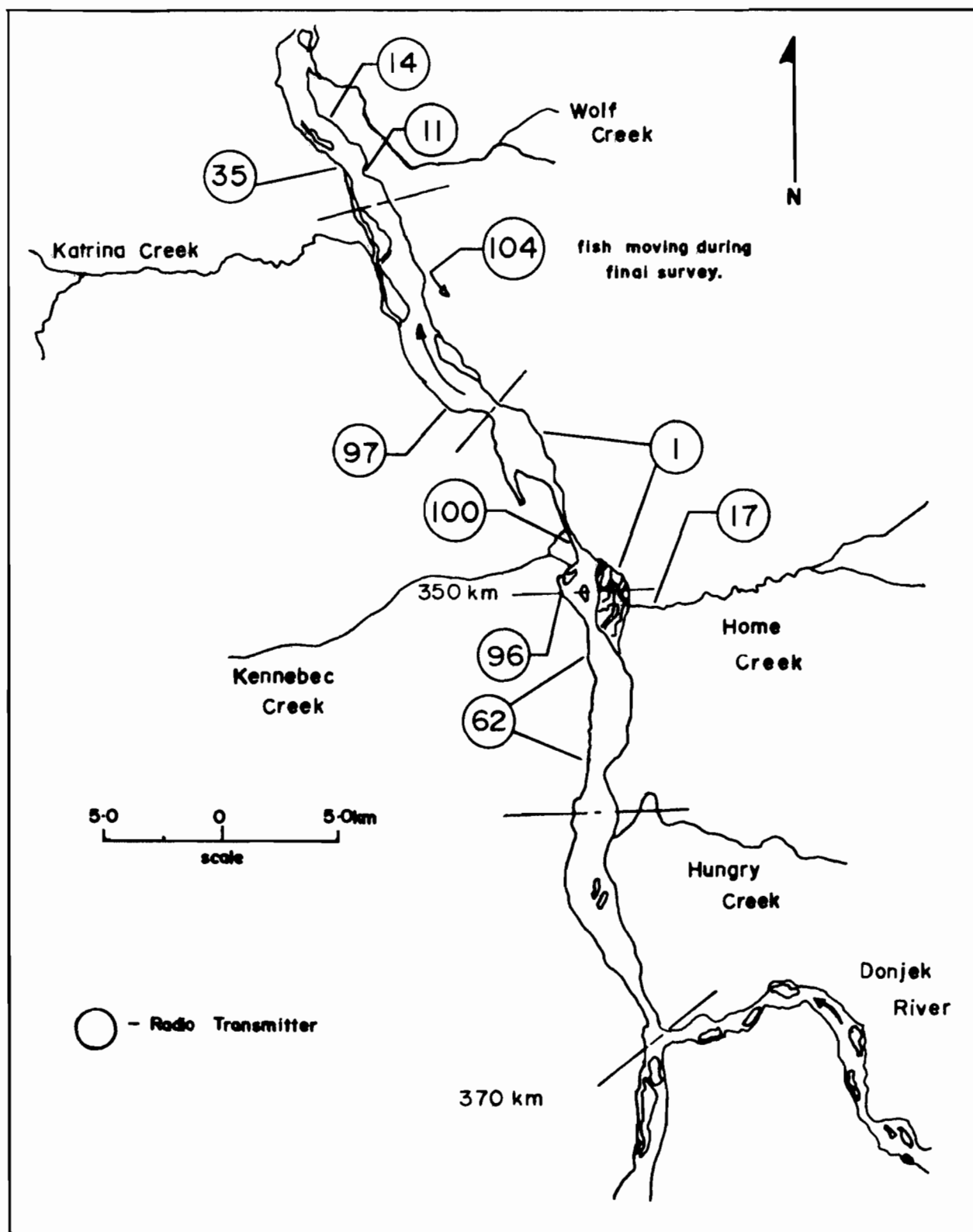
Figure 27 Location of radio transmitters in spawning areas on the White River between km 320 and km 370, 1982. Distances shown are from the lowest tagging site
