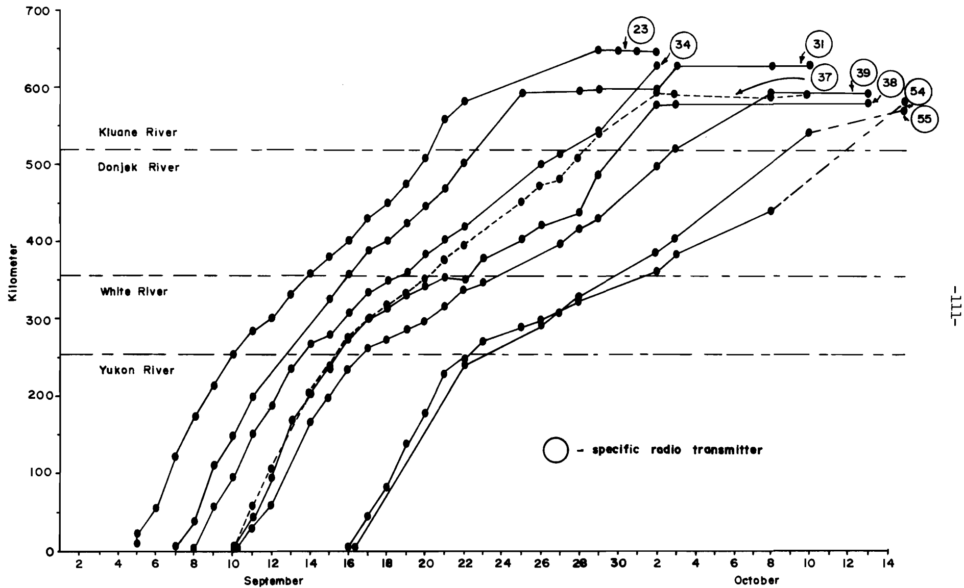
Figure 36a Radio tracking records of chum bound for the Kluane River, 1982. Distances shown are from the lowest tagging site
