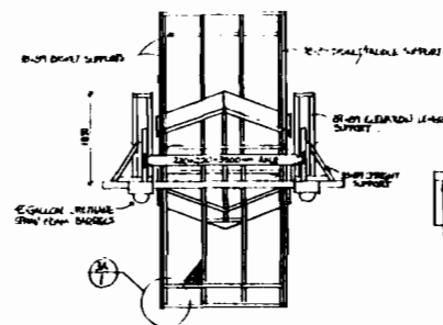
② ELEVATION VIEW OF FISHWHEEL SCALE 1/50
