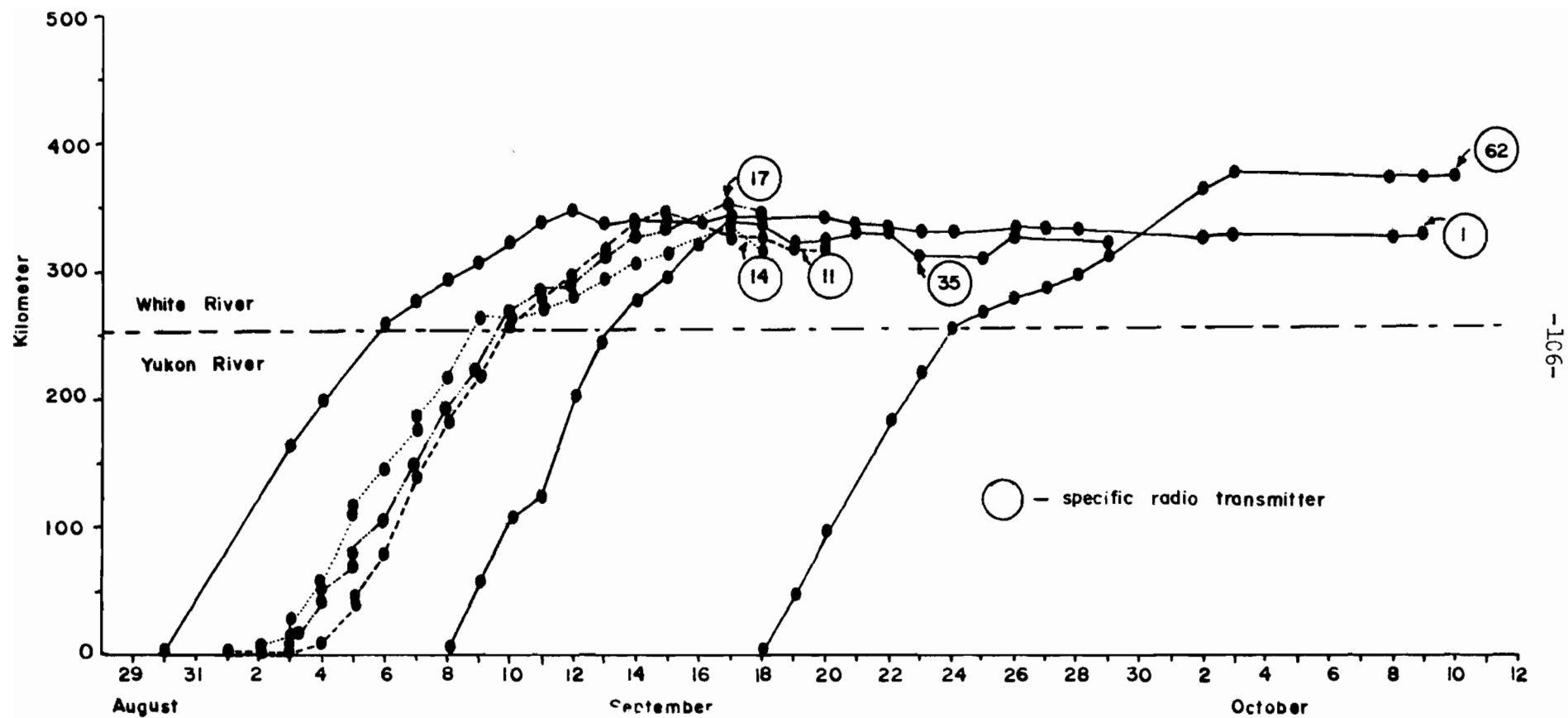
Figure 34a Radio tracking records of chum bound for the White River, 1982. Distances shown are from the lowest tagging site
