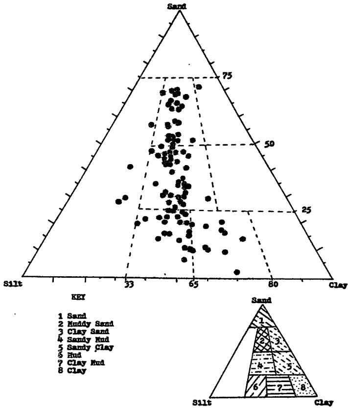
Figure 7 - Ternary Diagram of Sediment Composition
