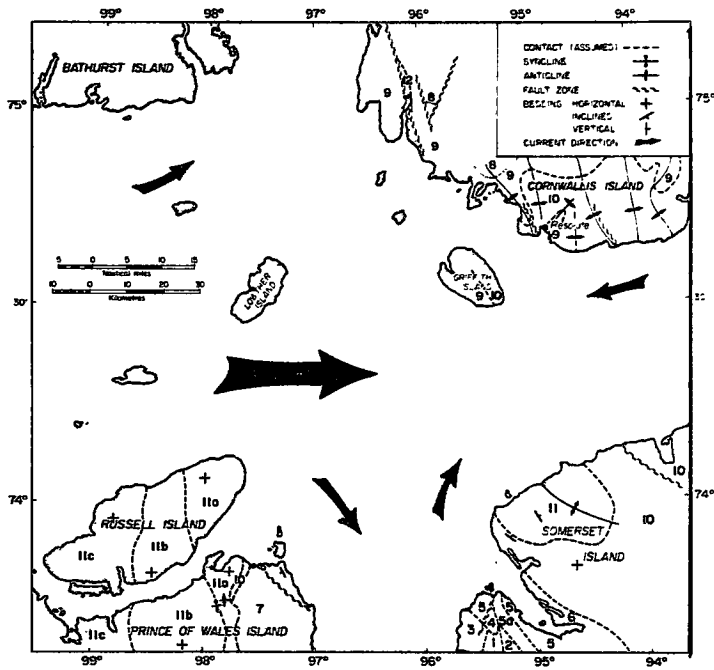
Figure 2 - Regional Geology and Currents
