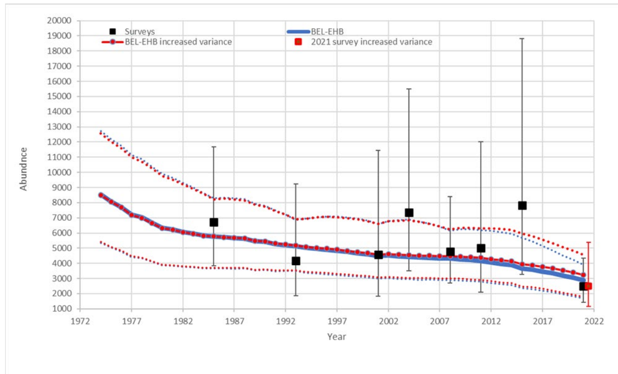
Figure 5 14 . Aerial survey (black) with 95% confidence intervals, population model estimates of BEL-EHB beluga abundance and 95% credibility intervals during 1974-2021. Two model runs were completed. The first fitted to the aerial survey time series (blue). The second run fitted to the aerial survey time series (black squares) with an increase of the coefficient of variation around the 2021 survey estimate from 29% to 40% 15 (red square).
