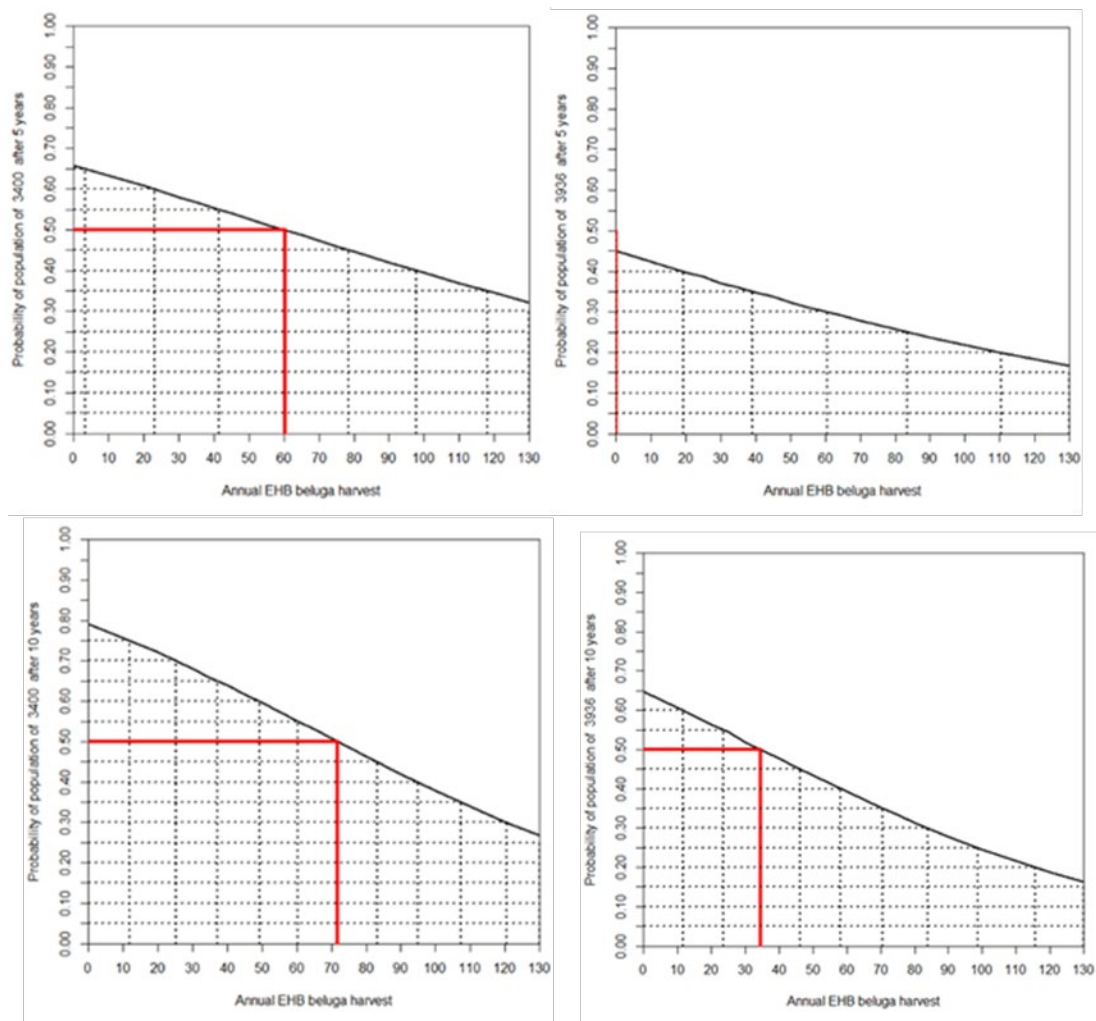
Figure 7 23 . Probability (y-axis) that the BEL-EHB stock would be greater than 3,400 animals (left) or estimated abundance of 3,900 (right) beluga in 2015 using the most recent corrected estimates assuming a 2021 survey coefficient of 40%, over a period of 5 years (top) or 10 years (bottom). X-axis is the reported harvest. Red line shows the harvest level with a 50% probability of being above the benchmark. 24
