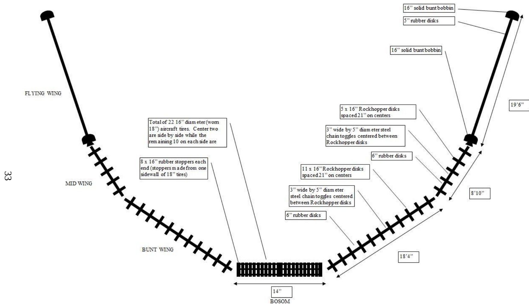
Figure 9. Details of the Rockhopper foot gear for the Atlantic Western Ila box trawl used on the 2018 WCVI synoptic bottom trawl survey.
