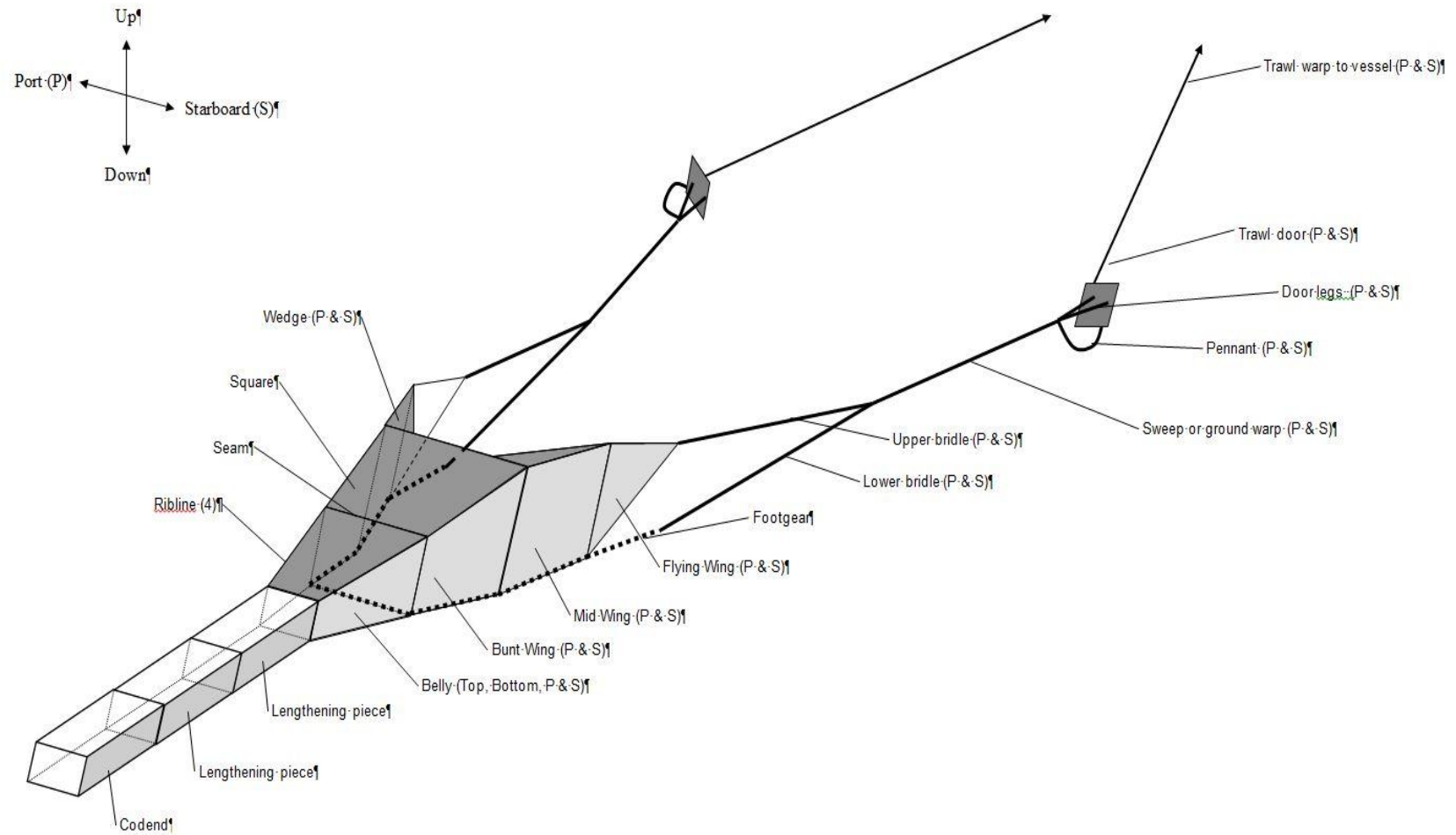
Figure 4. Overview diagram of the Atlantic Western Ila box trawl used on the 2018 WCVI synoptic bottom trawl survey.
