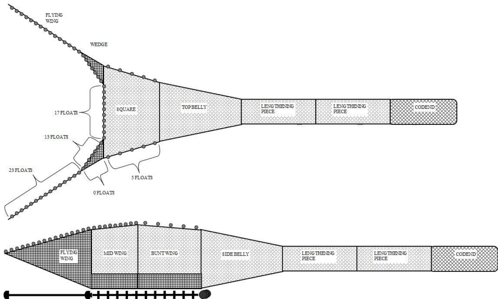
Figure 5. Top and side view of the Atlantic Western Ila box trawl used on the 2018 WCVI synoptic bottom trawl survey.
