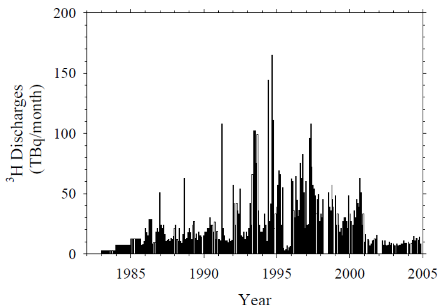
Figure 9. Monthly atmospheric discharges of tritium ( ^3\text{H} ) from the Point Lepreau Nuclear Generating Station (NBEPG 2006).
