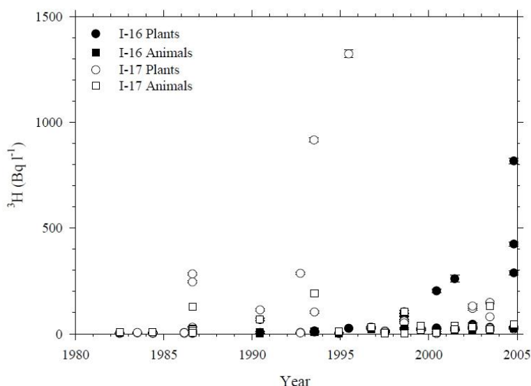
Figure 25. Tritium time series (1980-2005) for marine plants and animals collected near reactor cooling water intake (I-16) and discharge (I-17) sampling sites (Source: Nelson et al. 2007 MS).
