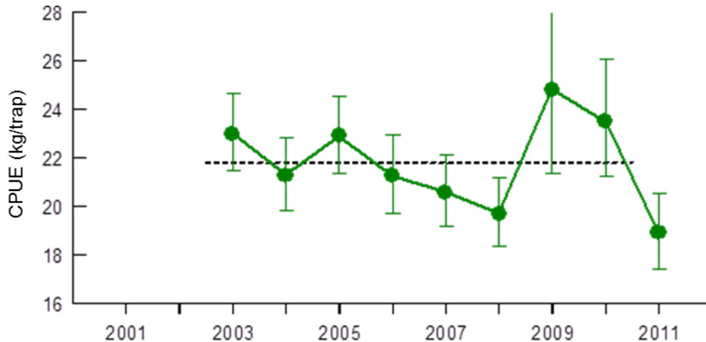
Figure 51. Standardized catch per unit effort (CPUE \pm 95% confidence interval) in the whelk fishery from 2001 to 2011 in Fishing Area 15. The horizontal line represents the 2003–2010 baseline level.
