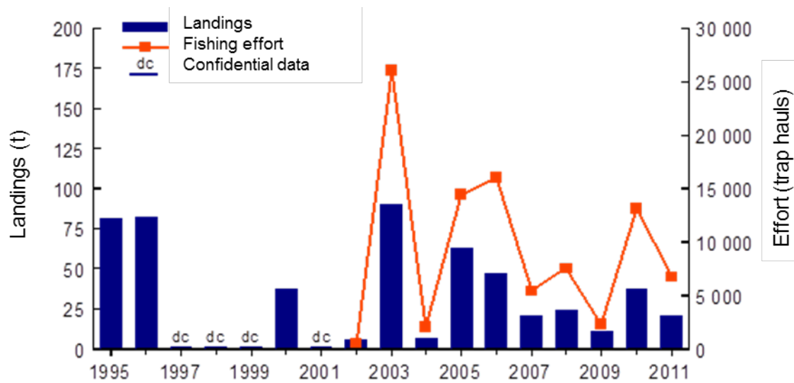
Figure 34. Whelk landings and fishing effort from 1995 to 2011 in Fishing Area 8.
