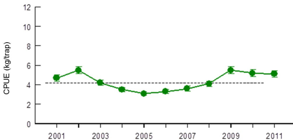
Figure 28. Standardized catch per unit effort (CPUE \pm 95% confidence interval) in the whelk fishery from 2001 to 2011 in Fishing Area 6. The horizontal line represents the 2001–2010 baseline level.
