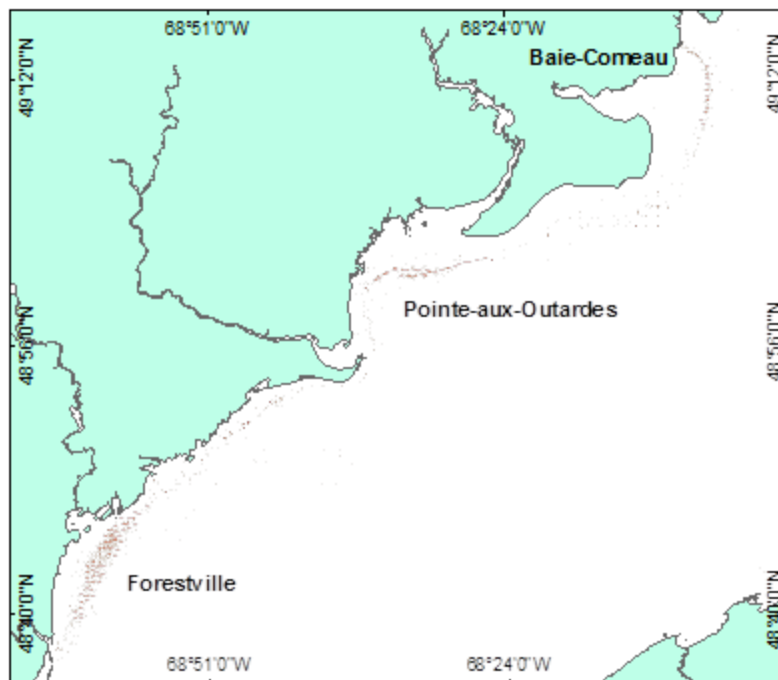
Figure 53. Distribution of commercial fishing effort from 2001 to 2004 (black circle) and research survey sampling stations (red square) from Forestville to Baie-Comeau.
