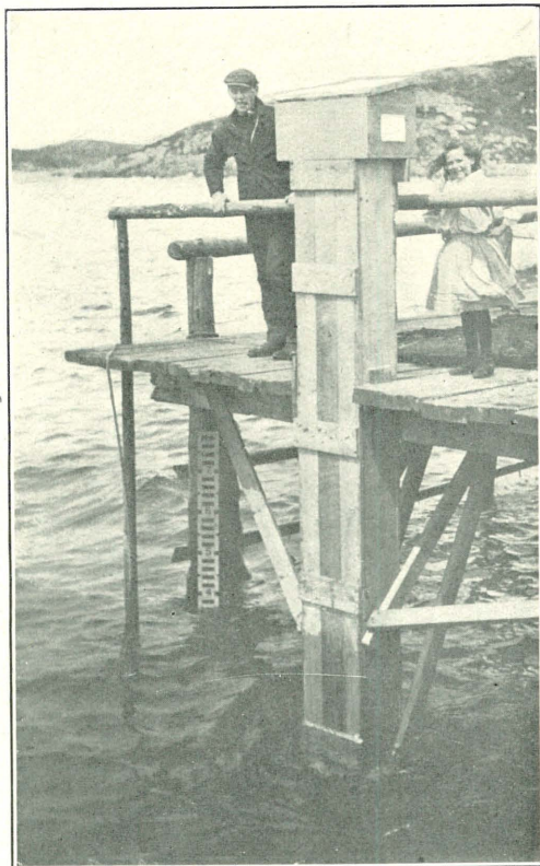
TEMPORARY TIDAL STATION showing a scale and tide column with shelter box on top which contains the Recording Instrument.
