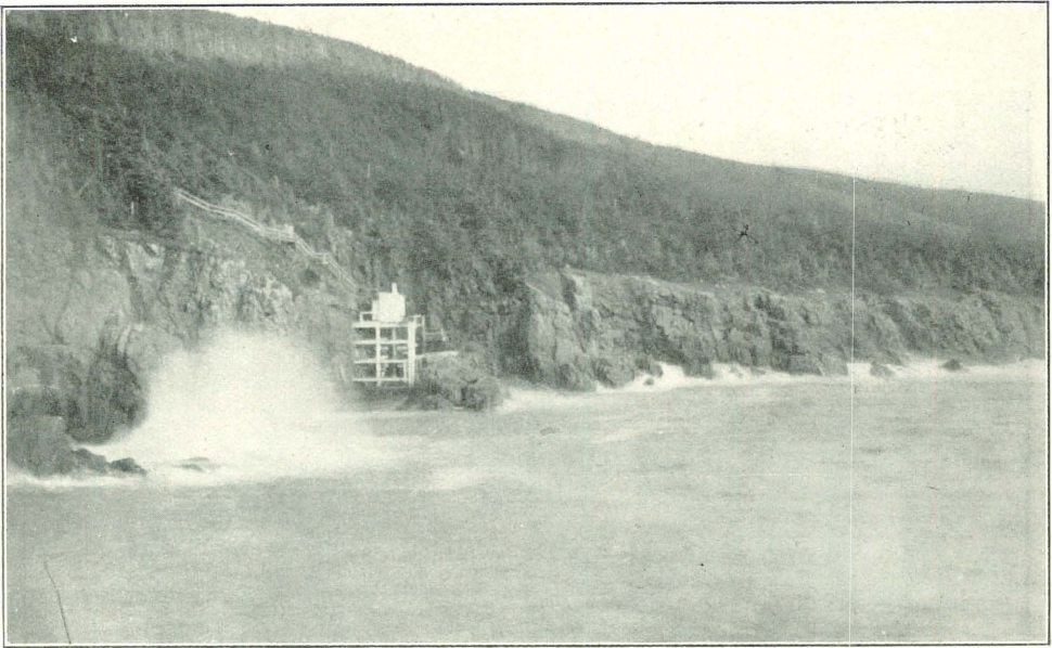
A principal Tidal Station. The Tide gauge on St. Paul Island, Cabot Strait; a small island in the main entrance to the Gulf of St. Lawrence.
