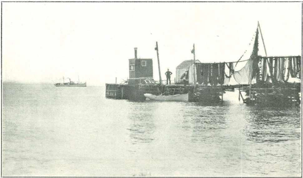
A principal Tidal Station. The Tide-house at Forteau Bay, in Belle Isle Strait. Built on cribwork, balasted with stone, placed at the end of a fishing stage.
