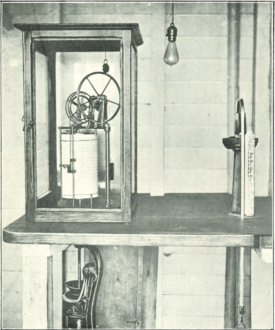
THE TIDE-RECORDING INSTRUMENT.
