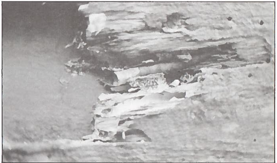
Oak rubbing strake infested with teredo (shipworm)
