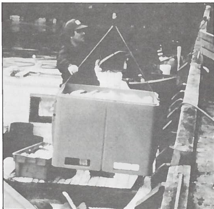
Each of these containers can hold approximately 450 lbs. of round cod, can be moved with ease (note the fork lift adapters on the bottom), and has drainage holes which allow the catch to drain on board.
