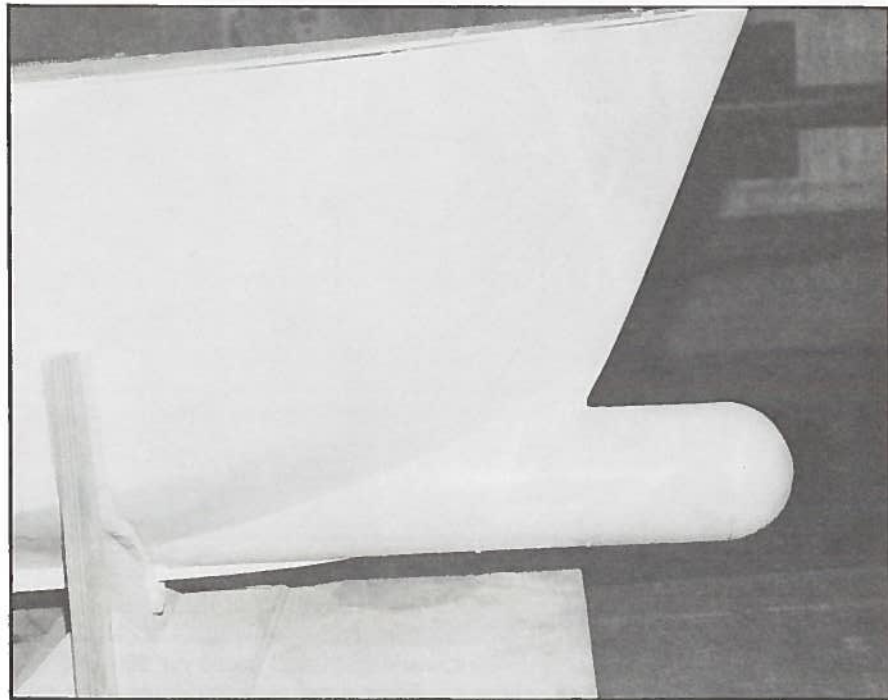
Bulbous Bow — Trawler Model
