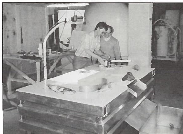
Fish are moved along a conveyor belt (circular in this case) for image assessment by an electronic camera (mounted on a metal arm and positioned directly above the conveyor). This data is then processed by algorithm to determine species, length, and weight.
