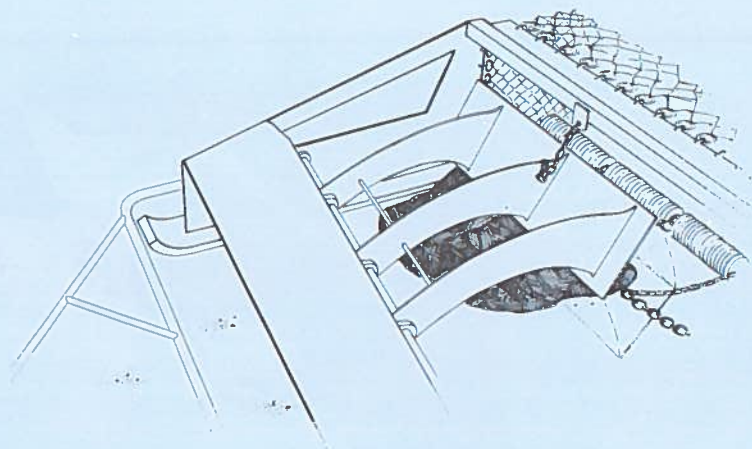
Prototype scallop rake showing hinged blade (one of three) in raised position encountering large anchored rock
