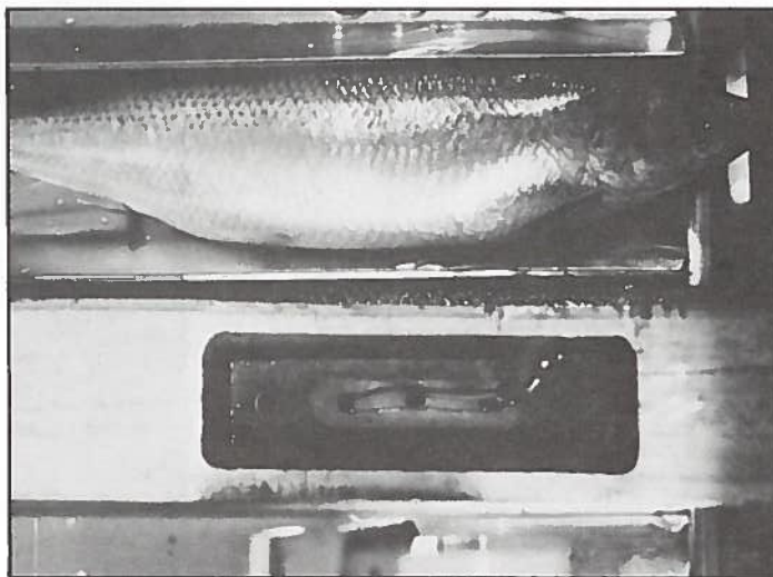
View showing light transmission through Male Herring properly positioned for source and sensor
