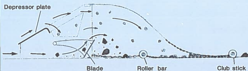
Prototype scallop rake (side view) arrows indicate water flow direction
