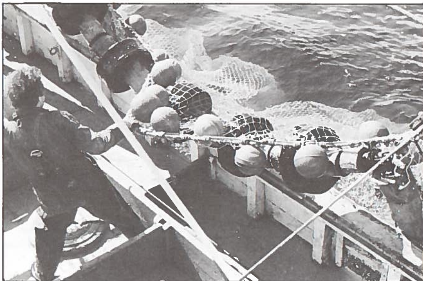
The Yankee 36 Trawl — note wooden footgear and rubber tire bobbins.
