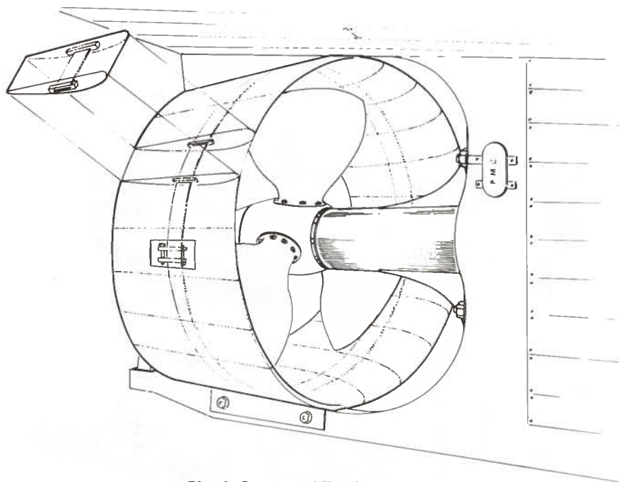
Plastic Segmented Nozzle
