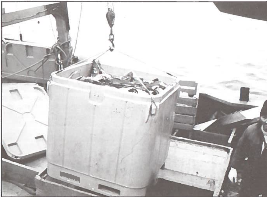
Containers Offer a Practical Alternative to Net Bags and Fish Hold Insulation.
