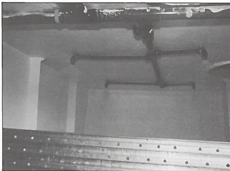
Spray system heads at the top of an onboard crab holding pen
