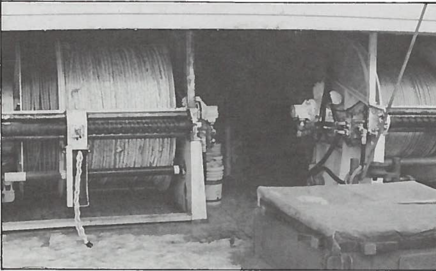
Combination fully-powered reels for Trawling and Scottish Seining. The capacity of each reel is 9,000 feet of rope plus 4,200 feet of trawl wire; there is a dividing flange on each reel. Change-over time from trawling to Scottish seining or vice versa is approximately 20 minutes. The reels shown above are located under the bow of "The Jessie and Shelly" out of Sambro, N.S.
