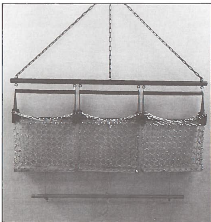
Inshore Scallop Rake — The Cayenne
