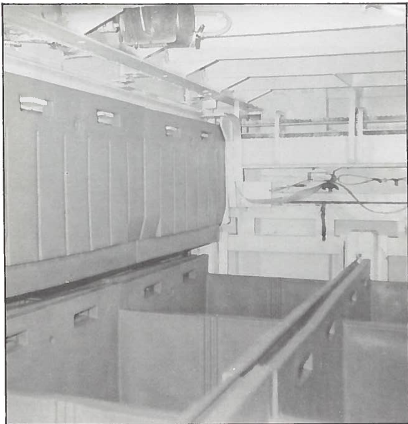
Forty-eight 460-litre boxes can be manipulated and stored in the forward hold of the Atlantic Margaret. This is done completely automatically after the containers leave the factory deck.
