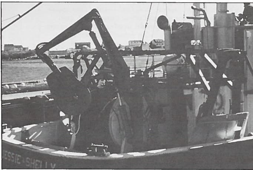
At the stern, the drum (above) is used to haul and store the seine/trawl after all the wire has been hauled and wound onto the reels at the bow. In the foreground is the crane and power block used to haul the Scottish Seine and the bag of the net.
