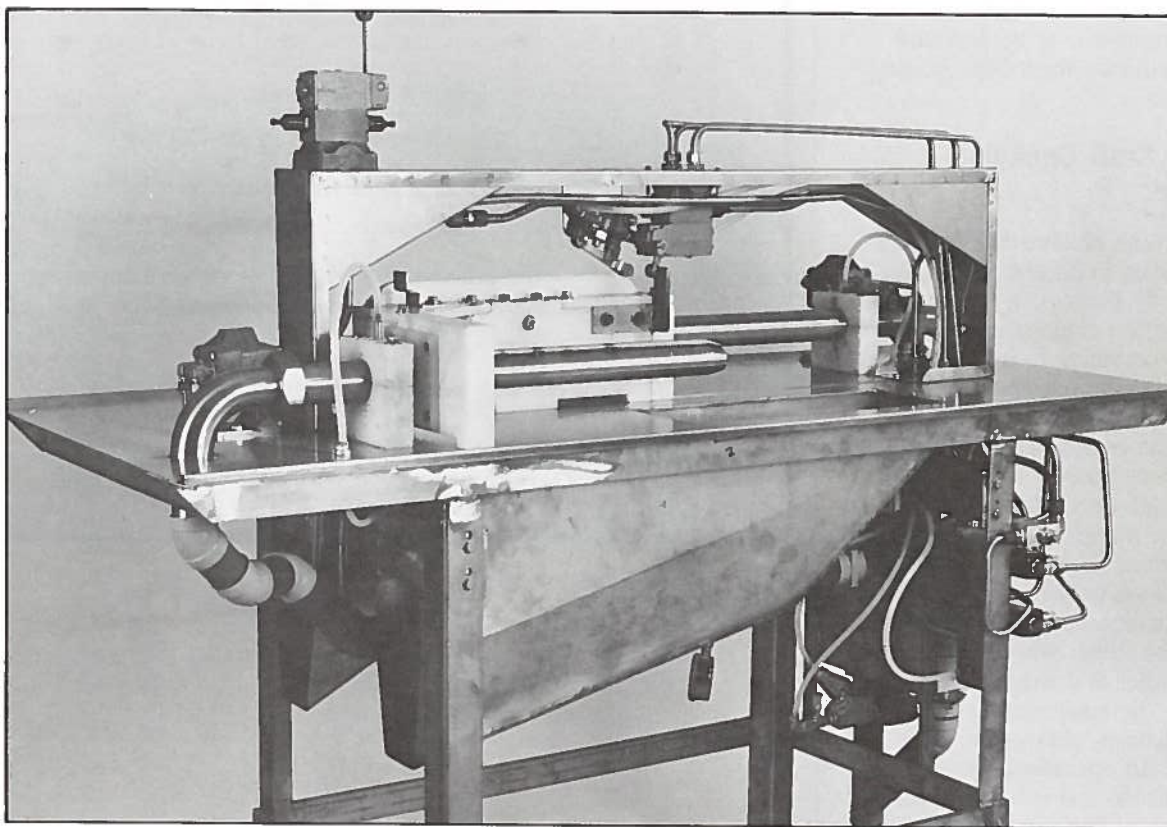
Suction Gutter (Groundfish)
