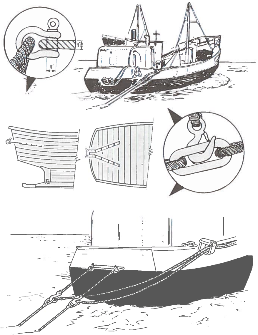
The Wire Guide System permits side trawlers to fish from the stern.
