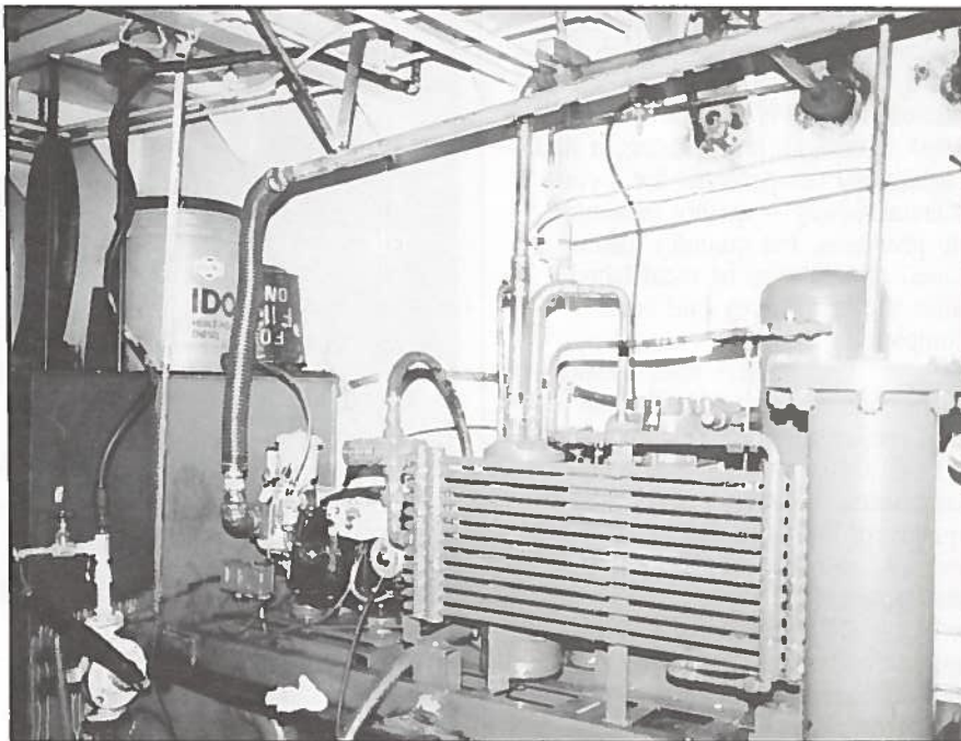
Plate Coil Refrigeration System
