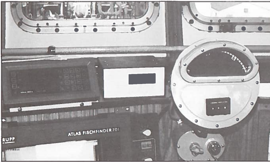
Fuel rack sensor — bridge control panel (above); engine room component (below)
