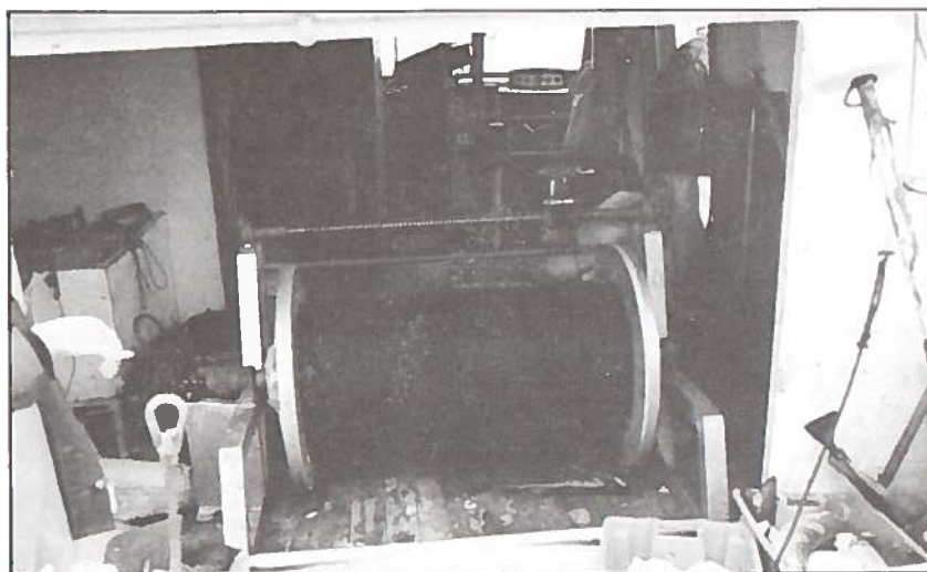
Halibut Longline aboard the "Cassie IV" using the Snap-on Drum
