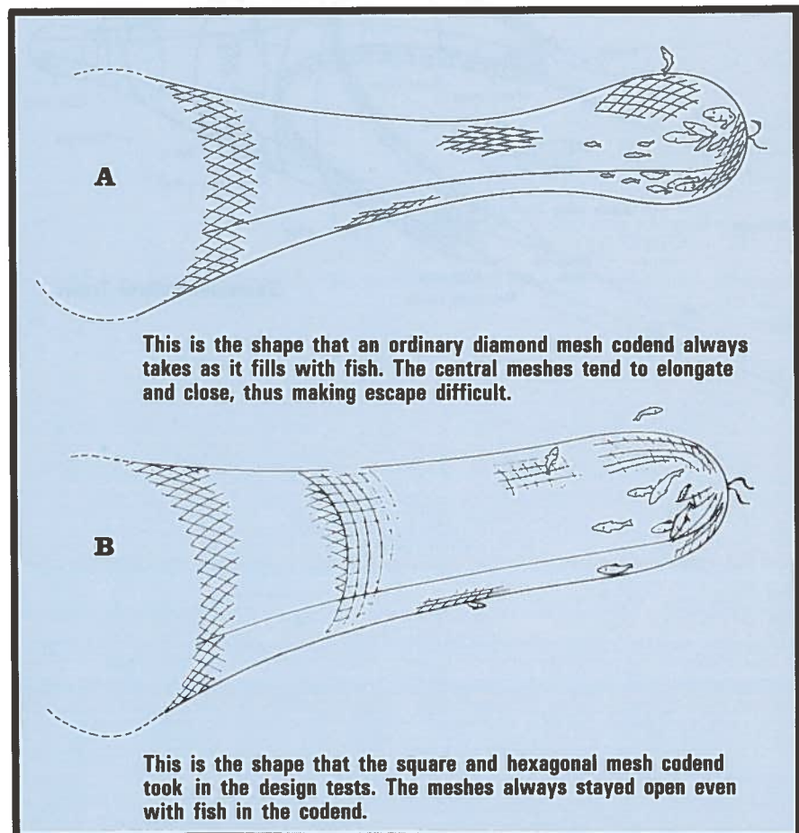
Square mesh codend
