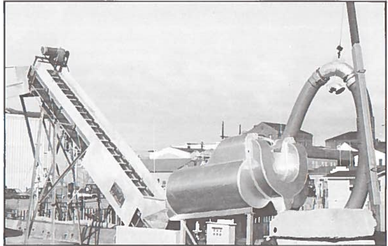
Transvaac herring pump original model 1010, forerunner of the 2020
