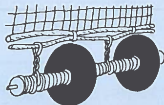
Toggle chains with Lancaster false fishing line through chains. Rockhopper discs tied to false fishing line
