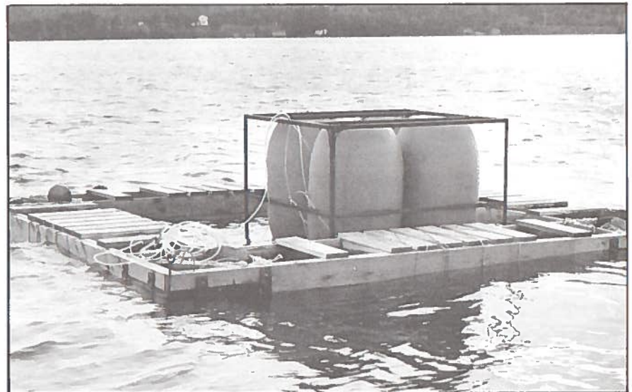
Prototype Rafts designed, constructed and evaluated for AFDP, Scotia Fundy Region by the Technical University of Nova Scotia.
