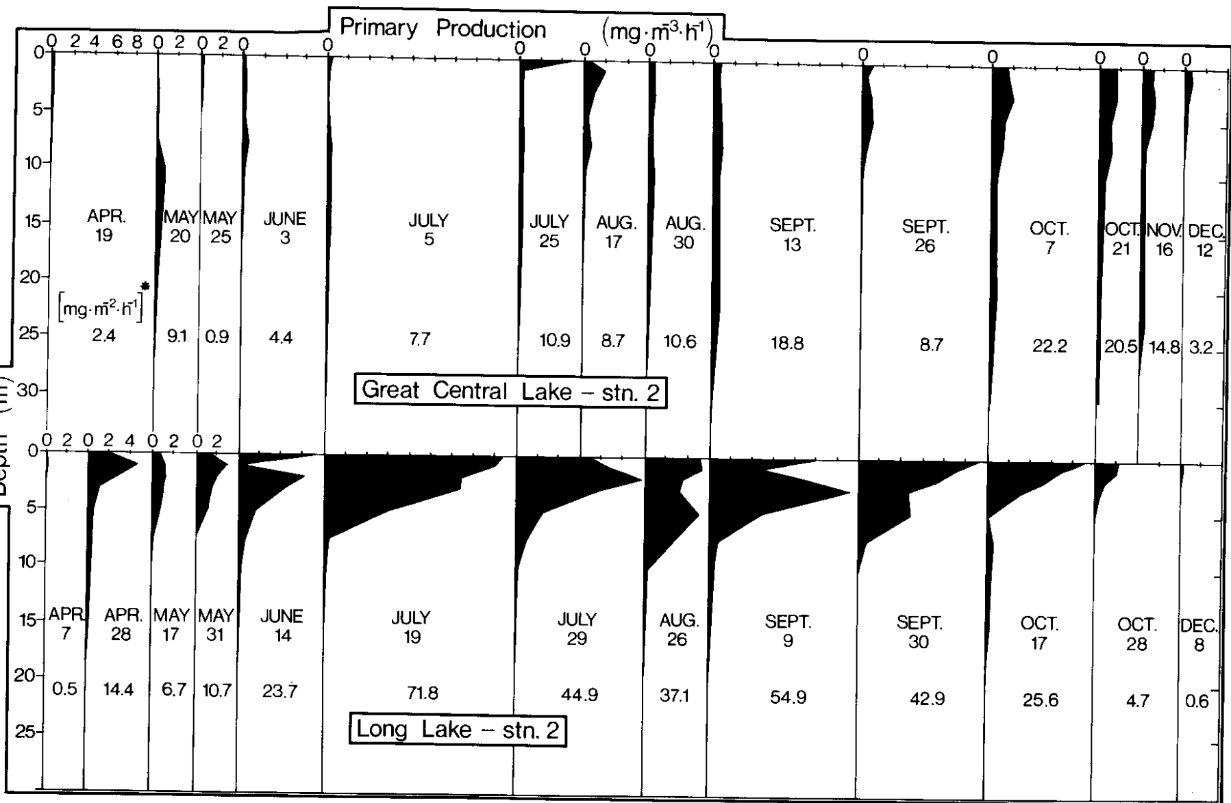
Figure 16. Annual primary production vs. depth profile and integrated values of production of Great Central Lake (Station 2) and Long Lake (Station 2) in 1978.
