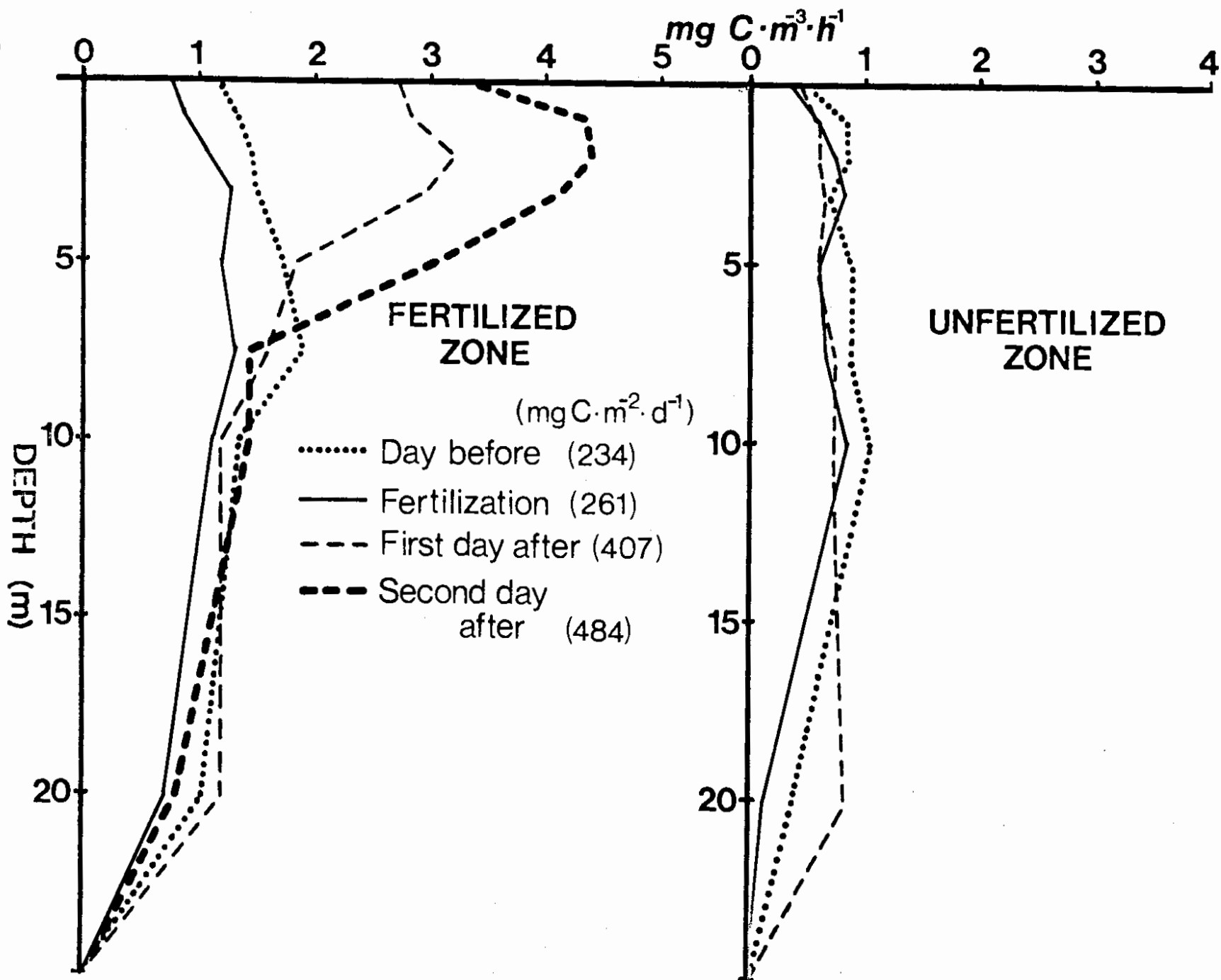
Figure 13. Carbon uptake vs depth profile in the fertilized and unfertilized zones of Great Central Lake on the day before fertilization, day of fertilization and on the first and second days after fertilization.
