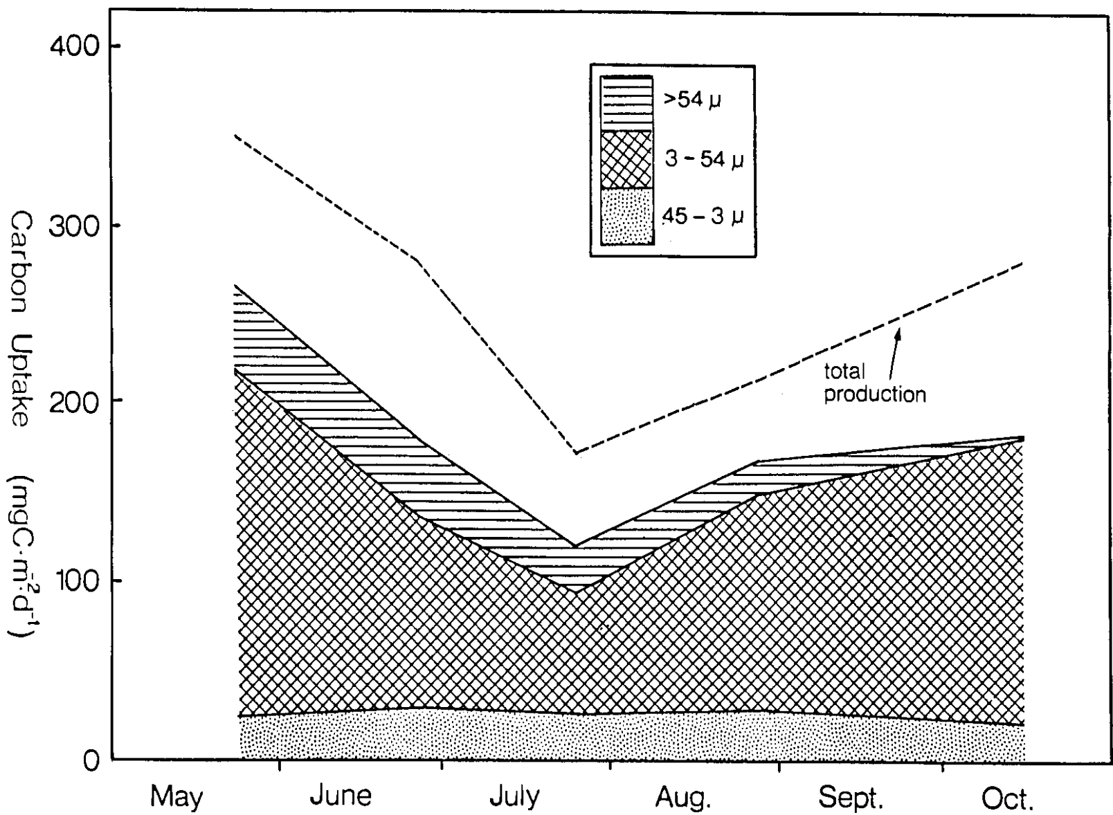
Figure 14. Mean carbon uptake values (mg C·m -2 ·d -1 ) of ultraplankton, nanoplankton and net plankton. Total production measured separately (from Costella et al. 1979).
