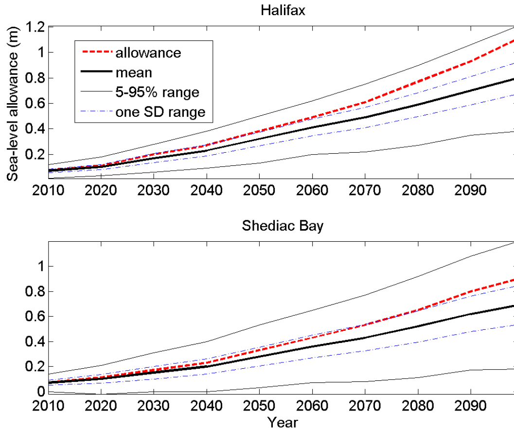
Figure 2: Time evolution of sea-level allowances and projections for RCP8.5 for (top) Halifax and (bottom) Shediac Bay. Thick red dashed line indicates sea-level allowances. Thick solid line, thin solid lines, and thin dash-dotted lines indicate the mean, the 5-95% percentile range, and the mean- 0.5 \times \text{SD} to mean+ 0.5 \times \text{SD} range of relative sea-level projections for RCP8.5 respectively.
