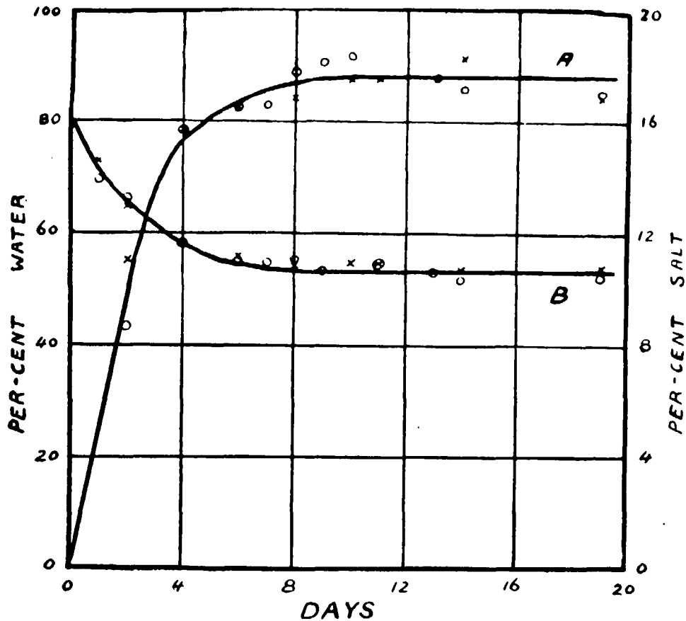
Fig. 1. Dehydration and Salt Penetration Curves.
