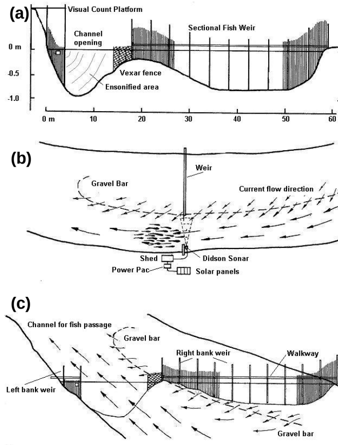
Figure 2. River cross-section and measured bottom profile (a), plan view (b) and current flow pattern (c) at the DIDSON acoustic site on the Horsefly River in 2005. These diagrams illustrate the equipment configuration relative to water flow patterns and the spatial pattern of fish movement upstream. The handrails for the sectional weirs are not shown. Note that the vertical conduit dowels and poles are not drawn to scale.
