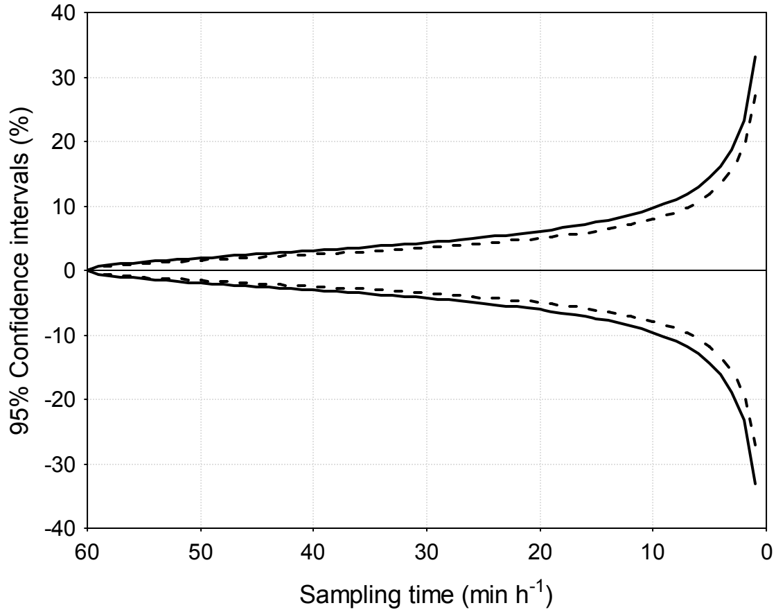
Figure 12. The relationship between the length of time sampled and the resulting 95% confidence limits in per cent for temporal sub-sampling. The solid black line represents confidence intervals when the counts from the first 10 minutes are used and the dashed line represents the confidence intervals when the second 10 minutes are used.
