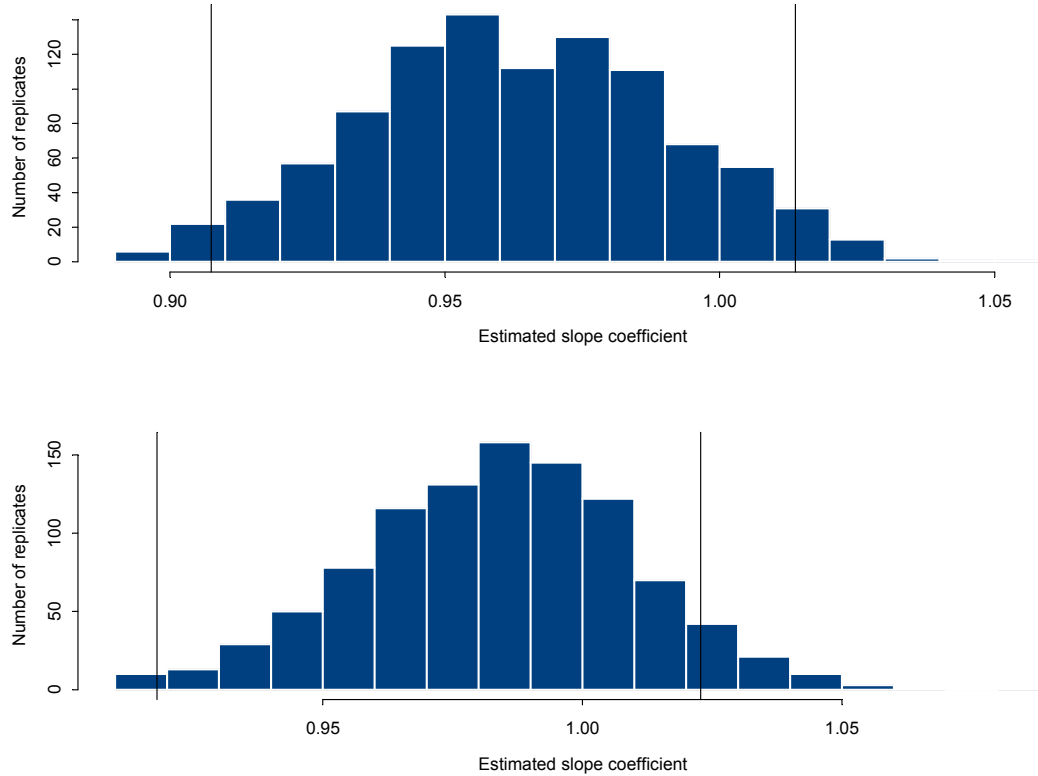
Figure 9. Distribution of boot-strapped estimates of slope coefficients for DIDSON vs. visual and visual vs. DIDSON regressions in Figure 8, based on 1000 replicates. The top histogram assumes that all of the error is in the DIDSON counts and the bottom histogram assumes that all the error is in the visual counts. The vertical lines represent the 95% confidence intervals.
