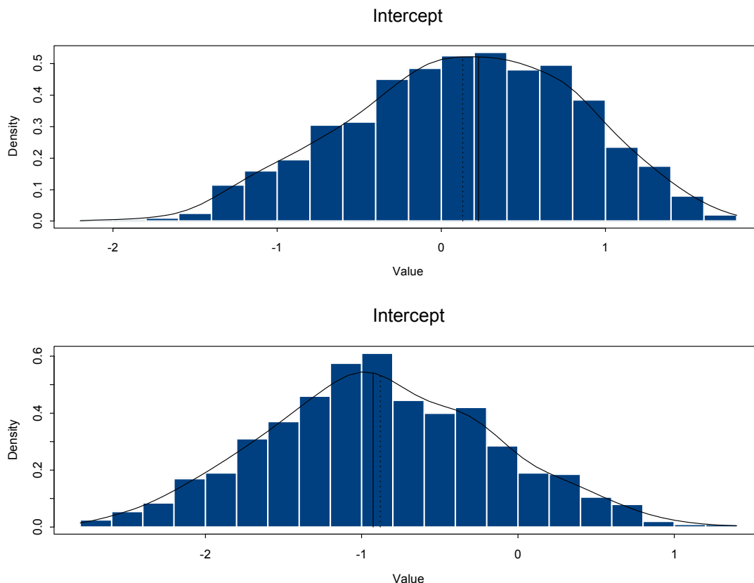
Figure 10. Distribution of boot-strapped estimates of Y-intercept values for DIDSON vs. visual and visual vs. DIDSON regressions in Figure 8, based on 1000 replicates. The top histogram assumes that all of the error is in the DIDSON counts and the bottom histogram assumes that all the error is in the visual counts. The solid vertical lines indicate the observed intercept values for the original data, and the dotted vertical lines indicate the means of the replicates. The difference between these two lines is the estimated bias.
