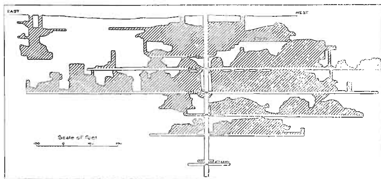
Figure 2. Longitudinal section of the workings on the fissure vein at the Micmac mine, Leipsigate.
