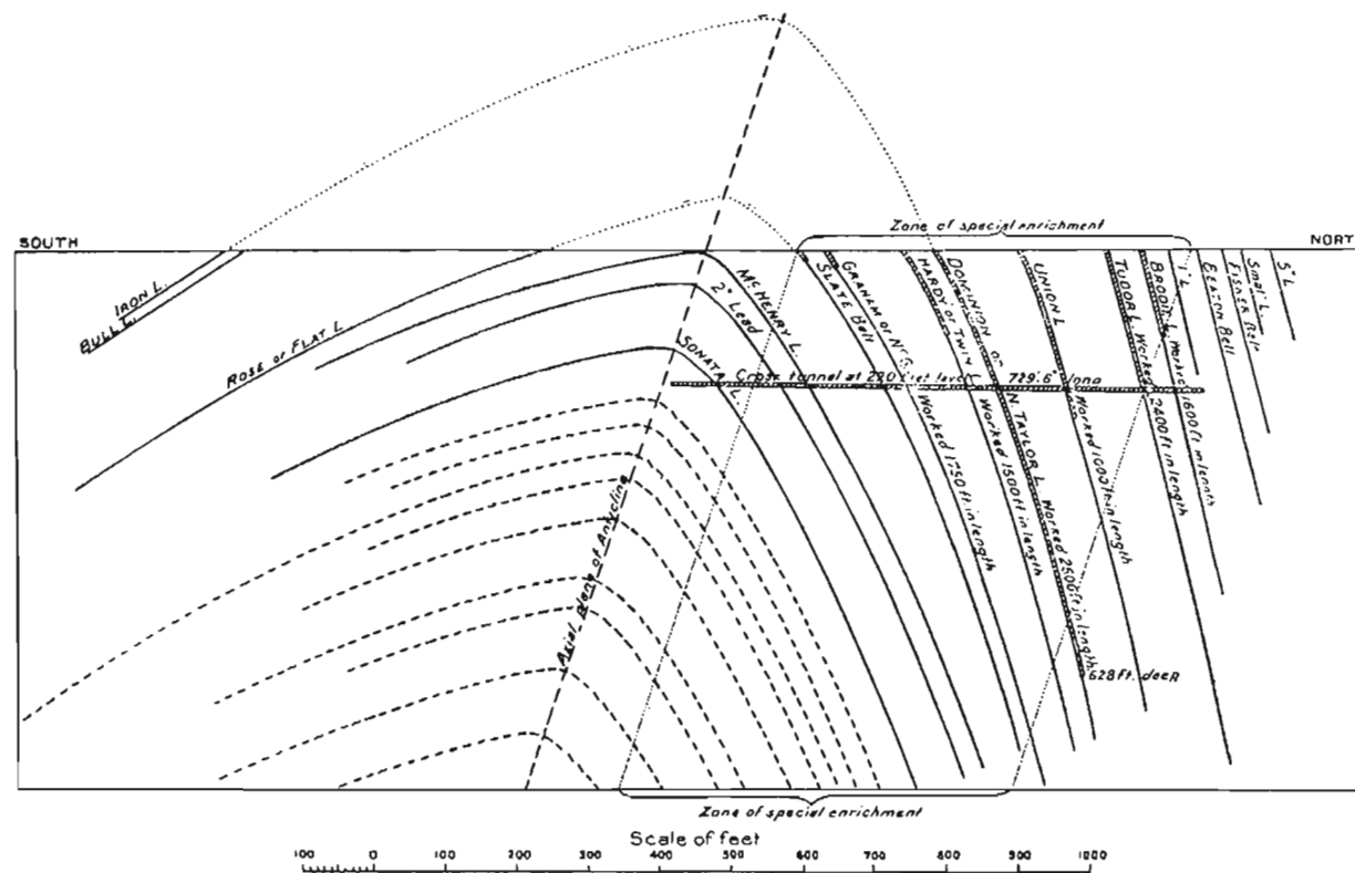
Figure 10. Section across anticlinal fold on Tudor mine, Waverley gold district.
