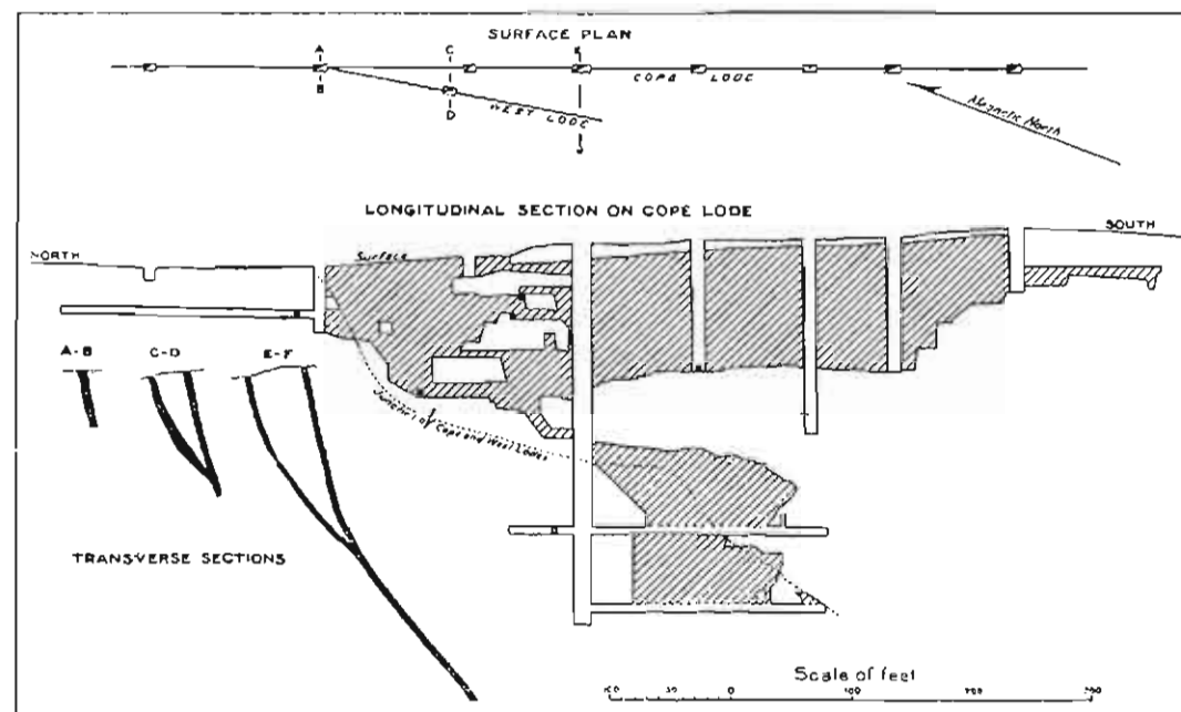
Figure 1. Workings on Cape and West lodes, Central Rawdon.
