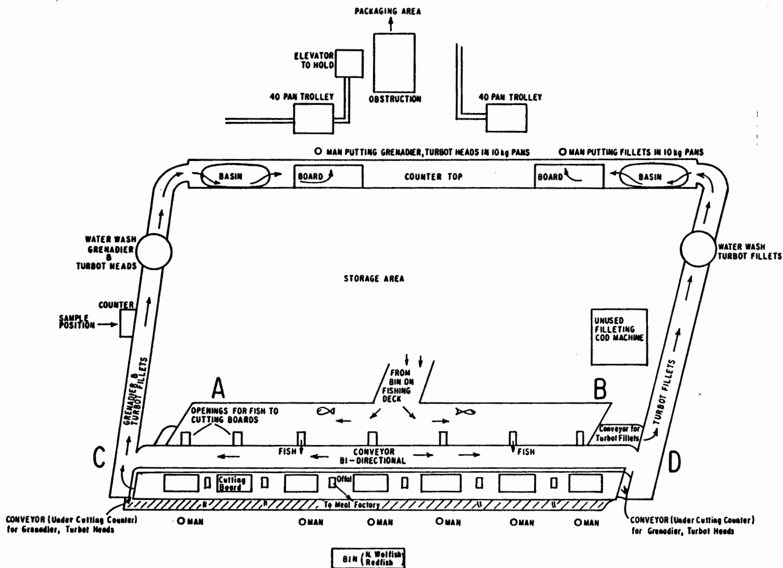
Fig. 2. Layout of the processing area on the Kuprin, showing possible sampling positions: A, B, C, D.
