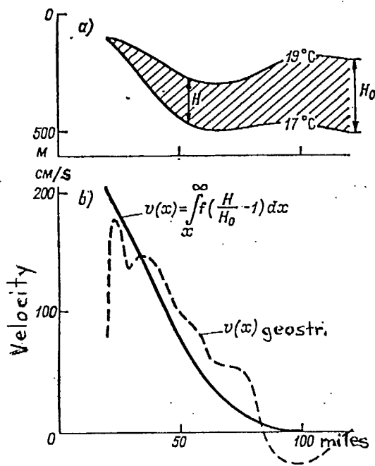
Fig. 2.33. Analysis of vorticity in a cross-section of the Gulf Stream in the vicinity of 39^{\circ}40' \text{ N} and 79^{\circ} \text{ W} , after Stommel [237]
