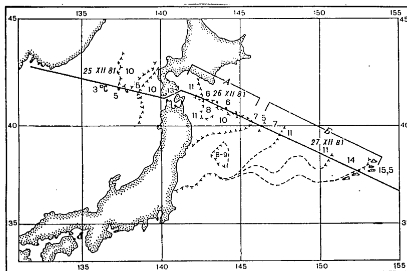
Fig. 4.1. Thermal structure of the ocean surface, reproduced on the basis of temperature measurements and an IR image from a NOAA satellite
