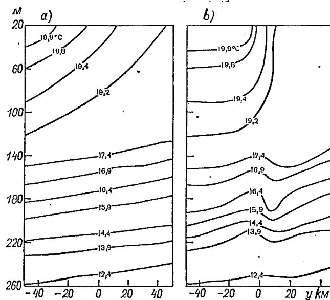
Fig. 2.26. Temperature distribution in the upper 250-m layer of the ocean a - for t=0 , b - for t=240 hrs (variable stratification)
