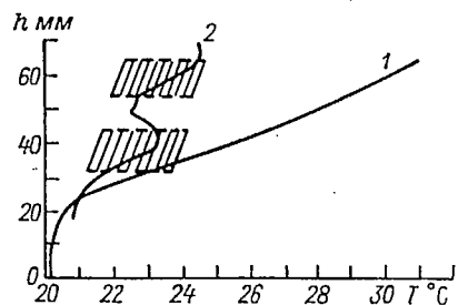
Fig. 4.10. Vertical temperature profile across the lower part of an intrusion in an experimental tank (1st experiment)
