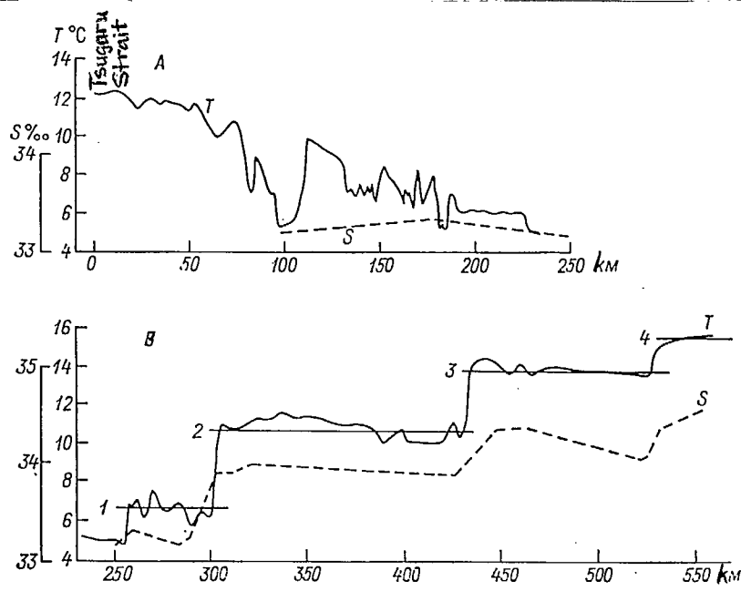
Fig. 4.2. Temperature distribution in an area intersecting the zone of convergence of the Kuroshio-Kurile Current
