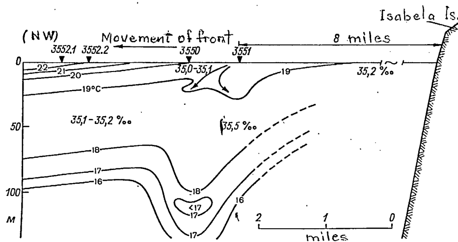
Fig. 2.19. An example of overturning when cold waters override warm waters in the area where the Cromwell Current comes to the surface near Isabel Is. (Galapagos Islands)
