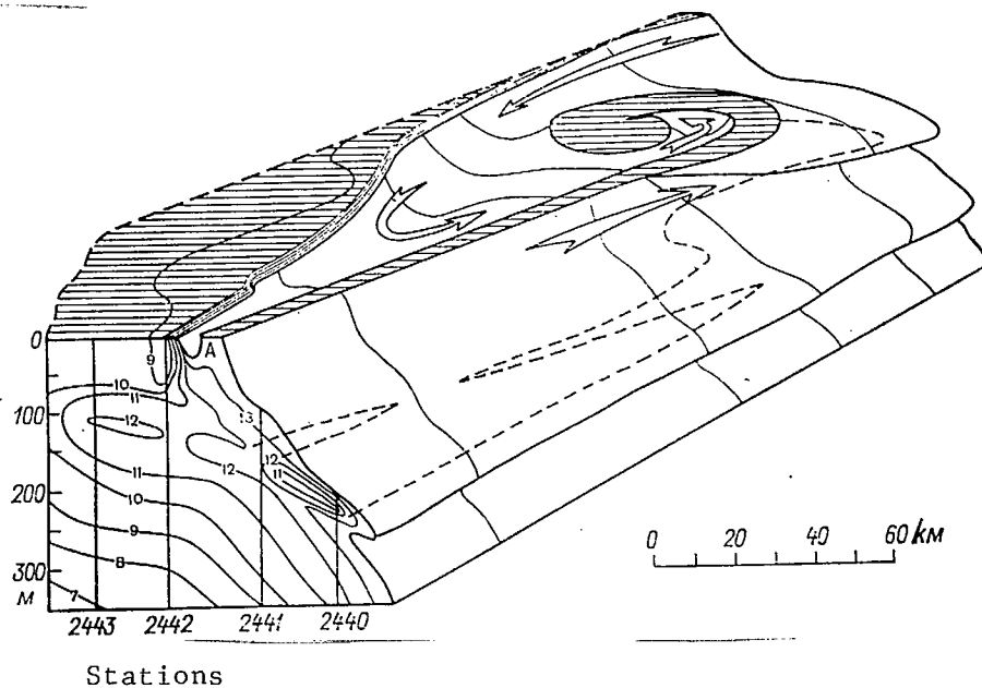
Fig. 4.17. Hypothetical depiction of the three-dimensional fine structure of the frontal zone of the Gulf Stream in the vicinity of a cold entrainment and cyclonic eddy
