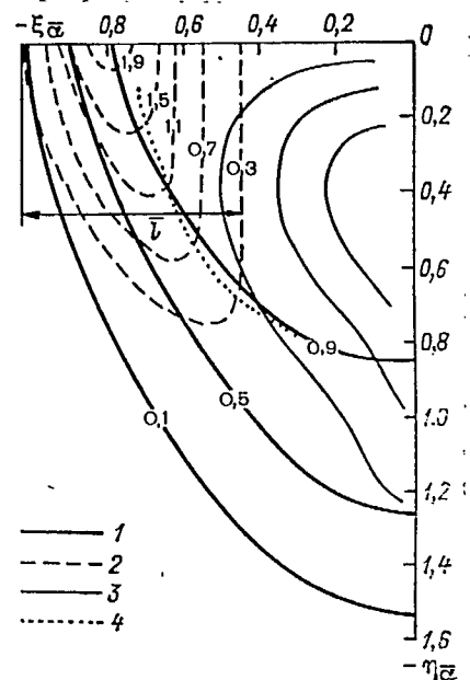
Fig. 2.36. Quasi-stationary structure of a frontal interface in cross-section with E=0.025 (the same for all \tilde{R}_0 ), based on Kao's model data [156]
