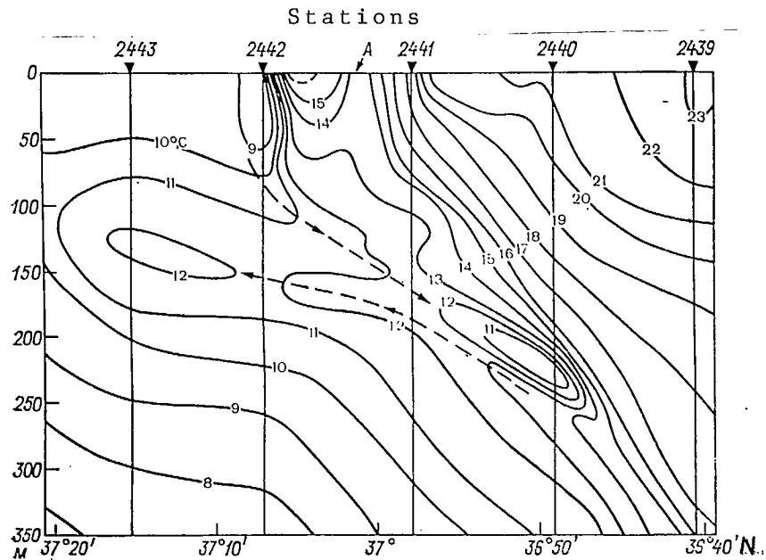
Fig. 4.15. Temperature distribution at a profile across the frontal zone of the Gulf Stream
