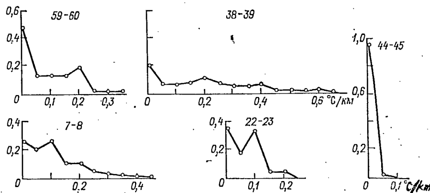
Fig. 2.6. Histograms of horizontal temperature gradients for individual recorded segments in the Indian Ocean. Histograms calculated with a step of 0.05^{\circ}\text{C}/\text{km} (numbering of segments the same)
