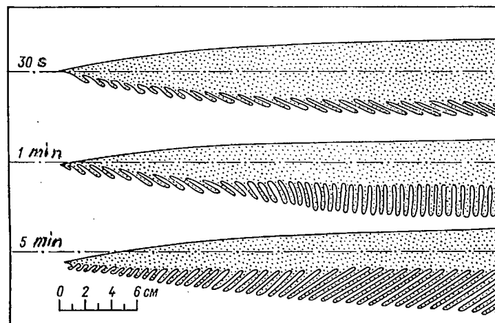
Fig. 4.8. A sketch of the development of a convection in the form of salt fingers at the lower boundary of an intrusive layer in the first experiment
