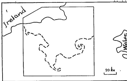
Fig. 3.9. Hooked form of the warm manifestations of cyclonic eddies on IR images of the front (dashed line) in the Irish Sea (NOAA-5 satellite) on 3 September 1976, based on the data of [208]. Thin solid lines show outer contour of IR image.
