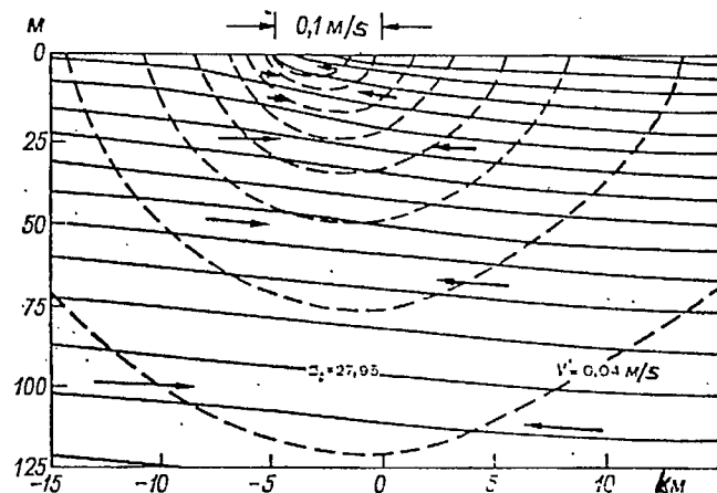
Fig. 2.28. Result (from [178]) of the frontogenetic deformation of an initially weak baroclinic zone after 57 and 76 hrs with D = 10^{-5} \text{ s}^{-1}
