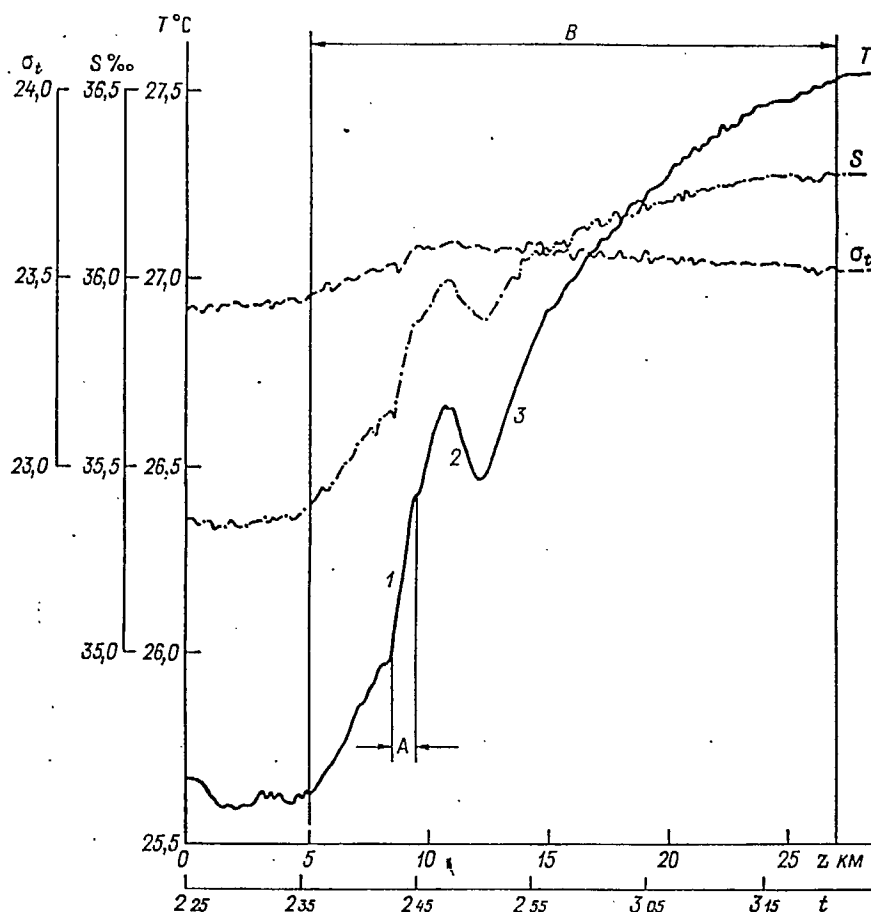
Fig. 2.18. An example of the crossing of a frontal zone in which several frontal interfaces (1, 2, 3) are observed. The actual width of one of the fronts is marked by the letter A. The total width of the zone (B) exceeds 20 km. These data were collected by the author during the 25th trip of the "Akademik Kurchatov" research vessel in the Sargasso Sea on 14 Sept 1977. The frontal zone presumably bounds the cold wake of the tropical cyclone "Clara" from the south. The cyclone passed through this area a day before the vessel.
