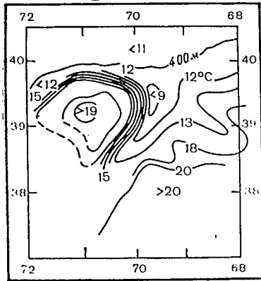
Fig. 3.5. Flow of cold water along the eastern periphery of an anticyclonic ("warm") ring north of the Gulf Stream, based on the results of an aerial survey carried out by Saunders [224] with the help of an IR radiometer and aerial expendable bathythermographs (AXBT) on 4 December 1969
