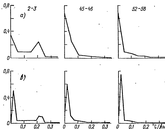
Fig. 2.5. Histograms of horizontal temperature gradients for individual recorded segments in the Pacific Ocean: a - with a step of 0.05^{\circ}\text{C}/\text{km} , b - with a step of 0.02^{\circ}\text{C}/\text{km} (numbering of segments the same)
