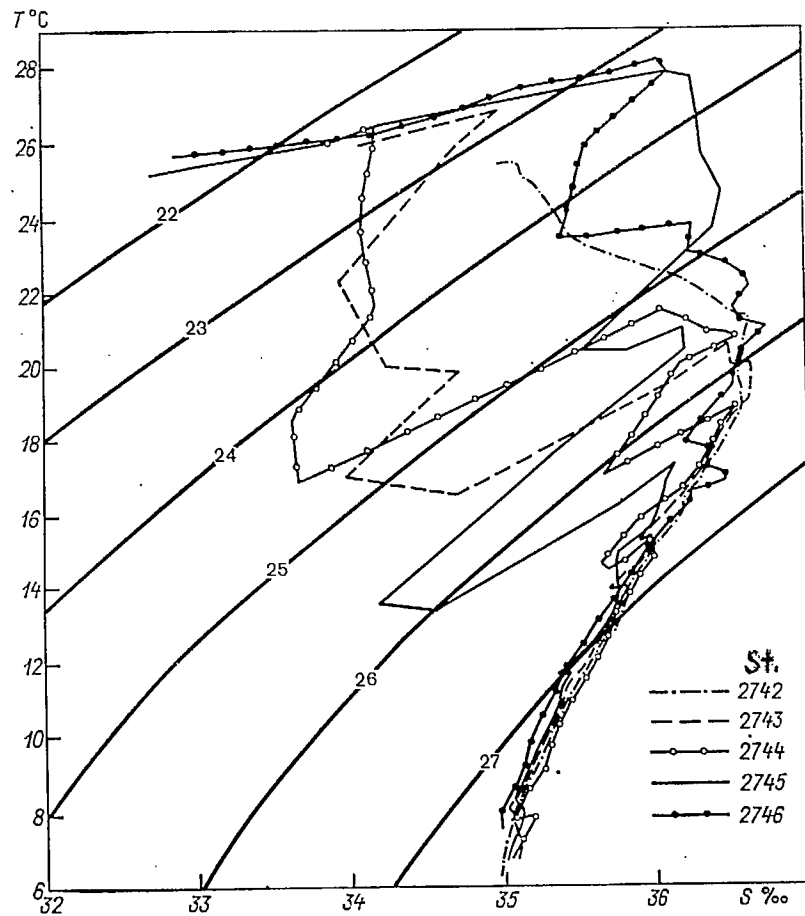
Fig. 3.20. T, S-curves for stations No. 2742—2746
