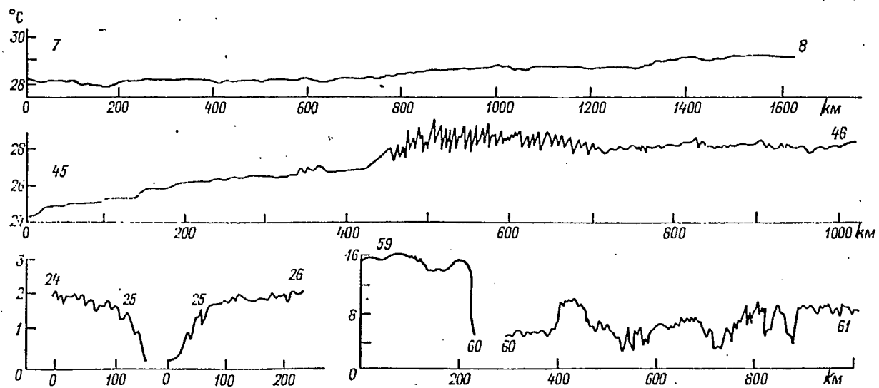
Fig. 2.3. Examples of temperature changes in the surface layer of water along individual recorded segments in the Pacific Ocean. The numbers near the curves correspond to the numbers in fig. 2.1
