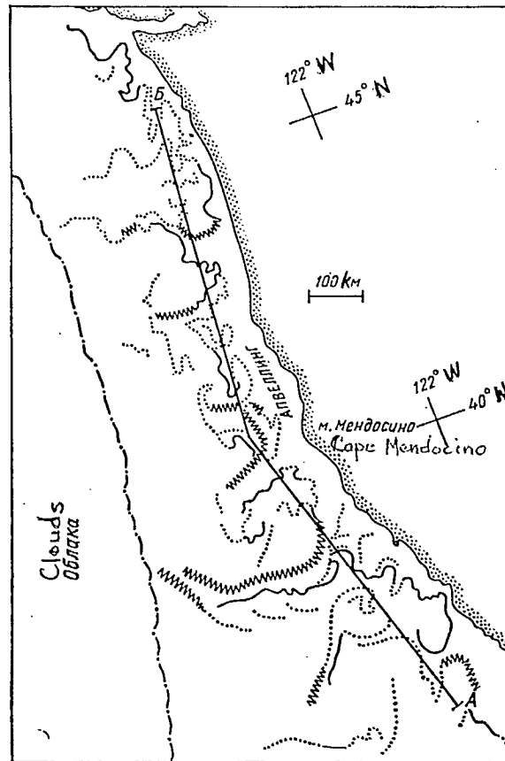
Fig. 2.7. Example of an analysis of the position of thermal fronts on the basis of an IR image of the frontal zone of the Oregon upwelling, obtained from the American satellite NOAA-5 [195]
