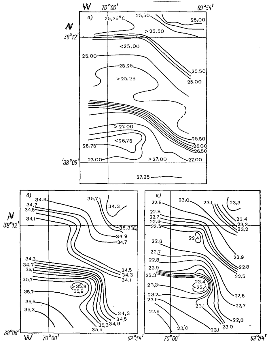
Fig. 3.15. Distribution of temperature (a), salinity (b) and density (c) at the 3 m level in the frontal zone of the warm ring of the Gulf Stream
