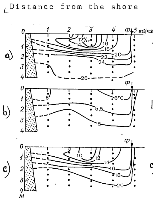
Fig. 3.33. Distribution of salinity (a), temperature (b) and nominal specific density (c) in the drainage lens of the Connecticut R., based on Garvine's data [126]
