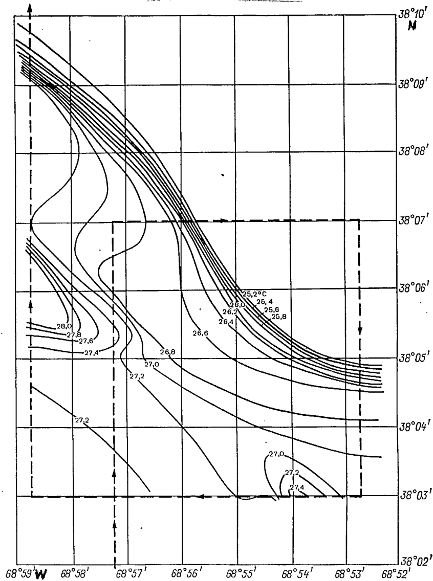
Fig. 3.12. Temperature distribution in the surface layer of the ocean in the frontal zone near the northern boundary of the Gulf Stream on 5 September 1978, based on the data of a towed temperature sensor ( z=0.15 m)
