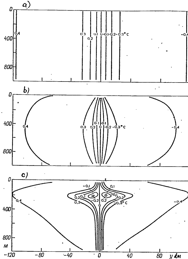
Fig. 2.24. Isolines of the field of temperature deviations from the mean state in the ocean
