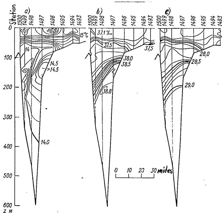
Fig. 4.7. Sections in the field of temperature (a), salinity (b) and nominal specific density (c) across the narrowest part of the Strait of Sicily, executed by the author with the help of an AIST STD probe on 13-14 April 1974 during the 18th trip of the "Akademik Kurchatov" research vessel
