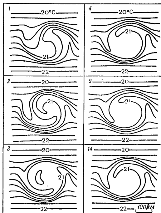
Fig. 3.3. Temperature maps of ocean surface in the case of a stationary cyclonic eddy. Figures in top corner - day of integration. Diagram borrowed from [47]
