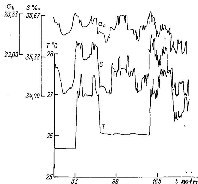
Fig. 3.16. Changes in temperature, salinity and density on the perpendicular tacks of the vessel during maneuvering in the frontal zone of the warm ring of the Gulf Stream, obtained with the help of an AIST probe in a flow-through system on 11 September 1978 between 01 h 47 min and 05 h 18 min (ship time)
