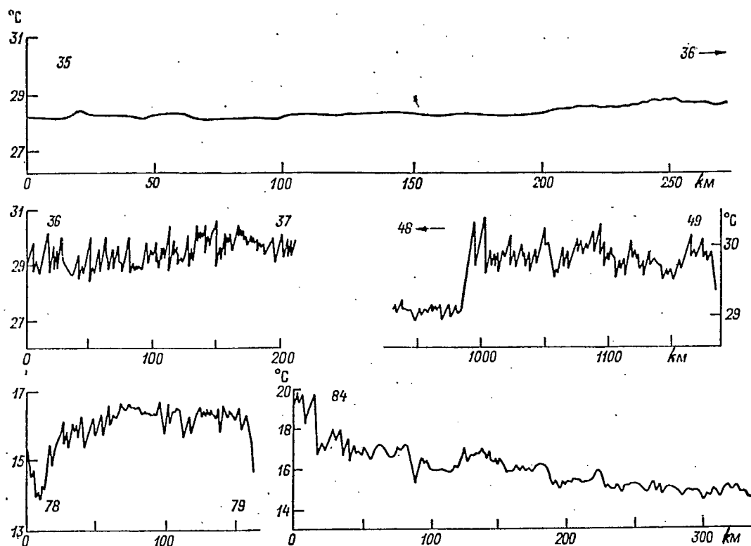
Fig. 2.4. Examples of temperature changes in the surface layer of water along individual recorded segments in the Indian Ocean and adjacent seas. The numbers near the curves correspond to the numbers in fig. 2.2
