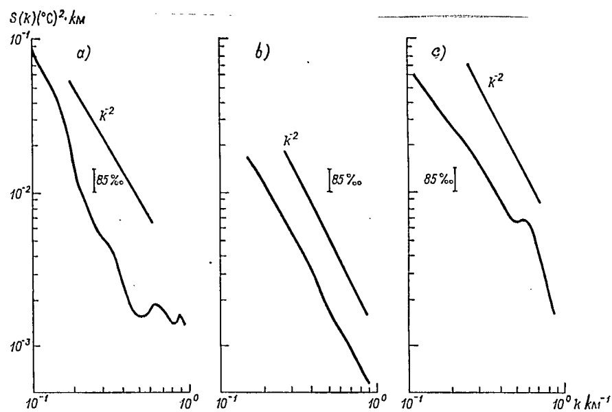
Fig. 3.45. Examples of spectra of temperature fluctuations for entry No. 1 (a), No. 3 (b) and No. 5 (c) (see table 3.6)
