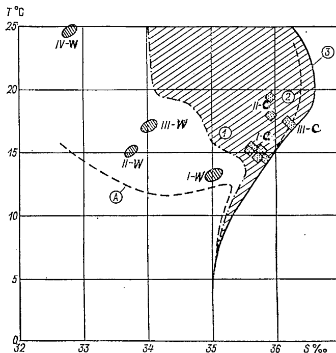
Fig. 3.26. Position of intrusion-related temperature inversions on a general T, S-diagram of waters in the Gulf Stream area
