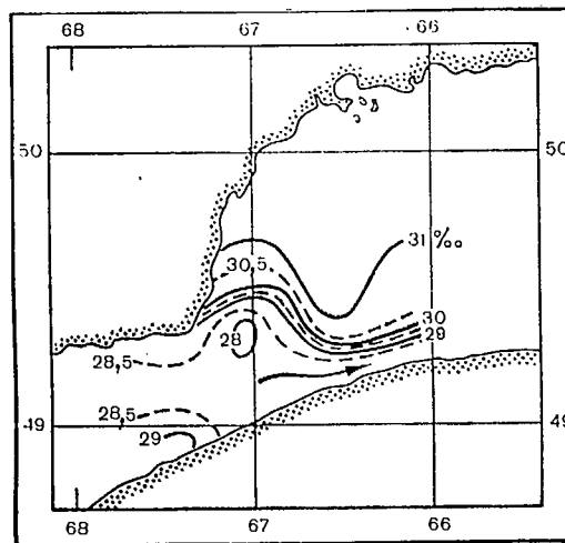
Fig. 3.37. Salinity distribution (in ‰) in the Gulf of St. Lawrence (based on [243])
