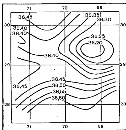
Fig. 2.16. Distribution of salinity (%) near the surface in the Sargasso Sea on 18-26th of July 1977
