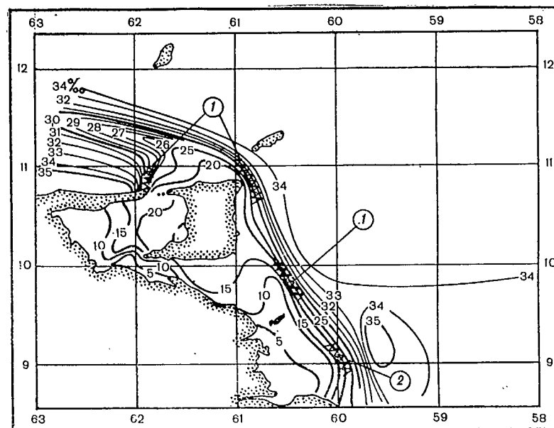
Fig. 3.32. Salinity distribution at the ocean surface in the drainage lens of the Orinoco R., based on [123]
