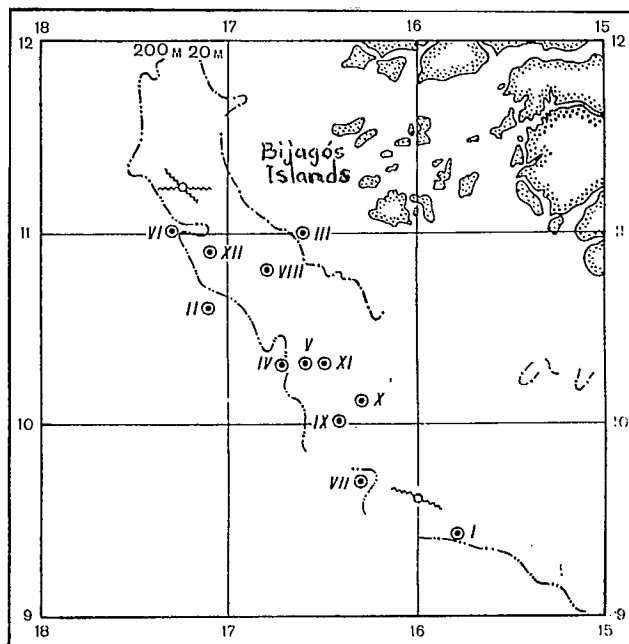
Fig. 3.27. Average monthly positions of the points at which rips and overfalls are most frequently observed near the coast between 9^{\circ} and 12^{\circ} N, based on [226]
