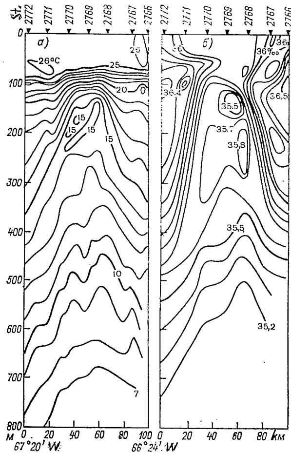
Fig. 3.21. Section across the dome of a cold ring along 35° N a - temperature, °C; b - salinity, ‰
