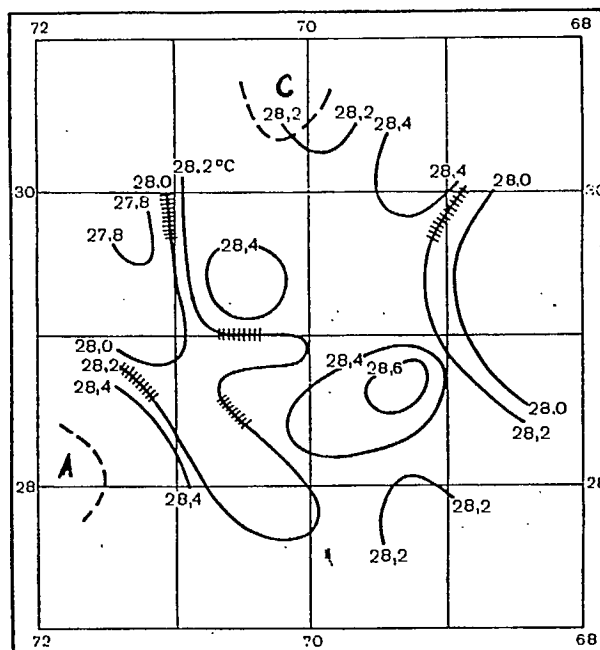
Fig. 2.8. Distribution of temperature at the 10 m level on the polygon of the POLYMODE experiment on 18-29th of September 1977
