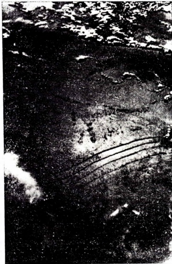
Fig. 3.40. Photographic depiction of solitons in the Andaman Sea, obtained in the Soviet-American "Soyuz-Apollo" experiment [200]
