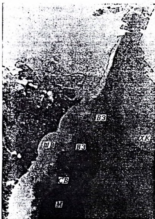
Fig. 1.3. IR image of the frontal zone of the Gulf Stream from the Florida peninsula to Cape Lookout, obtained on 1 April 1974 with the help of ultra-high-resolution (1 km) IR radiometry from the American satellite NOAA-3. The three main gradations of tonalities correspond to the shelf waters (MB - the lightest, 8-10°C), the slope waters (CB - of intermediate tone, 12-18°C) and the waters of the Gulf Stream (the darkest, 20-22°C). At this time of the year, the waters of the Sargasso Sea (on the right) are considerably colder than the waters of the Gulf Stream, and are characterized by intermediate tonality (18-19°C). The abundance and complex distribution of the frontal temperature contrasts between these gradations are noted. We can clearly see spiral eddies (B3) on the left side of the Gulf Stream (see subsection 3.1.2), a meander (M) and a cold cyclonic ring (XK) on the right (see subsection 3.1.3). The dotted line indicates the approximate position of the boundary of stratified cloudiness. The above image was kindly made available to the author by R. Legekis* (NOAA)
