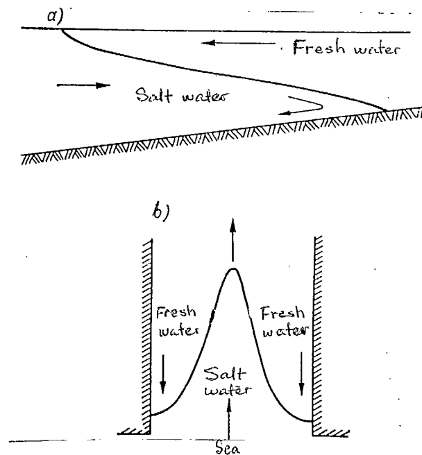
Fig. 3.36. Salt wedge in the vertical axial plane of an estuary (a) and in the horizontal plane at the mouth of a small river (b)
