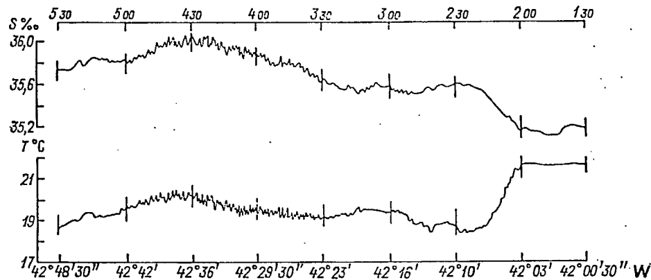
Fig. 2.14. An example of how a negative T, S-correlation changed to a positive correlation at the 3 m level along a section at 23^{\circ}04' S lat in the vicinity of Cabo Frio (Brazil upwelling), based on the data of Ikeda et al. [152]
