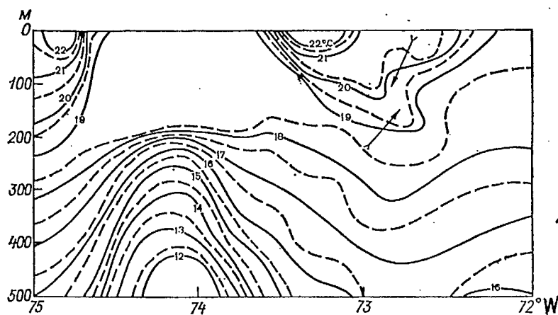
Fig. 2.27. Vertical section of temperature field in an eddy (based on the data of F.M. Vukovich [255])
