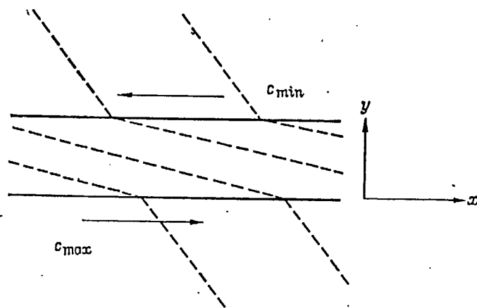
Fig. 2.23. Diagram demonstrating the increase in the horizontal gradient of the concentration of the scalar admixture c across a frontal interface under the effect of an along-frontal current with a velocity shear
