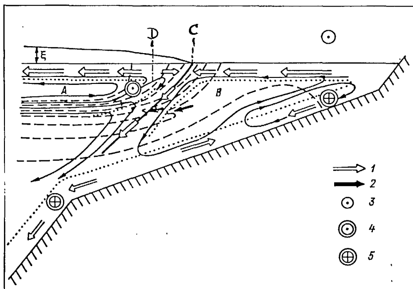
Fig. 2.38. A diagram of "two-cell" circulation in a coastal upwelling.
