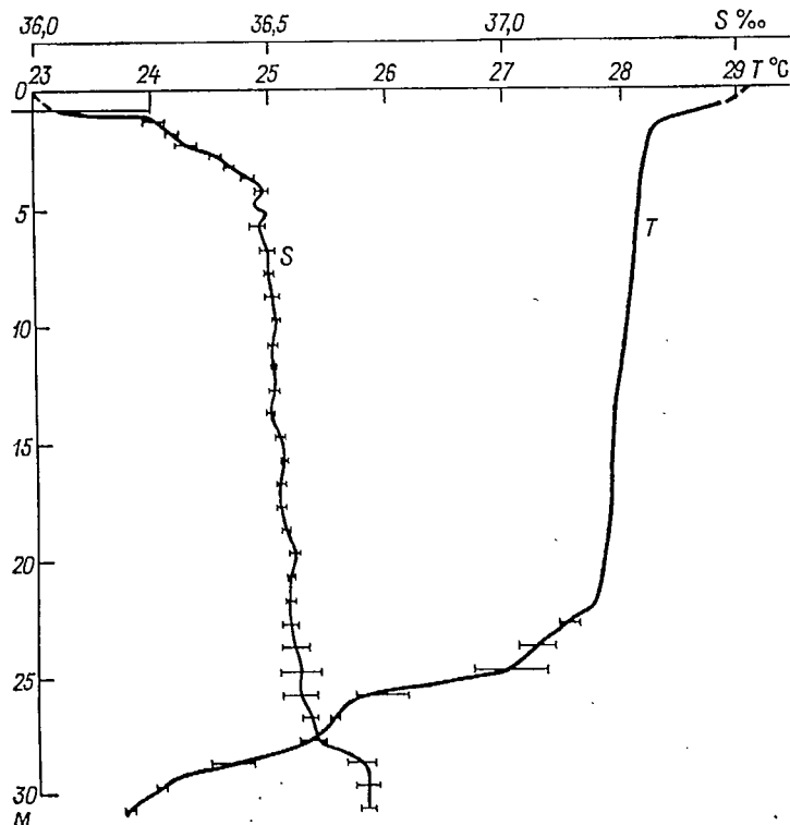
Fig. 3.47. Vertical temperature and salinity profiles recorded with an AIST probe in the Sargasso Sea in the afternoon hours of a calm day with intensive solar heating (15 h 00 min, 25 August 1978) after the freshening effect of a rainfall on the preceding days
