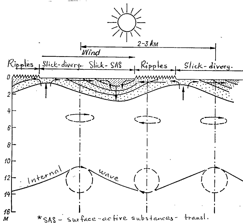
Fig. 3.41. Diagram of modulation of the thickness of a heated near-surface layer and the state of the sea surface by a periodic internal wave
