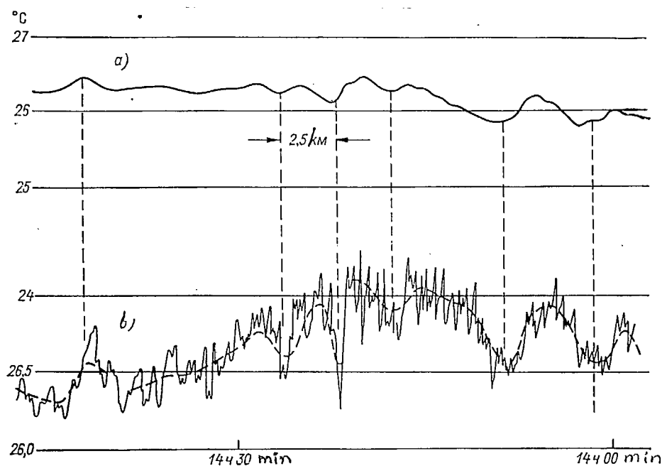
Fig. 3.43. Simultaneous recordings of thermal inhomogeneities of calm weather from a moving vessel
