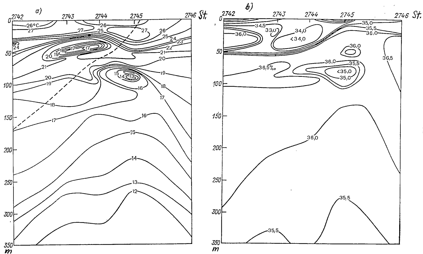
Fig. 3.18. Meridional section in the field of temperature (a) and salinity (b) across the southern periphery of a warm ring, based on the data of vertical probings with an AIST thermohaline probe Position of stations Nos. 2742-2746 shown in fig. 3.14.
