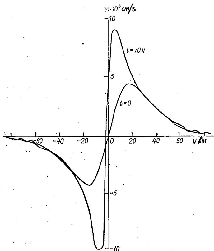
Fig. 2.32. Distribution of vertical velocity at the level z=20 m at t=0 and t=70 hrs
