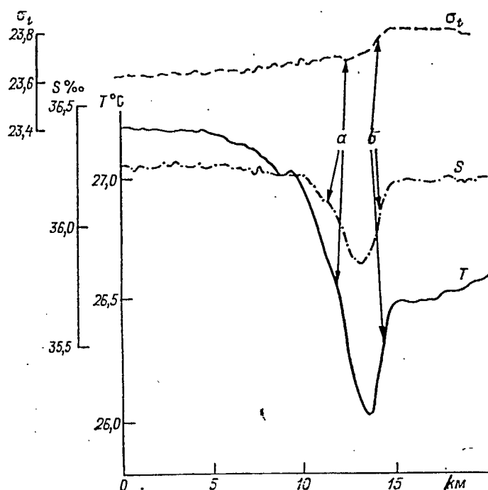
Fig. 2.9. Example of the recording of horizontal temperature (T) and salinity (S) gradients in the Sargasso Sea in September 1977 a - area without changes in density \sigma_t ; b - area with a small change in density \sigma_t due to the dominance of the salinity contribution
