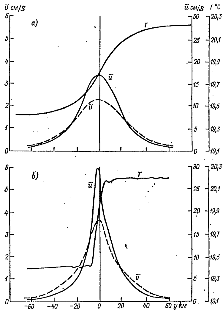
Fig. 2.31. Distribution of temperature \tilde{T} , and the along-frontal \tilde{u} and transverse \tilde{v} components of velocity at the level z=20 m
