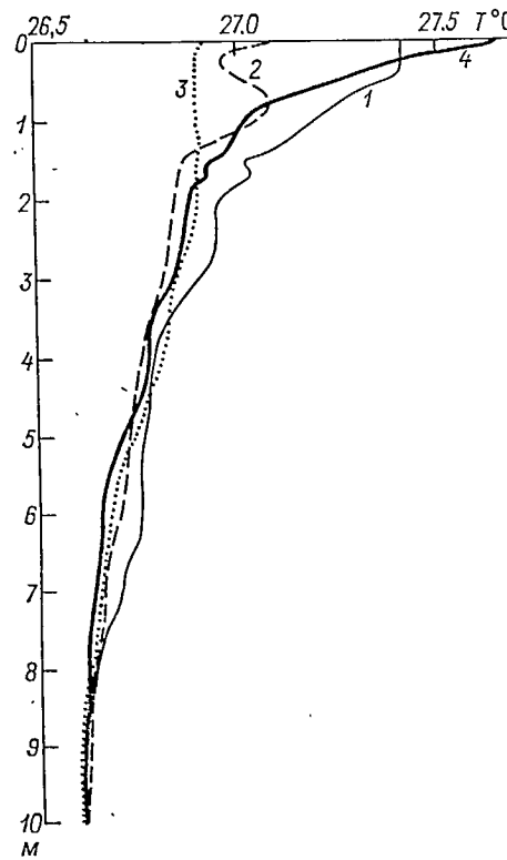
Fig. 3.46. Vertical temperature profiles obtained in calm weather in the Sargasso Sea on 25 September 1978 with the help of a surfacing probe during slight drifting of the survey vessel (not more than 0.5 knot)
