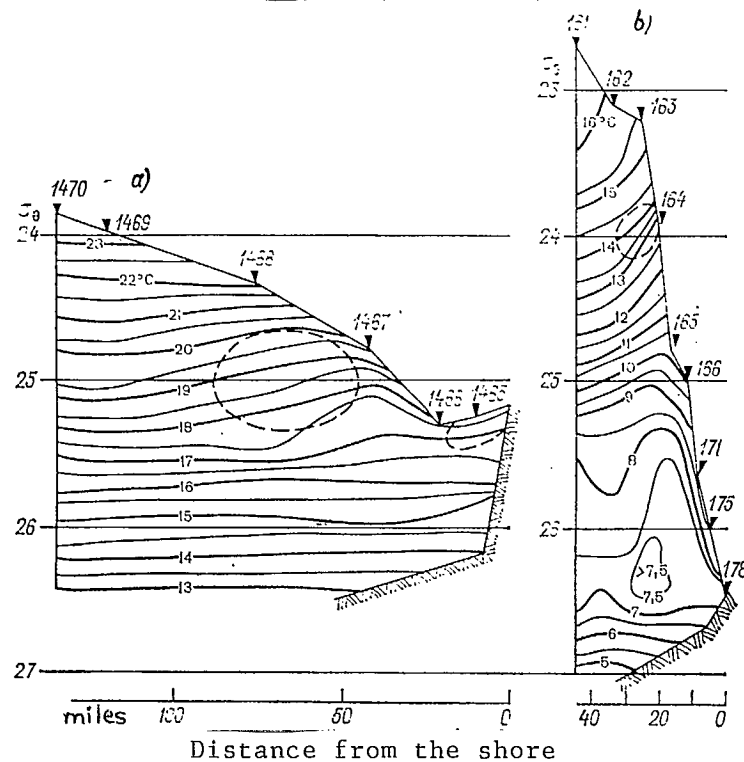
Fig. 3.30. Temperature distribution as a function of nominal potential density ( \sigma_\theta ) in the vicinity of the Peru upwelling (a) based on the author's data, and in the area of the Oregon upwelling (b) based on the data from [140]
