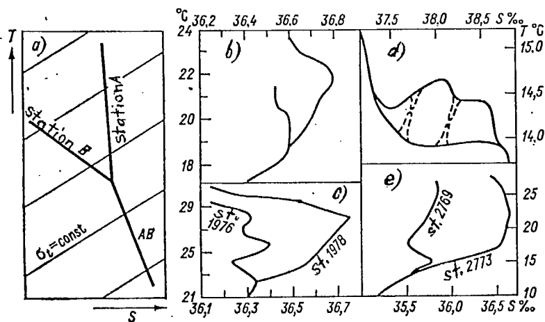
Fig. 2.20. Examples of the typical Y-form of a T, S-curve for pairs (or groups) of stations executed on different sides of a frontal interface
