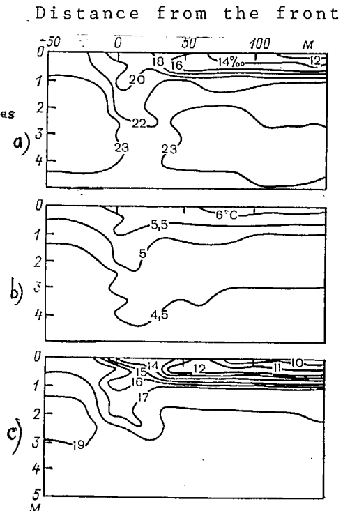
Fig. 3.34. Details of the distribution of salinity (a), temperature (b) and nominal specific density (c) near the frontal interface of the drainage lens of the Connecticut R., based on Garvine's data [126]
