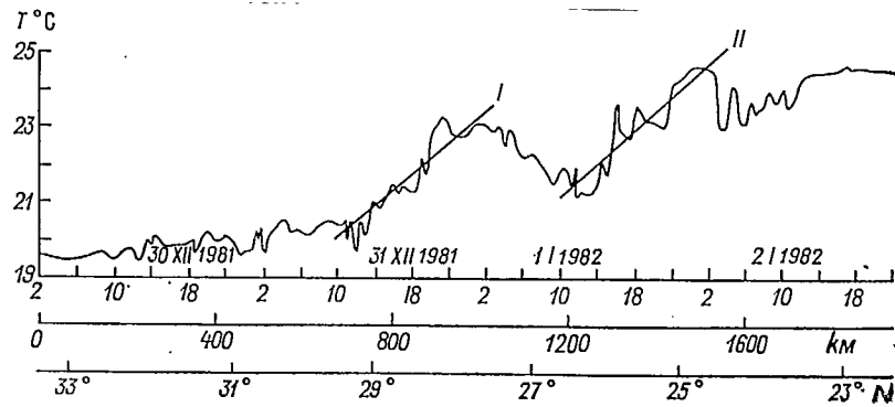
Fig. 4.3. Temperature distribution in the zone of the northern subtropical convergence (NSC)
