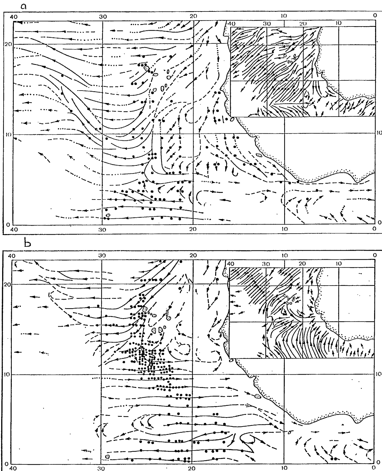
Fig. 1.1. Points at which navigators observed rip or overfall zones (black dots) in the area west of the African coast in January (a) and in August (b) from 1855 to 1900 (according to the data of A. Schumacher [226]).
