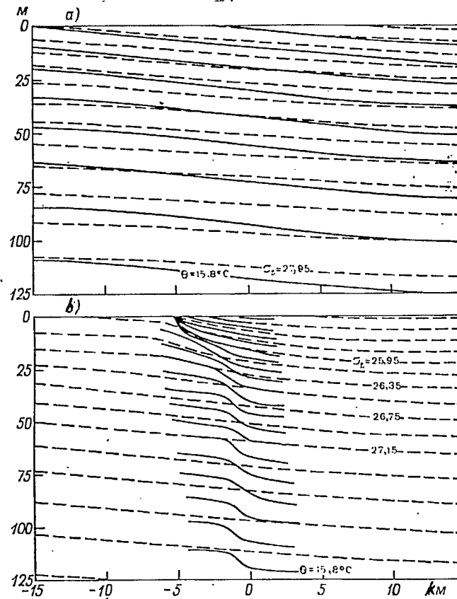
Fig. 2.29. Semi-geostrophic frontogenesis (based on [178]) in the baroclinic zone where density is determined not only by temperature, but also by salinity: isotherms (continuous lines across 0.8^{\circ}\text{C} ) intersect isopycnals (dashed line - across 0.2 units \sigma_t )
