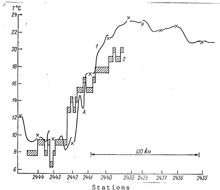
Fig. 4.14. Change in sea-surface temperature (SST) during the crossing of the Gulf Stream frontal zone on 20-21 March
