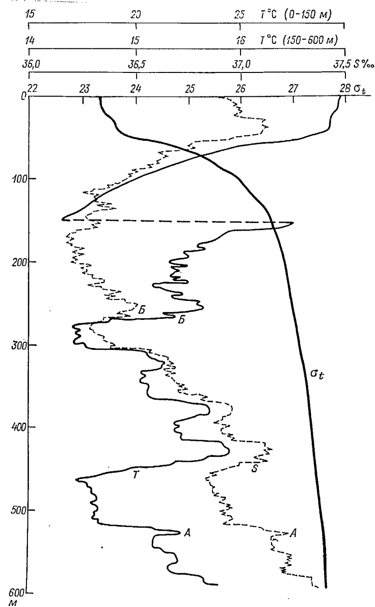
Fig. 4.5. Intrusive thermohaline structure in the 180-600 m layer in the Gulf of Aden, associated with the spreading of waters of Red Sea origin, at station No. 1984 of the 22nd expedition of the "Akademik Kurchatov" research vessel, 12^{\circ}09'42'' N and 44^{\circ}24'36'' E, 10 June 1976
