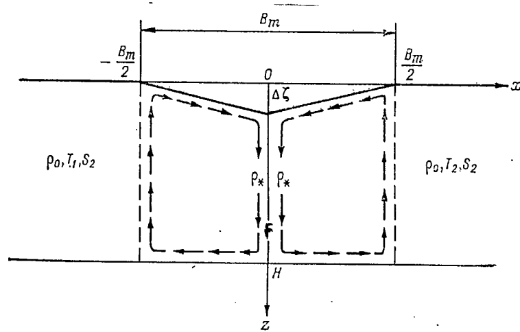
Fig. 4.18. Diagram of the decrease in level and motion in the zone of mixing near the frontal interface F .
