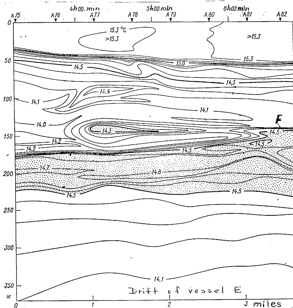
Fig. 4.6. Isolated warm-water lens of intrusive origin ( T > 14.5^{\circ}\text{C} ), separated from the frontal interface (F) in the Strait of Sicily (see fig. 4.7 and T, S-curve in fig. 2.20 d), based on the data of repeated sampling with an AIST probe on 2 May 1974 in the Strait of Sicily from a drifting vessel around 36^{\circ}37' \text{ N} and 12^{\circ}19' \text{ E} during the 18th expedition of the "Akademik Kurchatov" research vessel (station No. 1569)
