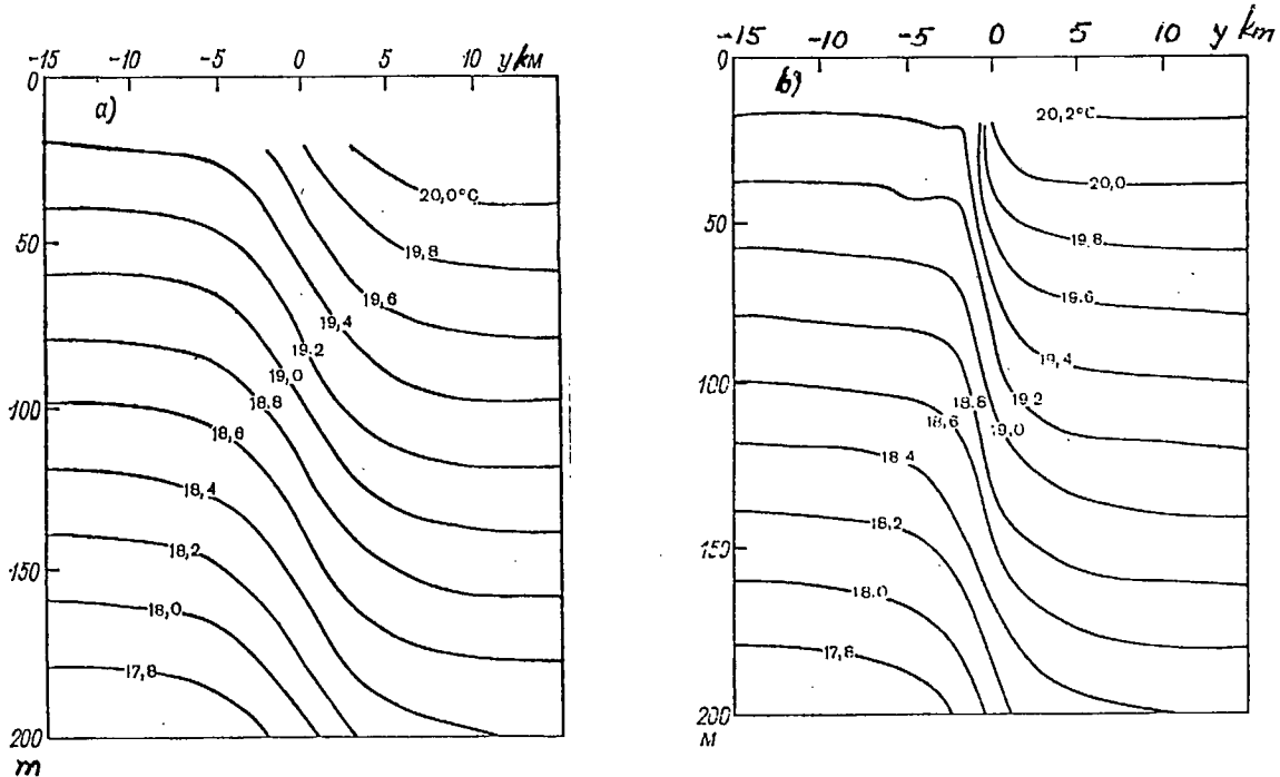
Fig. 2.30. Temperature distribution in the surface layer of the ocean a - at the initial moment ( t=0 ), b - at t=70 hrs
