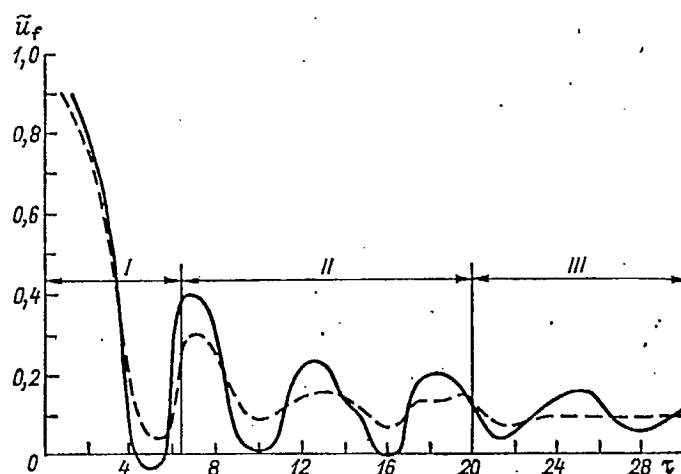
Fig. 2.34. Dependence of the dimensionless velocity of frontal migration \tilde{u}_f on the intensity of turbulent exchange, based on Kao's data [156]
