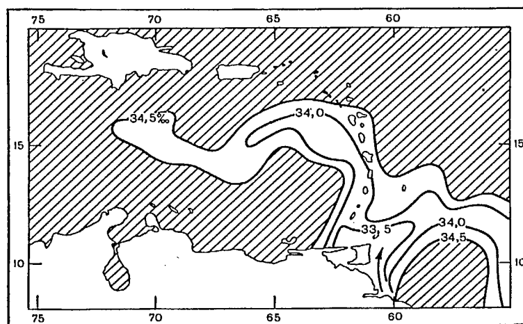
Fig. 2.17. Large-scale freshening effect of the Orinoco R., based on the data of G. Wüst [271]
