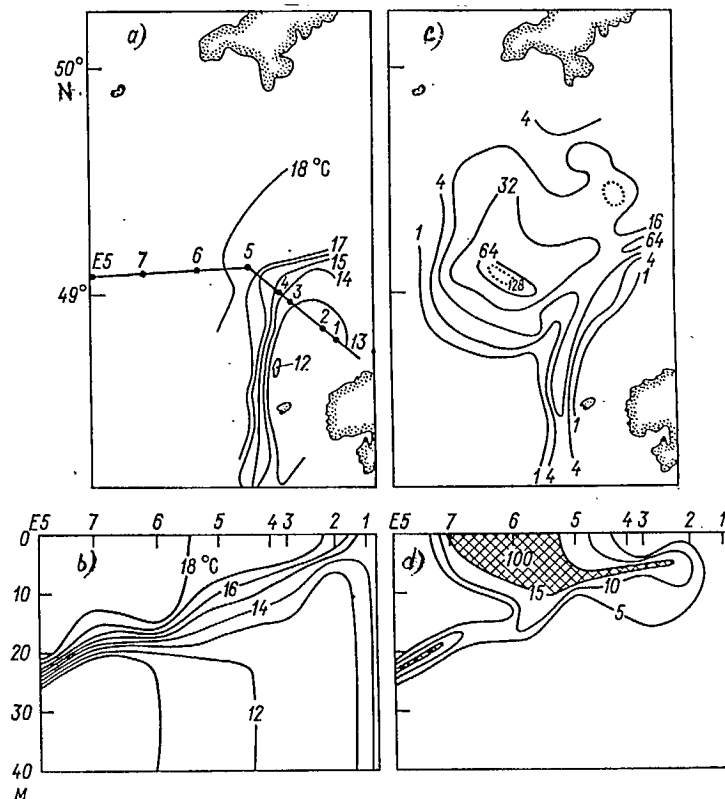
Fig. 3.39. Distribution of temperature at the surface of the ocean (a) and in a section (b), and the distribution of chlorophyll-a (c and d) (mg/m 3 ) in the shelf frontal zone west of Ushant at the entrance to the English Channel in August 1976, based on Simpson and Pingree's data [229]
