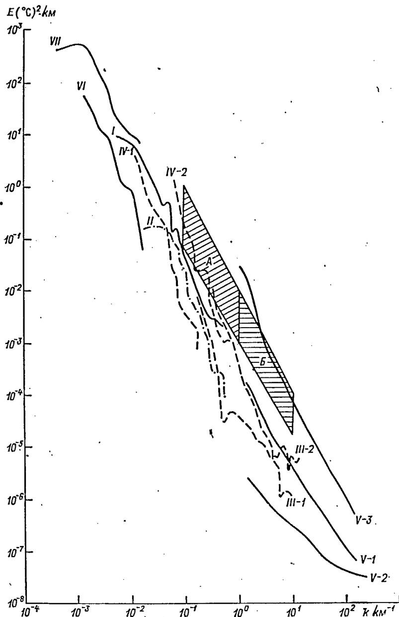
Fig. 2.12. Combined spectrum of horizontal temperature variability in the upper quasi-homogeneous layer of the ocean
