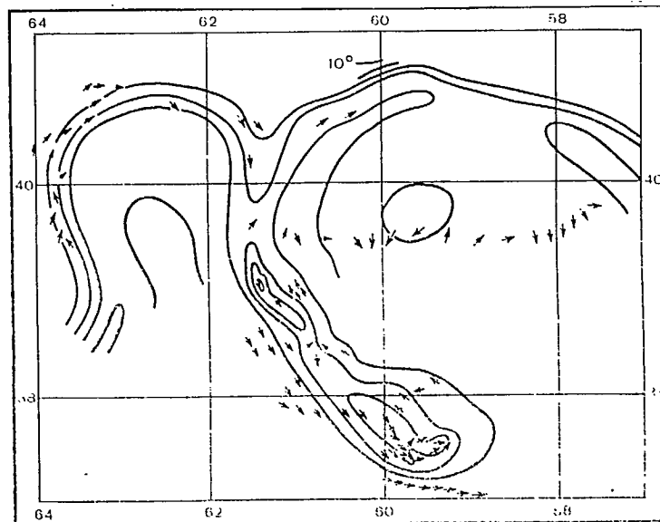
Fig. 3.1. The large cyclonic meander "Edgar" at the main front of the Gulf Stream in the temperature field of the surface layer of the ocean, based on data from ref. [122]. The meander is in the process of separation and transformation into a cyclonic ("cold") ring. The isotherms run through 5.5^{\circ}\text{C} . The arrows show the directions of the currents, based on measurements taken with a geomagnetic electrokinetograph from a moving vessel
