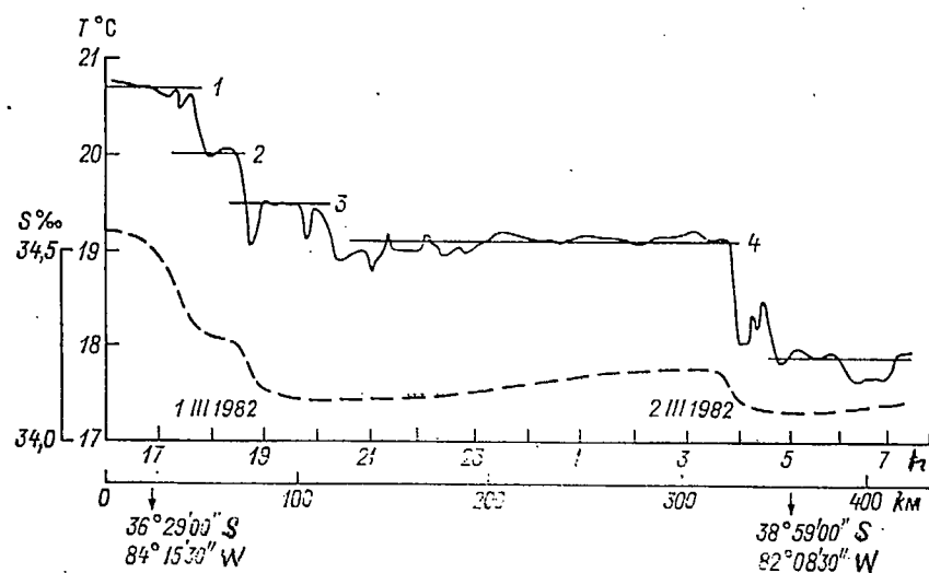
Fig. 4.4. Temperature and salinity distribution in an area of the southern subtropical convergence
