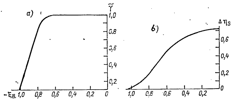
Fig. 2.37. Changes in the dimensionless density (a) and dimensionless overrun of the free-surface level (b) across the frontal zone, based on Kao's model data [156].
