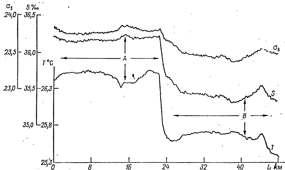
Fig. 2.10. An example of regions with a negative T, S-correlation (A and B) along both sides of a positive T, S-correlated front in the Sargasso Sea
