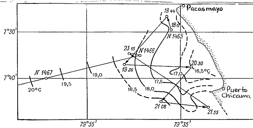
Fig. 3.29. Temperature distribution of the surface layer of the ocean near Puerto Chicama and Pacasmayo (Peru), based on the data of a survey carried out by the author from the "Akademik Kurchatov" research vessel on 28 Feb 1974. Thin solid lines show the tracks of the vessel. The stations used to plot fig. 3.30 a are marked
