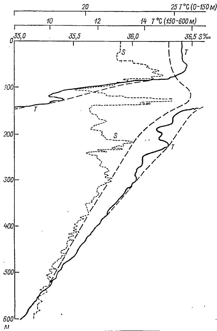
Fig. 3.22. Vertical profiles of temperature (T - solid line) and salinity (S - dotted line) at the edge of the cold core of a cyclonic ring (St. 2770, position shown in fig. 3.21)
