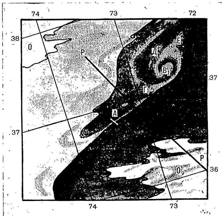
Fig. 4.13. Schematized fragment of an IR image of a radiated section of the Gulf Stream frontal zone for 20 March 1978
