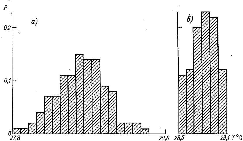
Fig. 3.44. Examples of histograms (with a 0.1^{\circ}\text{C} step of discreteness) which correspond to the recorded temperature inhomogeneities
