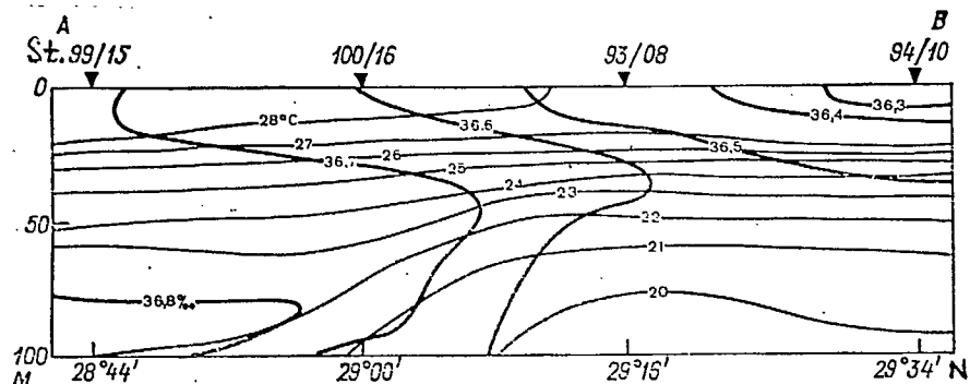
Fig. 2.15. Temperature and salinity at a section along 69^{\circ}40' W long in the Sargasso Sea
