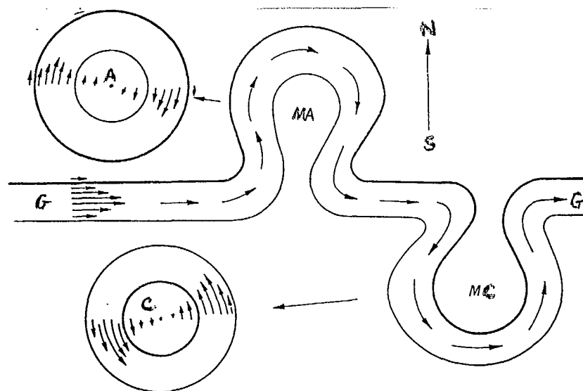
Fig. 3.10. Diagram of the separation of anticyclonic (A) and cyclonic (C) rings from the Gulf Stream (G) as a result of the formation of anticyclonic (MA) and cyclonic (MC) meanders
