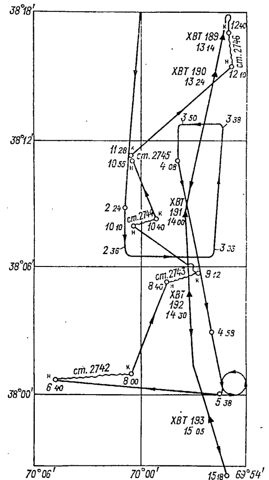
Fig. 3.14. Diagram of maneuvering of the "Akademik Kurchatov" research vessel in the frontal zone on the southern periphery of the warm ring of the Gulf Stream on 11 September 1978 (ship time)
