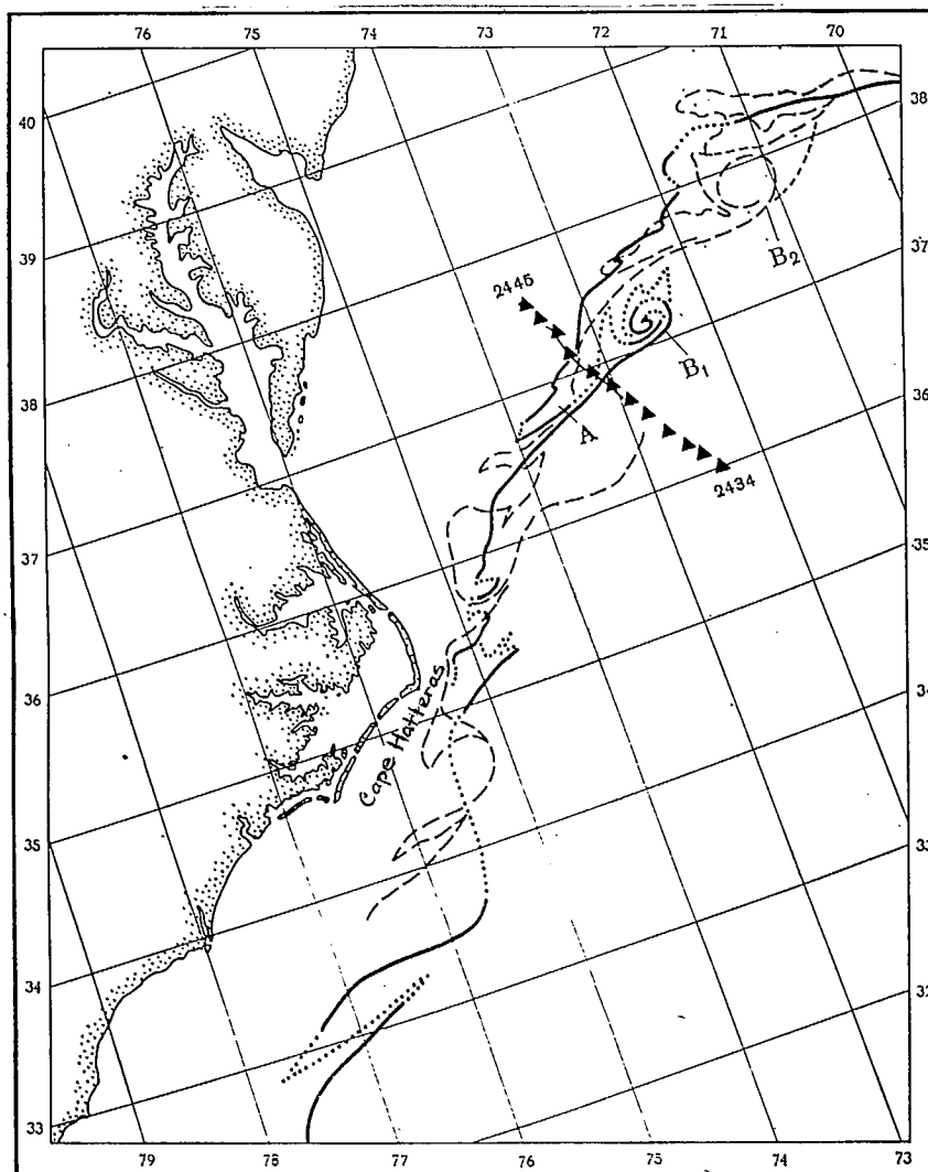
Fig. 4.16. Diagram of the positions of the northern Gulf Stream boundary, based on the data of IR images for 20 and 23 March 1978
