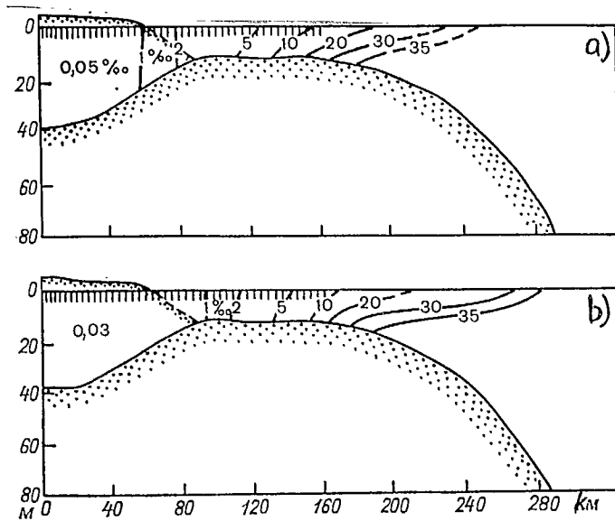
Fig. 3.31. Vertical section in the salinity field across the drainage lens of the Amazon R., based on [134], during the minimum discharge (a) and during high water (b)
