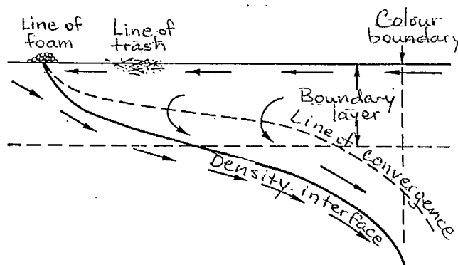
Fig. 3.35. Relative distribution of foam and trash accumulations, and of the colour boundary near an estuarine front, after Klemas [162]
