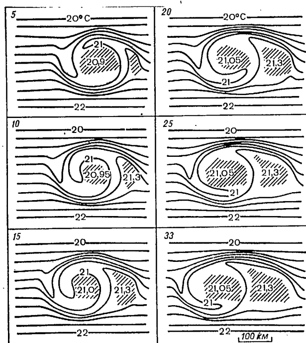
Fig. 3.4. Temperature maps of ocean surface in the case of a cyclonic eddy moving westward with a speed of 5 km/day. Figures in upper left-hand corner - day of integration. Diagram borrowed from [47]
