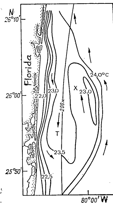
Fig. 3.8. Spin-off eddy at the boundary of the Gulf Stream off the Florida coast in the surface temperature field, based on the data of [171].
