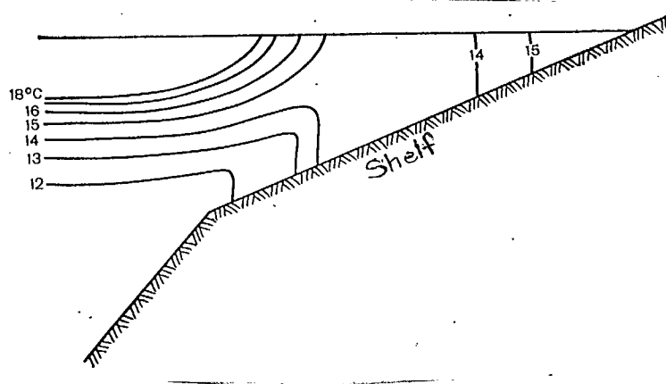
Fig. 3.38. Diagram of the position of isotherms in a summer shelf frontal interface that forms during mixing in shallow waters
