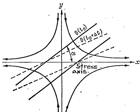
Fig. 2.21. Diagram of a hyperbolic deformation field and changes in the position of the isolines of potential temperature \theta in this field for the time interval \Delta t .
