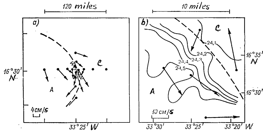
Fig. 3.2. a - daily average current vectors at the 1000-metre level at a polygon in the Tropical Atlantic on 3 July 1970, based on the data of instrumental measurements. The dashed line marks the rear boundary of the anticyclonic eddy (A) passing across the polygon from east to west. The zigzag line shows the position of the frontal interface in the upper layer of the ocean (for greater detail see fig. 3.1 b). The scale of the vectors is indicated in the lower left-hand corner of the diagram; b - isotherms in the region of the front at the isopycnic surface \sigma_t = 25.00 (50-60 m) on 3 July 1970. Arrows indicate the daily average current vectors at the 25 m horizon at the buoy stations closest to the front. The cyclonic vorticity of the near-frontal currents are clearly visible.
