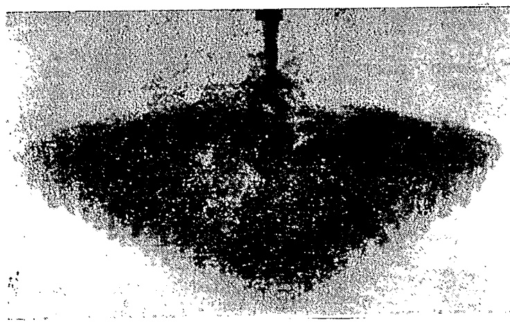
Fig. 4.11. Photograph showing the sinking of salt fingers from an axisymmetric thermohaline intrusion in the initial phase of spreading ( t \approx 450 \text{ s} ) in the second experiment
