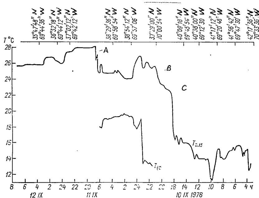
Fig. 3.17. Temperature changes near the surface ( T_{0.15} ) and at a depth of 80 m ( T_{80} ), recorded on 10-12 September 1978 en route from Boston to the POLYMODE area along 70^{\circ} W
