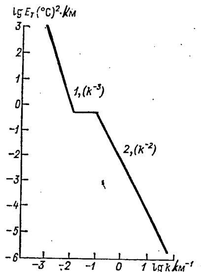
Fig. 2.13. Conjectural combined spectrum of horizontal temperature variability with an abrupt transition from synoptic ( eddy ) scales (1) to frontal ones (2)
