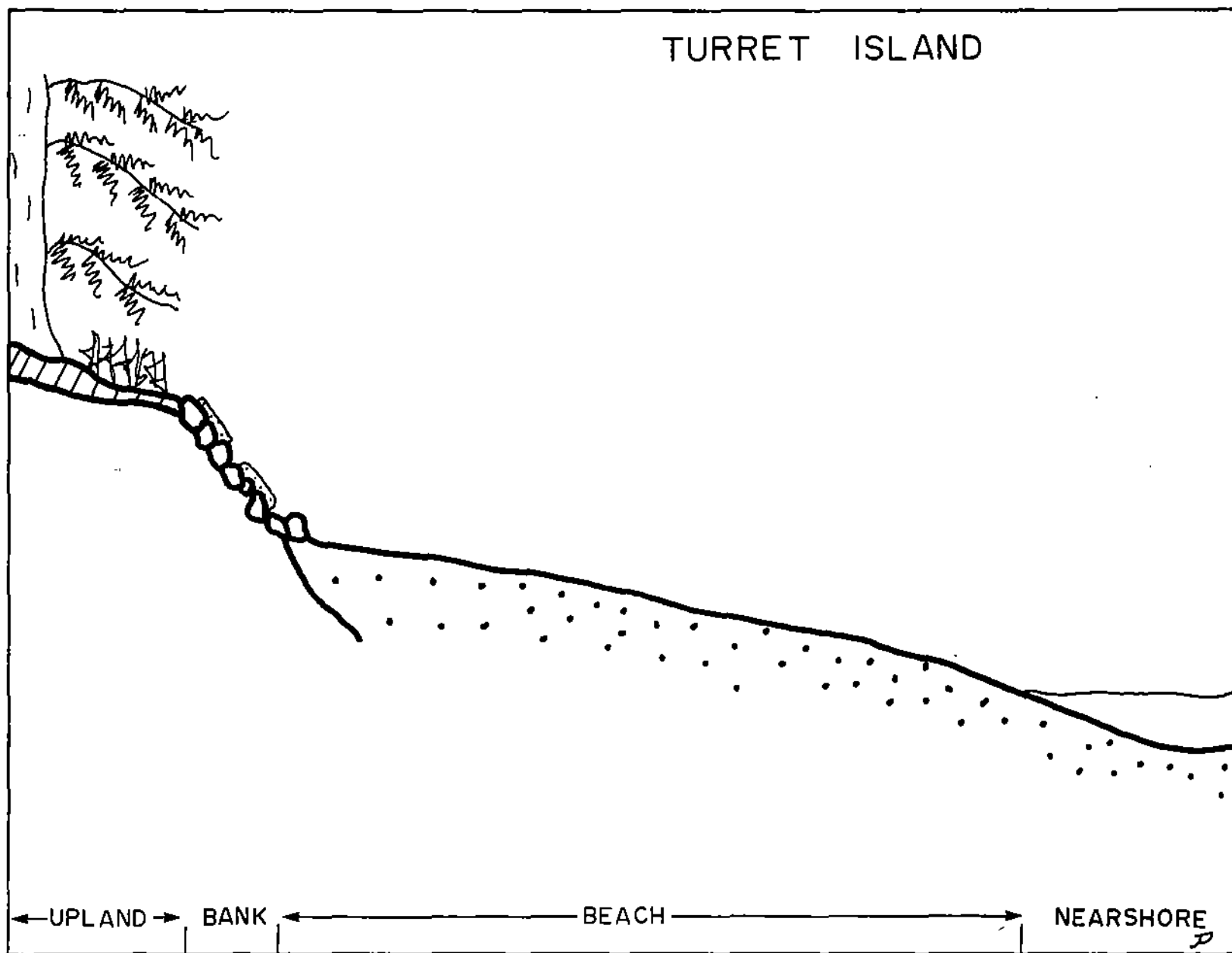
Fig. 49. Schematic profile of Turret Island system concept
