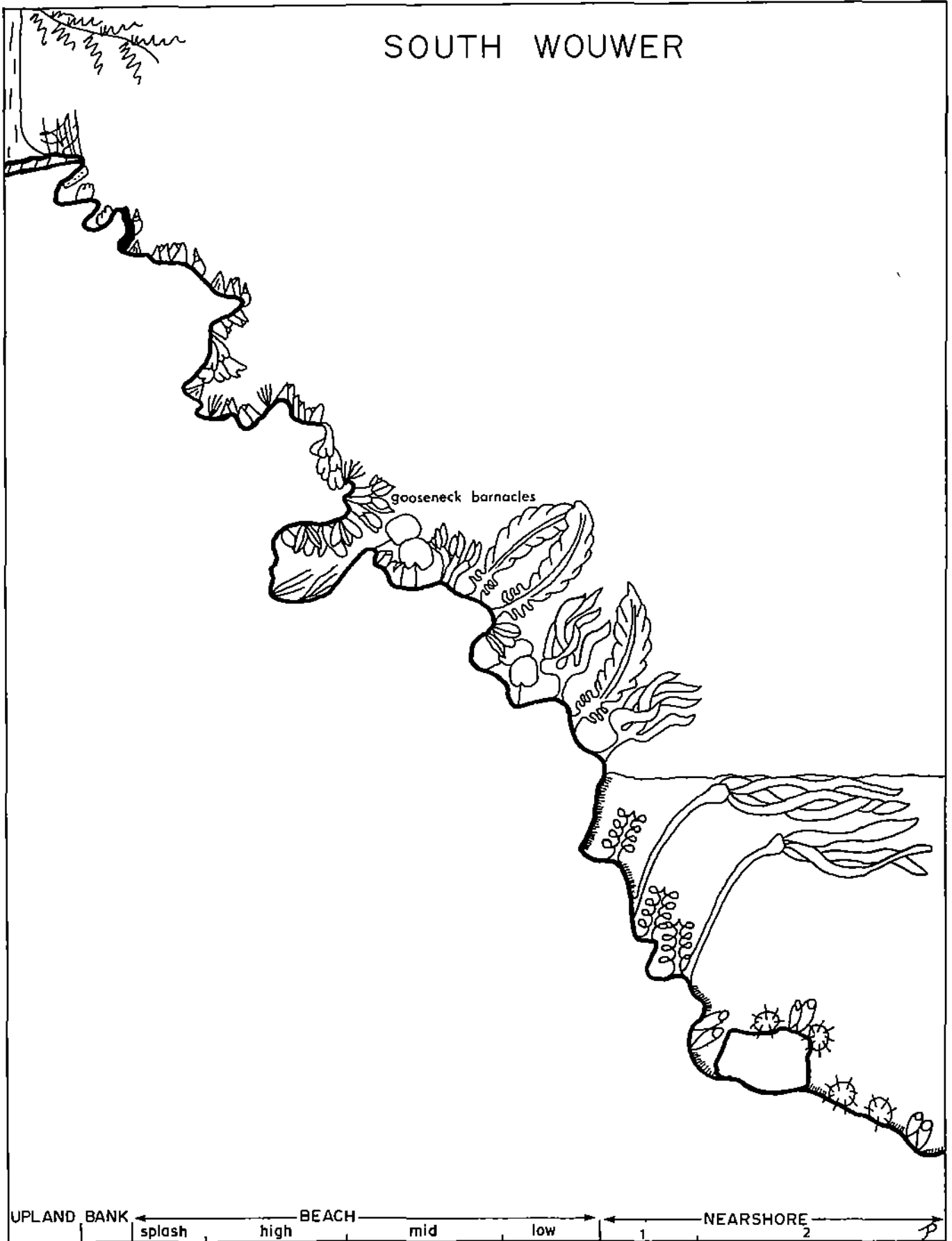
Fig. 67. Schematic profile of South Wouwer system concept.
