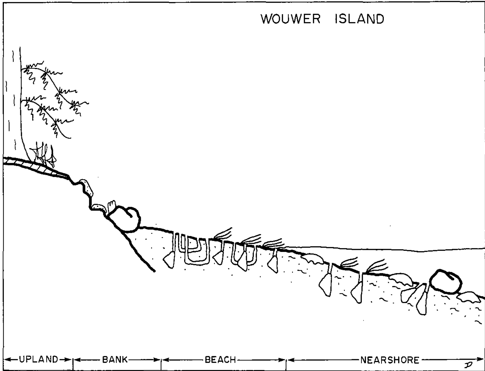
Fig. 35. Schematic profile of Wouwer Island system concept
