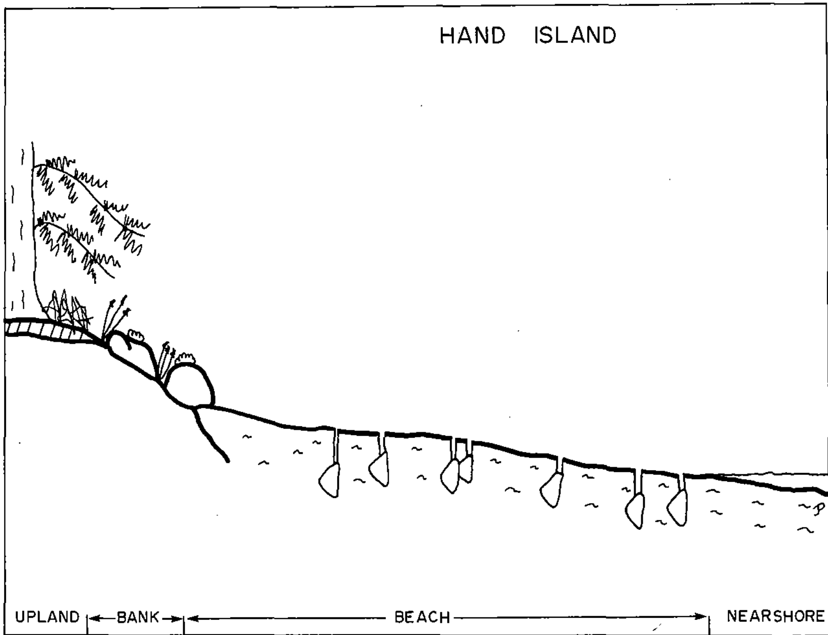
Fig. 51. Schematic profile of Hand Island system concept
