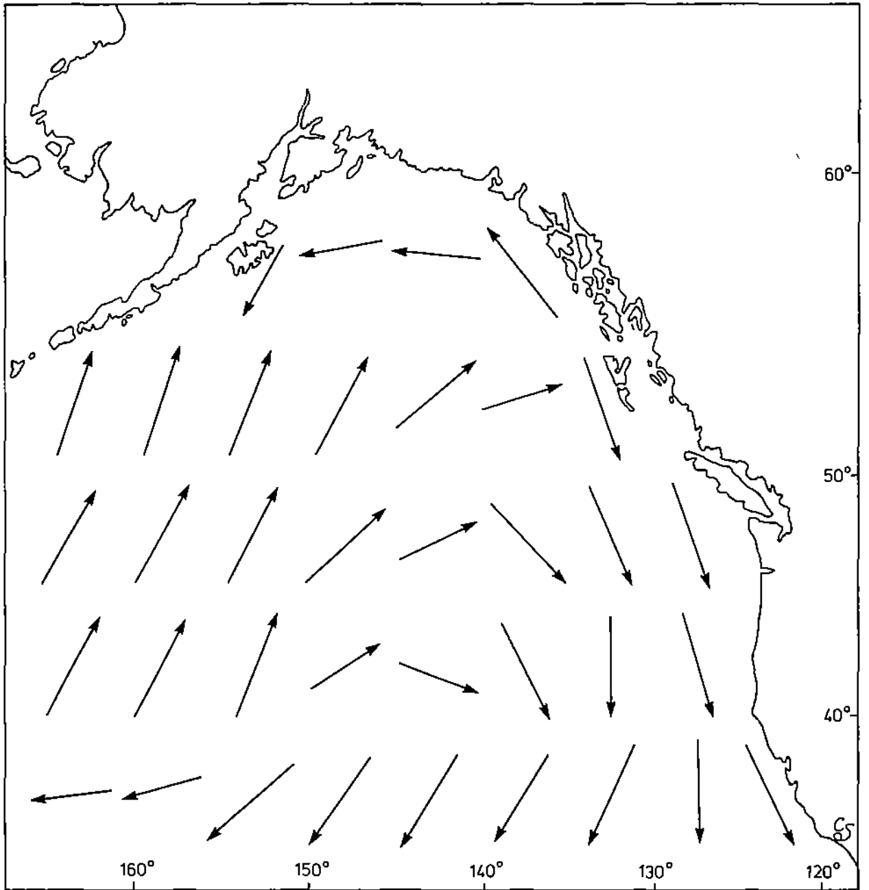
Fig. 21. Prevailing summer surface winds in the eastern subarctic Pacific Ocean (revised from Dodimead, Favourite and Hirano 1963)
