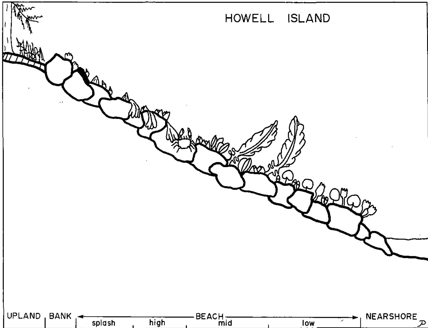
Fig. 66. Schematic profile of Howell Island system concept
