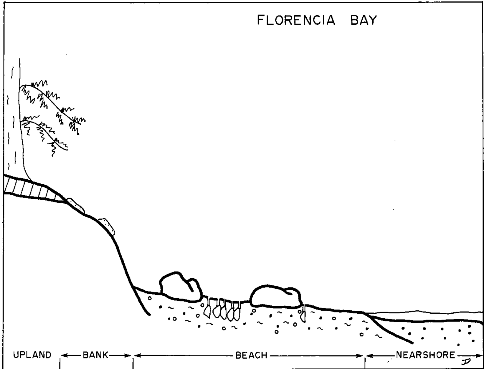
Fig. 53. Schematic profile of Florencia Bay system concept
