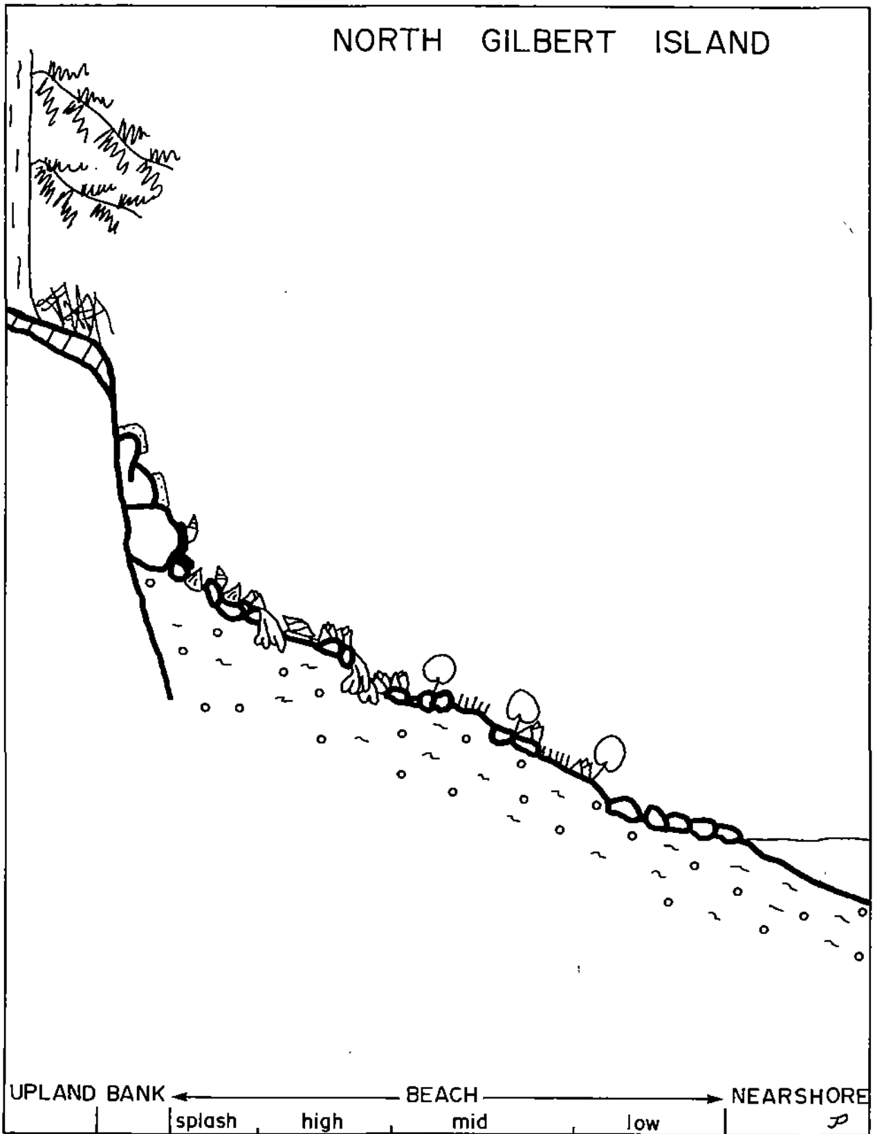
Fig. 55. Schematic profile of North Gilbert Island system concept
