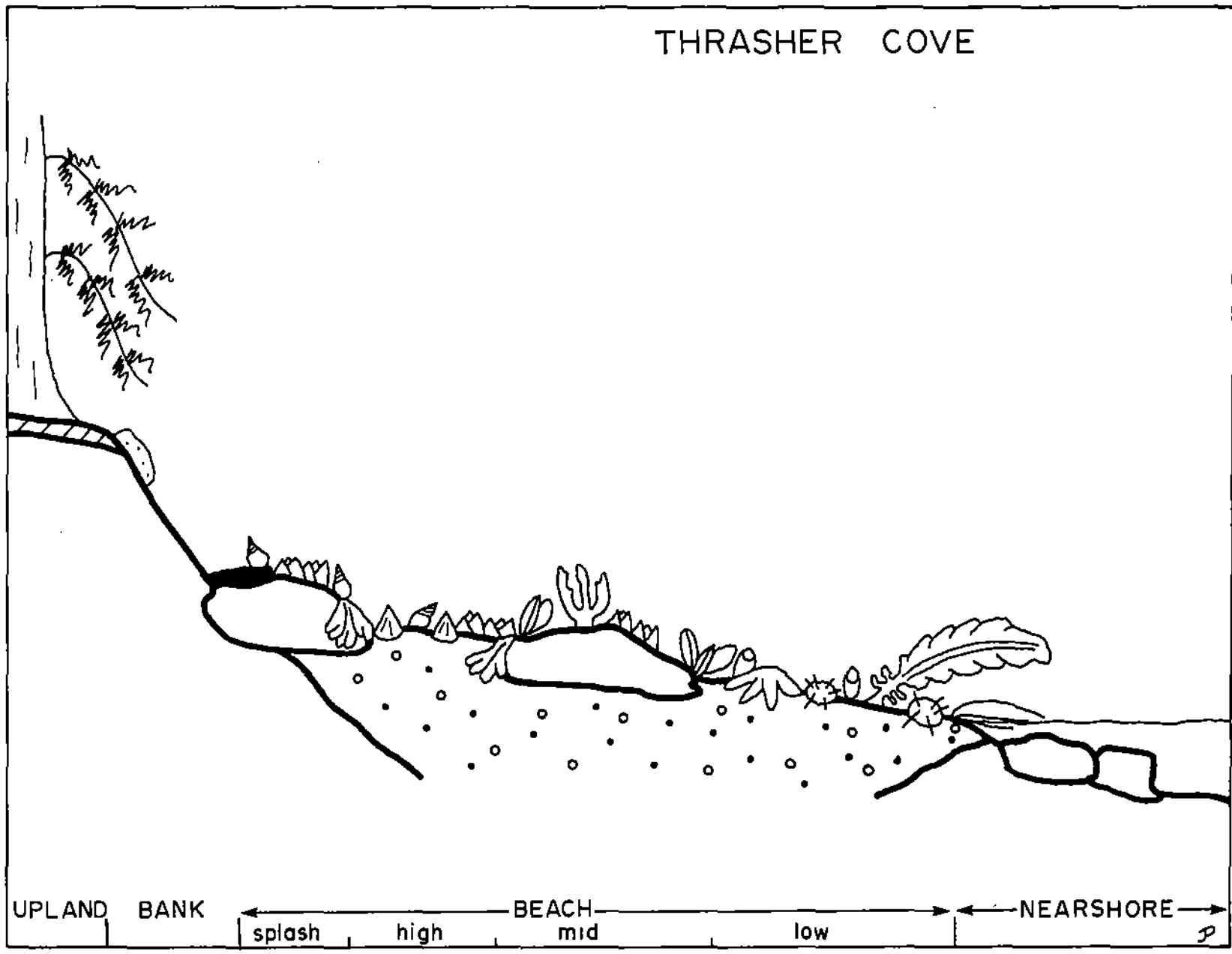
Fig. 58. Schematic profile of Thrasher Cove system concept
