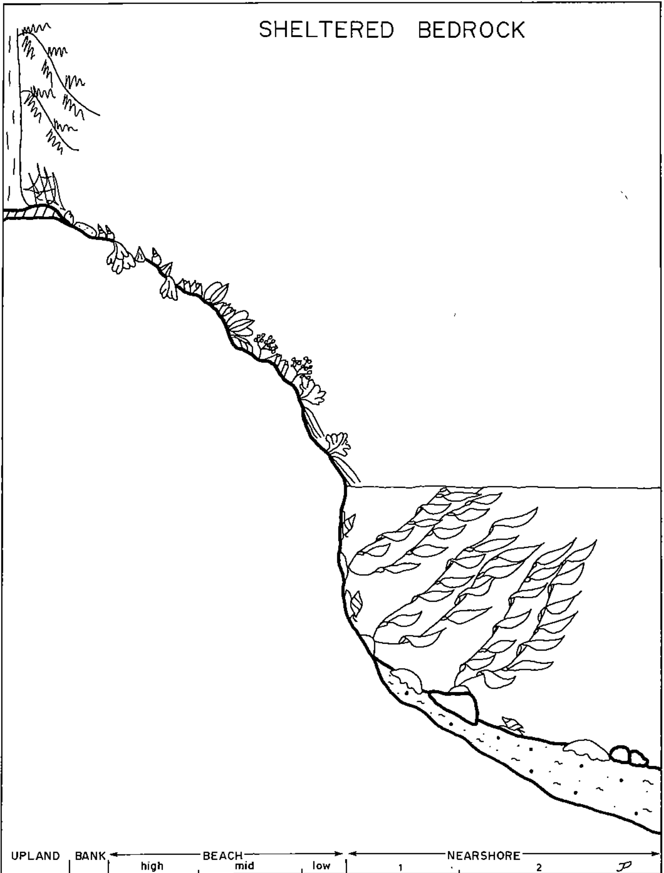
Fig. 46. Schematic profile of Sheltered Bedrock system concept.
