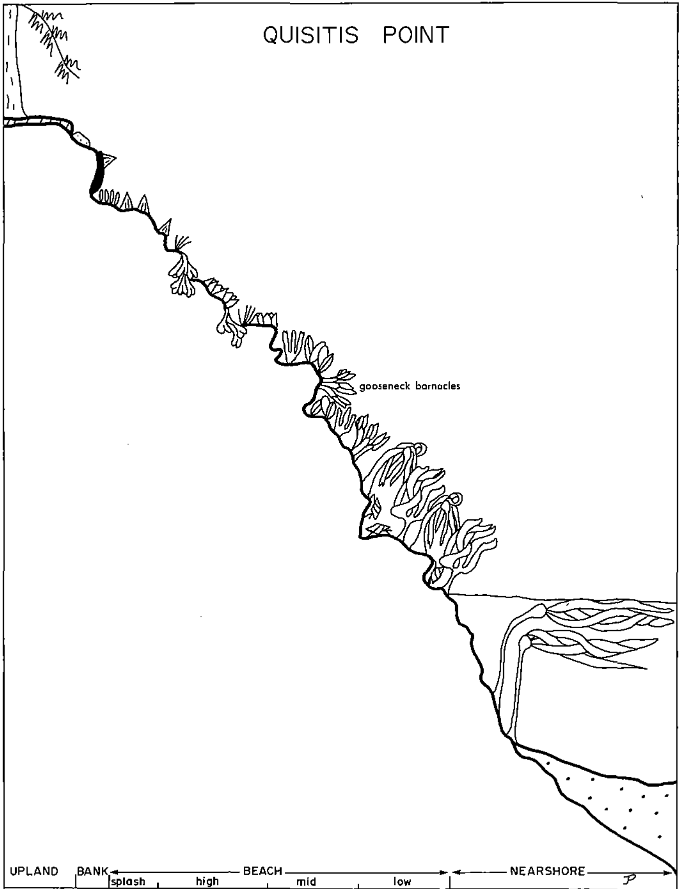
Fig. 68. Schematic profile of Quisitis Point system concept.
