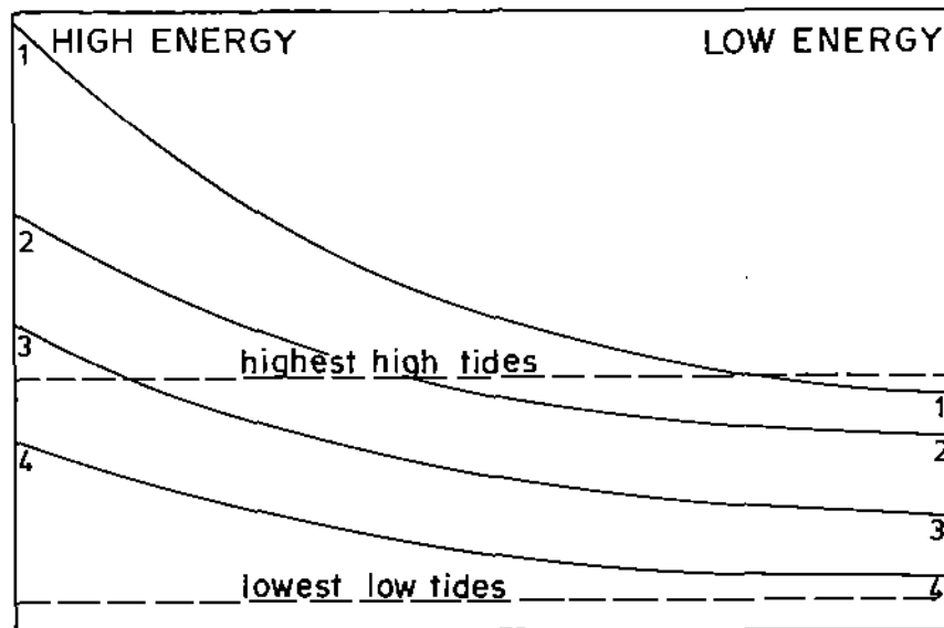
Fig. 28. Schematic diagram of upward displacement of biotic zones as one proceeds toward the higher energy part of the coast (1 = splash zone, 2 = high intertidal zone, 3 = mid intertidal zone, 4 = low intertidal zone) (revised from Ricketts and Calvin 1968)
