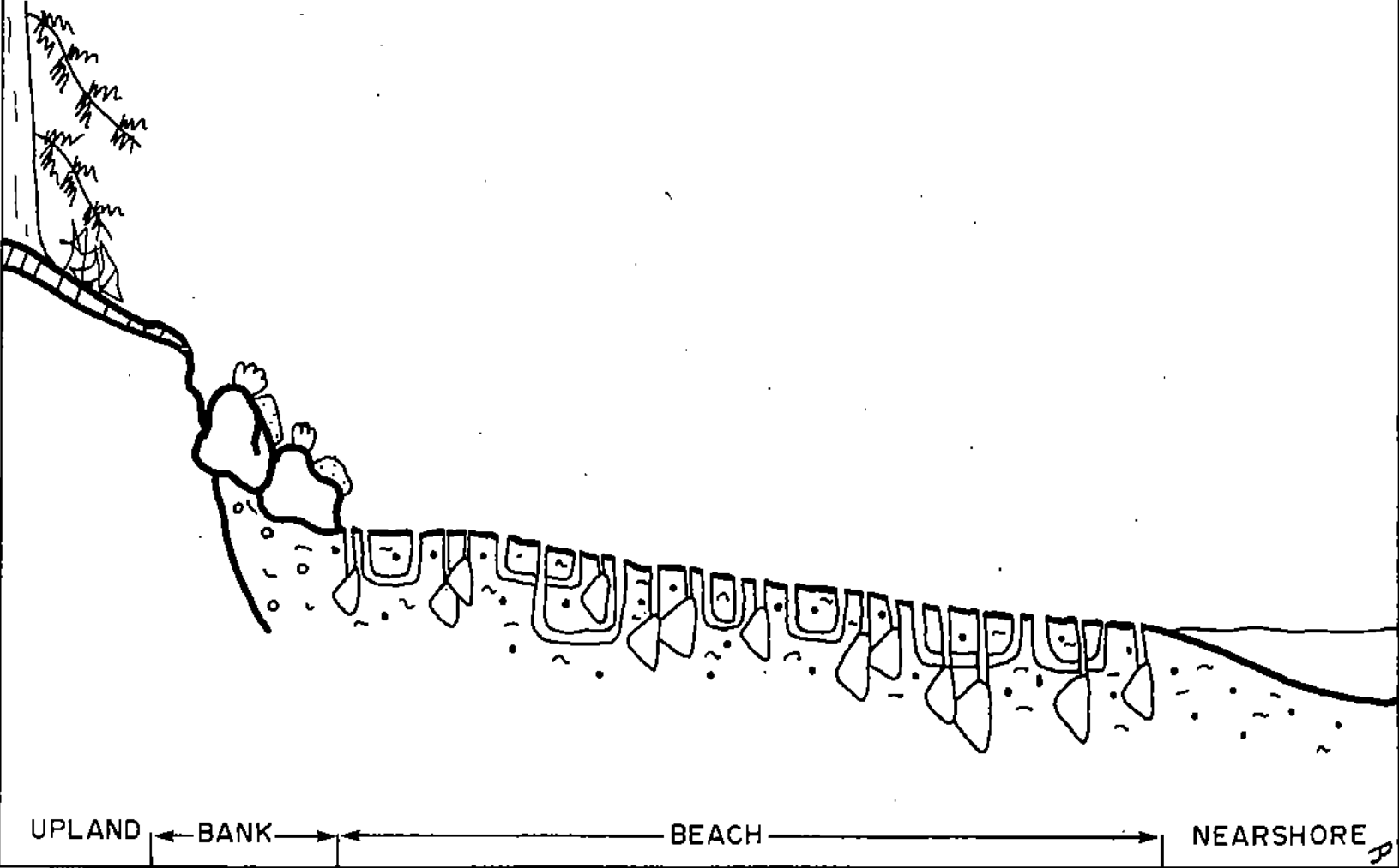
Fig. 38. Schematic profile of South Gibraltar Island system concept
