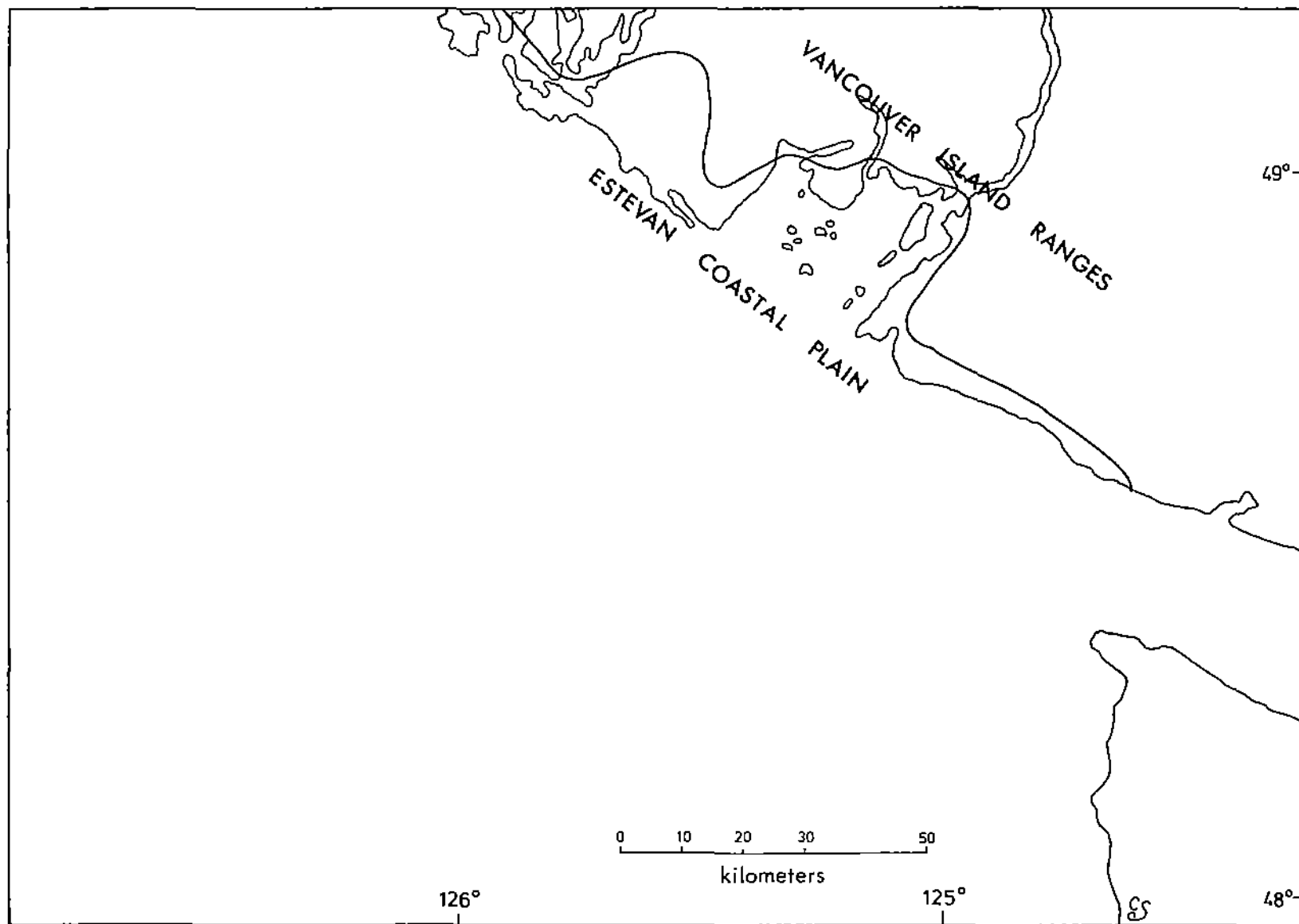
Fig. 4. Physiographic divisions of southwestern Vancouver Island (Holland 1976)
