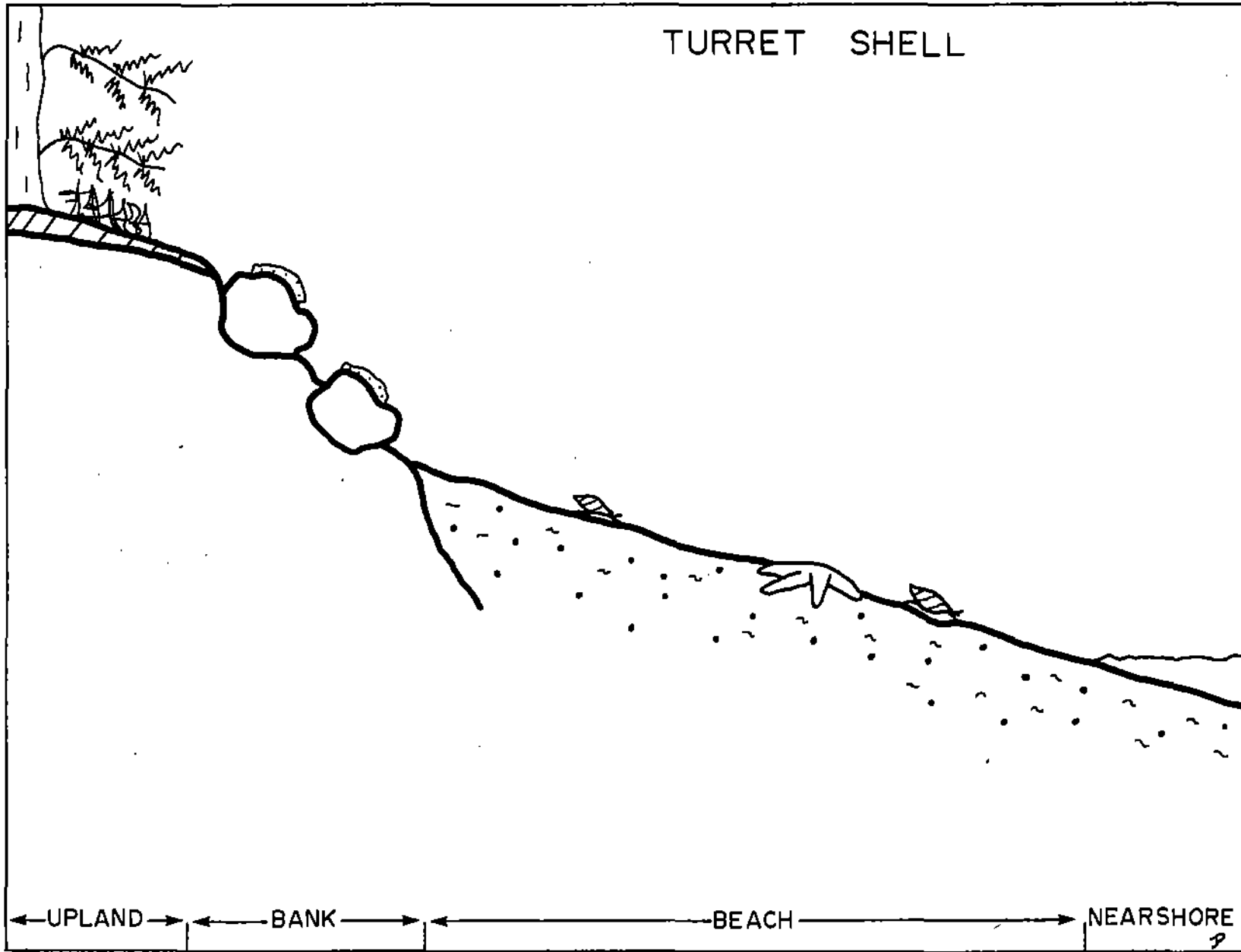
Fig. 50. Schematic profile of Turret Shell system concept
