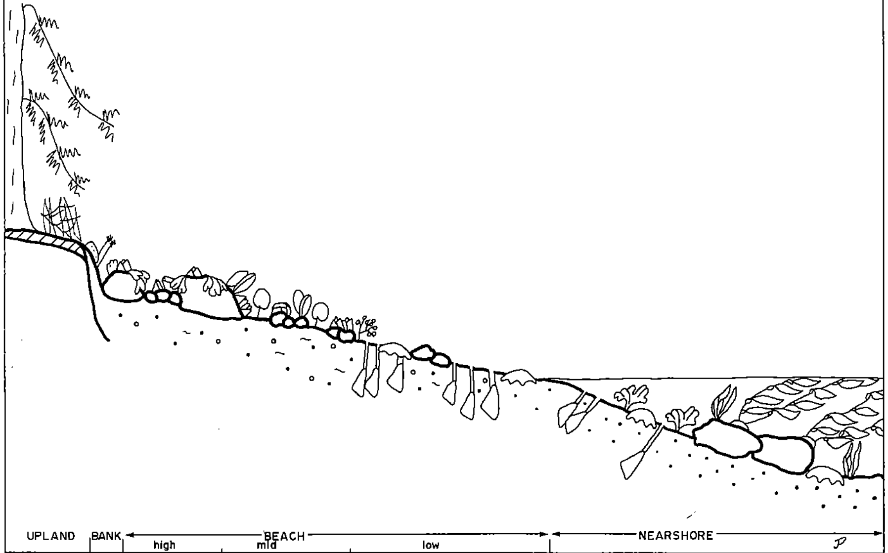
Fig. 43. Schematic profile of Gilbert Island system concept.
