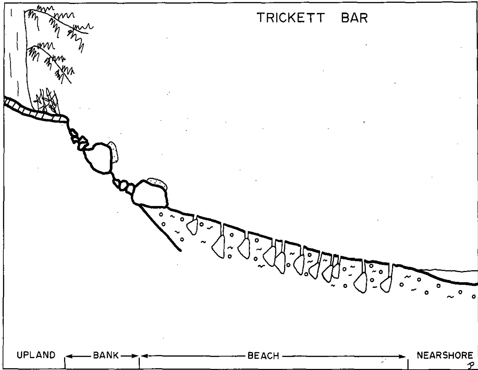
Fig. 52. Schematic profile of Trickett Bar system concept
