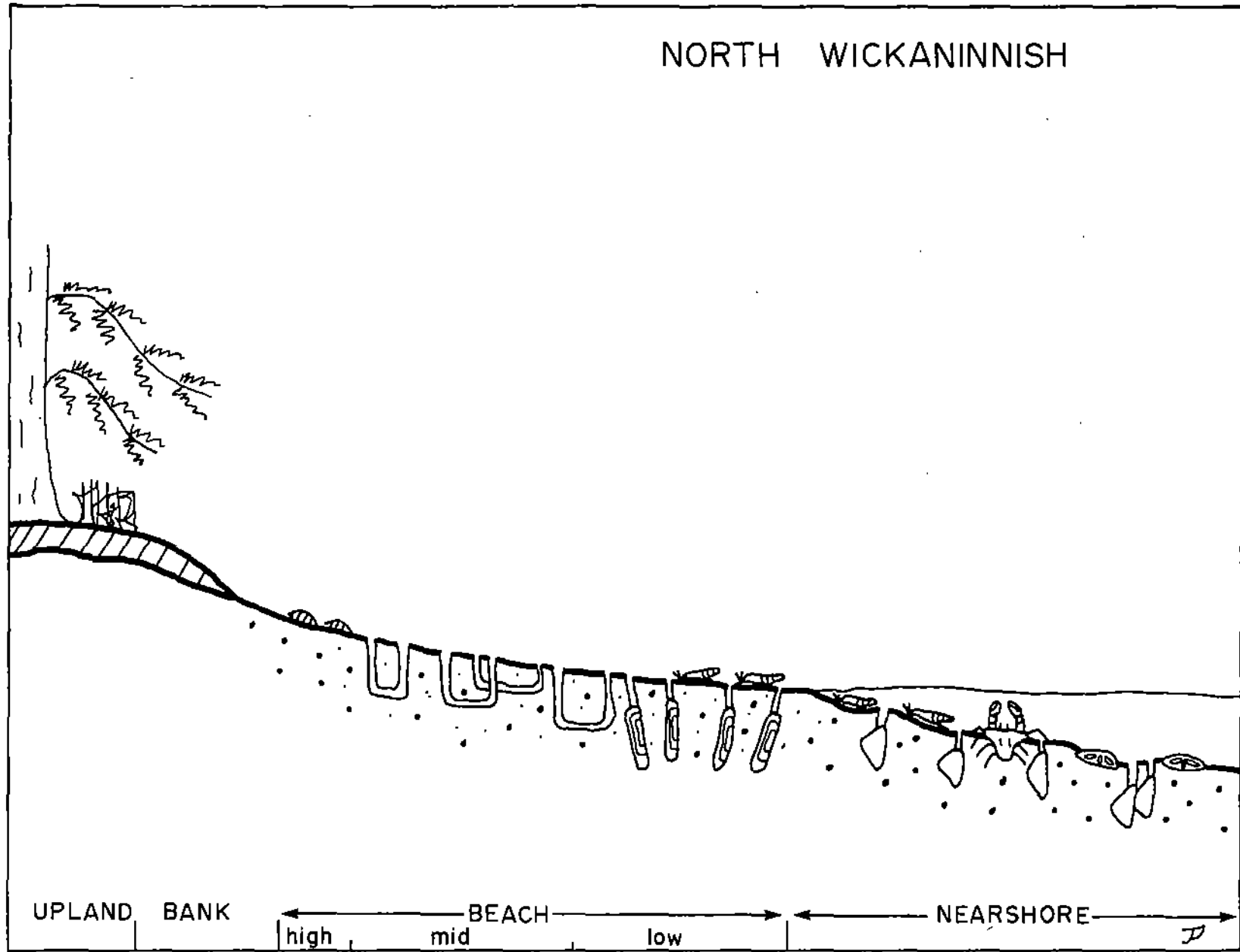
Fig. 47. Schematic profile of North Wickaninnish system concept
