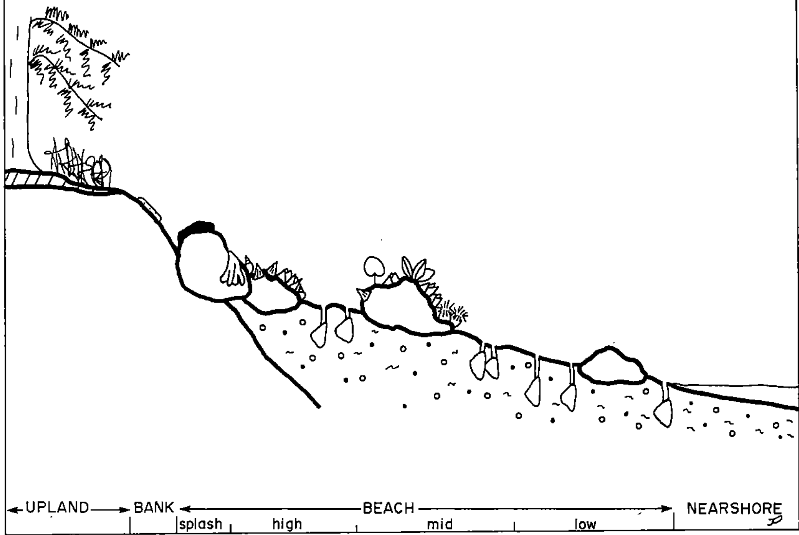
Fig. 57. Schematic profile of Cooper Island system concept
