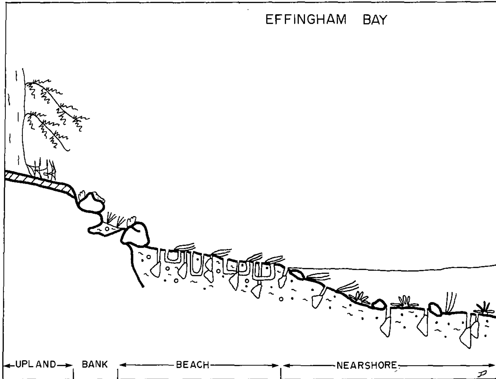
Fig. 41. Schematic profile of Effingham Bay system concept
