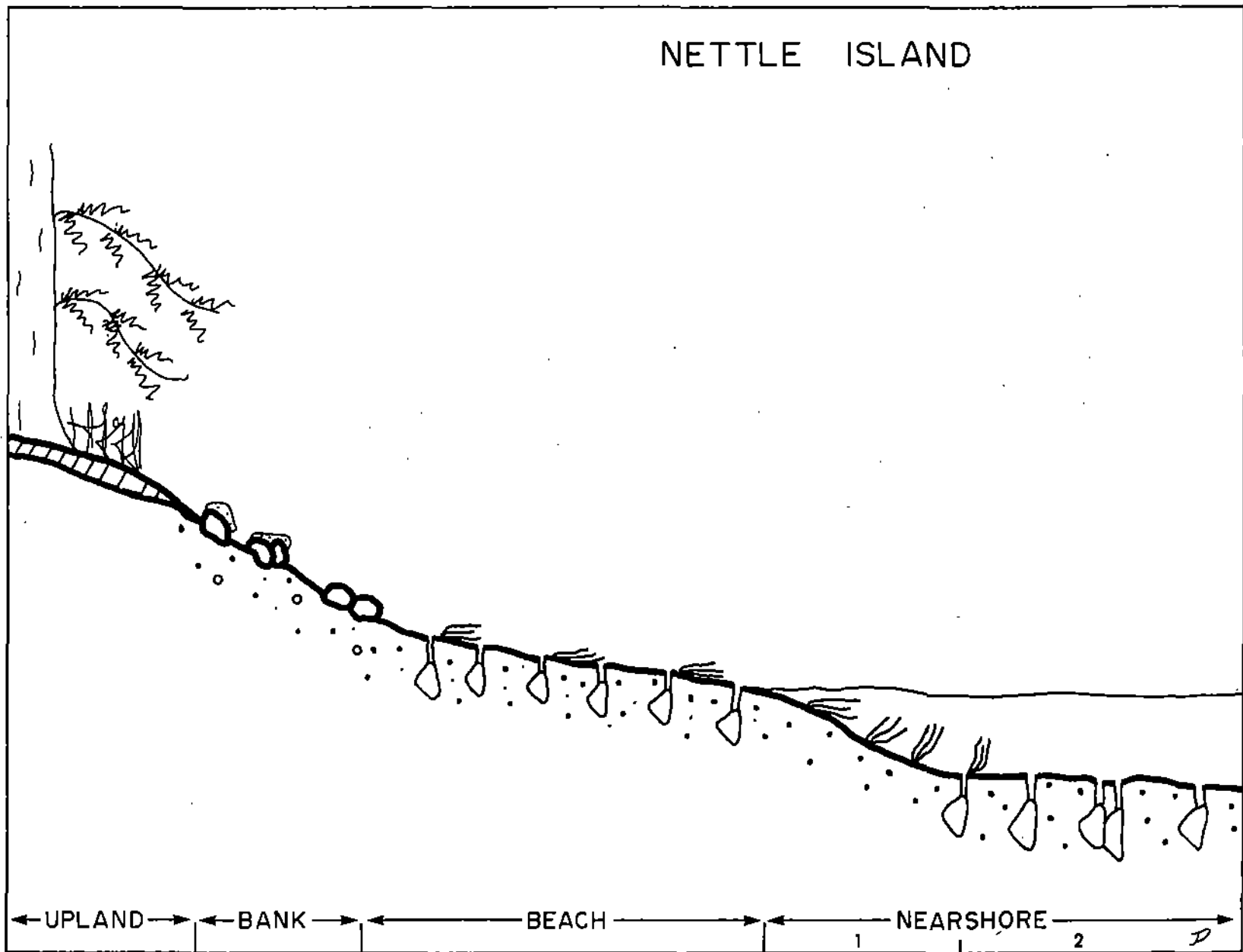
Fig. 37. Schematic profile of Nettle Island system concept
