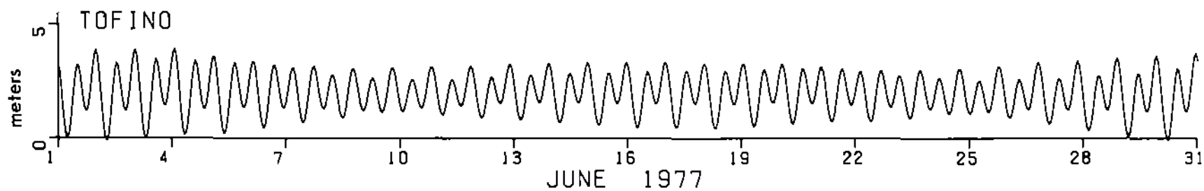
Fig. 25. Mixed, mainly semi-diurnal tidal curve, Tofino (June 1977) (Hydrographic Chart Distribution Office)
