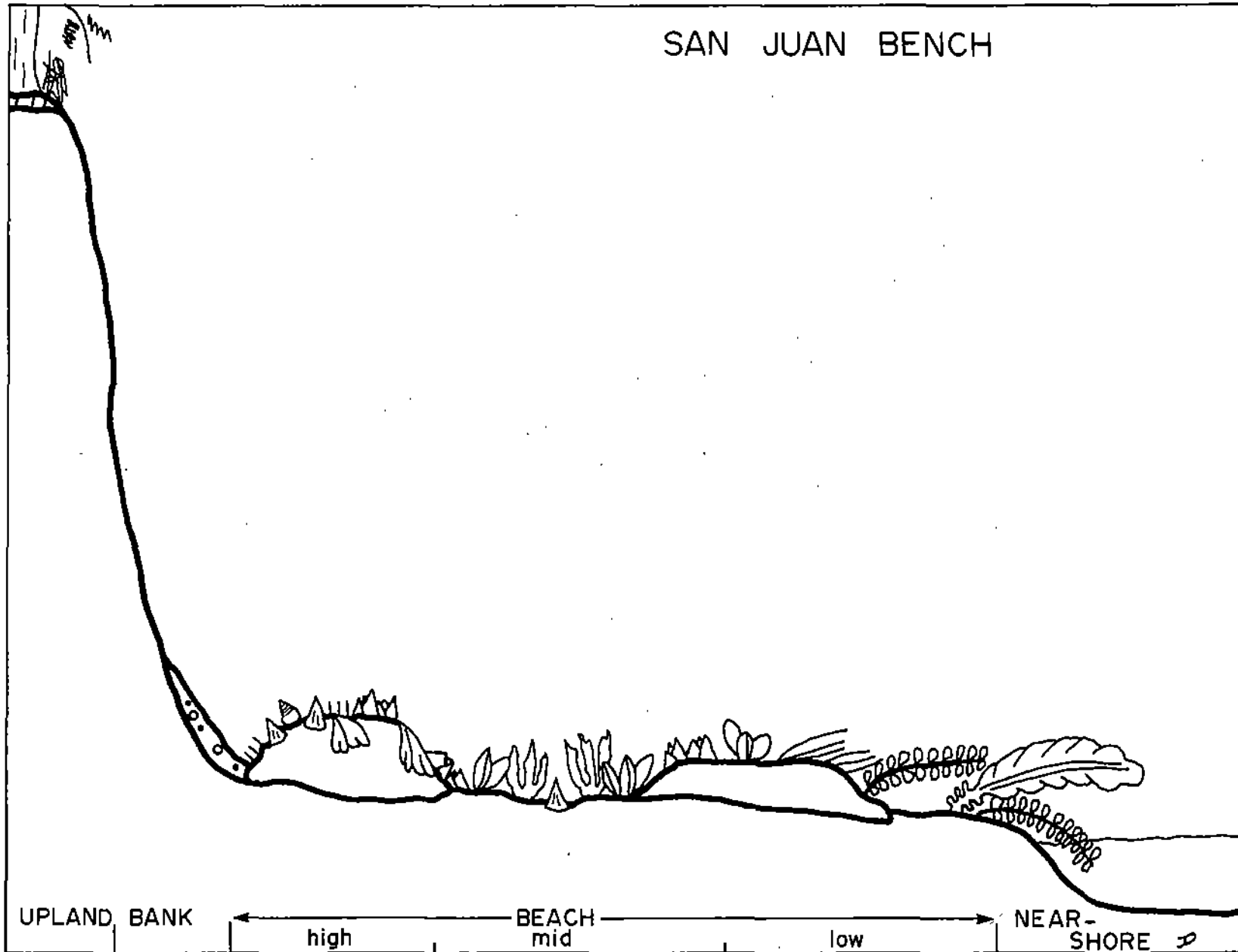
Fig. 62. Schematic profile of San Juan Bench system concept
