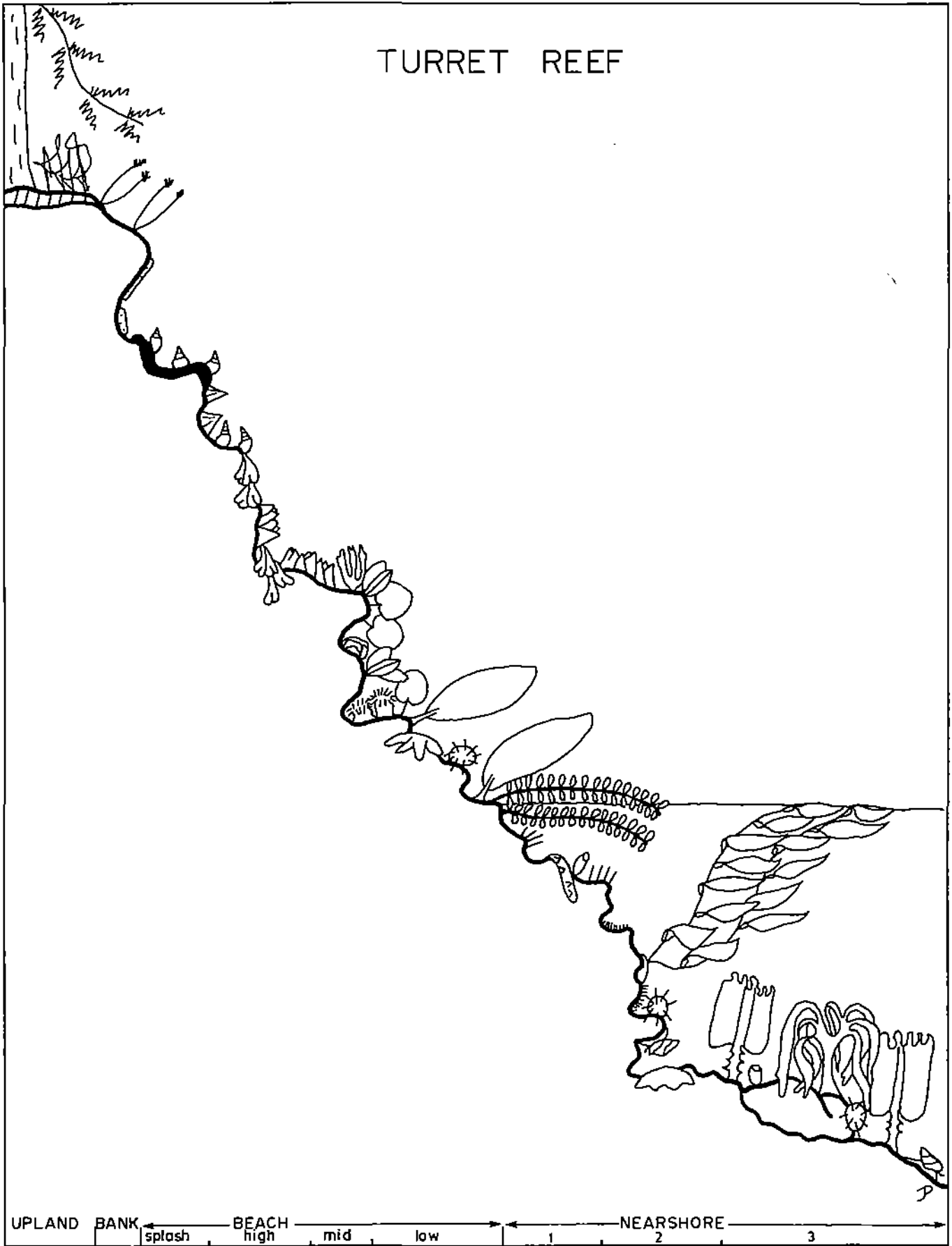
Fig. 61. Schematic profile of Turret Reef system.
