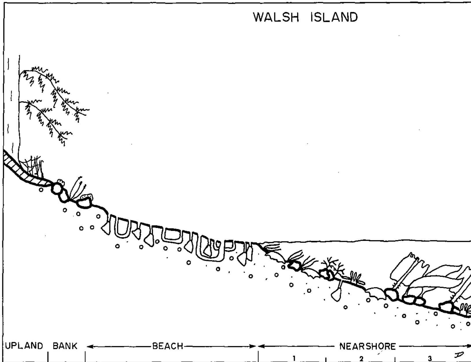
Fig. 40. Schematic profile of Walsh Island system concept
