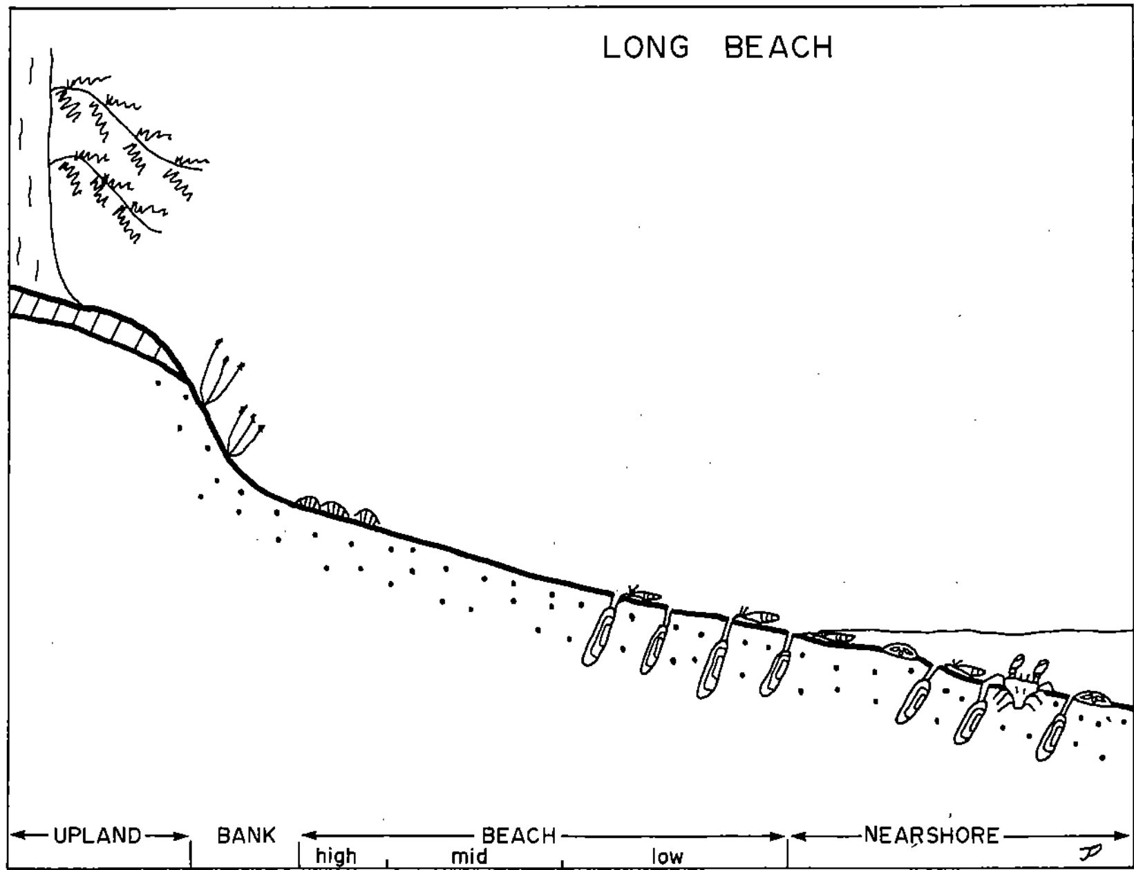
Fig. 63. Schematic profile of Long Beach system concept
