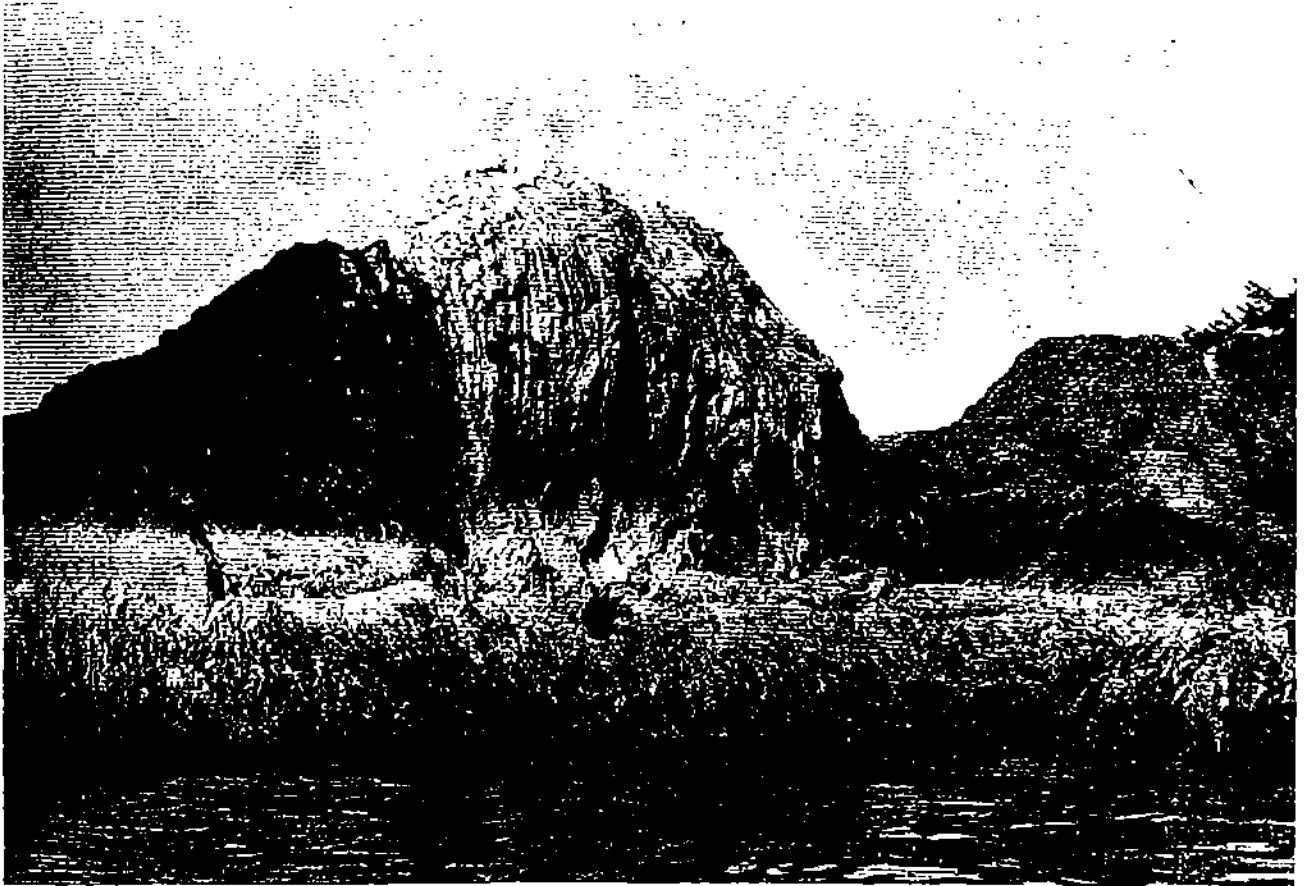
Fig. 10. Harder layers of rock standing out in relief, Broken Group Islands
