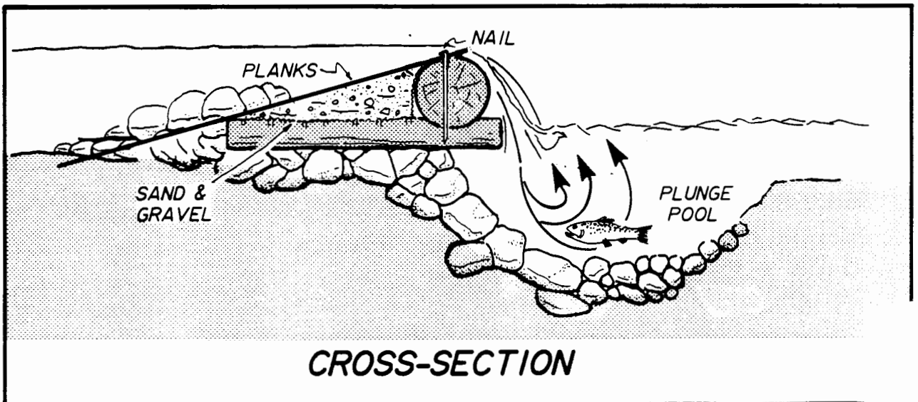
FIGURE E-4: SINGLE LOG DAM WITH PLANK FLOOR.
