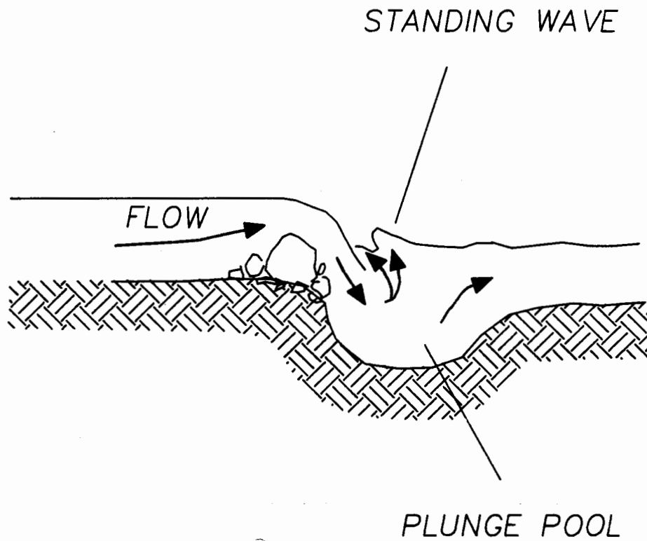
FIGURE E-2: CROSS-SECTION OF A LOW HEAD BARRIER SHOWING THE PLUNGE POOL AND STANDING WAVE.
