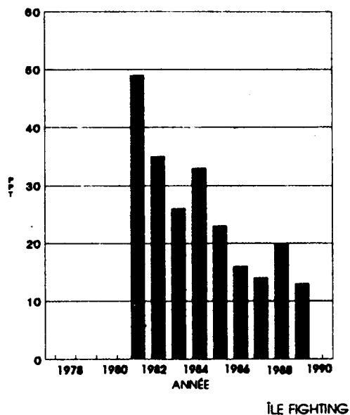
CONCENTRATIONS DE TCDD
