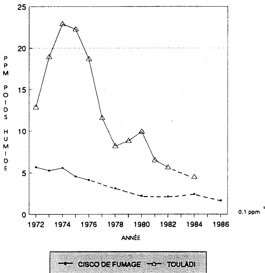
Figure 46
