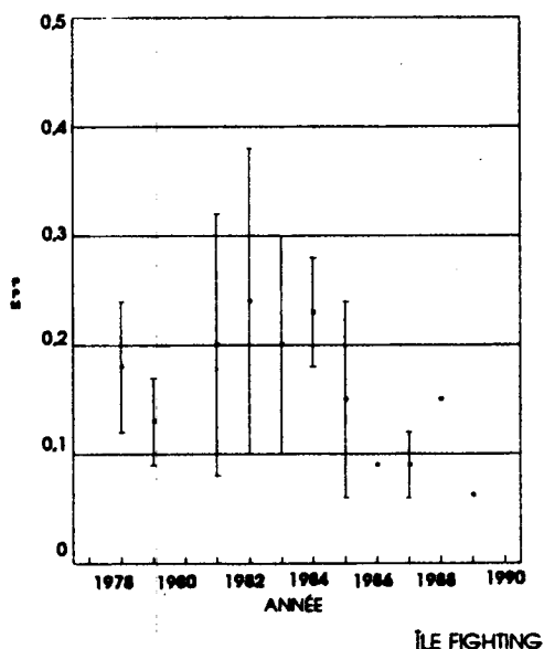
CONCENTRATIONS DE DIELDRINE
