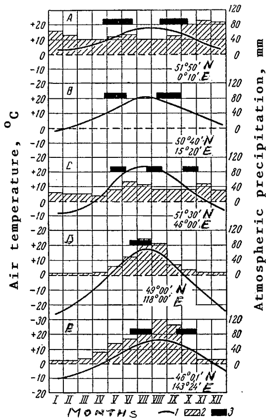
Fig. 3. Number of emergences per year by eurythermal species of the genus Chironomus from water bodies in the temperate zone of Eurasia (up to 2 m deep), located at about 50^{\circ} N lat
