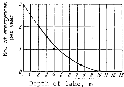
Fig. 4. Curve depicting the number of emergences of Chironomus plumosus a year from different depths in Lake Beloye near Kosino during 1935-1936
