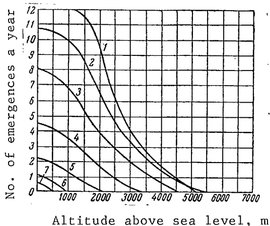
Fig. 5. Curves denoting the number of emergences of eurythermal Chironomus species from depths of up to 2 m in continental bodies of water located at different altitudes above sea level in various climatic zones of the northern hemisphere
