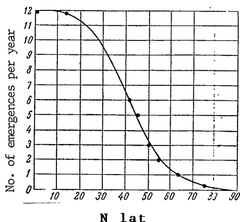
Fig. 2. Curve denoting the number of emergences per year by eurythermal species of the genus Chironomus in lowland continental water bodies from a depth of 2 m at different geographic latitudes between 30 and 50 E long
