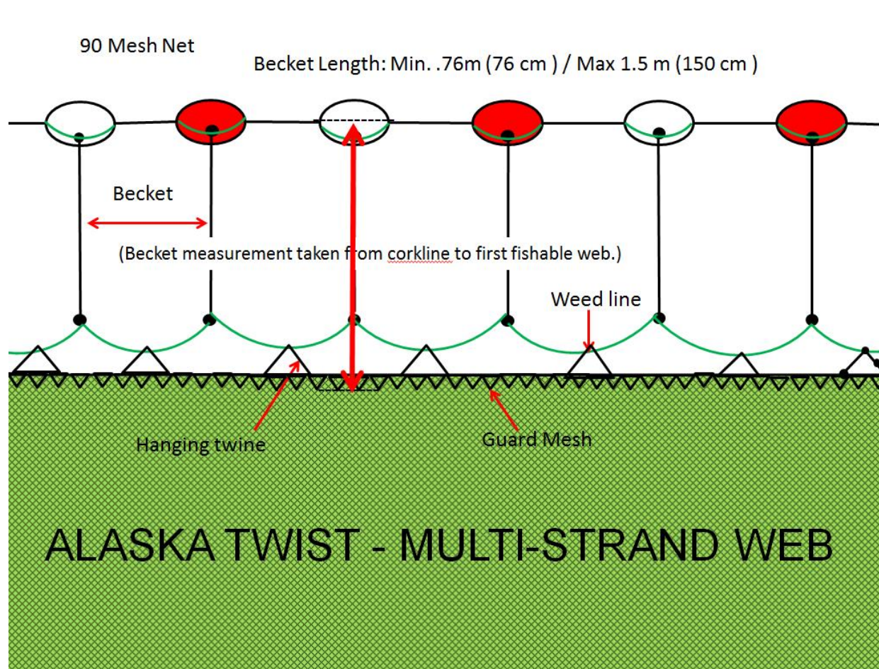
Figure 13.5-11: 90 Mesh Net Construction
