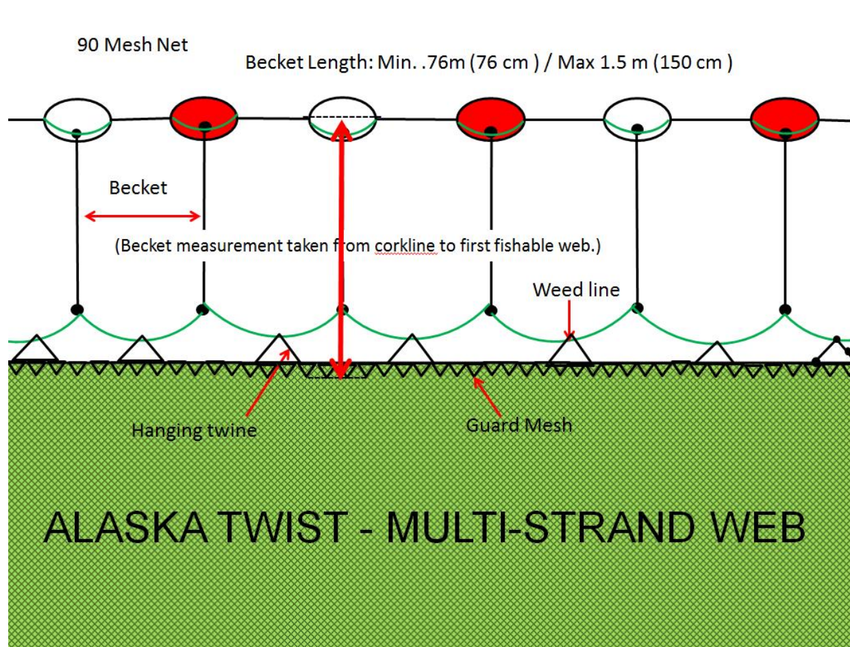
Figure 13.5-4: 90 Mesh Net Construction
