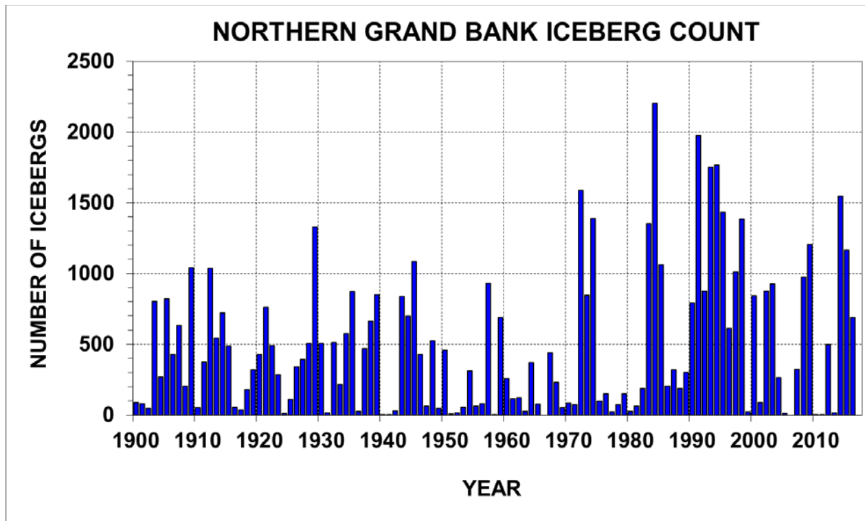
Figure 9. Annual iceberg count crossing south of 48°N on the northern Grand Bank (data courtesy of IIP of the USCG).
