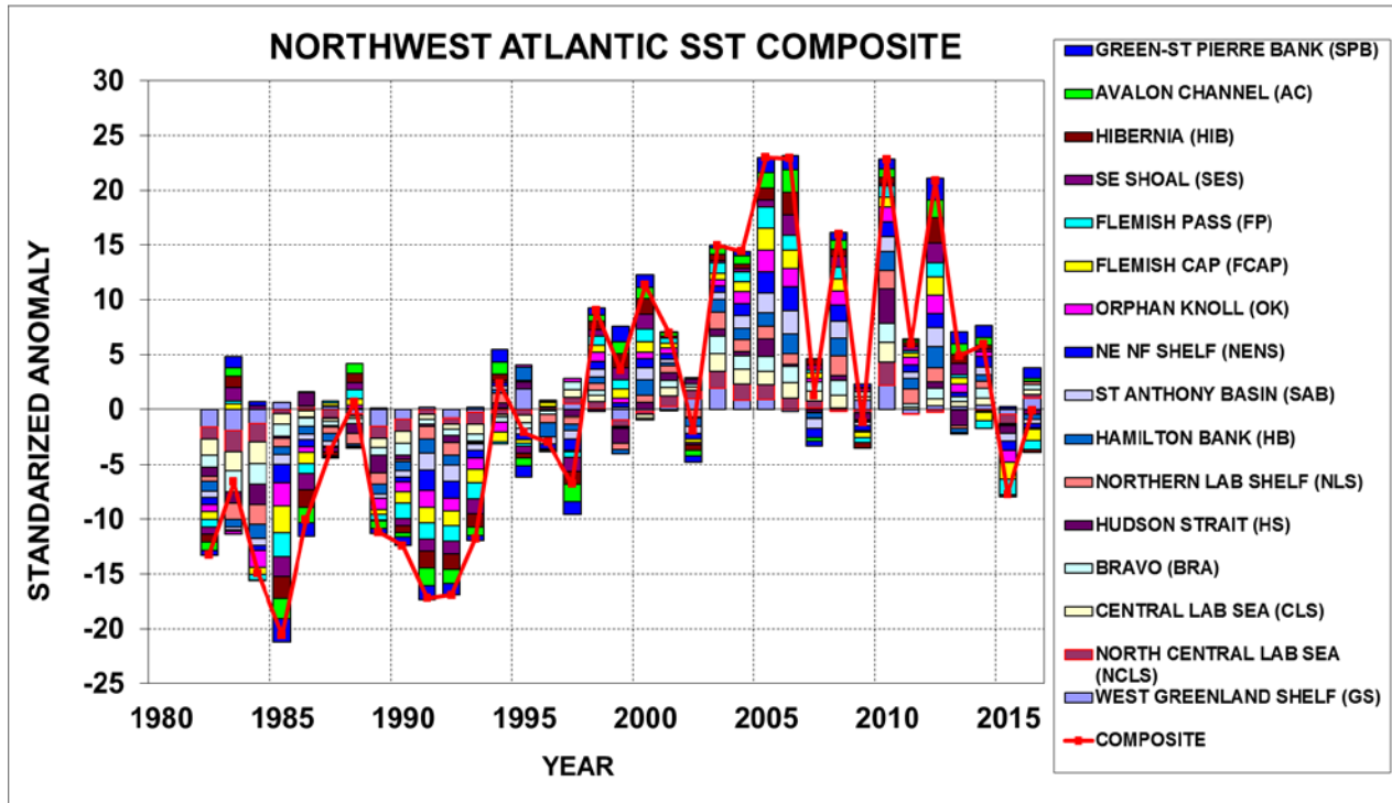
Figure 16 2 . Standardized annual SST anomalies from the subareas on the NL shelf presented in Figure 15. The solid red line represents the composite sum.
