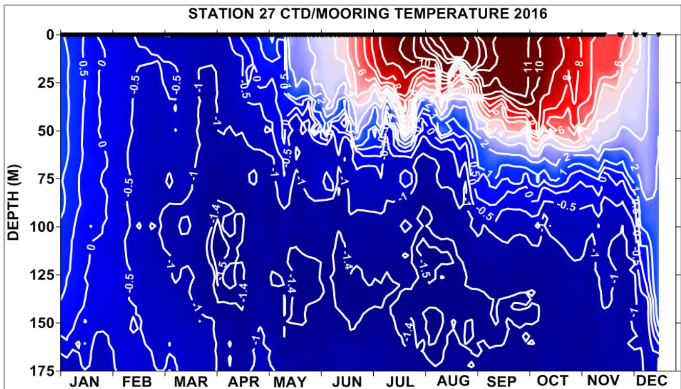
Figure 20. Contours of temperature ( ^{\circ}\text{C} ) as a function of depth at Station 27 during 2016. The symbols at the top indicate sampling times.
