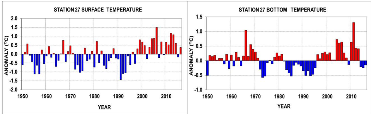
Figure 24. Annual Station 27 near-surface and near-bottom temperature anomalies referenced to the 1981-2010 mean.
