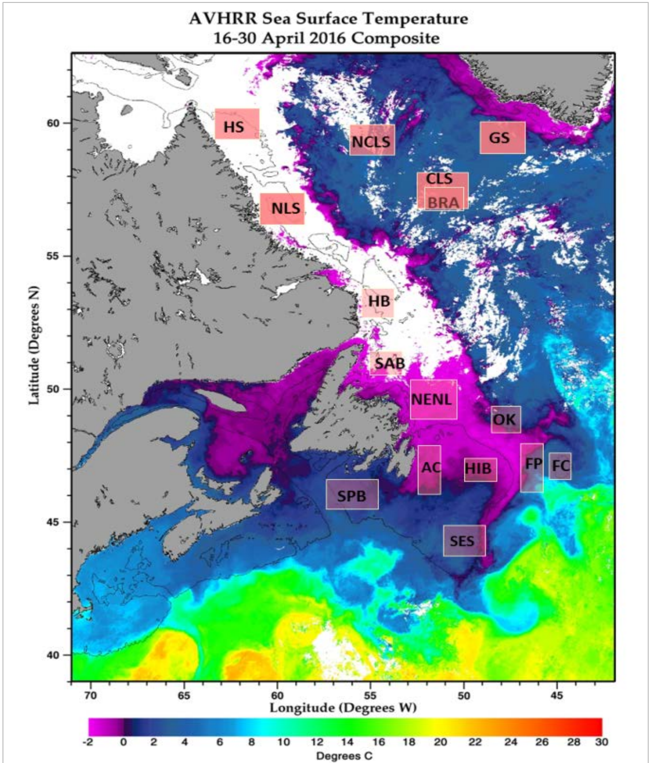
Figure 12. Map showing the April 16-30 SST and sea-ice extent and the subareas where SST time series were constructed for the Northwest Atlantic. (SST map courtesy of the Marine Ecosystem Section, BIO).
