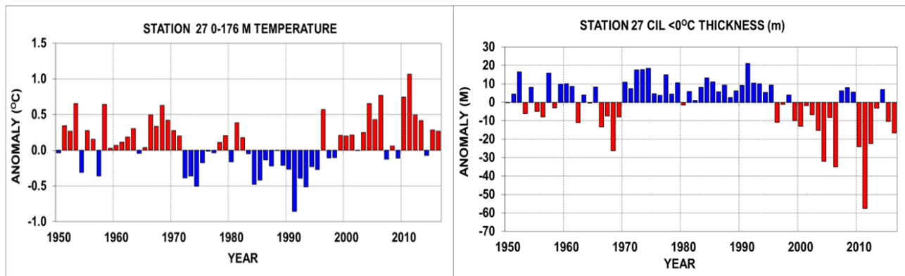
Figure 25. Annual Station 27 vertically averaged (0-176 m) temperature and CIL (<0°C) thickness anomalies referenced to the 1981-2010 mean.
