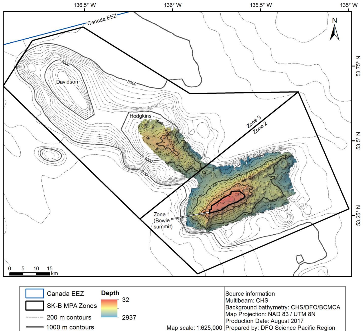
Figure 2. Sgaan Kinghlas Bowie Marine Protected Area boundaries and fishing zones. Zone 1 covers the peak of Bowie Seamount to approximately the 250 fathom (457 m) bathymetric contour, Zone 2 covers the rest of Bowie Seamount, and Zone 3 encompasses Hodgkins and Davidson Seamounts. High-resolution bathymetry from the Canadian Hydrographic Service (10–50 m resolution, color-shaded area on map) is only available for Bowie Seamount and part of Hodgkins Seamount and does not align perfectly with the less accurate 100 m resolution bathymetry (Gegr 2012) available for the remainder of the area.
