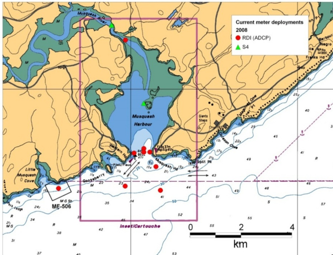
Figure 6. Locations of current meter deployments in the Musquash estuary area in 2008.
