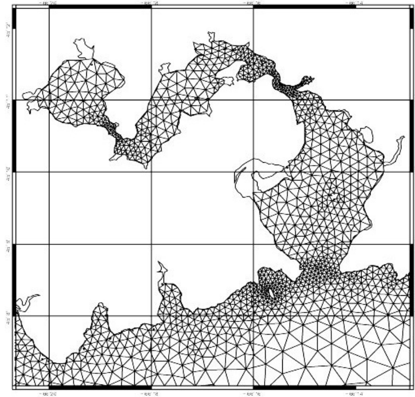
Figure 13. Model grid for the FVCOM circulation model in the Musquash area.
