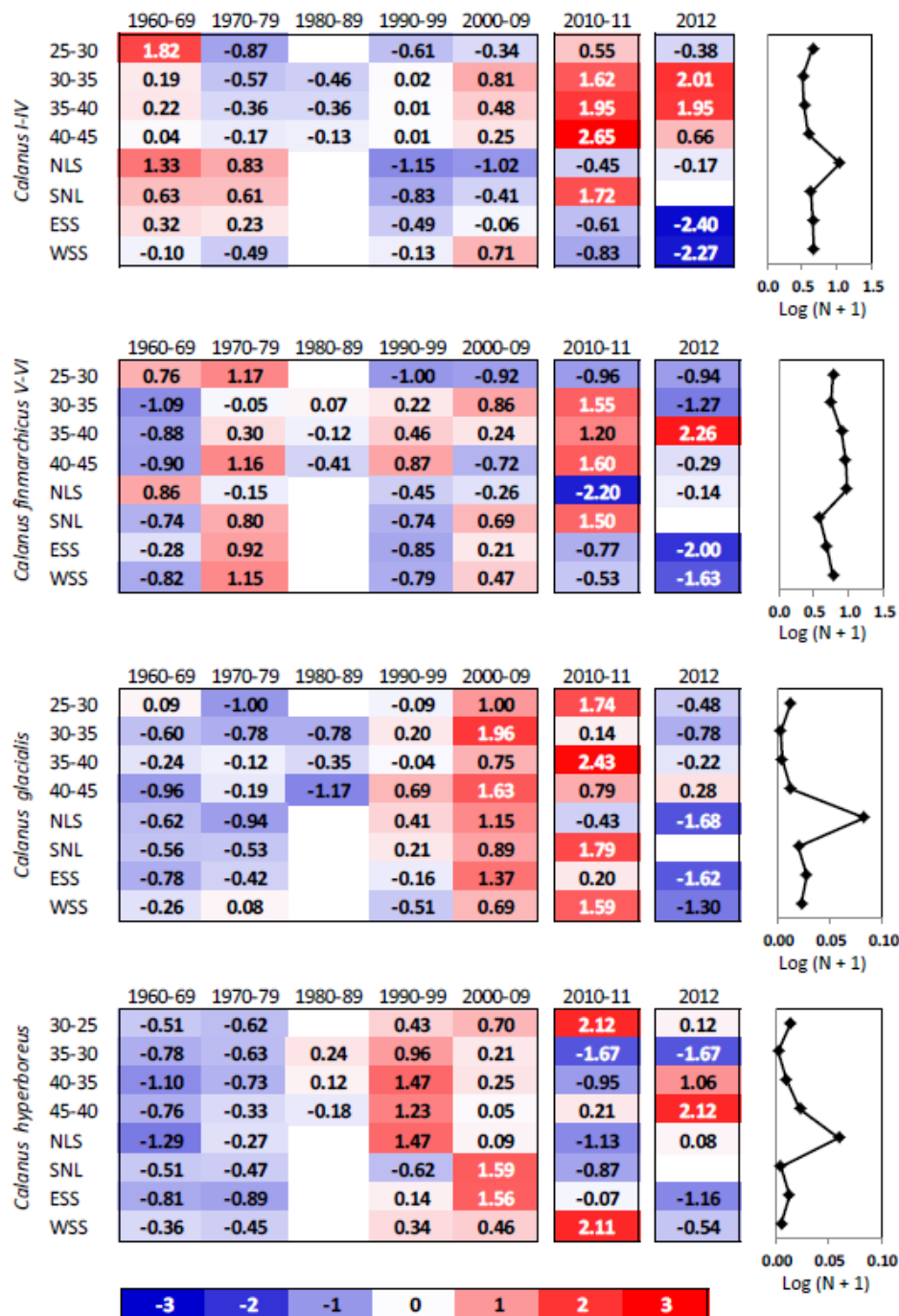
Figure 16: CPR time series for the annual average abundances for four Calanus taxa, calculated from monthly averages over decadal (1960-2009), bi-annual (2010-2011) or annual (2012) periods for eight regions in the Northwest Atlantic. Blank cells correspond to years or decades where sampling was too sparse to give annual values. Red (blue) cells indicate higher (lower) than normal values. The climatological averages were calculated from the decadal annual averages between 1960 and 2009, and are shown in the panels on the right. The numbers in the cells are the standardised anomalies. The regions are: Western Scotian Shelf (WSS), Eastern Scotian Shelf (ESS), South Newfoundland Shelf (SNL), Newfoundland Shelf (NS), and between longitudes 40-45°W, 35-40°W, 30-35°W, 25-30°W.
