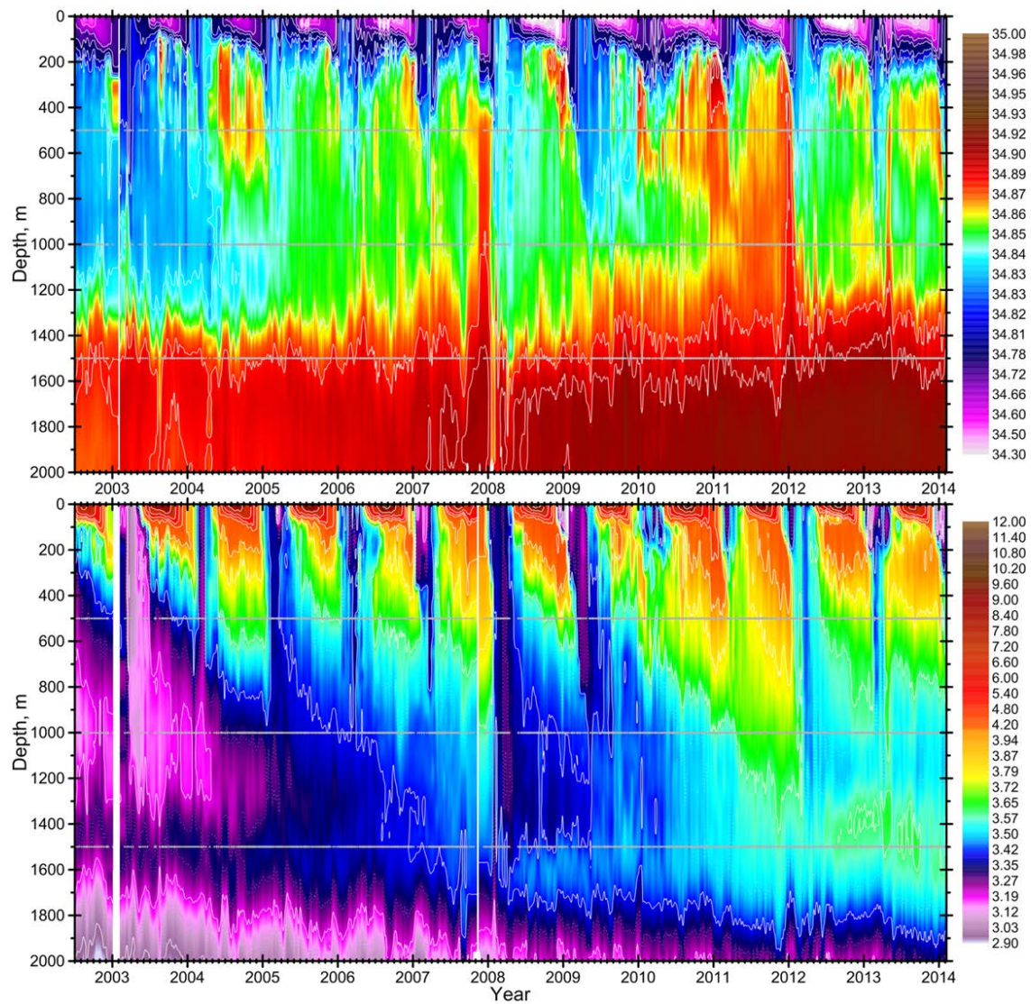
Figure 7: Salinity (top) and potential temperature (bottom) from Argo drifters in the Labrador Sea from 2002 to 2013. The winter 2008 deep convection event is clearly evident to a depth of 1600 m, and 2012 winter deep convection reaches 1400 m. Convection was limited to a depth of about 200 m in the winters of 2010 and 2011.
