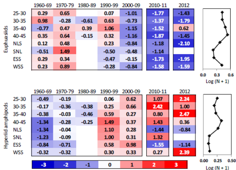
Figure 18: CPR time series for the annual average abundances for two macrozooplankton taxa, calculated from monthly averages over decadal (1960-2009), bi-annual (2010-2011) or annual (2012) periods for eight regions in the Northwest Atlantic. Blank cells correspond to years or decades where sampling was too sparse to give annual values. Red (blue) cells indicate higher (lower) than normal values. The climatological averages were calculated from the decadal annual averages between 1960 and 2009, and are shown in the panels on the right. The numbers in the cells are the standardised anomalies. The regions are: Western Scotian Shelf (WSS), Eastern Scotian Shelf (ESS), South Newfoundland Shelf (SNL), Newfoundland Shelf (NS), and between longitudes 40-45°W, 35-40°W, 30-35°W, 25-30°W.
