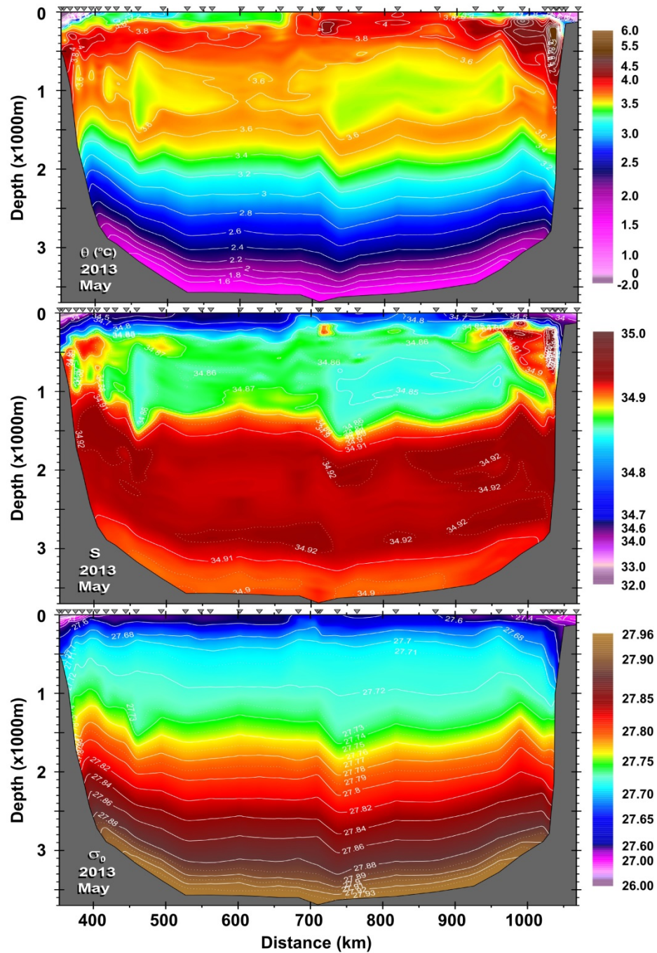
Figure 8a: Labrador Sea (AR7W Section) potential temperature (top row), salinity (middle row) and potential density (bottom row).
