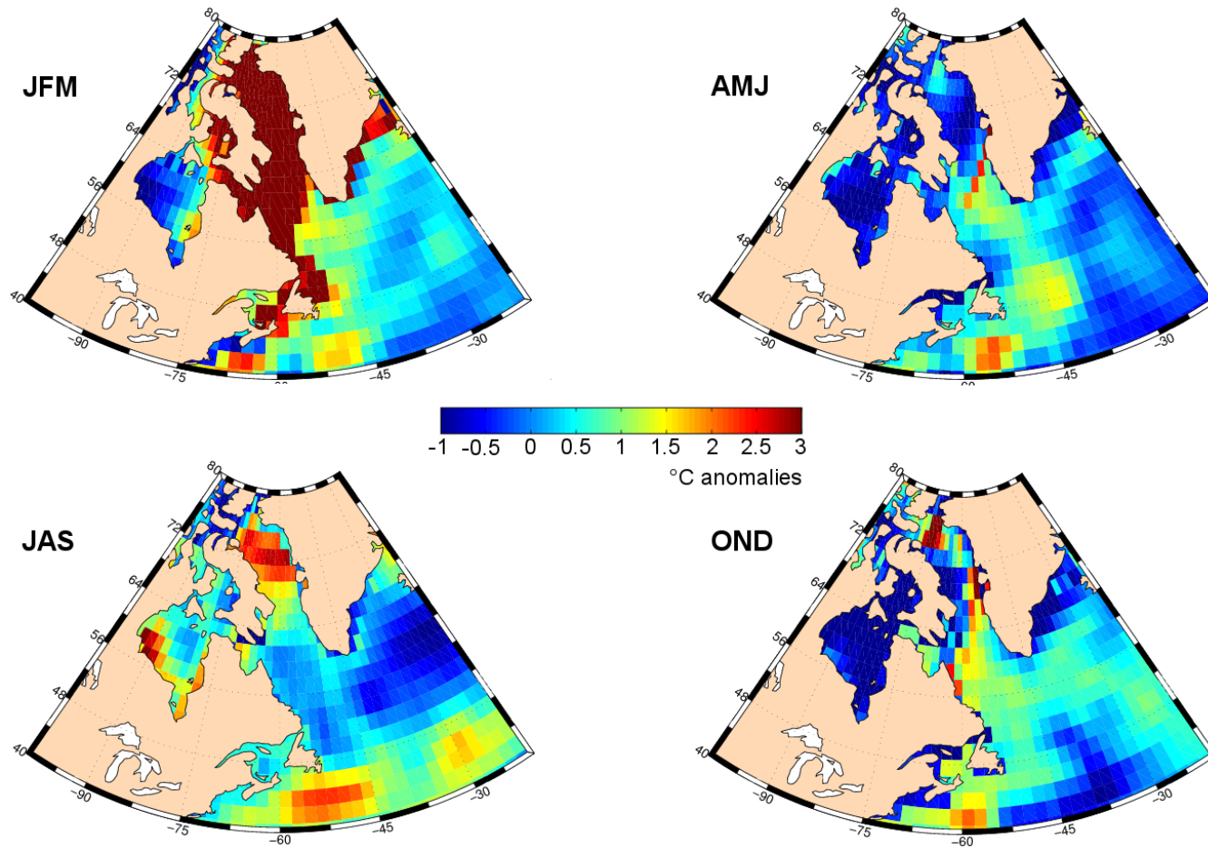
Figure 4: Sea surface temperature (SST) anomalies for winter (JFM), spring (AMJ), summer (JAS) and fall (OND) 2013 derived from NCEP/NCAR reanalysis .
