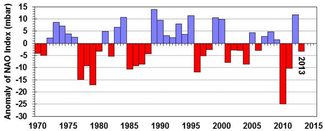
Figure 2: Average sea level pressure for DJF in mbar (winter NAO Index from 1970 to 2013).
