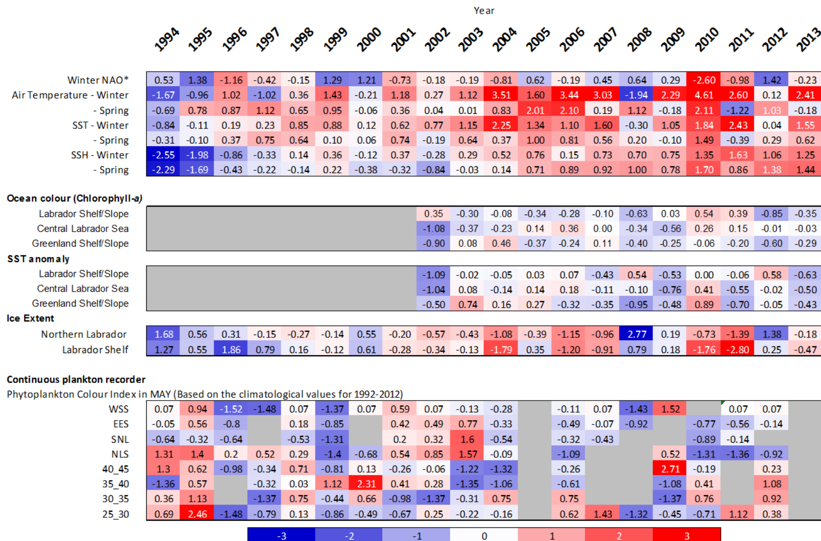
Figure 21: Normalised annual and/or seasonal anomaly of physical and biological variables integrated over large spatial scales estimated using NCEP, remote sensed data or CPR between 1994 and 2013.
