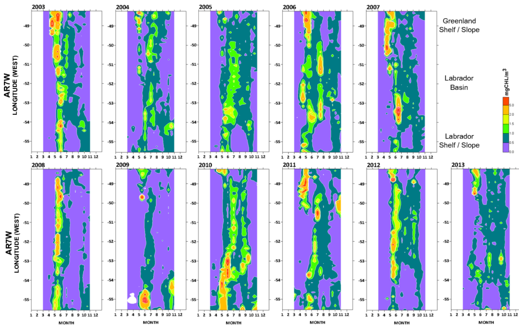
Figure 10: The concentration of sea surface chlorophyll estimated from remotely-sensed ocean colour at 2-week intervals from March to October spanning a 10-year time series, 2003-2013.
