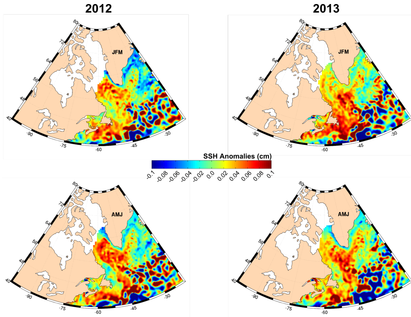
Figure 5: Weekly merged sea surface height anomalies for winter (JFM) and spring (AMJ) 2012 and 2013 from AVISO an objectively mapped product of TOPEX/Poseidon/Jason-1, ERS-1, ERS-2, Geosat-Follow.
