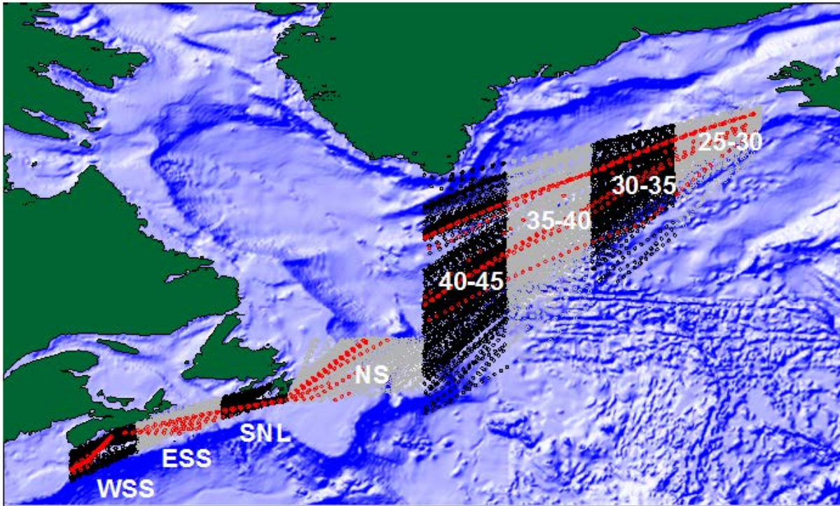
Figure 14: CPR lines and stations 1957 to 2012. Stations sampled in 2012 are shown in red. Data are analysed by region. Regions are: Western Scotian Shelf (WSS), Eastern Scotian Shelf (ESS), South Newfoundland Shelf (SNL), Newfoundland Shelf (NS), and between longitudes 40-45°W, 35-40°W, 30-35°W, 25-30°W.
