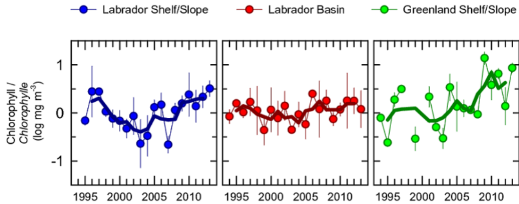
Figure 12: Upper ocean ( z < 100 m) average concentrations of phytoplankton on AR7W sampled in spring or early summer from 1994 to 2013. Circles indicate mean value for stations designated within each region, error bars indicate among-station standard deviation, and heavy line indicates 3-year running average of the time series.
