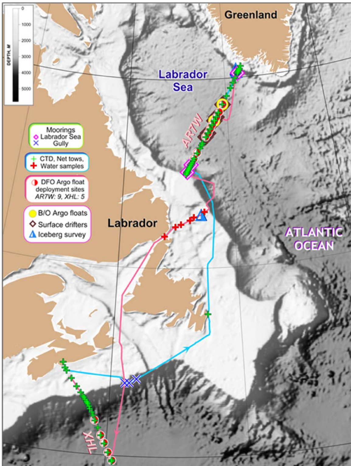
Figure 1: Schematic of the Labrador Sea component of the DFO AZOMP. Standard stations along the section are shown as green plus signs and red ones indicate the added shelf stations south of the pack ice. Location of Argo profiler deployments are indicated by the red/white circles. Yellow circles indicate BIO Argos deployments.
