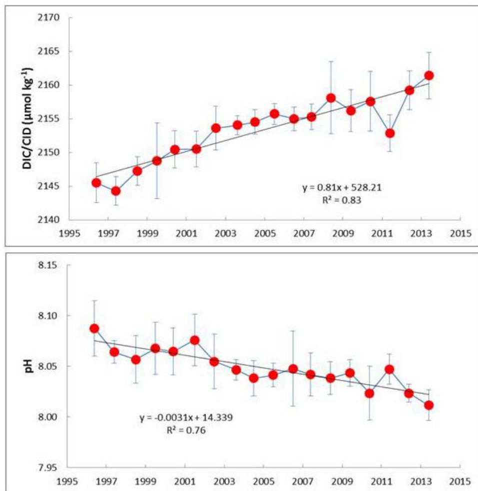
Figure 9: Time series of TIC and pH, top panel for TIC, bottom panel from pH. TIC and pH in in the 150–500 m depth range and corresponding regression lines for stations in the central part of the Labrador Basin for the period 1996–2013.
