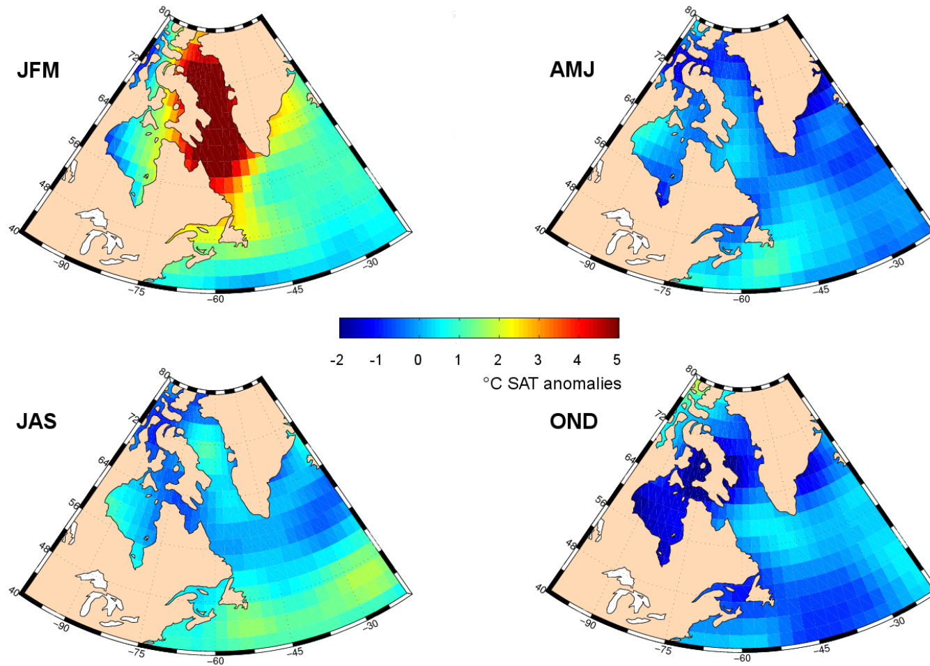
Figure 3: Surface air temperature anomaly for winter (JFM), spring (AMJ), summer (JAS) and fall (OND) periods in 2013 as derived from NCEP/NCAR reanalysis .
