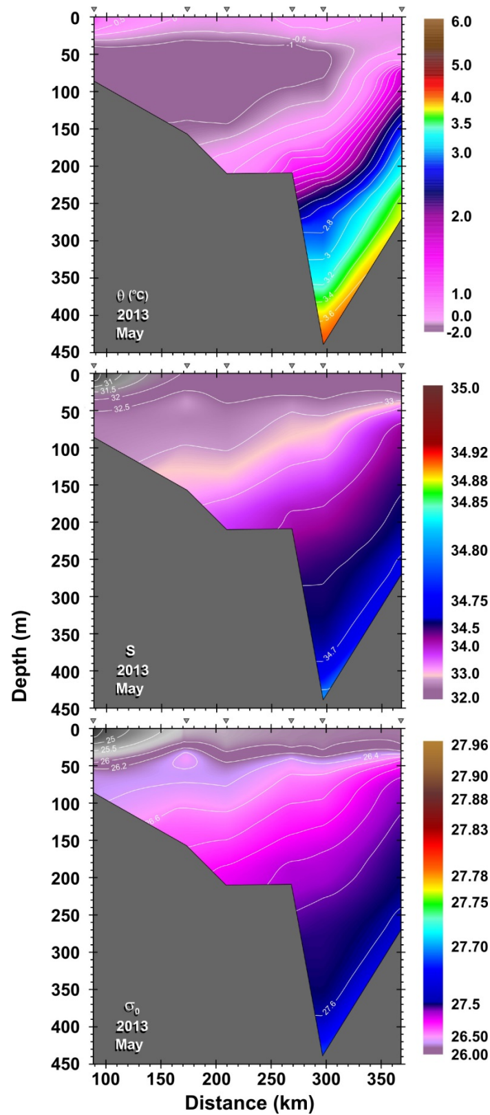
Figure 8b: Belle-Isle Strait new line potential temperature (top row), salinity (middle row) and density (bottom row). This section was added to cover the shelf area of Hamilton Bank that was inaccessible because of heavy ice concentration on the AR7W line.
