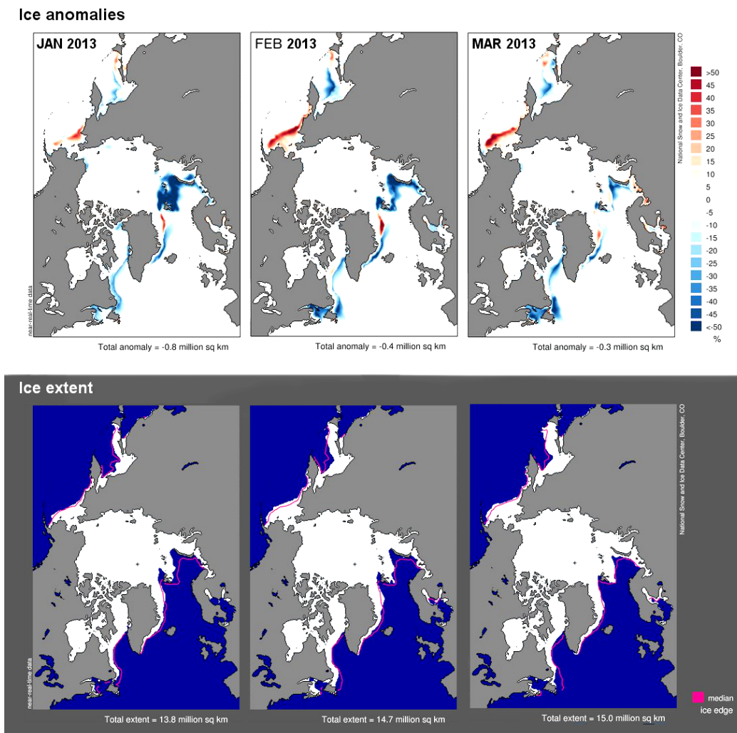
Figure 6: Sea ice concentration anomalies (top panel) and sea ice extent (bottom panel) for January-March 2013 as derived by the US National Snow and Ice Data Center (reference period 1979-2000).
