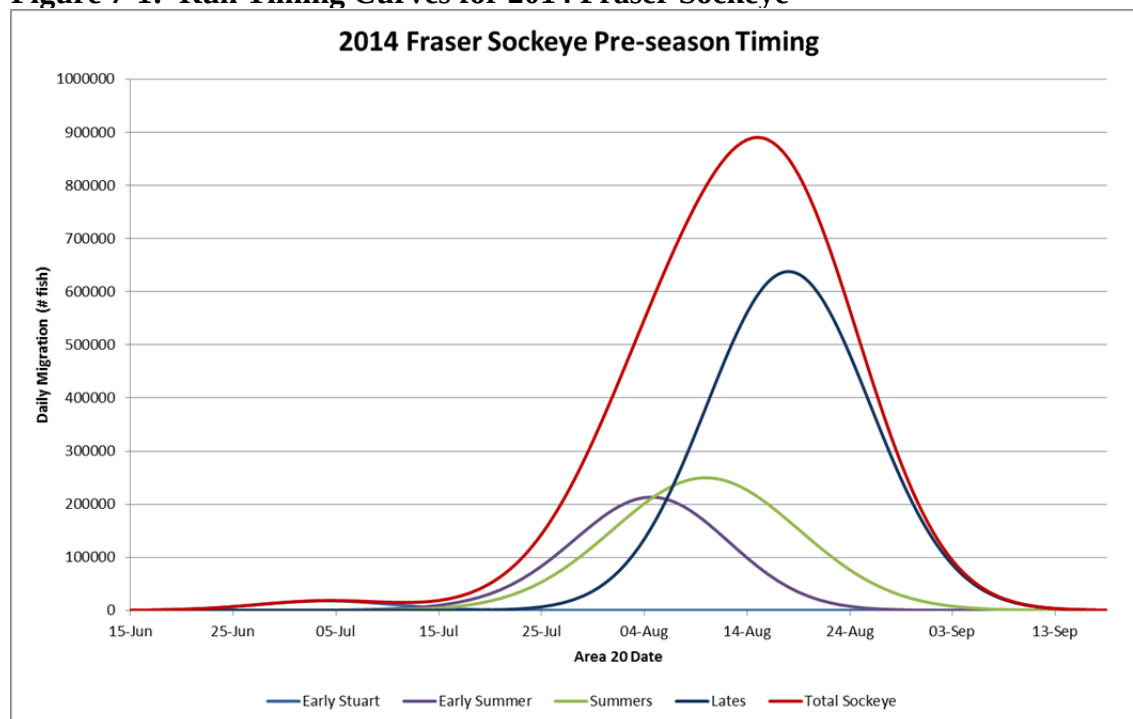
Figure 7-1: Run Timing Curves for 2014 Fraser Sockeye
