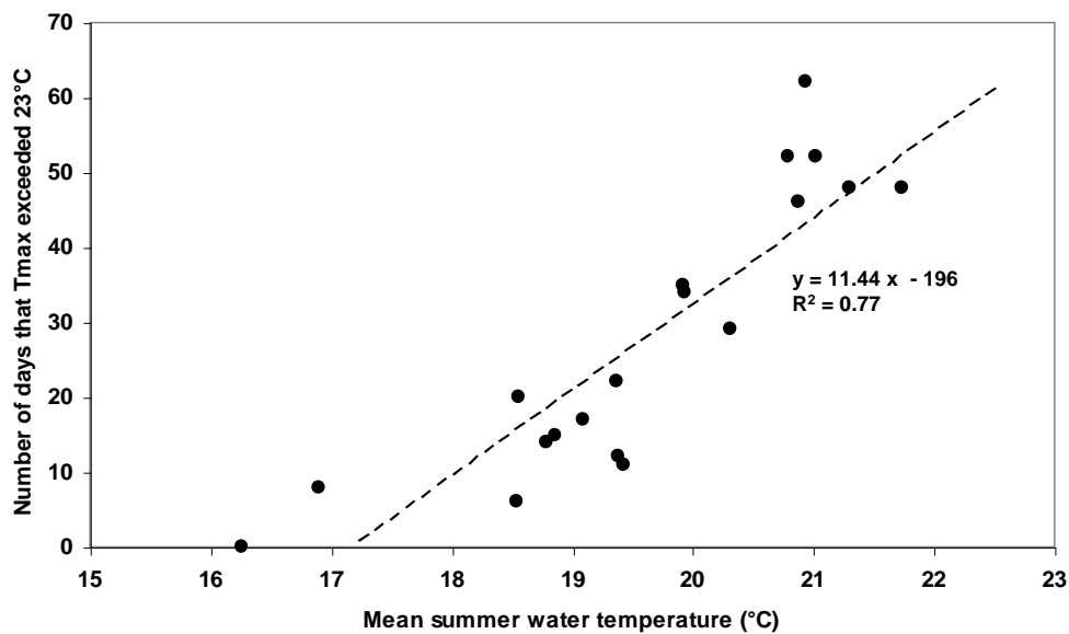
Figure 13-4 The number of days that T_{\max} exceeded 23^{\circ}\text{C} as a function of the mean summer water temperature for the Little Southwest Miramichi River (1992-2011, missing 1994).
