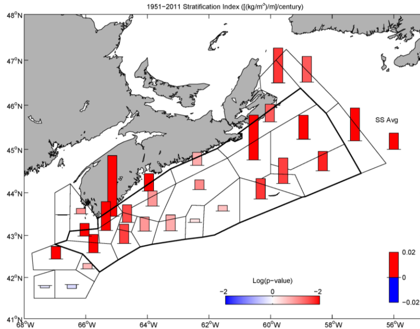
Figure 4-8 Stratification index trend ((kg/m 4 )/century) for 1951-2011, using the same format as Fig. 4-6.
