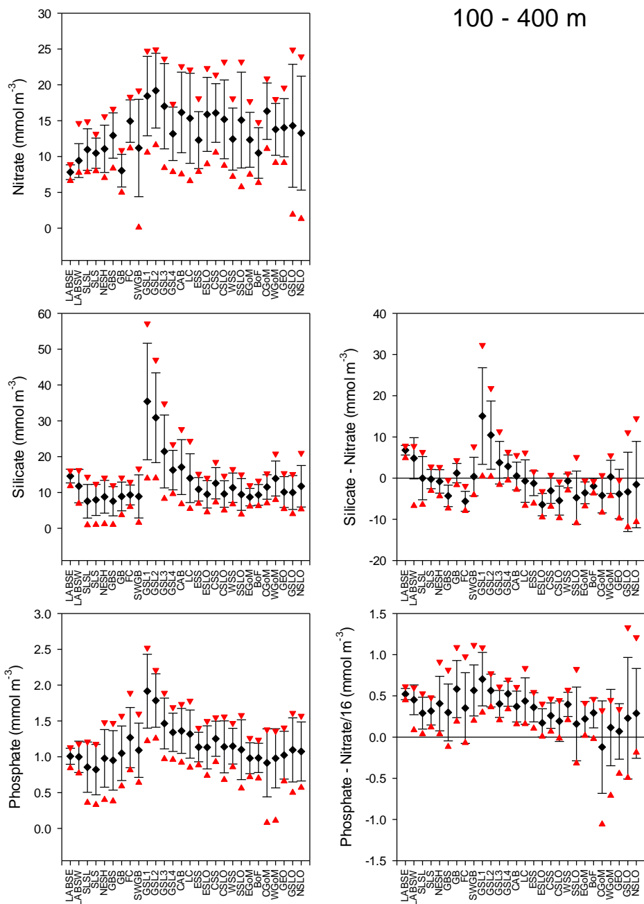
Figure 10-3 Descriptive statistics (overall mean, black symbol; standard deviation, black lines; 10th and 90th percentiles, red triangles) of nitrate concentrations in the lower (100 – 400 m) water column all the observations for all geographic areas.
