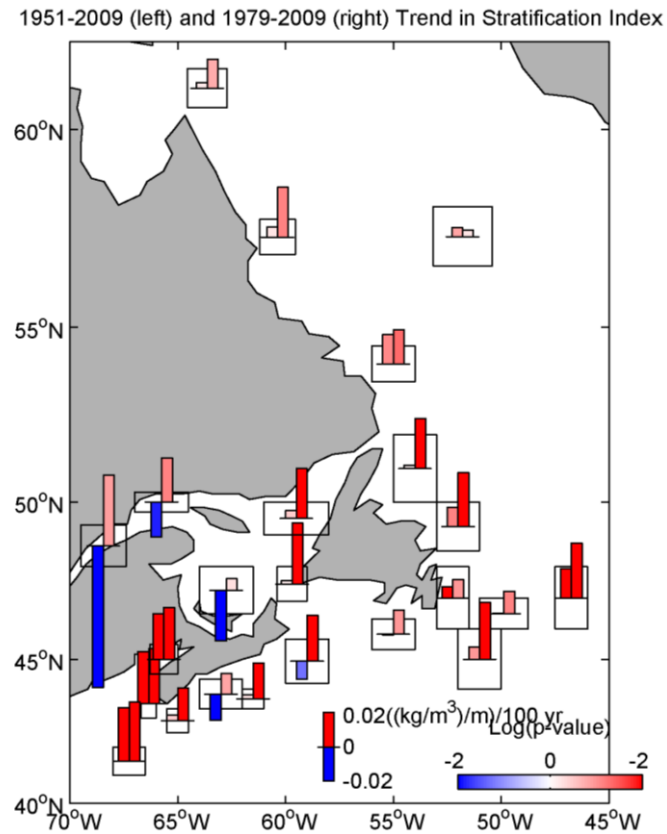
Figure 3-4 Stratification index trend ( (\text{kg}/\text{m}^3)/\text{century} ) for the 1951-2009 and 1979-2009 periods. The size of the bar is proportional to the trend. The intensity of the colour of the bar (red for increasing trend; blue for decreasing trend) indicates the p-value.
