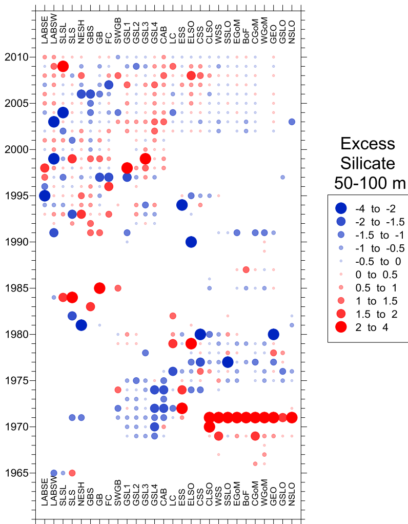
Figure 10-10 Annual standardized anomalies of average regional excess silicate concentrations (Si – N) in the upper (50 – 100 m) water column 1965 – 2010. Blue symbols represent values below the long term average for each region; red symbols represent values above the long term average. The size of the symbols reflects the magnitude of the departure of that year's average (in terms of the standard deviation of the time series of annual averages) from the long term average for the region.
