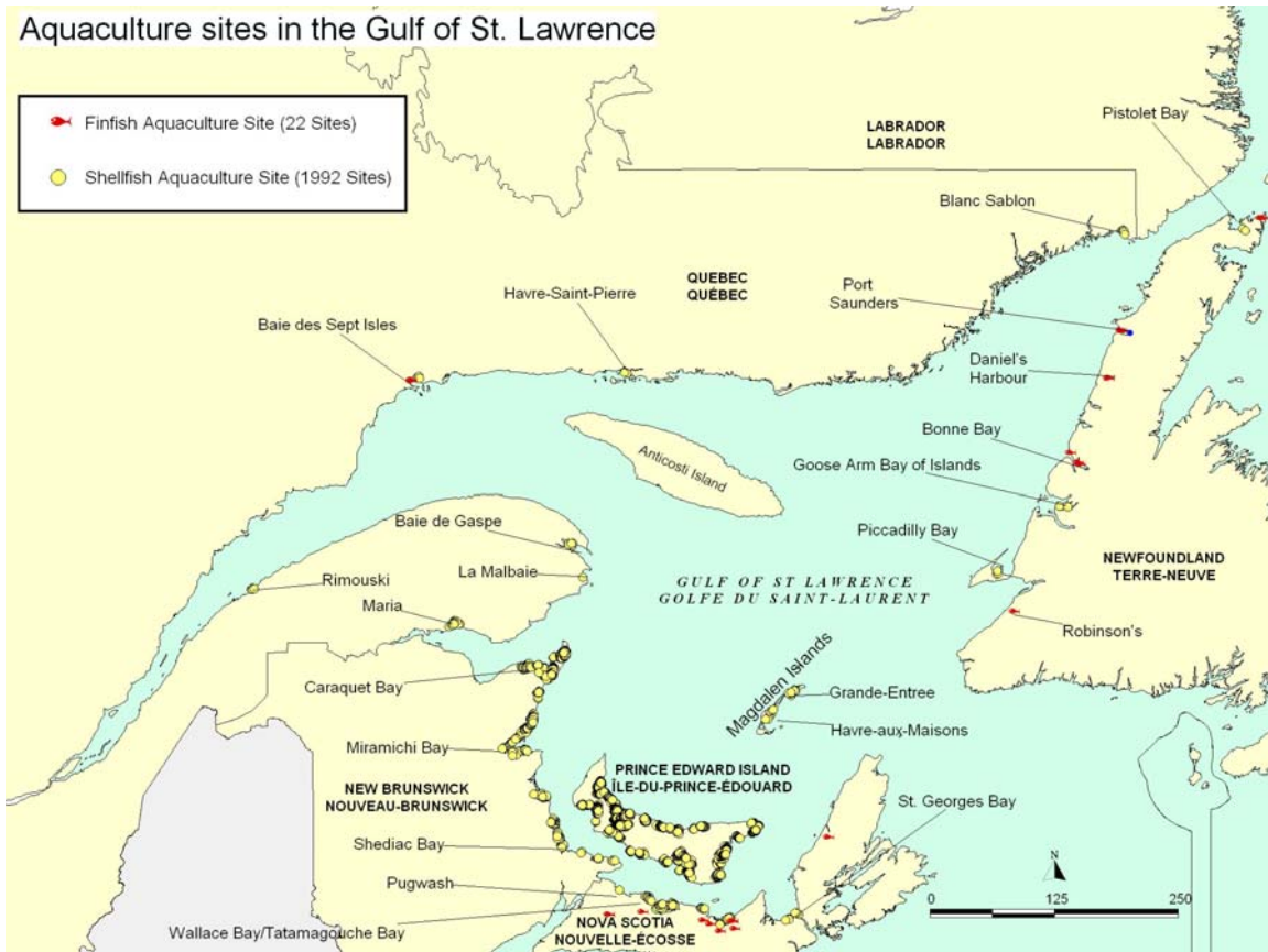
Figure 4-15 Distribution of aquaculture sites in the Gulf of St. Lawrence. 2003.
