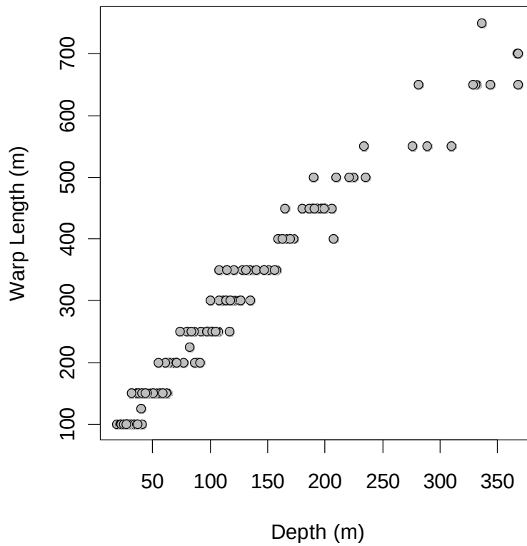
Figure 7. Warp length vs. starting depth.
