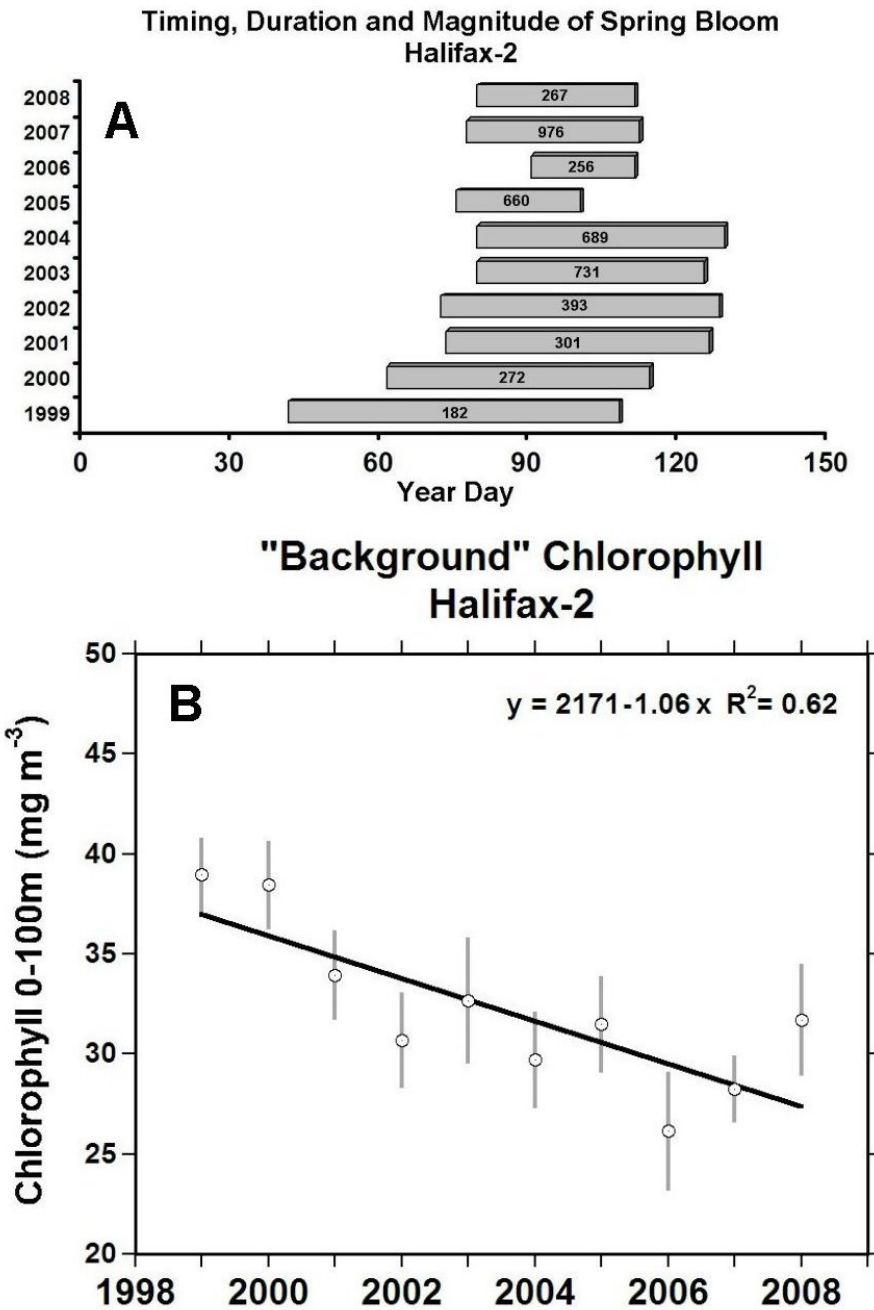
Figure 15. Dynamics of the spring phytoplankton bloom at the Halifax-2 fixed station, 1999-2008: (A) timing, duration (based on 40 mg CHL m 2 threshold for determining start and end of the bloom), and magnitude (numbers inside horizontal bars); (B) "background" chlorophyll levels, i.e. outside of spring bloom periods (annual averages +/- SE, line = least squares linear regression).
