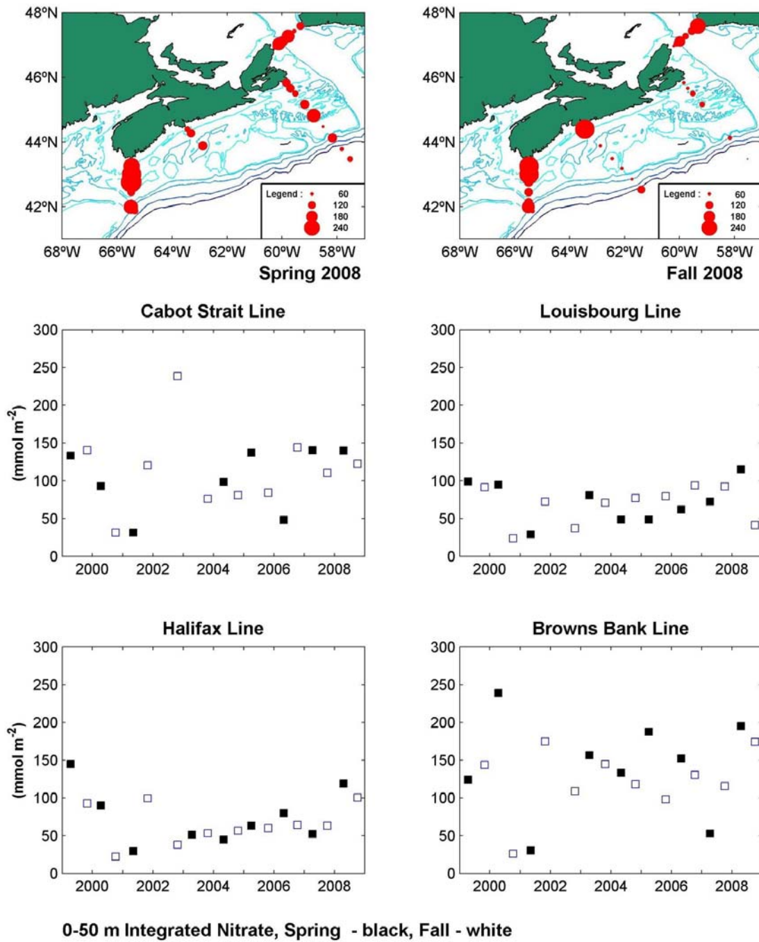
Figure 11a. Time series of line-averaged inventories of nitrate in the upper water column (0-50 m) for the spring and fall Scotian Shelf sections, 1999-2008.
