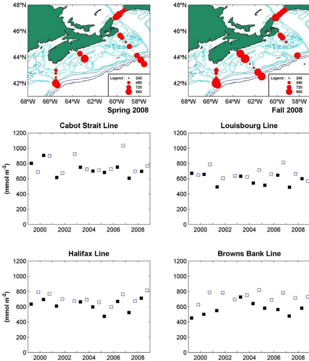
50-150 m Integrated Nitrate, Spring - black, Fall - white
