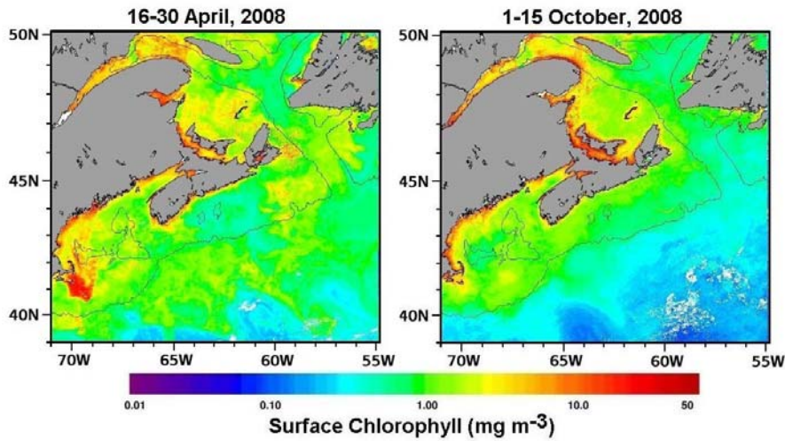
Figure 20. MODIS twice monthly composite images of surface chlorophyll in the Maritimes/Gulf regions: during the spring (April) and fall (October) shelf surveys in 2008. See Figure 2 for station locations.
