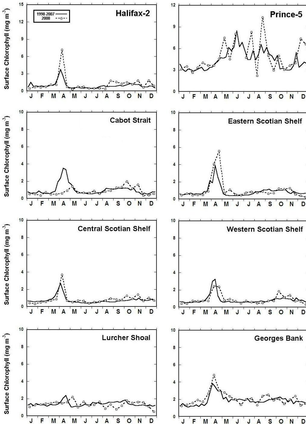
Figure 23. Seasonal variability in surface chlorophyll concentrations (from SeaWiFS 4 km weekly ocean colour data) for the fixed stations and statistical sub-regions of the Maritimes Region (see Figure 5). Solid lines represent mean (1998-2007) levels, dashed lines represent 2008 levels. Note: the spring and summer data gaps in the 2008 SeaWiFS data record (see Methods Section) were filled with adjusted MODIS data.
