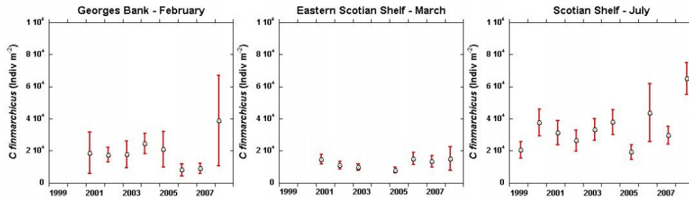
Figure 31. Zooplankton biomass and Calanus finmarchicus abundance from trawl (groundfish) surveys on Georges Bank (February), the eastern Scotian Shelf (March) and the Scotian Shelf and eastern Gulf of Maine (summer): upper panels in each set show 2008 spatial distributions, lower panels in each set show survey mean biomass or abundance, 1999-2008 (vertical bars are standard errors).
