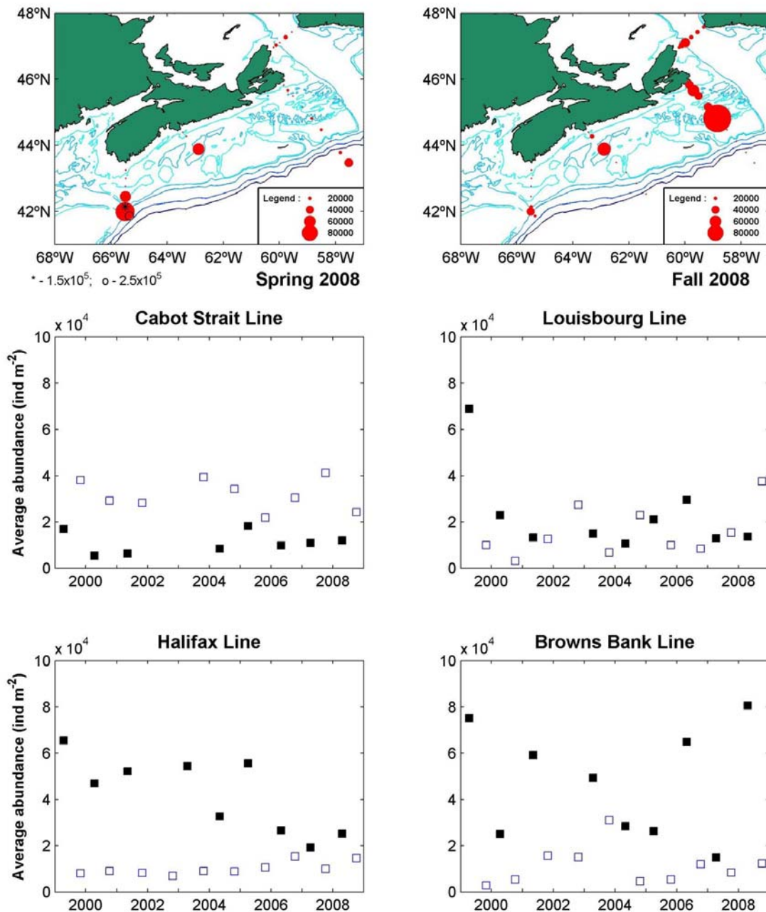
C. finmarchicus abundance, Spring - black, Fall - white
