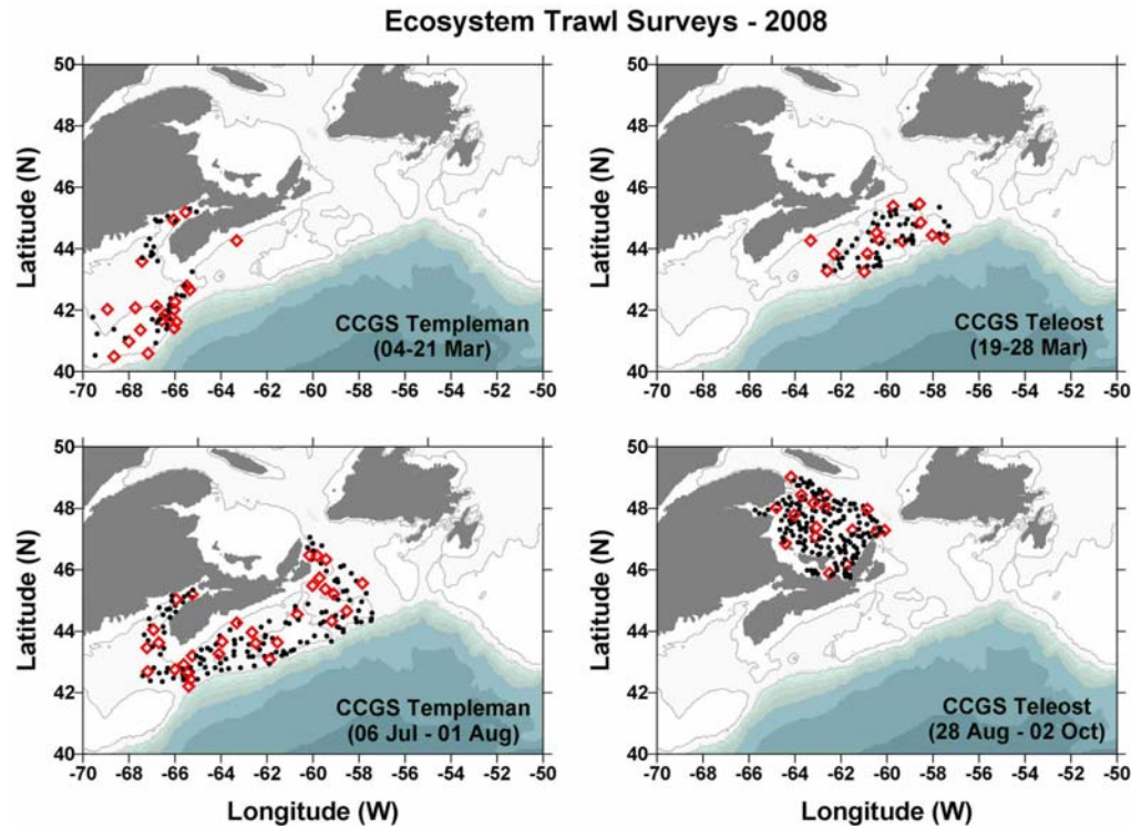
Figure 3. Stations sampled during major Maritimes/Gulf trawl (groundfish) surveys in 2008. Black symbols are hydrographic stations; red symbols are stations where vertical nets hauls were taken in addition to hydrographic measurements.
