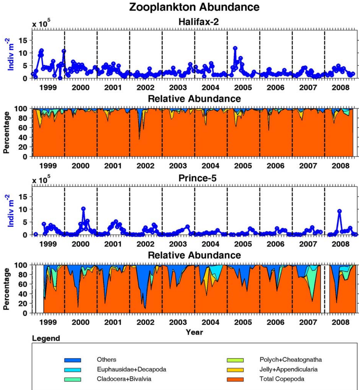
Figure 27. Time series of zooplankton (>200 \mu\text{m} ) abundance and community composition at the Maritimes fixed stations, 1999-2008.
