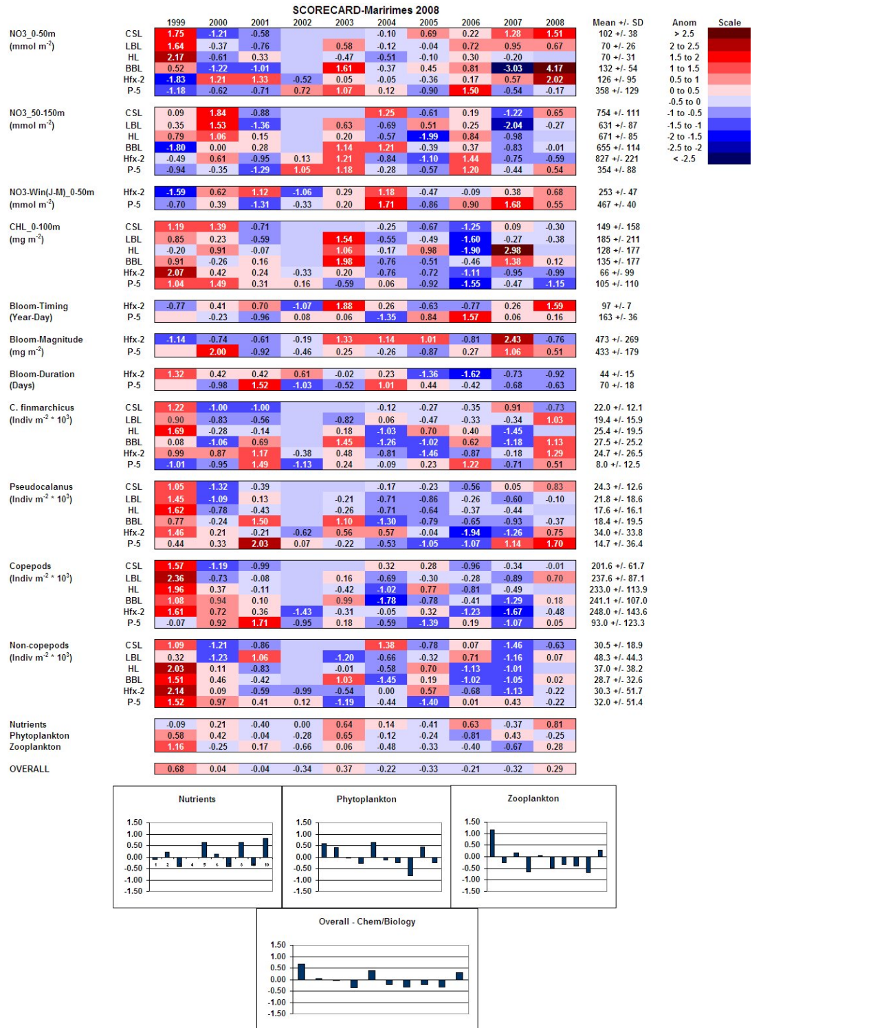
Figure 32. Maritimes Region scorecard: time series of chemical and biological variables, 1999-2008. A grey cell indicates missing data. Red cells indicate higher than normal nutrient, phytoplankton, zooplankton levels or later and longer than normal duration of phytoplankton blooms. Blue cells indicate lower than normal nutrient, phytoplankton, zooplankton levels, or earlier and shorter than normal bloom duration. More intense colours indicate larger anomalies, in increments of \pm 0.5 standard deviation of the long-term mean based on data from the reference period 1999- 2006. The numbers in the cells are the anomaly values (differences from the long-term means divided by the standard deviations). CSL: Cabot Strait Line; LBL: Louisbourg Line; HL: Halifax Line; BBL: Browns Bank Line.
