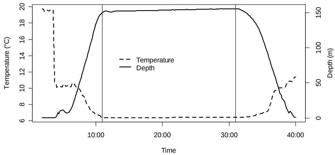
Figure 11. Seabird 39 temperature and depth profile from tow number 1. The vertical lines indicate the start and end of net contact with the sea floor.
