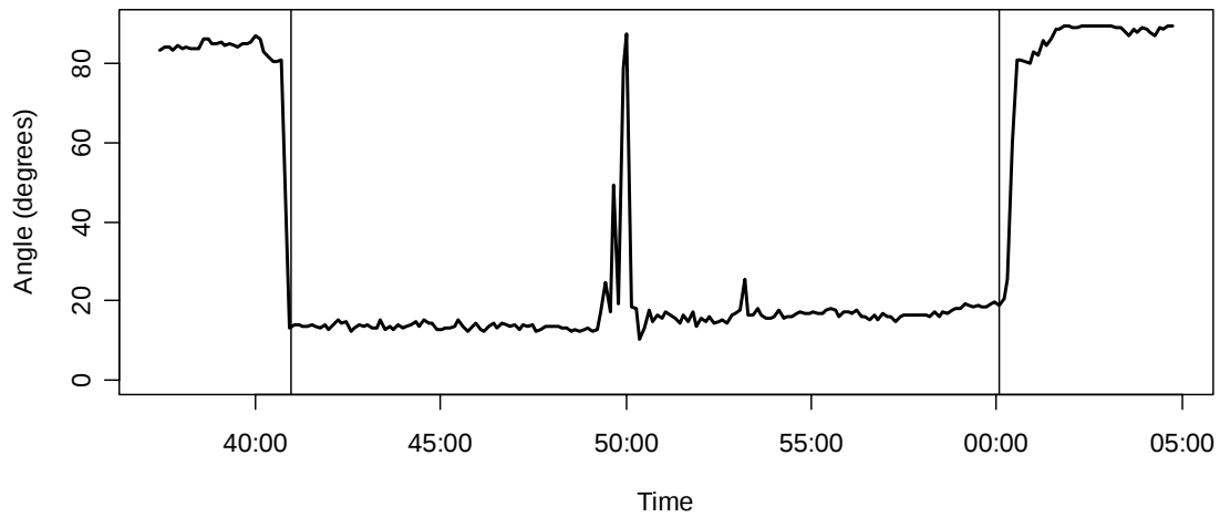
Figure 12. NMFS bottom contact sensor profile from tow number 25. The vertical lines indicate the start and end of net contact with the sea floor.
