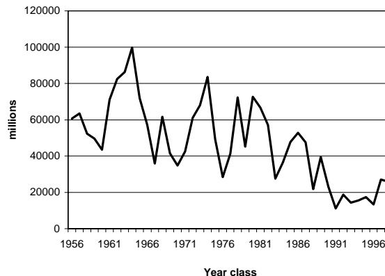
Figure 8. Recruitment (numbers at age 3).
