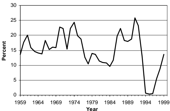
Figure 9. Exploitation rate.
