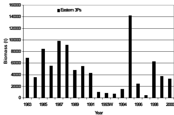
Figure 5. 3Ps survey biomass index (t).
