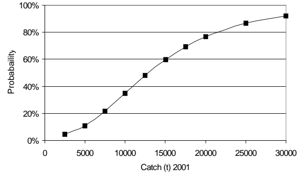
Figure 13. Risk of spawning stock biomass declining for the eastern 3Ps area.
