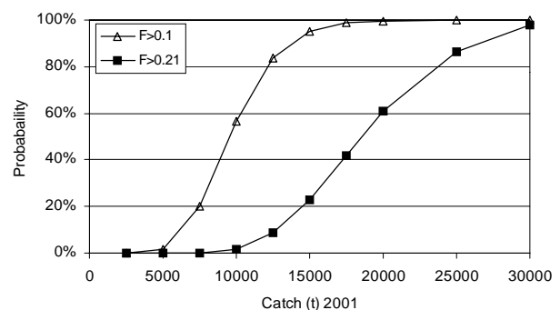
Figure 10. Risk of exceeding 0.1 and 0.21 fishing mortality.
