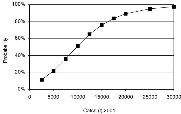
Figure 11. Risk of spawning stock biomass declining.
