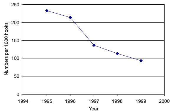
Figure 6. Standardized sentinel catch rates for gill nets (upper panel) and line-trawls (lower panel).
