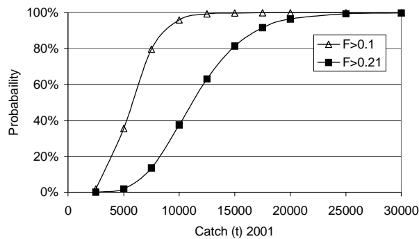
Figure 12. Risk of exceeding 0.1 and 0.21 fishing mortality for the eastern 3Ps area.
