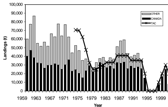
Figure 1. Reported landings (t) by country.
