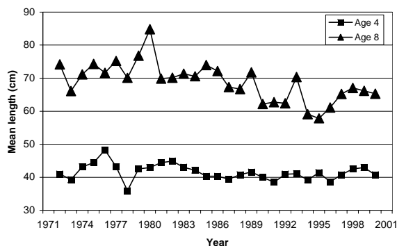
Figure 4. Mean lengths (cm) at age from RV survey.
