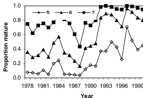
Figure 3. Estimated proportion mature at ages 5-7 (females).
