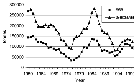
Figure 7. Spawner biomass and 3+ biomass.
