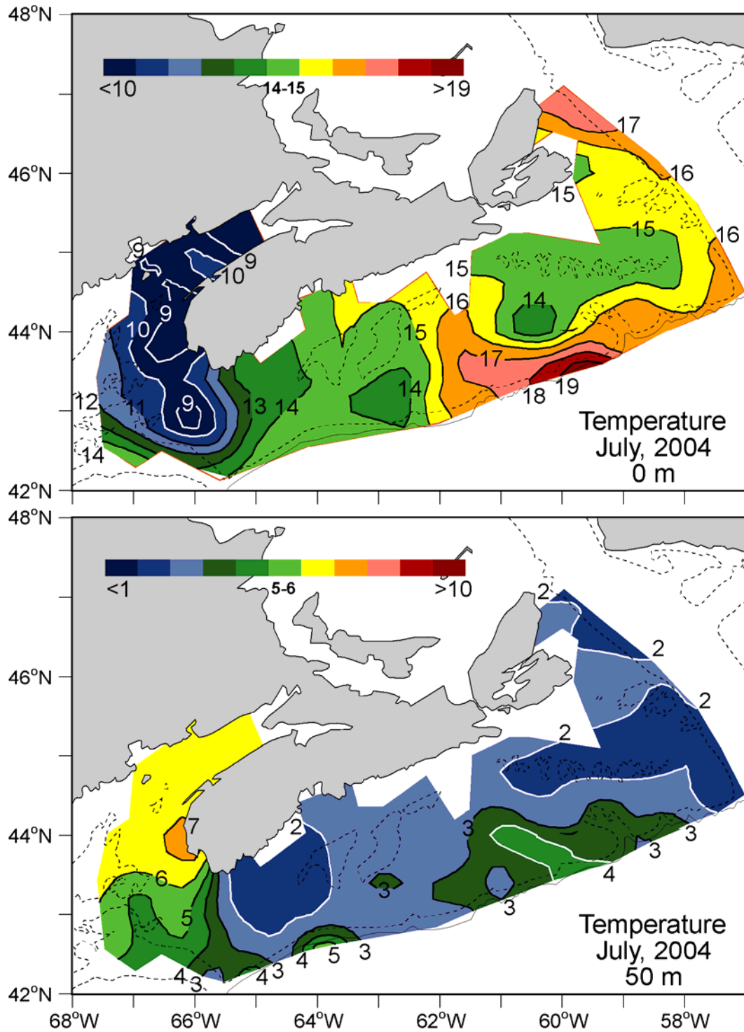
Fig.10a. Contours of temperatures at the surface (top panel) and 50 m (bottom panel) during the 2004 July groundfish and ITQ surveys.
