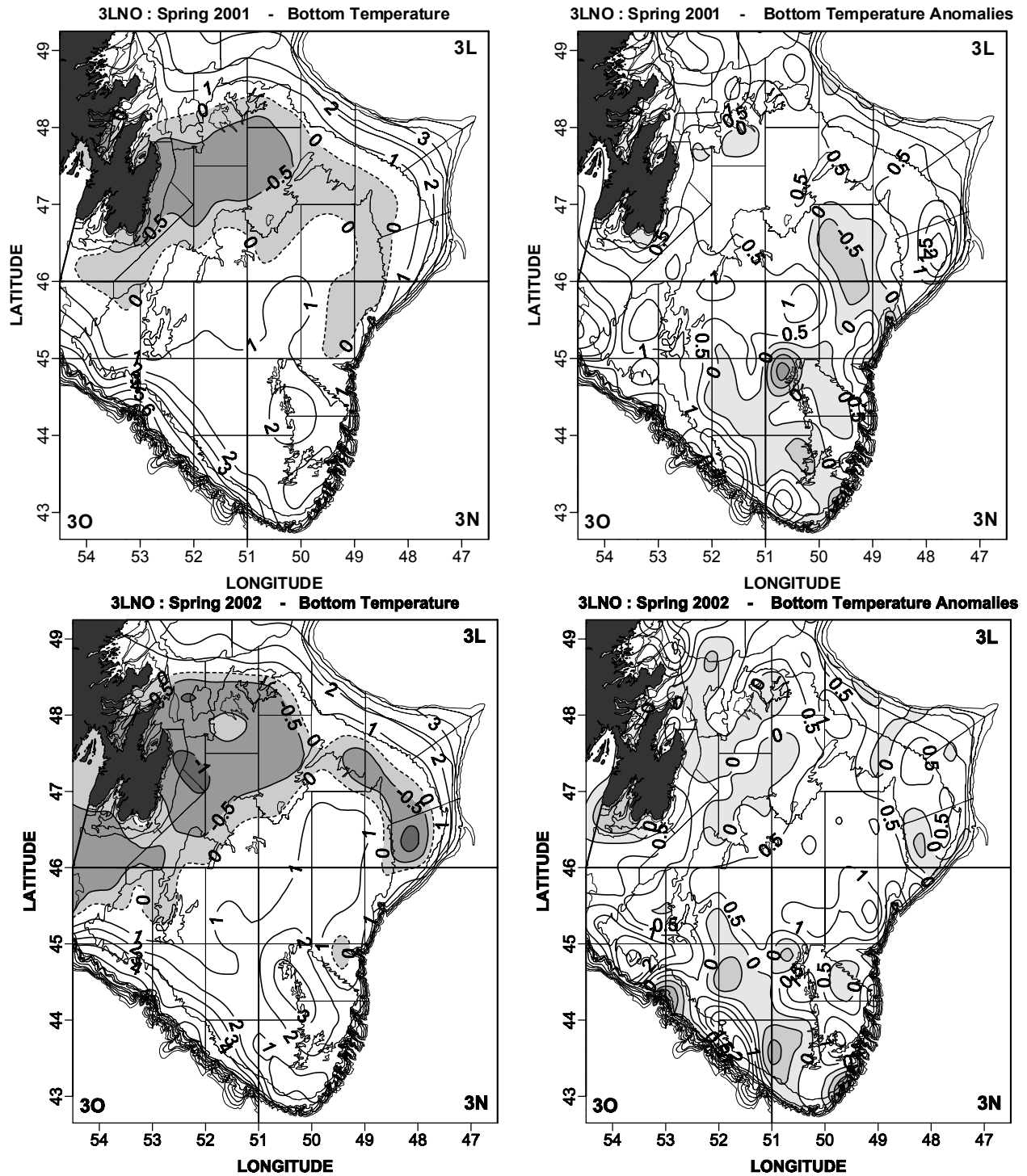
Fig. 24. Contours of bottom temperature and their anomalies (in °C) for the spring of 2001 and 2002 from the multi-species survey of NAFO Divs. 3LNO.
