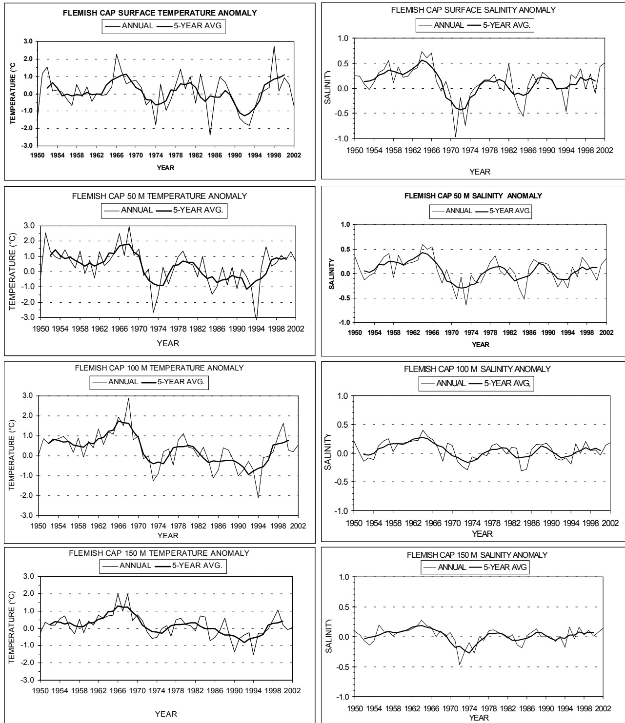
Fig. 6. Annual temperature anomalies (left panels) and salinity anomalies (right panels) on the Flemish Cap in NAFO Division 3M at selected water depths. The heavy lines are the 5-year running means.
