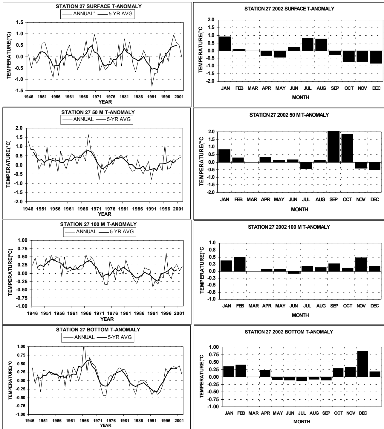
Fig. 3. Station 27 annual temperature anomalies and their 5-year running means at selected depths (left panels) and monthly temperature anomalies (right panels) for 2002.
