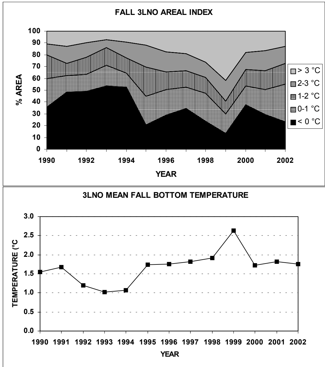
Fig. 27. Time series of the percentage area of the bottom in NAFO Divs. 3LNO covered by water with temperatures \leq 0^{\circ}\text{C} , 0-1^{\circ}\text{C} , 1-2^{\circ}\text{C} , 2-3^{\circ}\text{C} and \geq 3^{\circ}\text{C} during the fall (upper panel) and the mean bottom temperature in ^{\circ}\text{C} (bottom panel).
