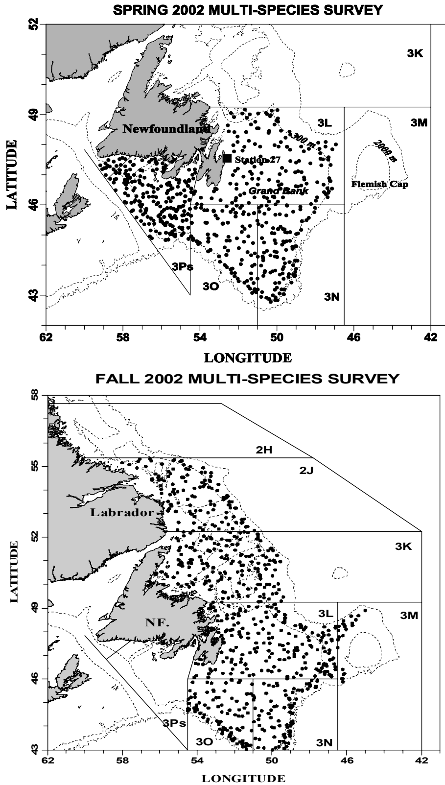
Fig. 1c. Location maps showing the positions of sets with oceanographic data from the multi-species surveys during the spring and fall of 2002. Bathymetry contours are 300 and 1000 m.
