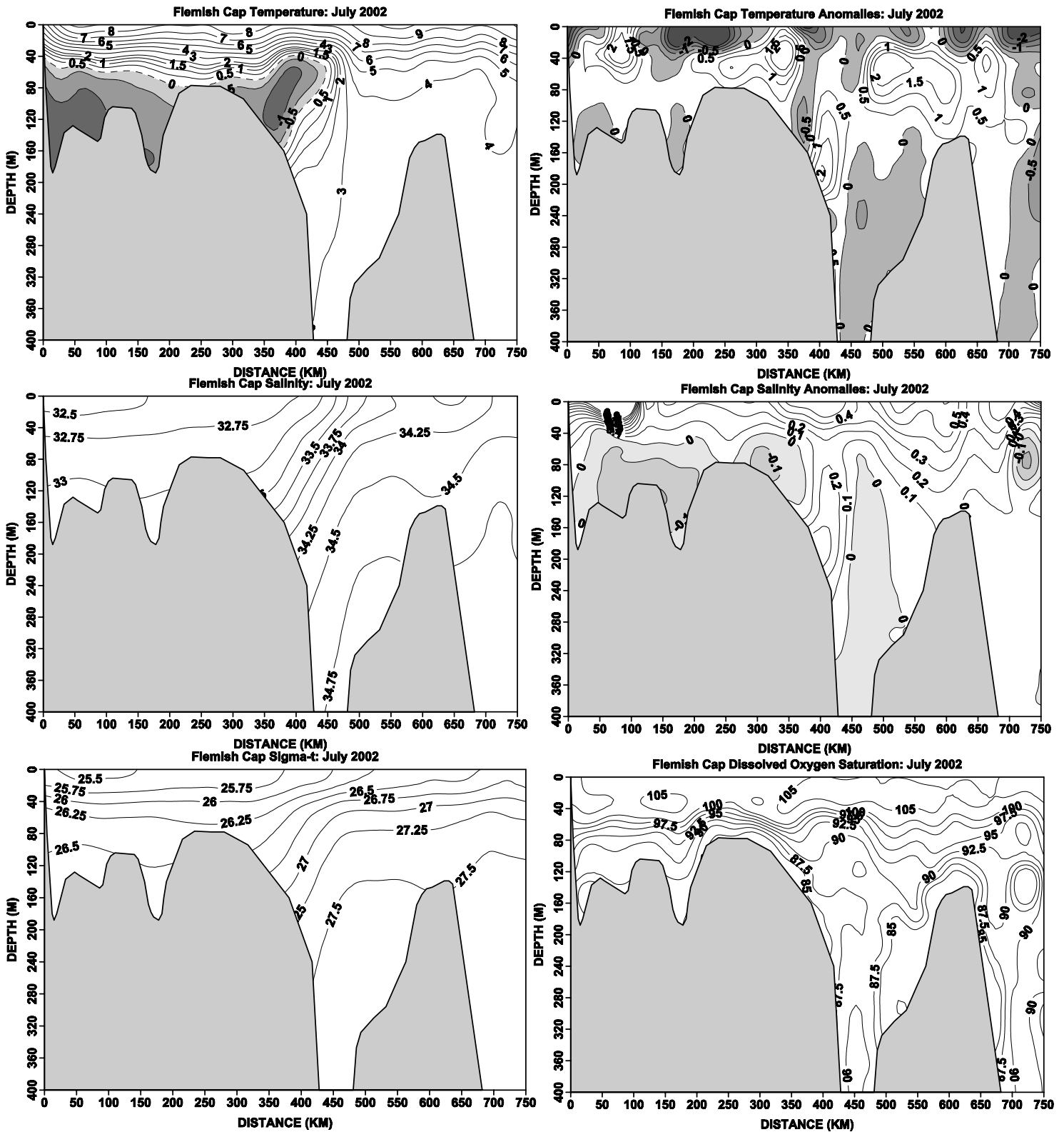
Fig. 11. Contours of temperature and salinity and their anomalies, sigma-t and dissolved oxygen saturation along the standard Flemish Cap section during the summer of 2002.
