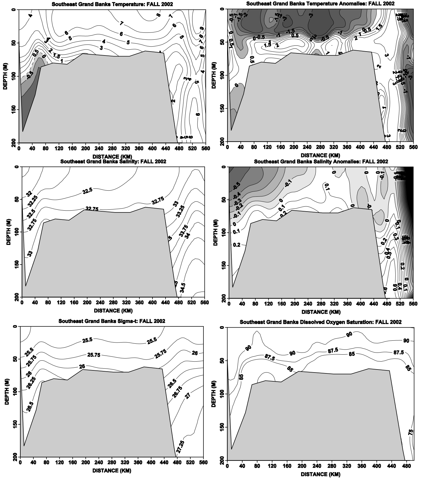
Fig. 9. Contours of temperature and salinity and their anomalies, sigma-t and dissolved oxygen saturation along the South East Grand Bank section during the fall of 2002.
