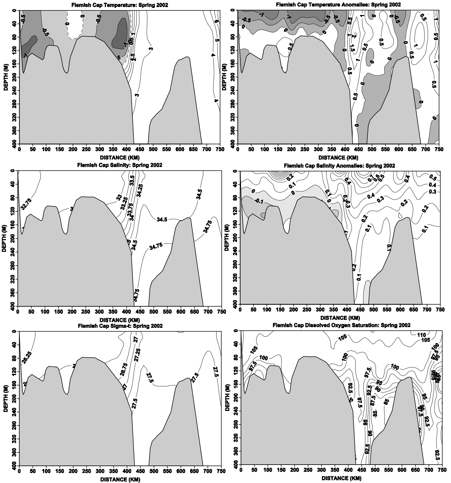
Fig. 10. Contours of temperature and salinity and their anomalies, sigma-t and dissolved oxygen saturation along the standard Flemish Cap section during the spring of 2002.
