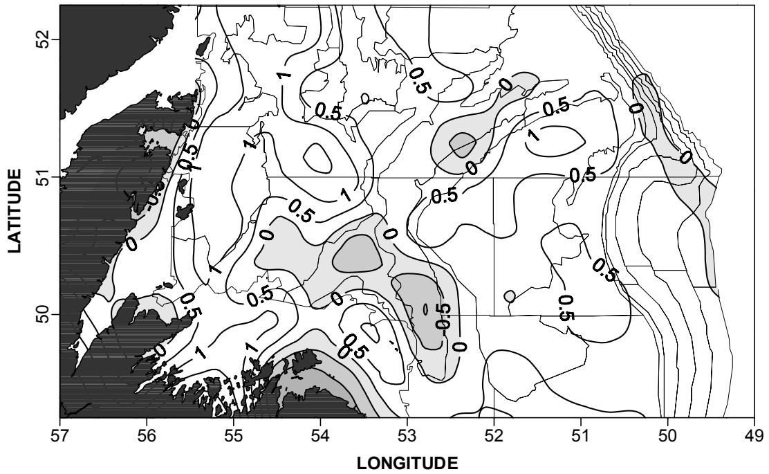
Fig. 28. Contours of bottom temperature and anomalies (in °C) for the fall of 2001, from the multi-species survey of NAFO Div. 3K.
