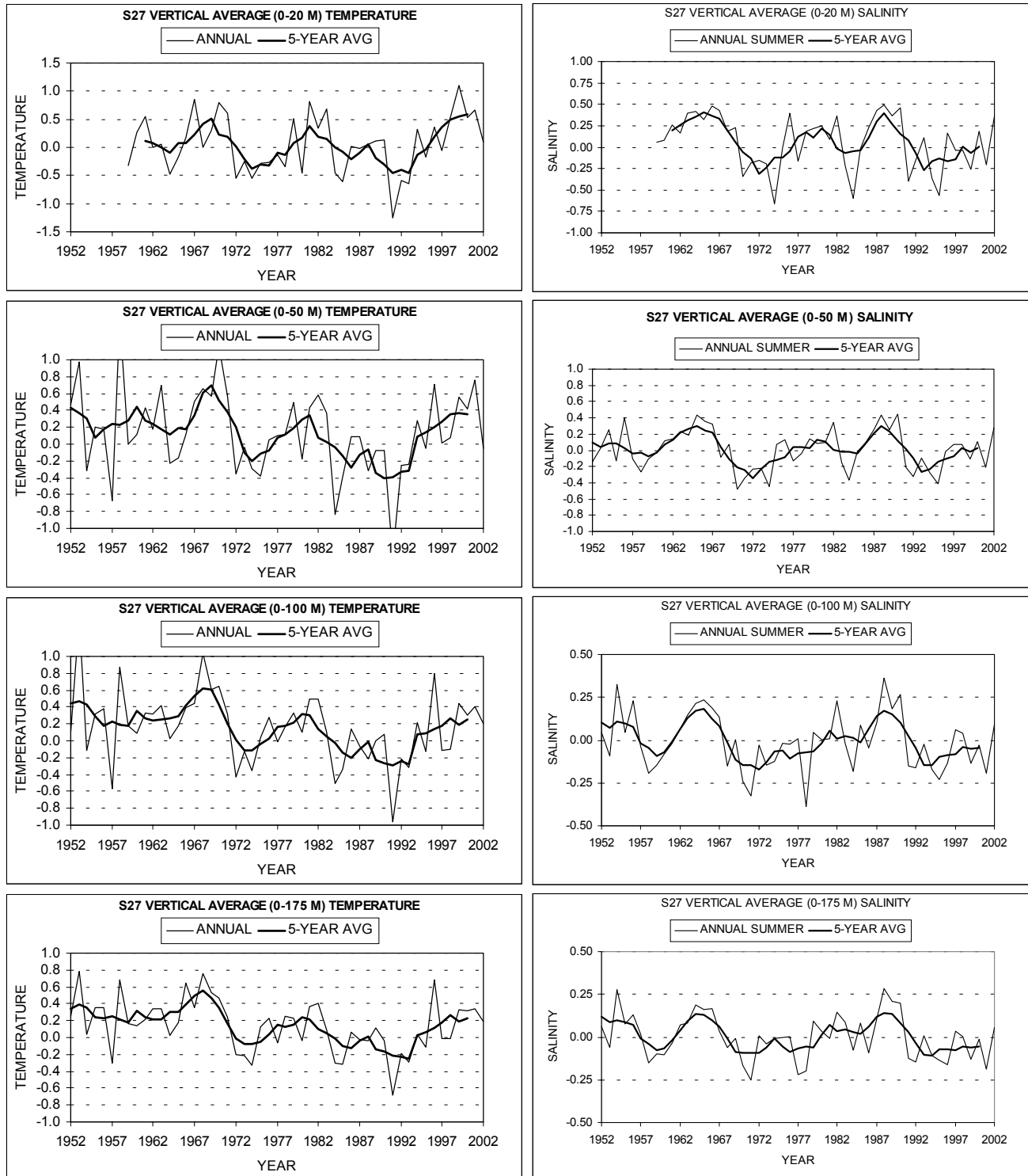
Fig. 5. Depth averaged Station 27 temperature (in °C) anomalies (left panels) and summer salinity anomalies (right panels) over selected depth ranges. The heavy lines are the 5-year running means.
