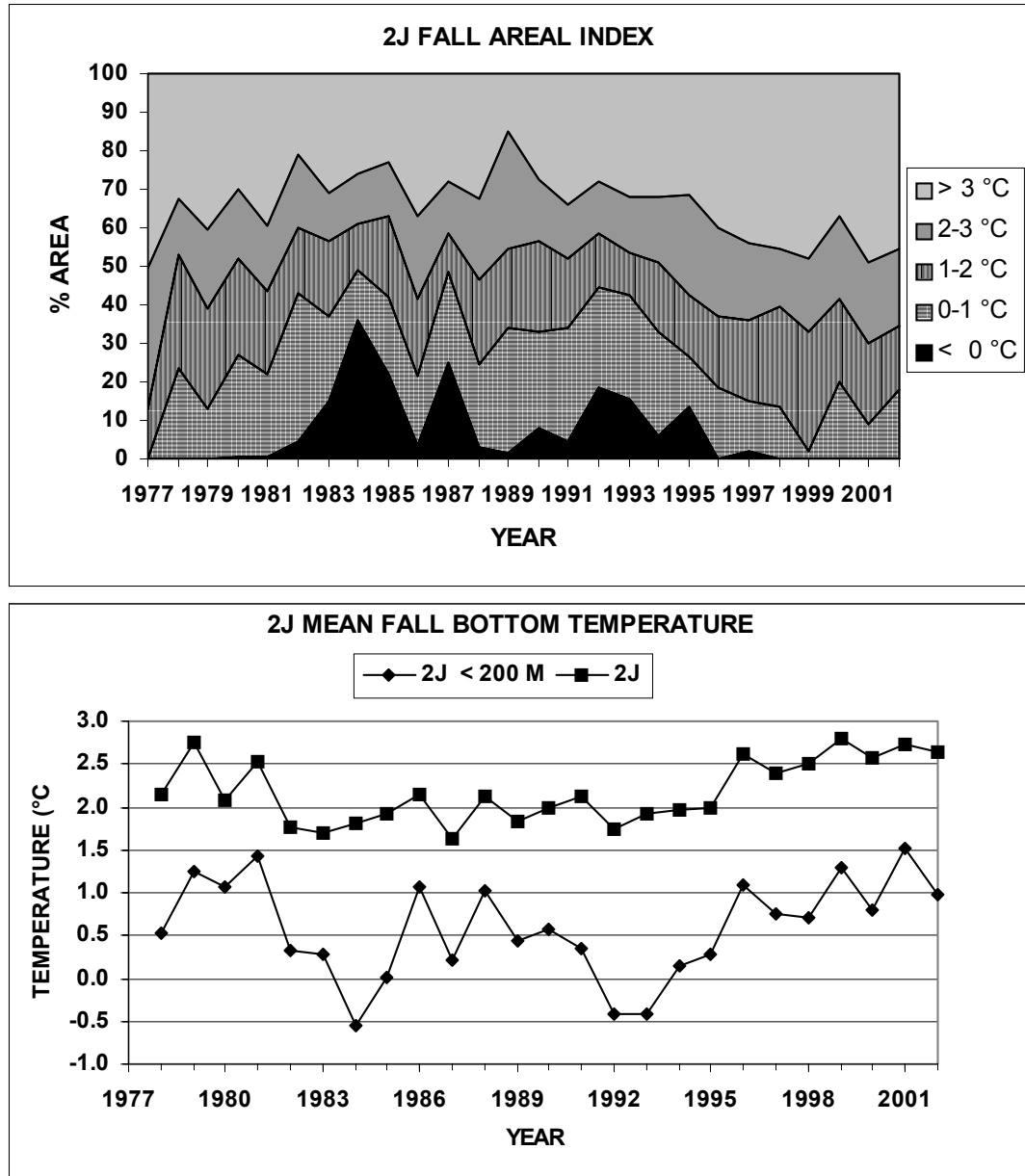
Fig. 33. Time series of the percentage area of the bottom in NAFO Div 2J covered by water with temperatures \leq 0^{\circ}\text{C} , 0-1^{\circ}\text{C} , 1-2^{\circ}\text{C} , 2-3^{\circ}\text{C} and \geq 3^{\circ}\text{C} during the fall (upper panel) and the mean bottom temperature in ^{\circ}\text{C} (bottom panel).
