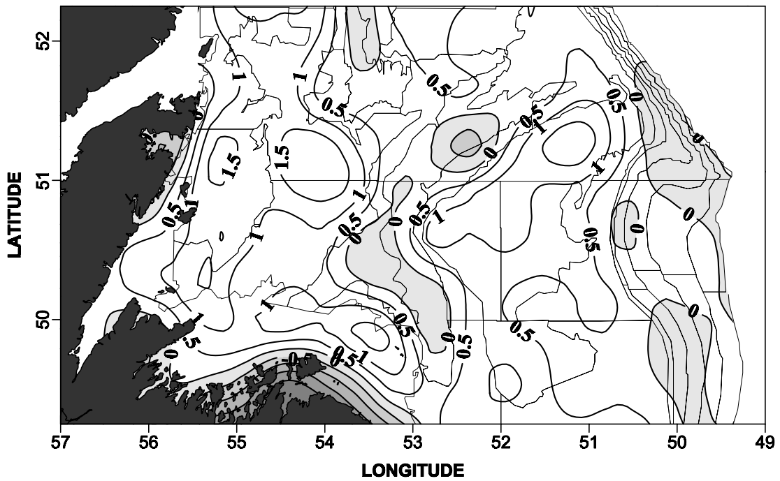
Fig. 29. Contours of bottom temperature and anomalies (in °C) for the fall of 2002, from the multi-species survey of NAFO Div. 3K.
