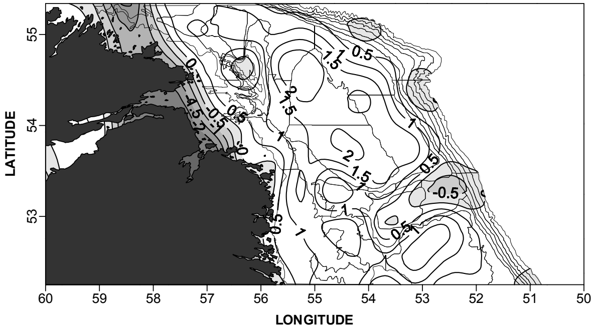
Fig. 31. Contours of bottom temperature and anomalies (in °C) for the fall of 2001, from the multi-species survey of NAFO Div. 2J.
