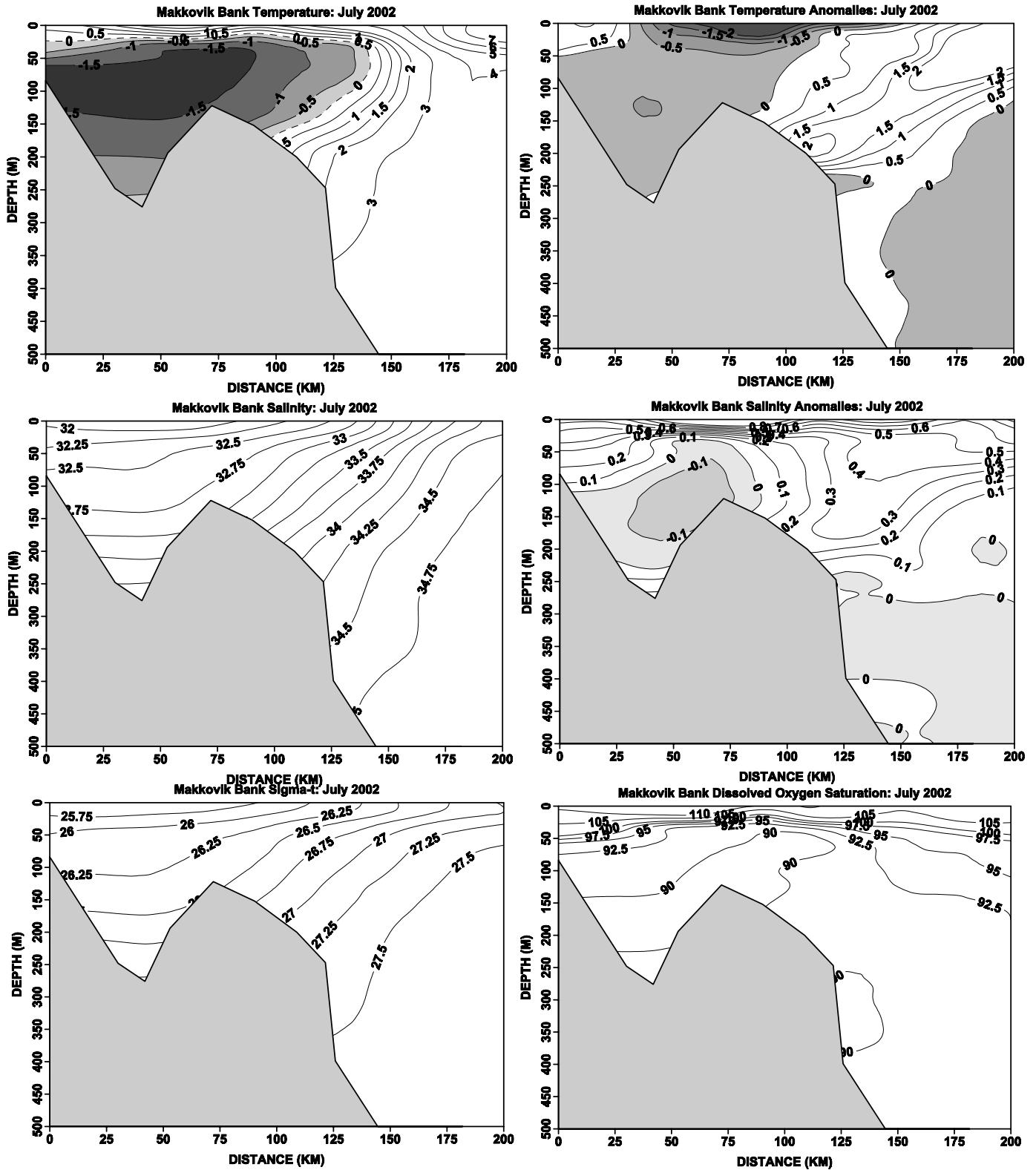
Fig. 18. Contours of temperature and salinity and their anomalies, sigma-t and dissolved oxygen saturation along the Makkovik Bank section during the summer of 2002.
