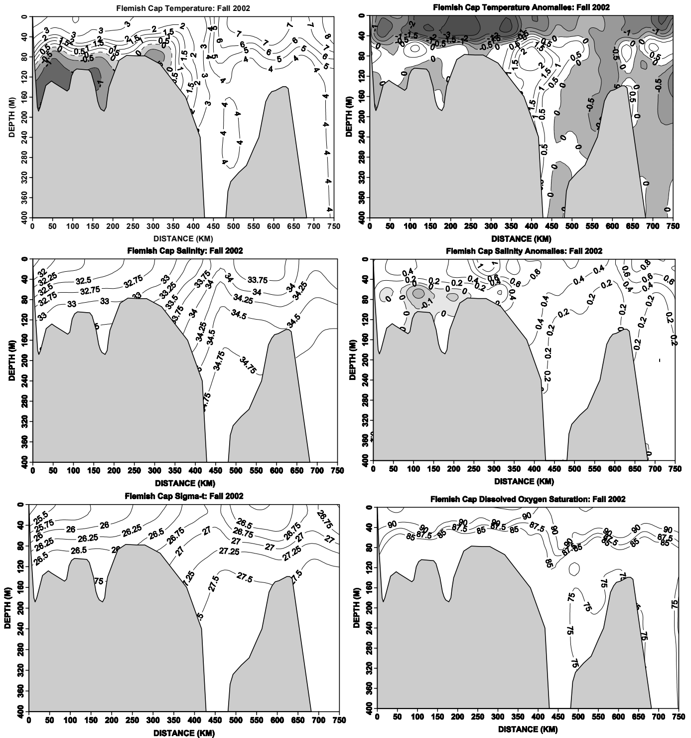
Fig. 12. Contours of temperature and salinity and their anomalies, sigma-t and dissolved oxygen saturation along the standard Flemish Cap section during the fall of 2002.
