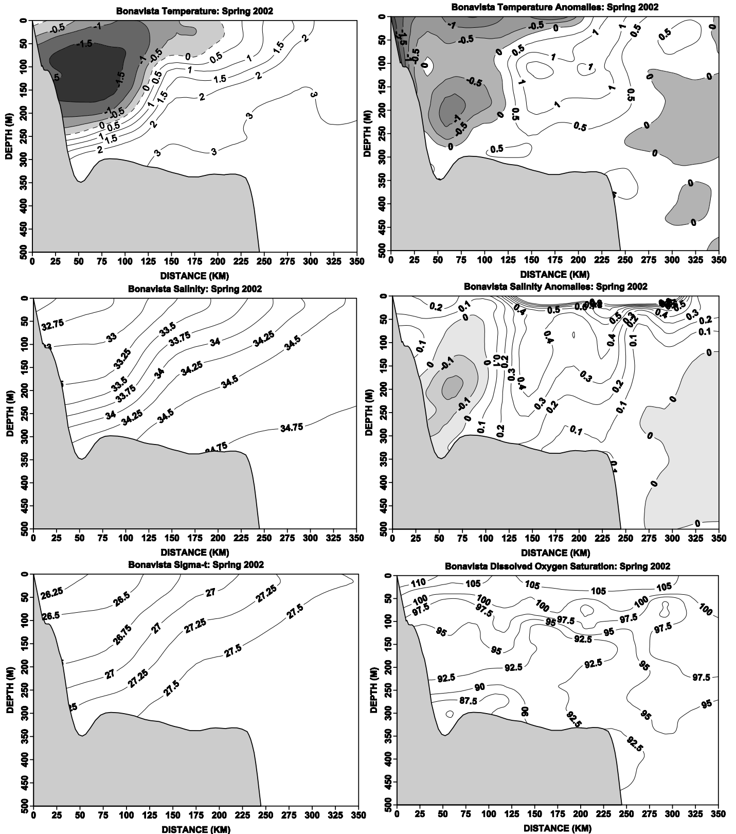
Fig. 13. Contours of temperature and salinity and their anomalies, sigma-t and dissolved oxygen saturation along the standard Bonavista section during the spring of 2002
