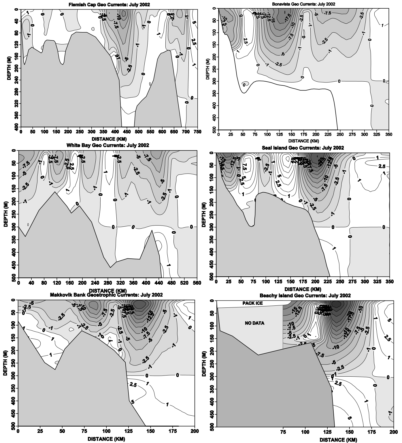
Fig. 22. Contours of geostrophic currents (in cm/s) along the Flemish Cap, Bonavista, White Bay, Seal Island, Makkovik Bank and Beachy Island sections during the summer of 2002. Negative shaded values are southward.
