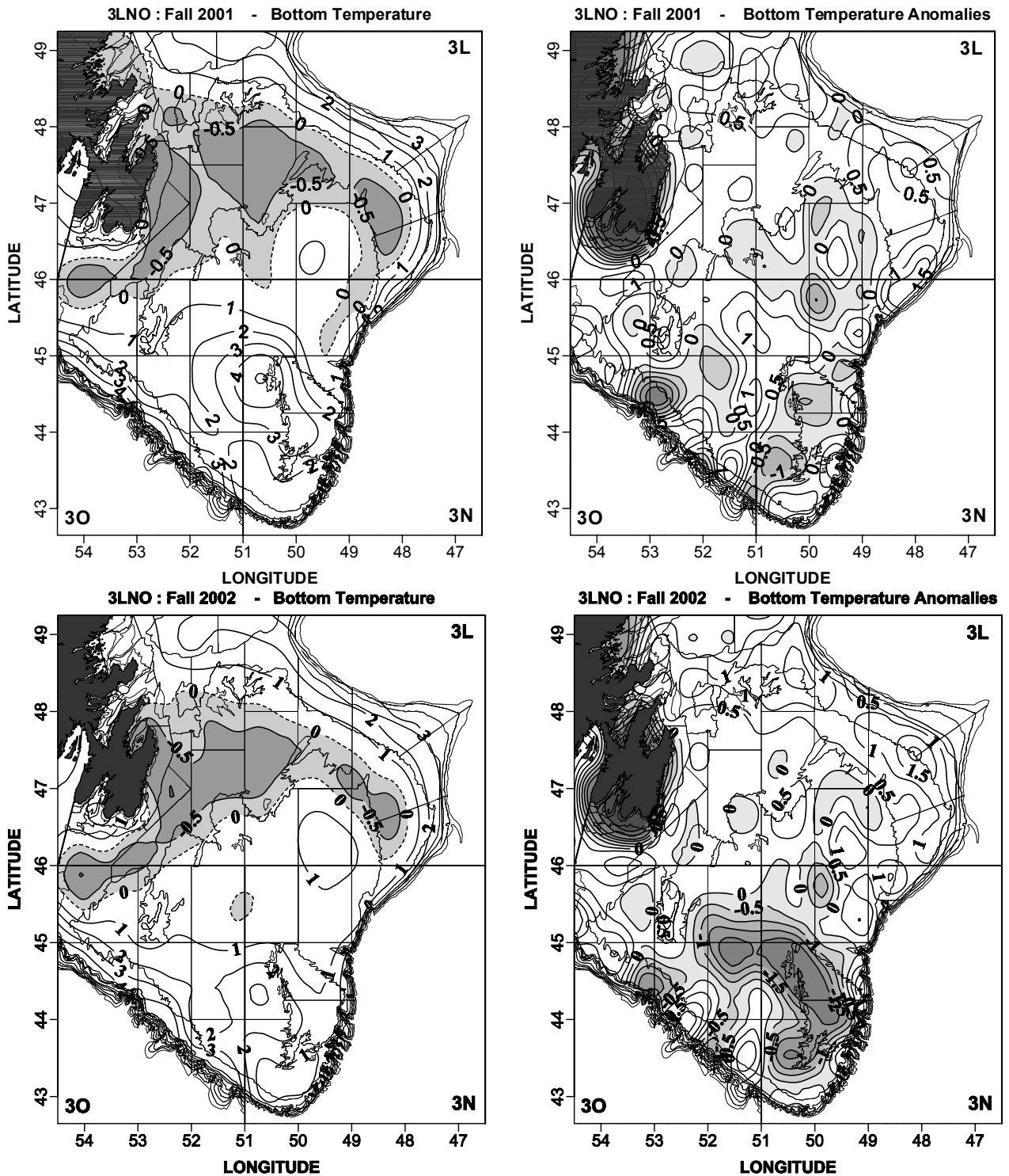
Fig. 26. Contours of bottom temperature and their anomalies (in °C) for the fall of 2001 and 2002 from the multi-species survey of NAFO Divs. 3LNO.
