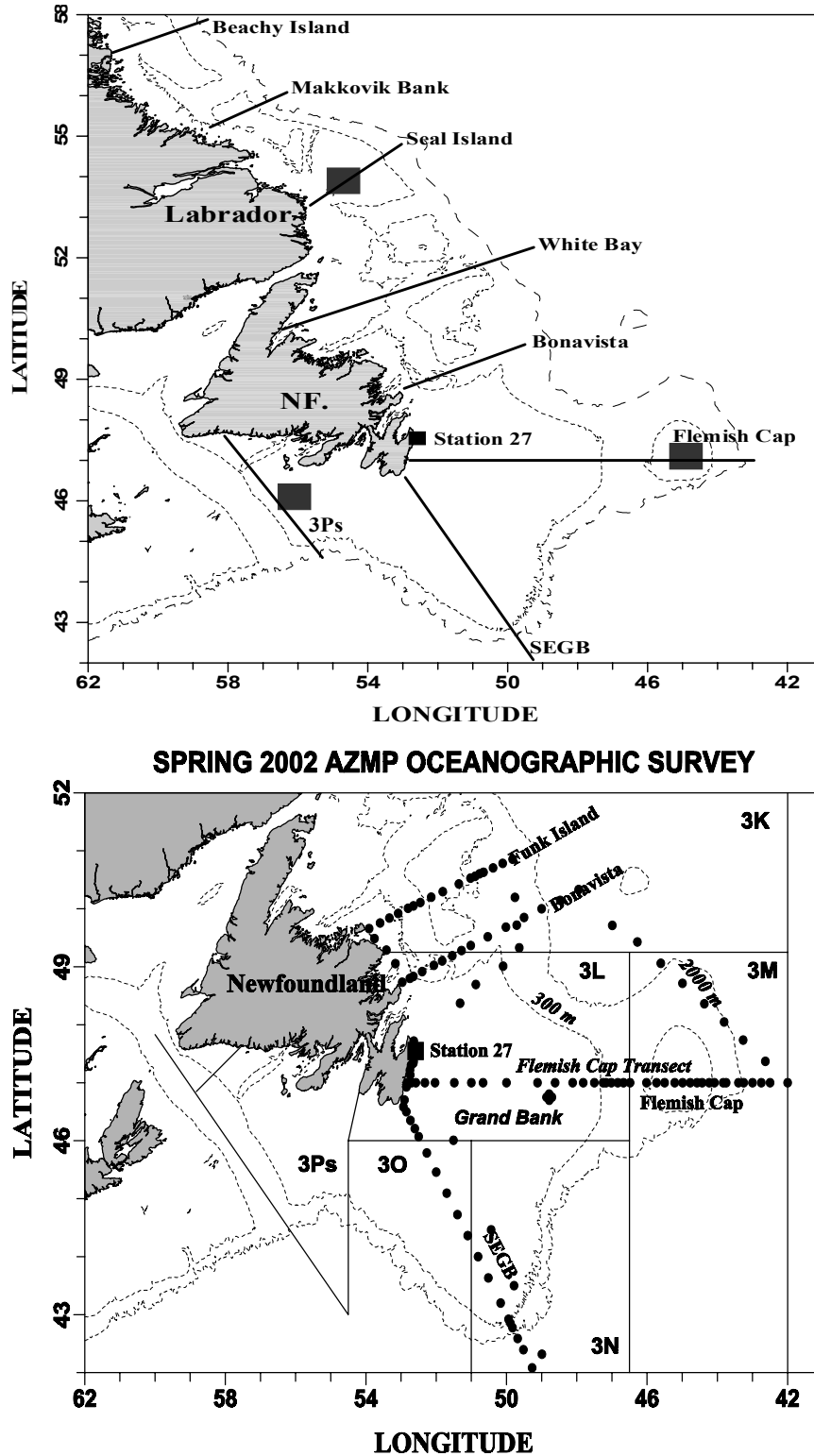
Fig. 1a. Location maps showing the position of standard sections, time series boxes, Station 27 and the position of all stations occupied during the spring AZMP 2002 survey. Bathymetry contours are 300 and 2000 m.
