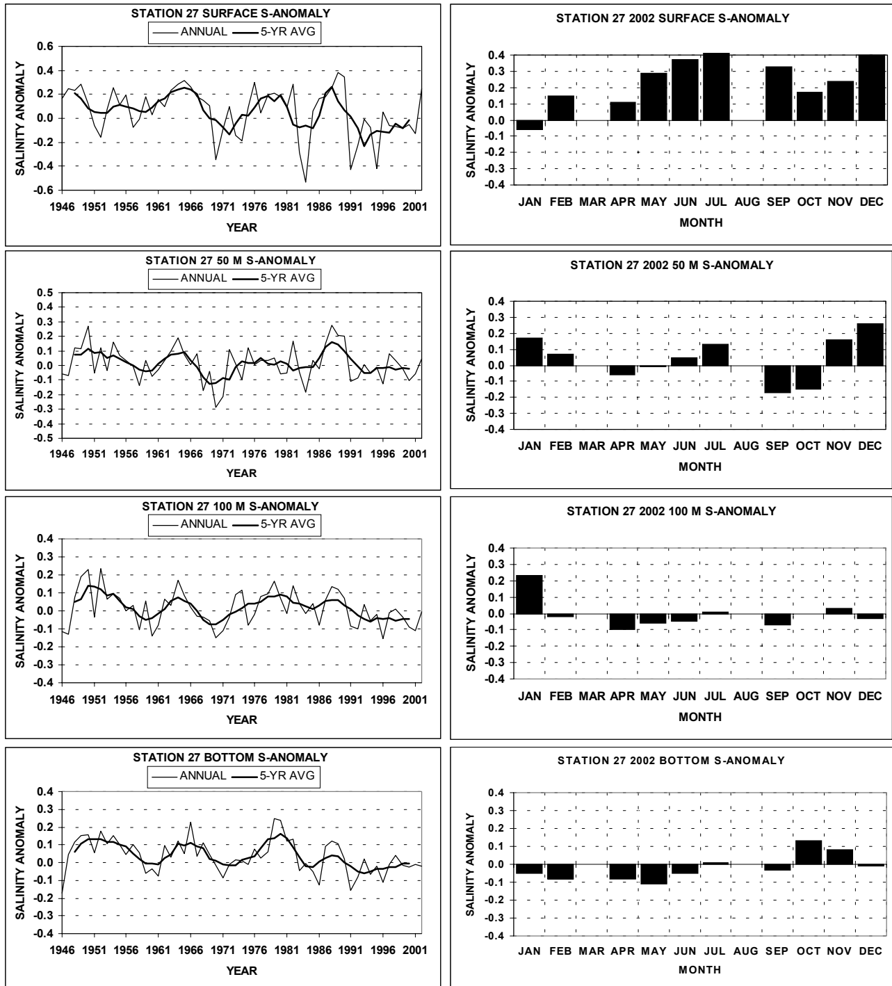
Fig. 4. Station 27 annual salinity anomalies and their 5-year running means at selected depths (left panels) and monthly salinity anomalies (right panels) for 2002.
