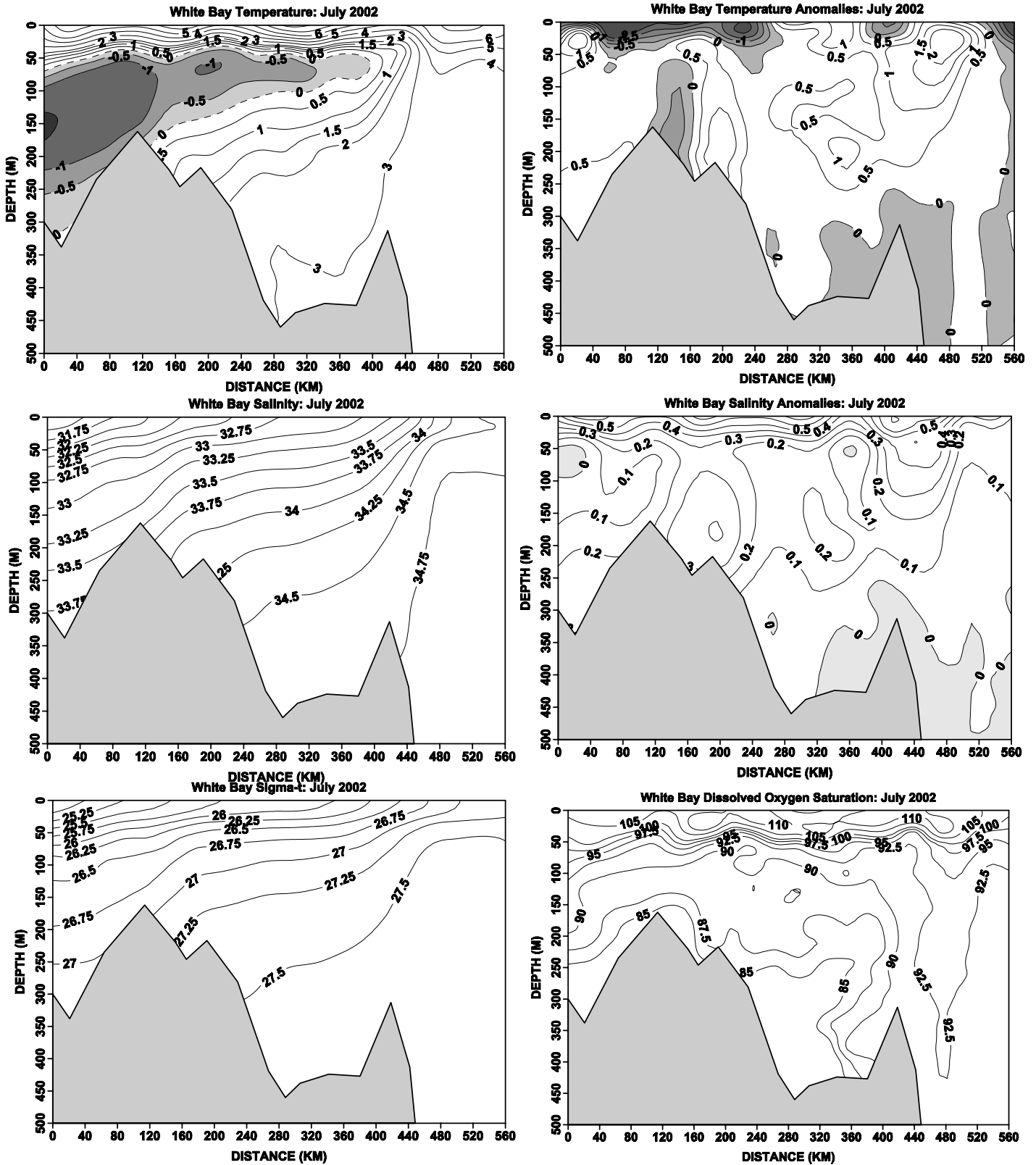
Fig. 16. Contours of temperature and salinity and their anomalies, sigma-t and dissolved oxygen saturation along the standard White Bay section during the summer of 2002.
