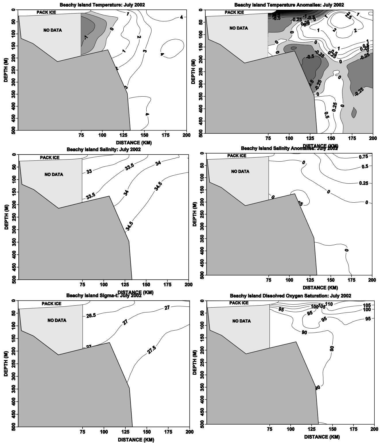
Fig. 19. Contours of temperature, salinity, sigma-t and dissolved oxygen saturation along the Standard Beachy Island section during the summer of 2002.
