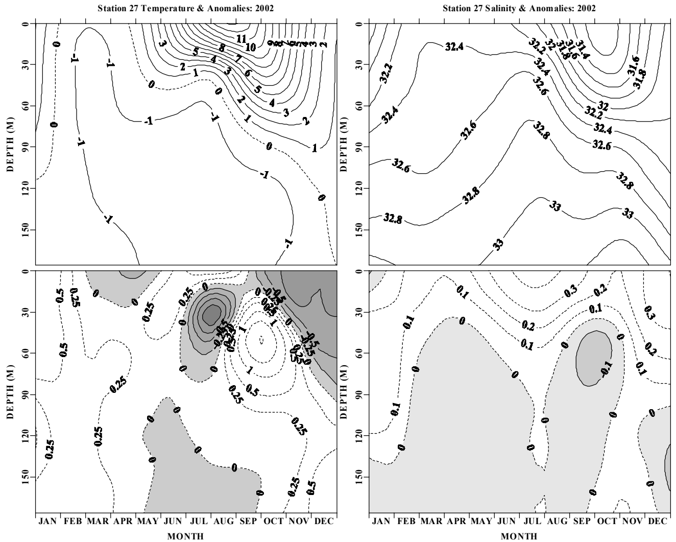
Fig. 2. Monthly temperatures (left panels) and salinity (right panels) and their anomalies (in °C) at Station 27 as a function of depth for 2002.
