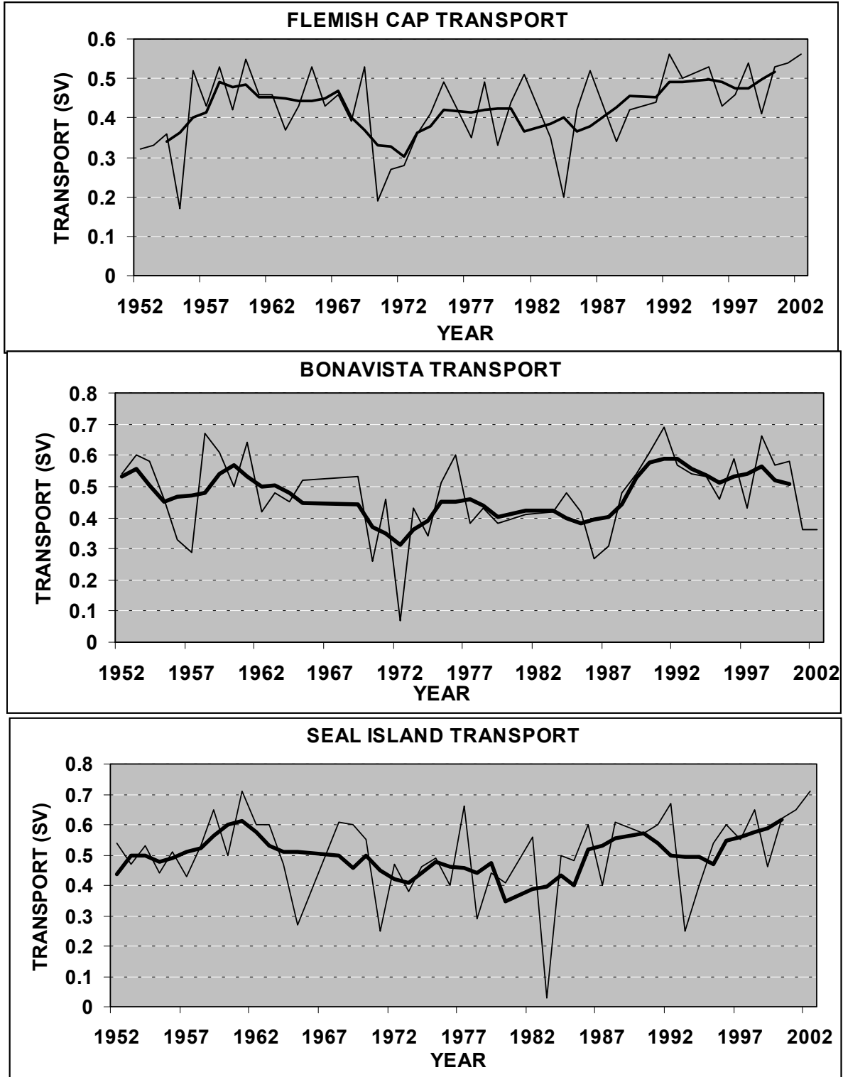
Fig. 23. Time series of geostrophic transport ( 10^6 \text{ m}^3/\text{s} ) relative to 135-m depth of the offshore branch of the Labrador Current through the Seal Island, Bonavista and Flemish Cap sections. The heavy line is the 5-year running mean.
