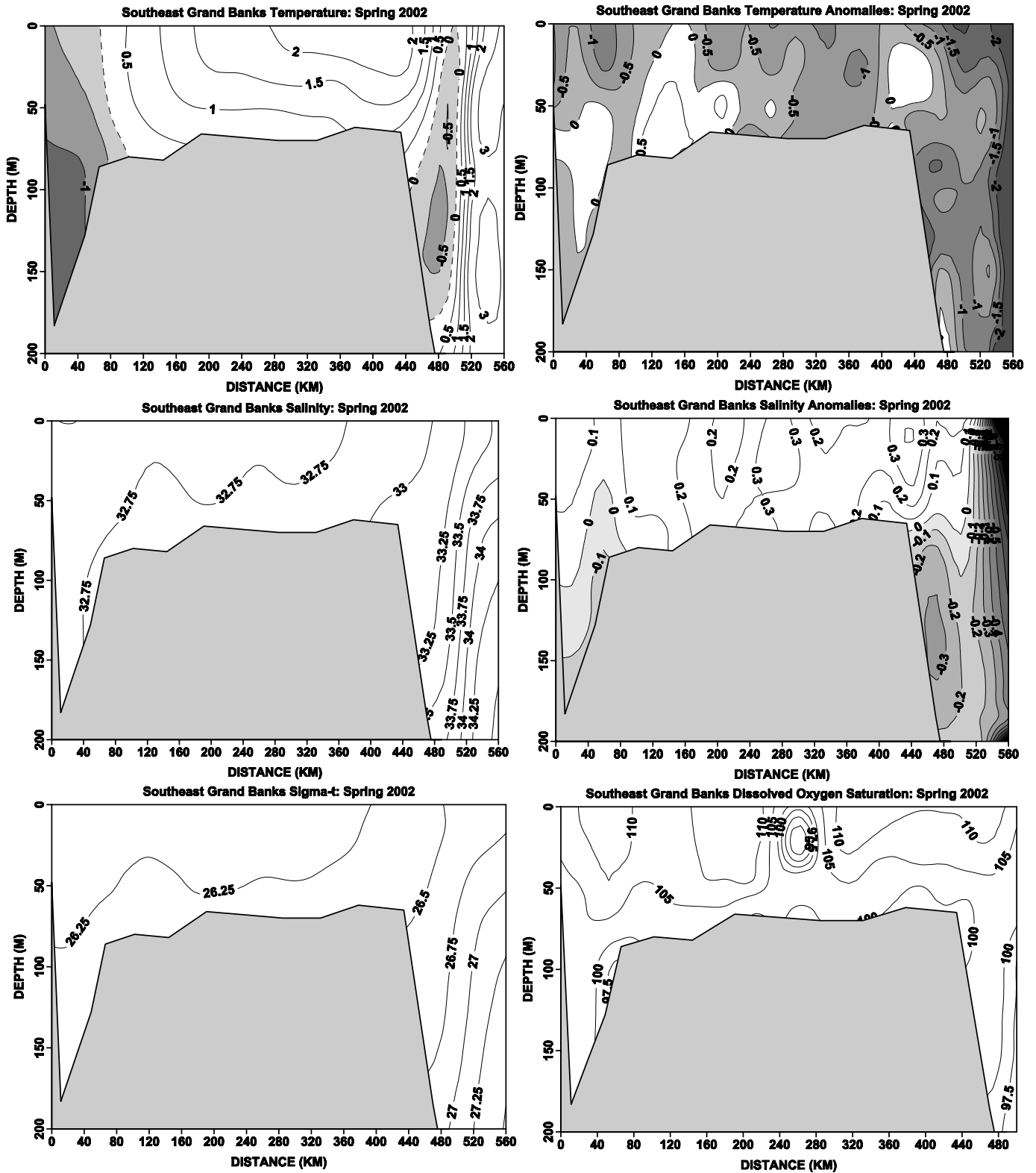
Fig. 8. Contours of temperature and salinity and their anomalies, sigma-t and dissolved oxygen saturation along the South East Grand Bank section during the spring of 2002.
