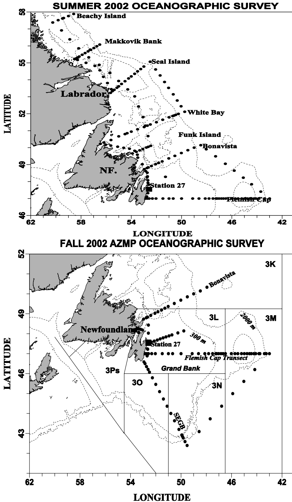
Fig. 1b. Location maps showing the position of all stations occupied during the summer and fall oceanographic surveys during 2002. Bathymetry contours are 300 and 2000 m.
