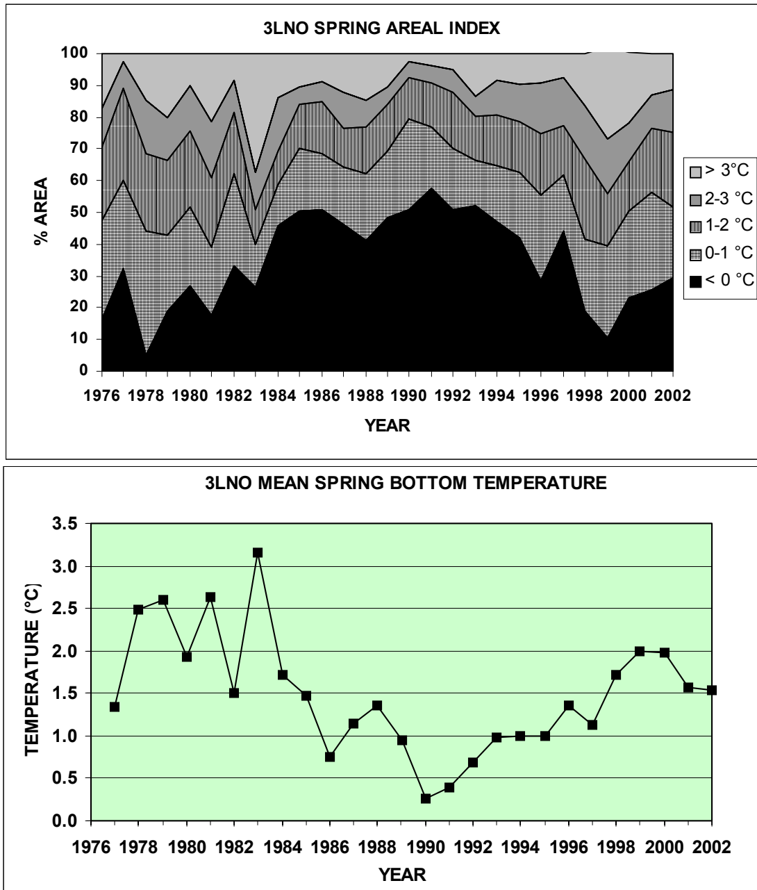
Fig. 25. Time series of the percentage area of the bottom in NAFO Divs. 3LNO covered by water with temperatures \leq 0^{\circ}\text{C} , 0\text{-}1^{\circ}\text{C} , 1\text{-}2^{\circ}\text{C} , 2\text{-}3^{\circ}\text{C} and \geq 3^{\circ}\text{C} during spring (upper panel) and the mean bottom temperature in ^{\circ}\text{C} (bottom panel).
