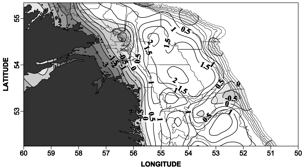
Fig. 32. Contours of bottom temperature and anomalies (in °C) for the fall of 2002, from the multi-species survey of NAFO Div. 2J.
