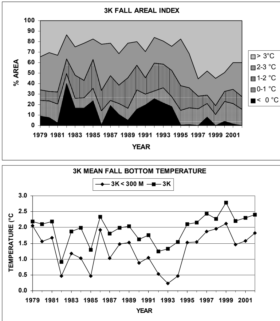
Fig. 30. Time series of the percentage area of the bottom in NAFO Div 3K covered by water with temperatures \leq 0^{\circ}\text{C} , 0-1^{\circ}\text{C} , 1-2^{\circ}\text{C} , 2-3^{\circ}\text{C} and \geq 3^{\circ}\text{C} during the fall (upper panel) and the mean bottom temperature in ^{\circ}\text{C} (bottom panel).
