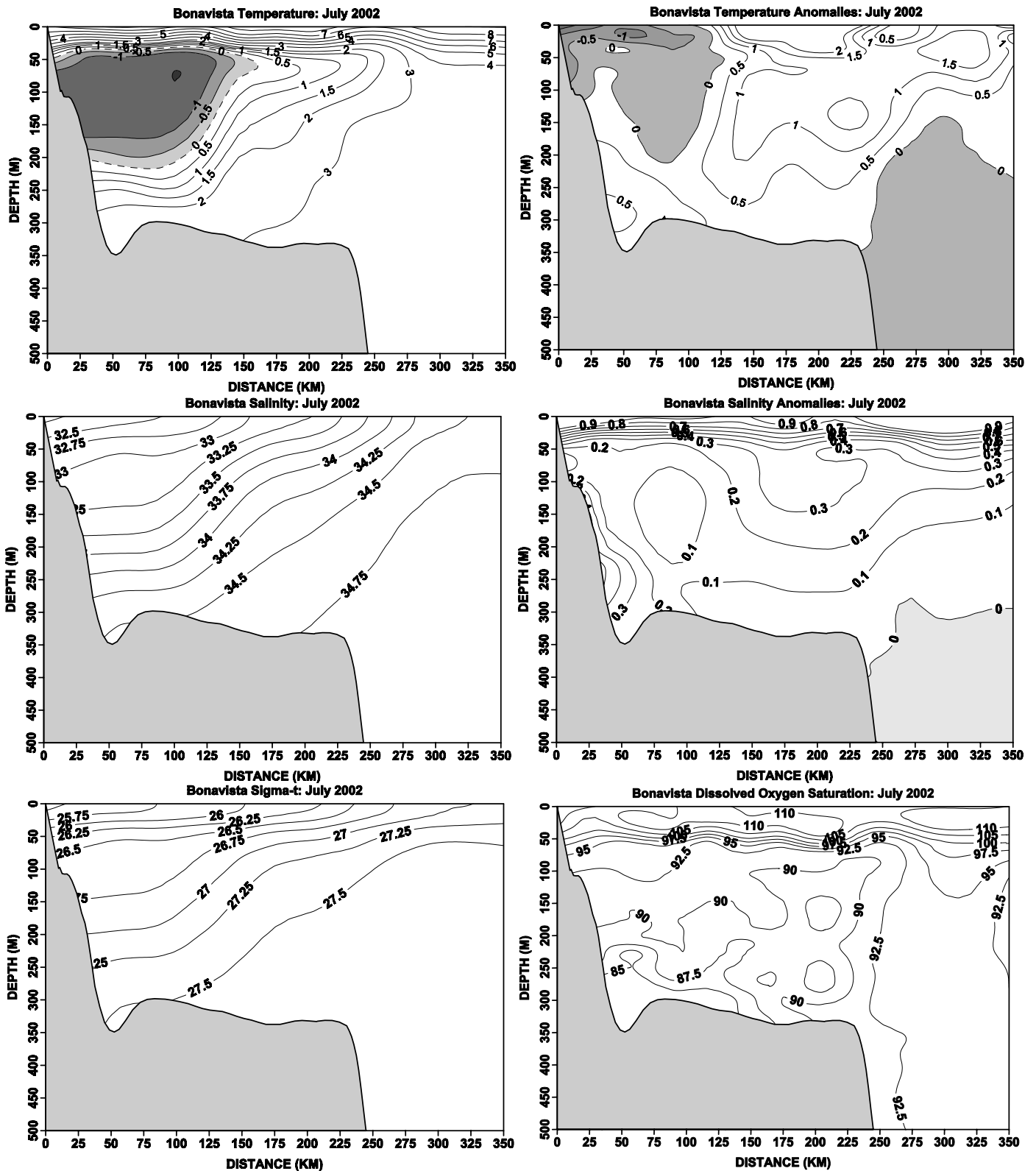
Fig. 14. Contours of temperature and temperature anomalies, salinity, sigma-t and dissolved oxygen saturation along the standard Bonavista section during the summer of 2002.
