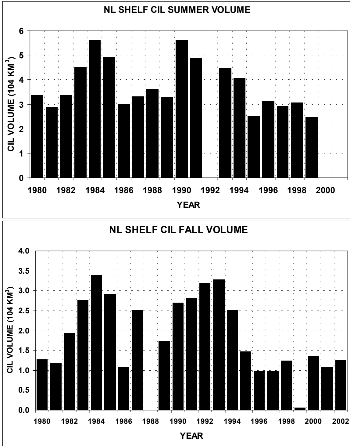
Fig. 21. Summer and fall cold-intermediate-layer (CIL) volumes with temperatures <0^{\circ}\text{C} over the 2J3KL areas. There were insufficient data to calculate the summer 2000 to 2002 values.
