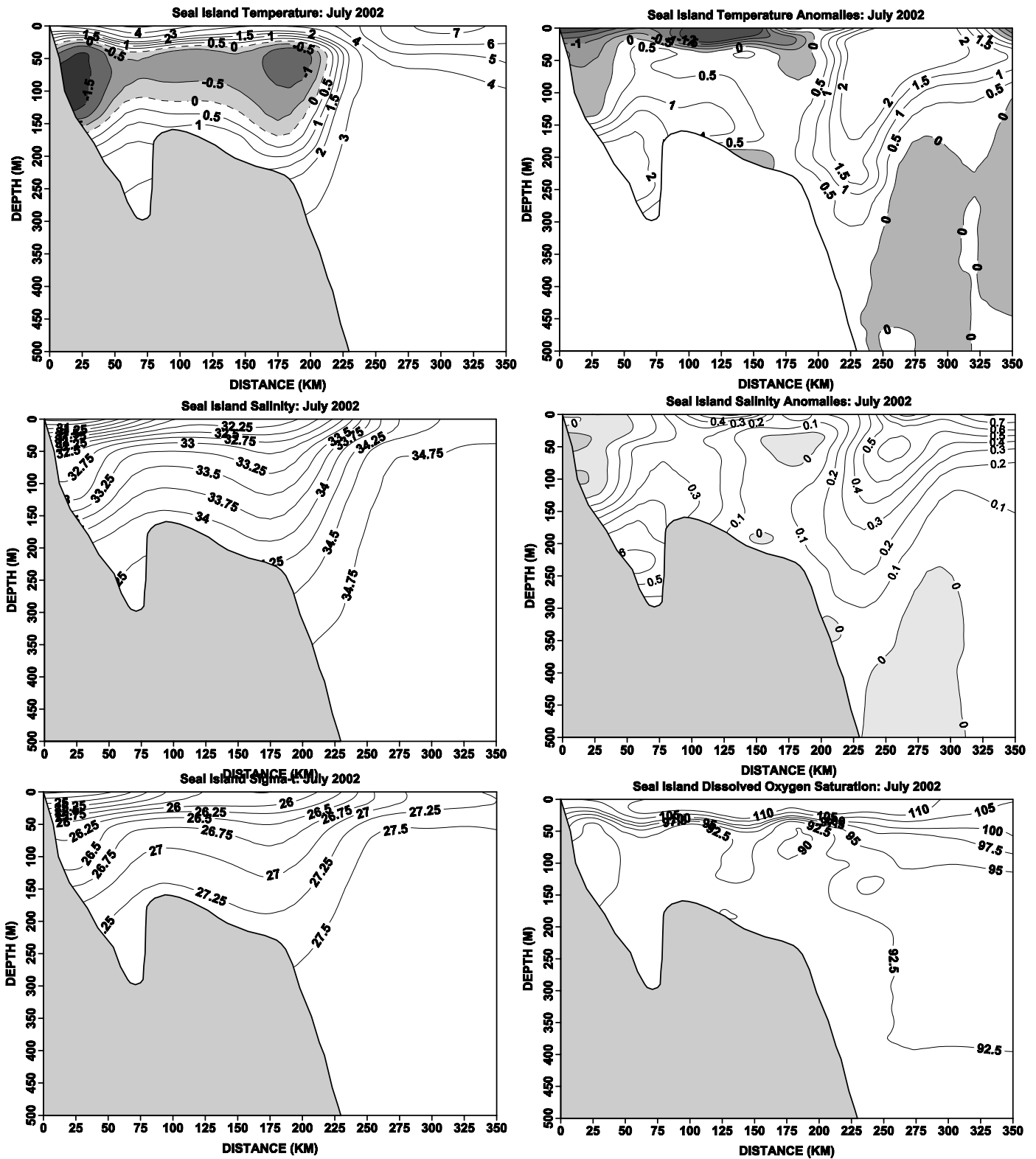
Fig. 17. Contours of temperature and salinity and their anomalies, sigma-t and dissolved oxygen saturation along the standard Seal Island transect during the summer of 2002.
