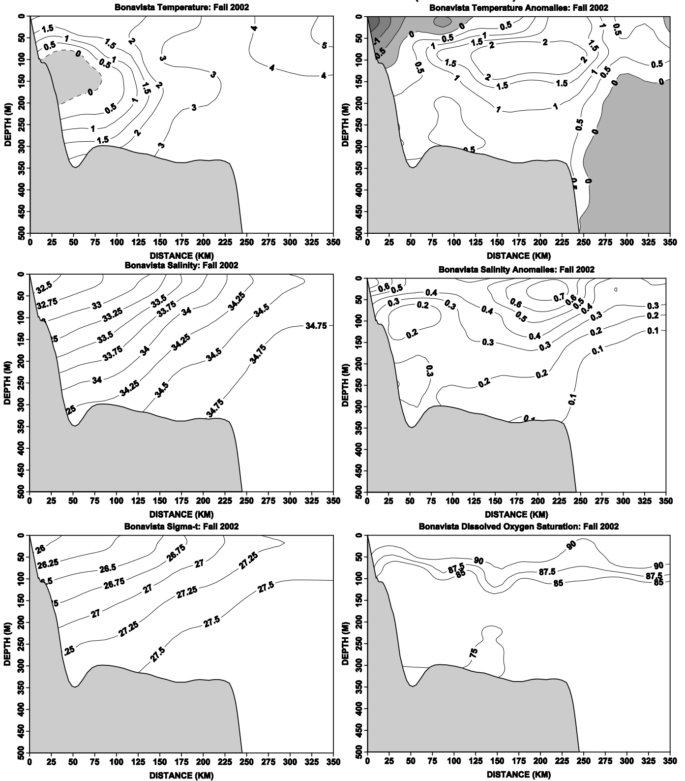
Fig. 15. Contours of temperature and salinity and their anomalies, sigma-t and dissolved oxygen saturation along the standard Bonavista section during the fall of 2002.
