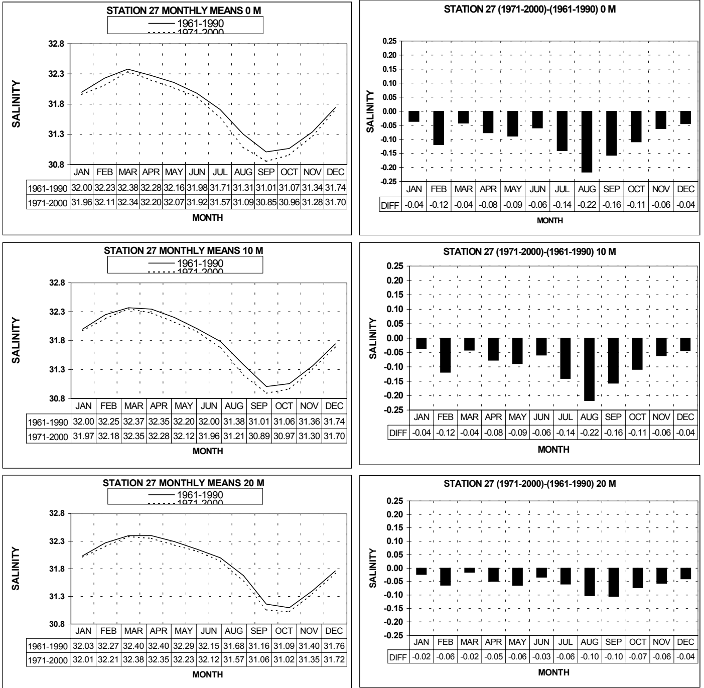
Fig. 3a. Monthly means (left panels) and differences (right panels) of salinity at Station 27 for the periods 1961-1990 and 1971-2000 at standard depths.
