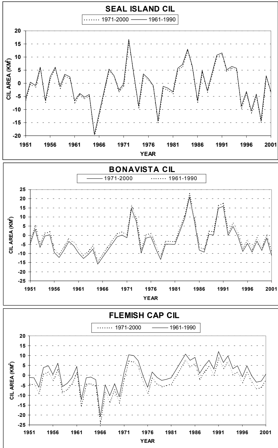
Fig. 9. Annual CIL anomalies along the standard Seal Island, Bonavista and Flemish Cap transects, referenced to the 1961-1990 and the 1971-2000 time periods.
