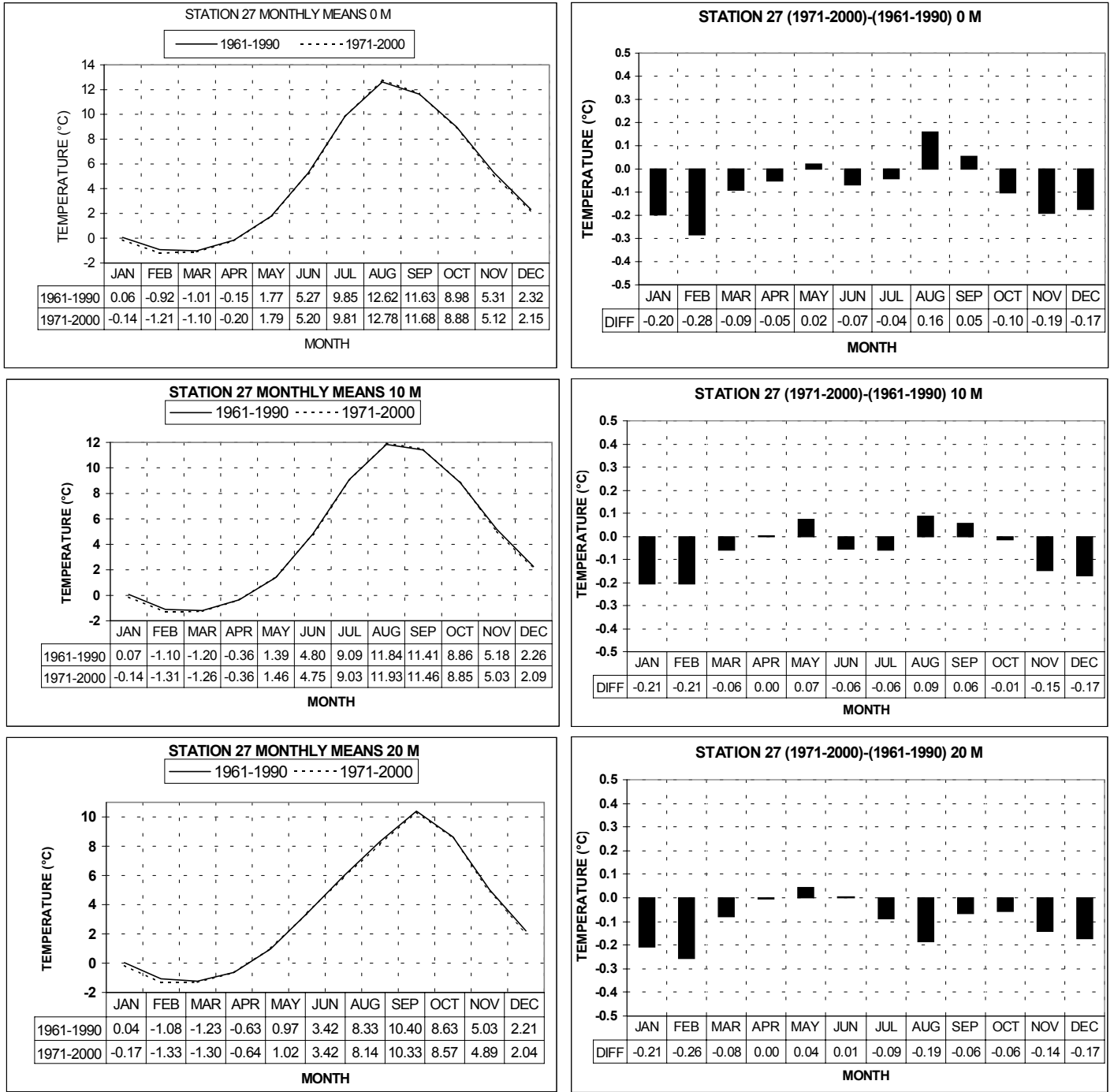
Fig. 1a. Monthly means (left panels) and differences (right panels) of temperature at Station 27 for the periods 1961-1990 and 1971-2000 at standard depths.
