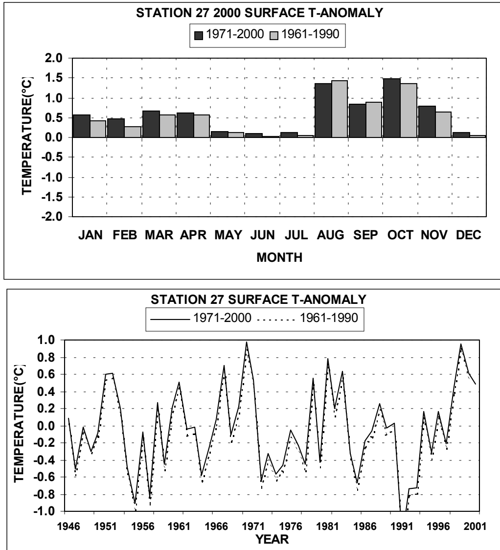
Fig. 2a. Monthly means (top panel) of surface temperature during 2000 and the annual anomalies (bottom panel) at Station 27 referenced to the periods 1961-1990 and 1971-2000.
