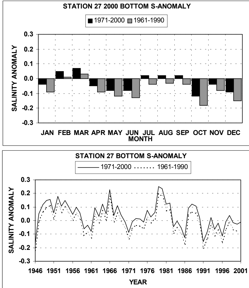
Fig. 4b. Monthly means (top panel) of bottom salinity during 2000 and the annual anomalies (bottom panel) at Station 27 referenced to the periods 1961-1990 and 1971-2000.
