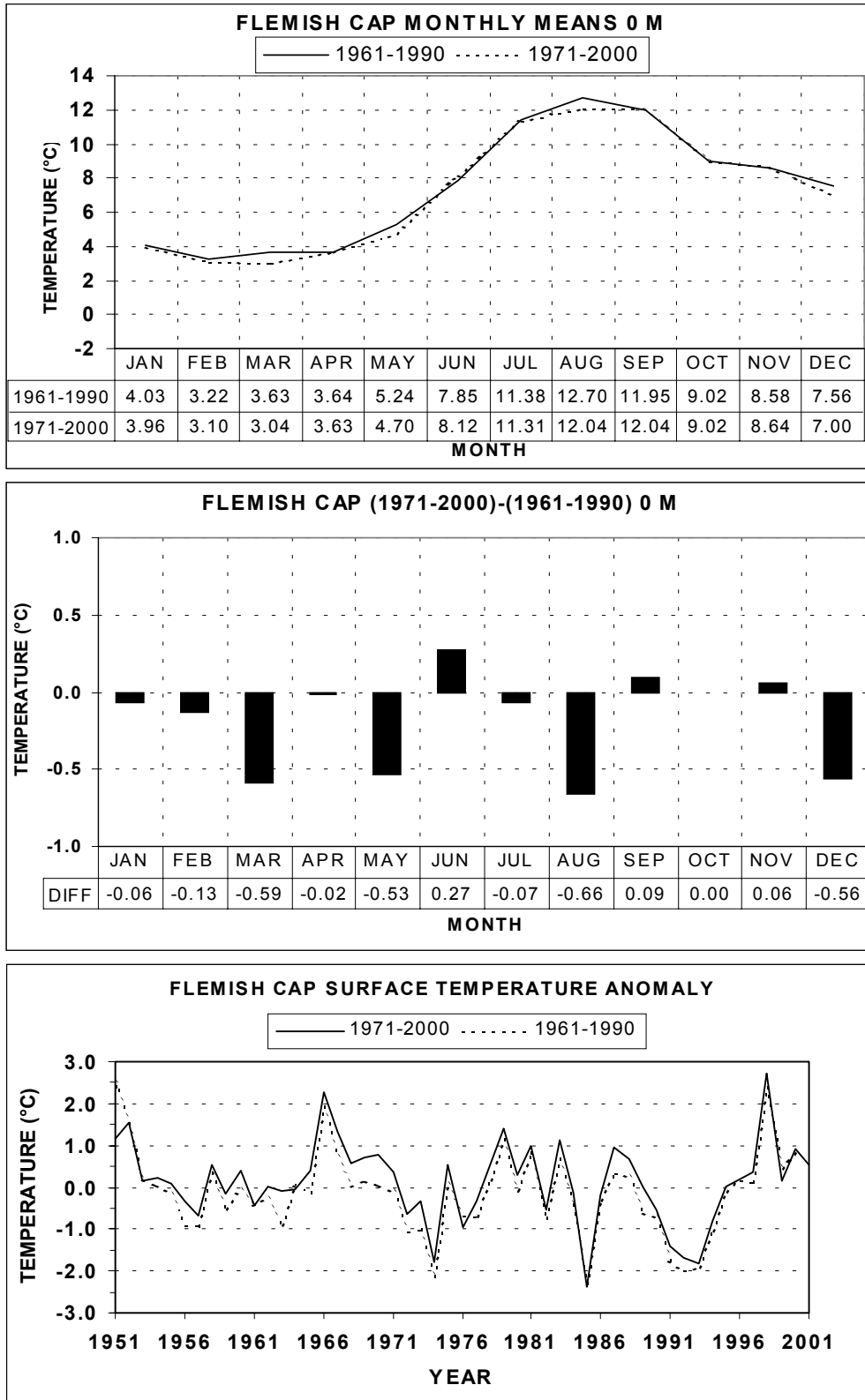
Fig. 6a. Monthly means (top panel), differences (centre panel) and annual anomalies (bottom panel) of surface temperatures on the Flemish Cap for the periods 1961-1990 and 1971-2000.
