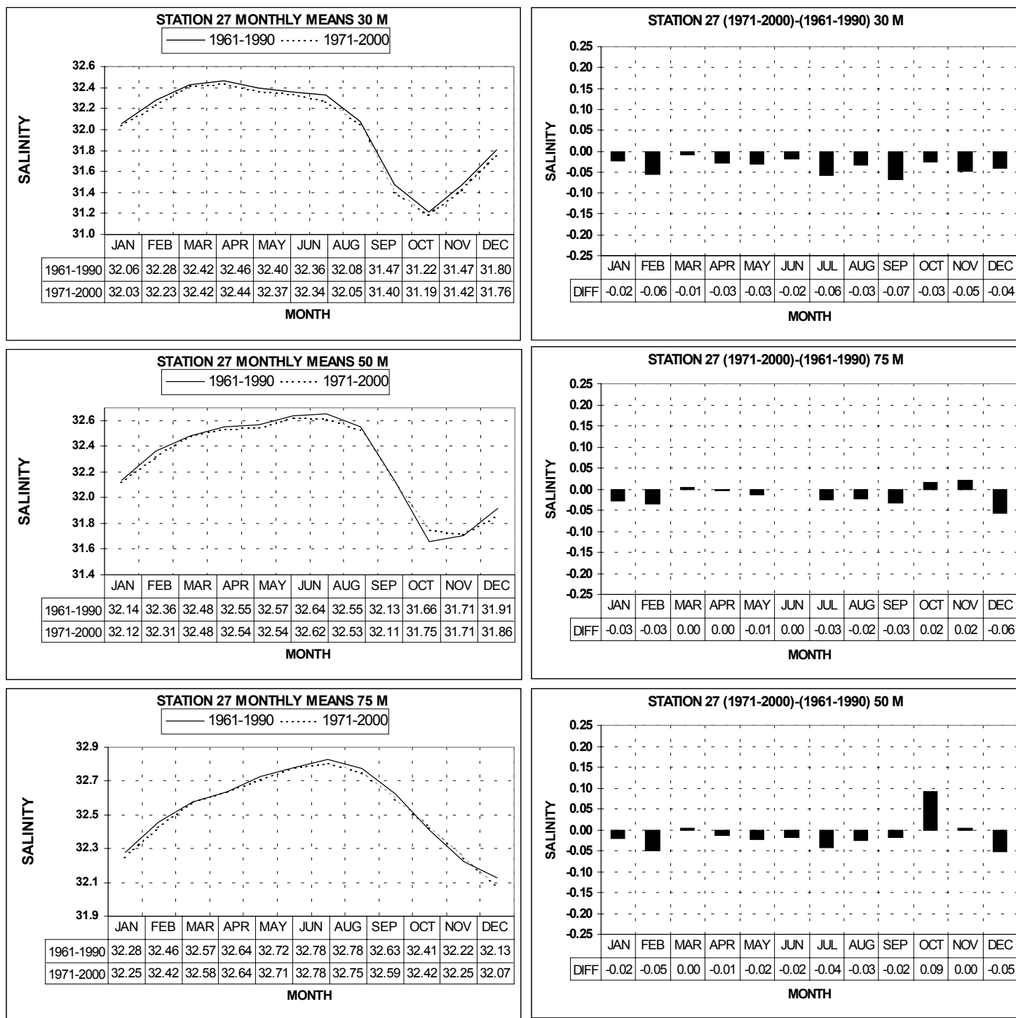
Fig. 3b. Monthly means (left panels) and differences (right panels) of salinity at Station 27 for the periods 1961-1990 and 1971-2000 at standard depths.
