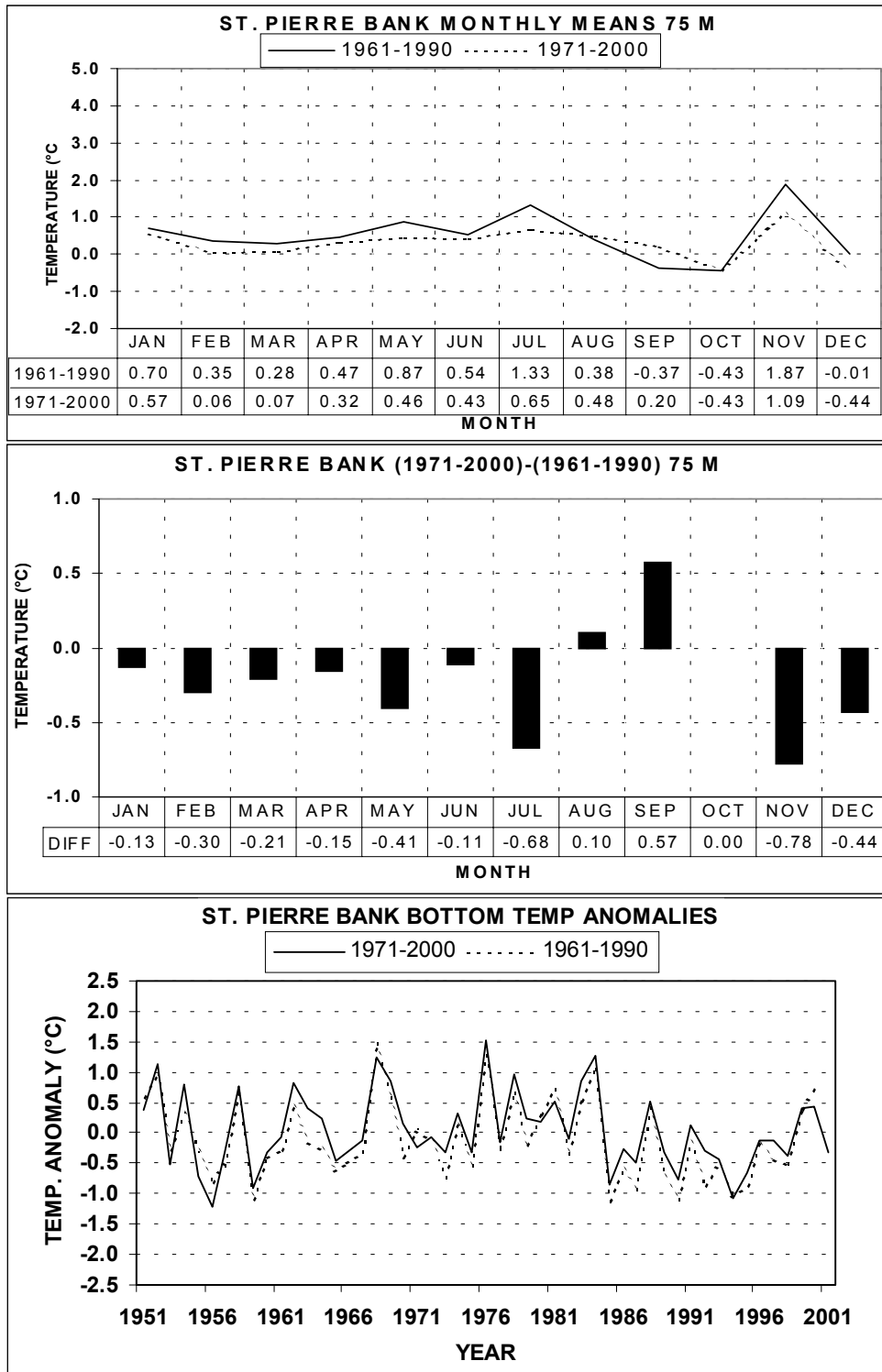
Fig. 5b. Monthly means (top panel), differences (centre panel) and annual anomalies (bottom panel) of near bottom temperatures on St. Pierre Bank for the periods 1961-1990 and 1971-2000.
