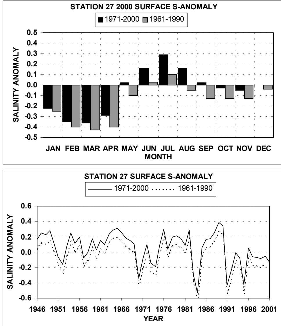
Fig. 4a. Monthly means (top panel) of surface salinity during 2000 and the annual anomalies (bottom panel) at Station 27 referenced to the periods 1961-1990 and 1971-2000.
