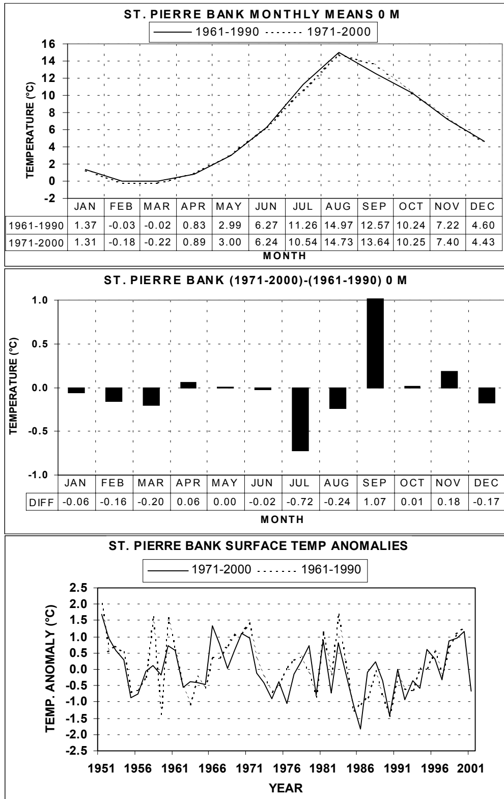
Fig. 5a. Monthly means (top panel), differences (centre panel) and annual anomalies (bottom panel) of surface temperatures on St. Pierre Bank for the periods 1961-1990 and 1971-2000.
