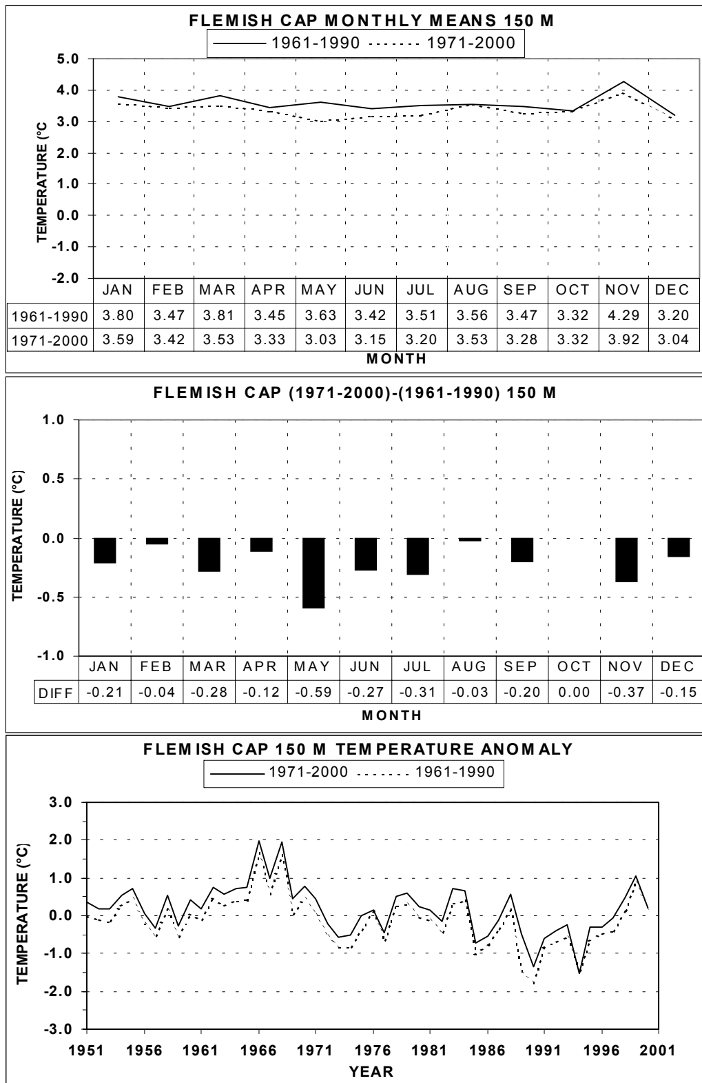
Fig. 6b. Monthly means (top panel), differences (centre panel) and annual anomalies (bottom panel) of near bottom temperatures on the Flemish Cap for the periods 1961-1990 and 1971-2000.
