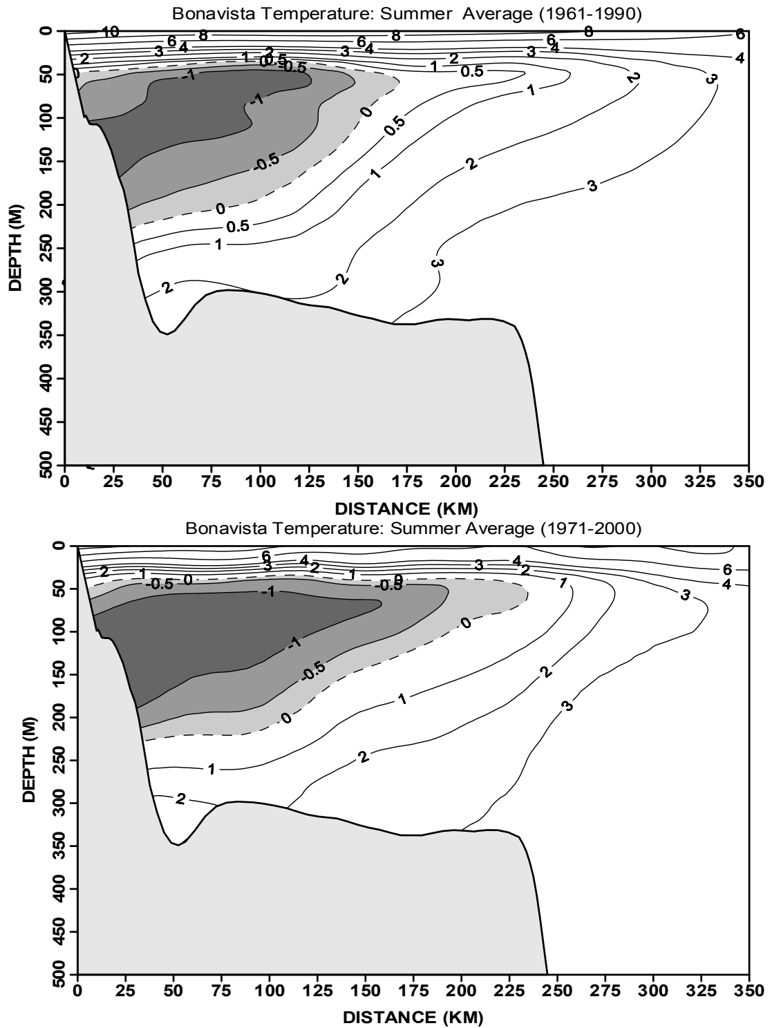
Fig. 8. Cross-sectional temperature contours along the standard Bonavista transect during the summer based on all data collected during the 1961-1990 and the 1971-2000 time periods.
