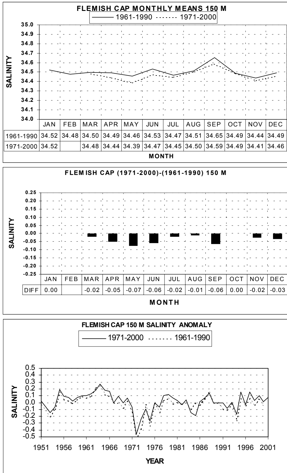
Fig. 7b. Monthly means (top panel), differences (centre panel) and annual anomalies (bottom panel) of near bottom salinity on the Flemish Cap for the periods 1961-1990 and 1971-2000.
