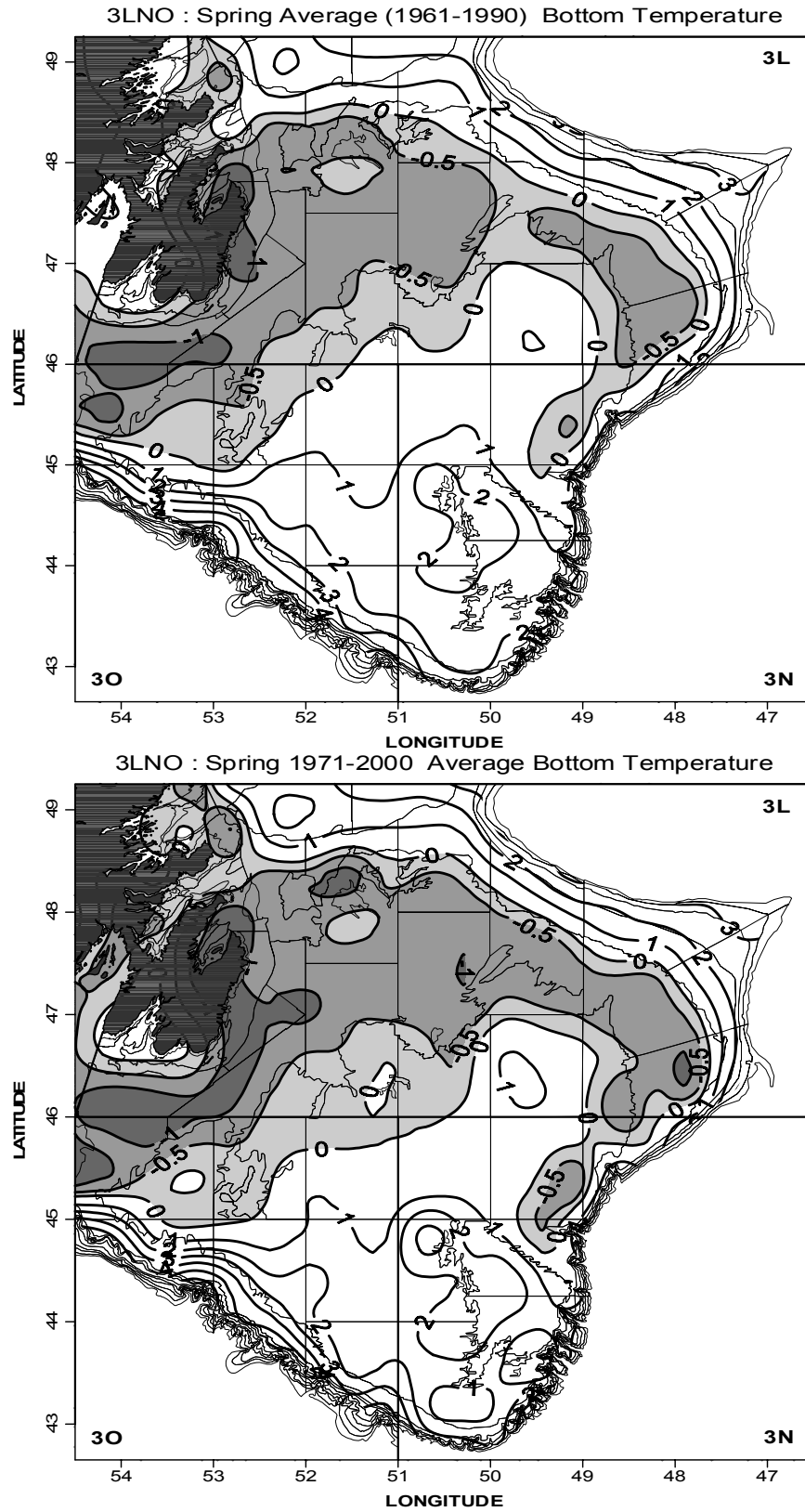
Fig. 10. Bottom temperature contours for the spring in NAFO Divs. 3LNO based on data collected during the 1961-1990 and the 1971-2000 time periods.
