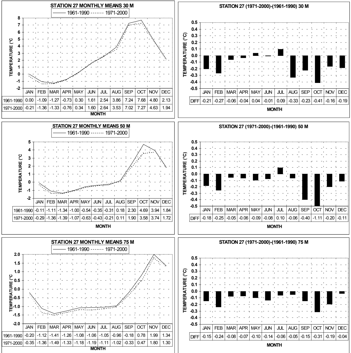
Fig. 1b. Monthly means (left panels) and differences (right panels) of temperature at Station 27 for the periods 1961-1990 and 1971-2000 at standard depths.
