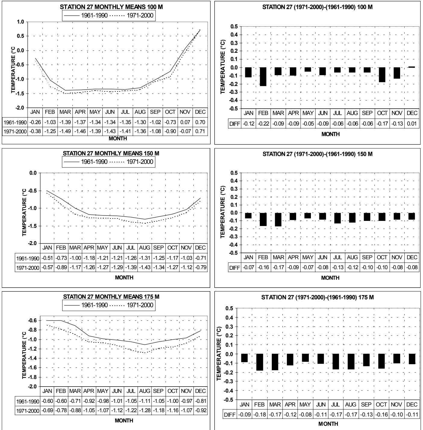
Fig. 1c. Monthly means (left panels) and differences (right panels) of temperature at Station 27 for the periods 1961-1990 and 1971-2000 at standard depths.
