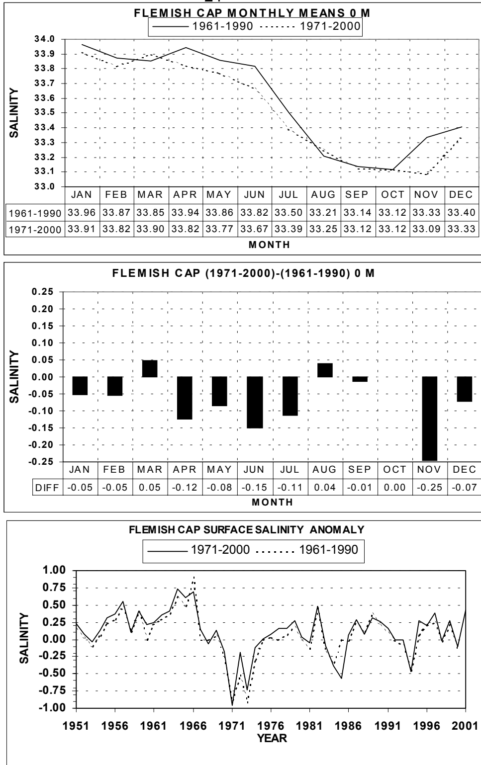
Fig. 7a. Monthly means (top panel), differences (centre panel) and annual anomalies (bottom panel) of surface salinity on the Flemish Cap for the periods 1961-1990 and 1971-2000.
