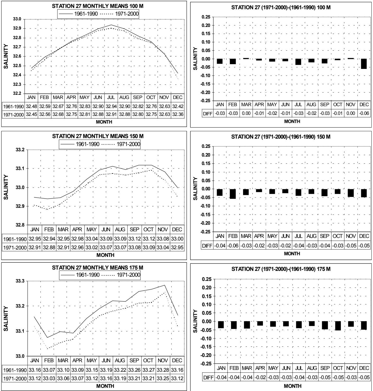
Fig. 3b. Monthly means (left panels) and differences (right panels) of salinity at Station 27 for the periods 1961-1990 and 1971-2000 at standard depths.
