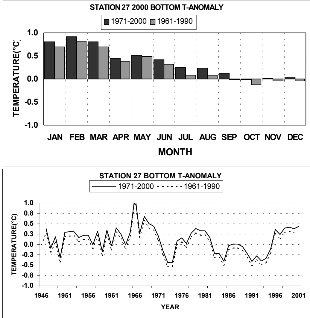
Fig. 2b. Monthly means (top panel) of bottom temperature during 2000 and the annual anomalies (bottom panel) at Station 27 referenced to the periods 1961-1990 and 1971-2000.
