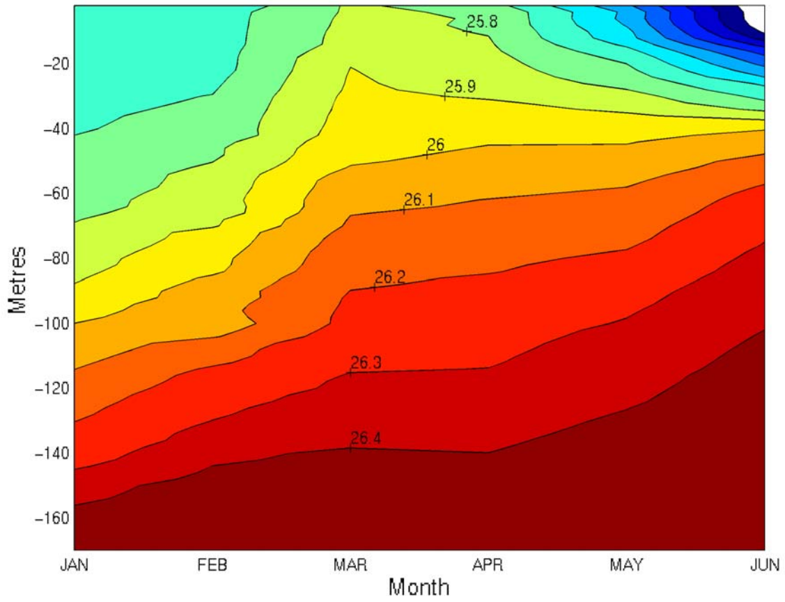
Fig.14. Density time series at increased resolution for winter and spring.
