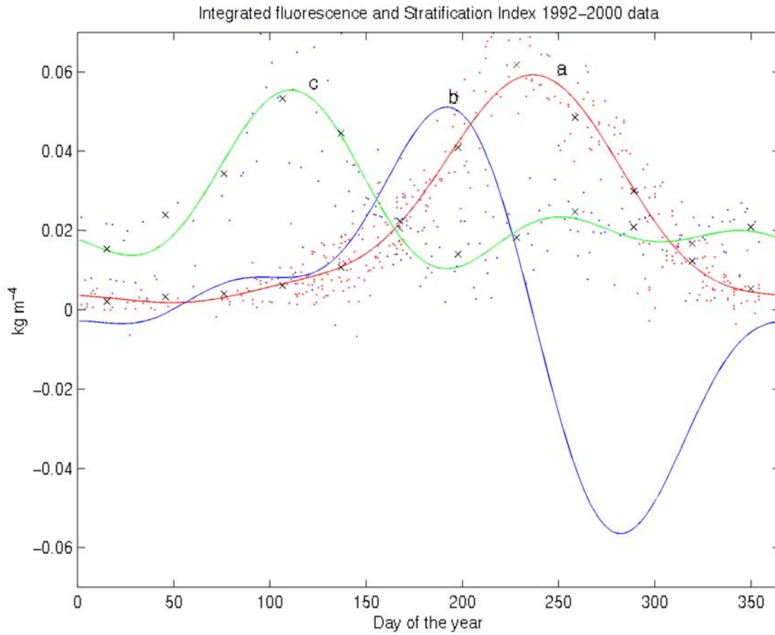
Fig.16. Stratification index (solid), the time derivative of stratification index (dashed) and integrated fluorescence (dotted) for data in the 1992-2000 period for Station 27. The scales for the derivative and fluorescence are relative. Small crosses show the values of the monthly mean stratification index and integrated fluorescence.
