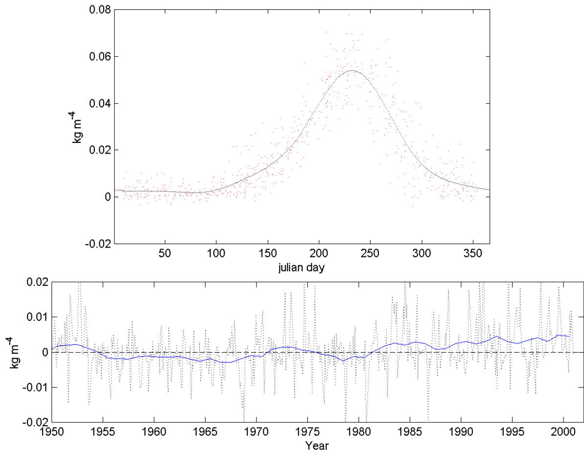
Fig.3. Harmonic regression of stratification index at station 27 and anomaly time series.
