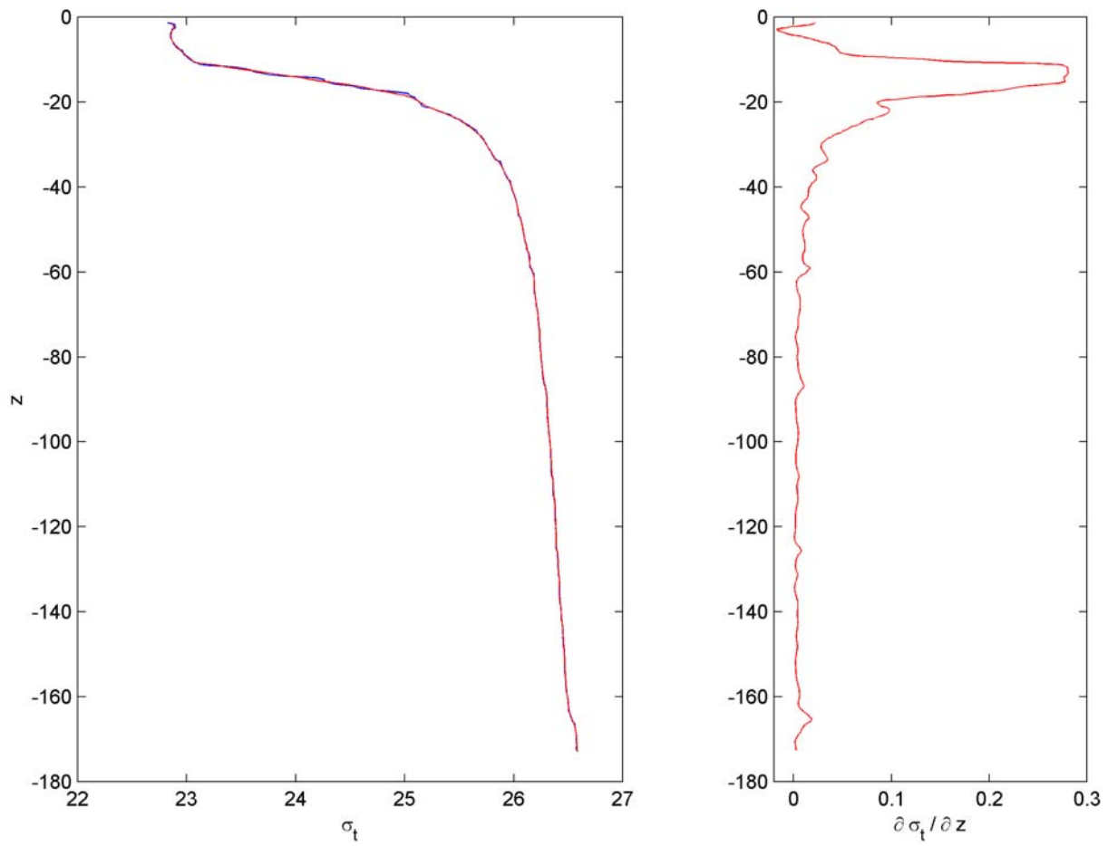
Fig.5. Numerical differentiation of density with respect to depth. The data and derivative have been filtered with 20 iterations of a three-point smoothing routine.
