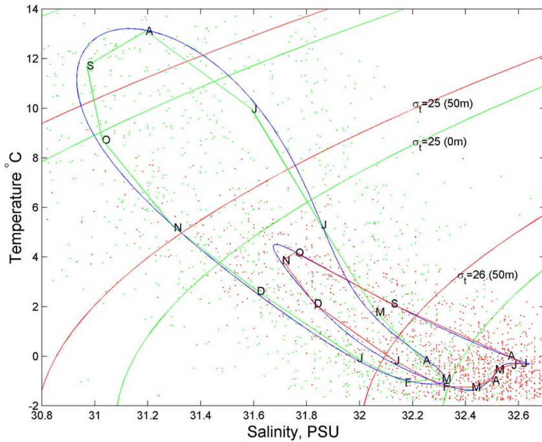
Fig.9. TS diagram for station 27 for the surface and 50 metre levels, based on the 1982 UNESCO equation of state. The letters indicate the months of the year. The dark annual cycle curves were obtained from harmonic regressions of the T and S data.
