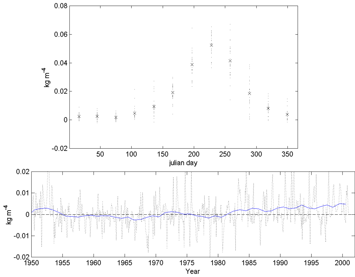
Fig.2. Annual monthly cycle of the stratification index for the 1961-1990 reference period and the time series of anomalies of monthly means (dotted line). The solid line is a 5 year running mean of annual anomalies.
