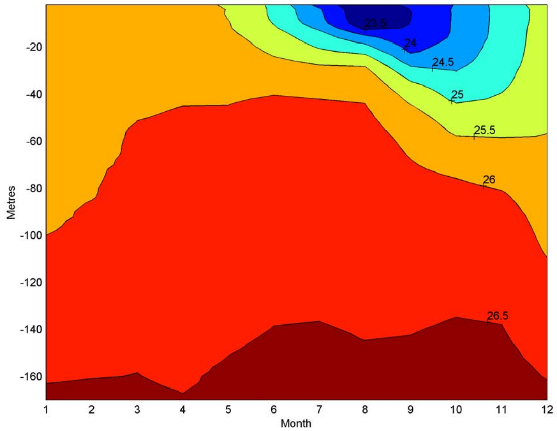
Fig.11. Density time series contour at Station 27 for 1992-2000.
