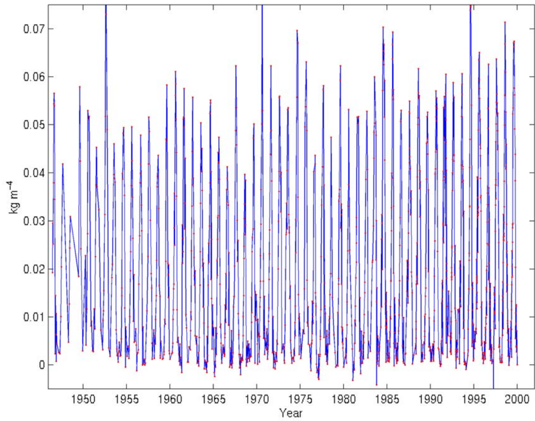
Fig.1. Time series of the stratification index at Station 27 (47° 32.8'N 52° 35.2'W)
