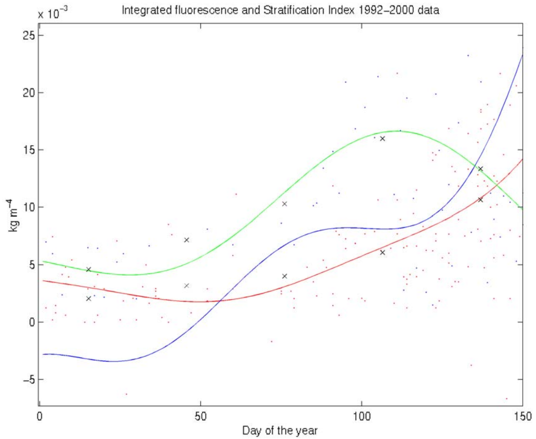
Fig.17. Expanded version of Fig.16 showing the timing of the spring bloom and onset of stratification.
