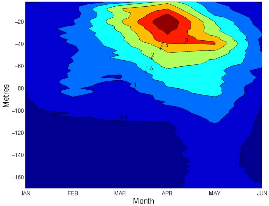
Fig.15. Fluorescence time series at increased resolution for winter and spring.
