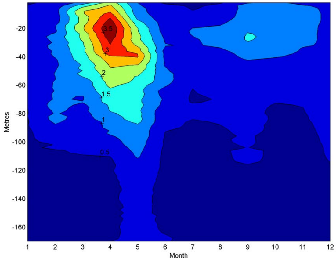
Fig.13. Fluorescence time series contour at Station 27 for 1992-2000.
