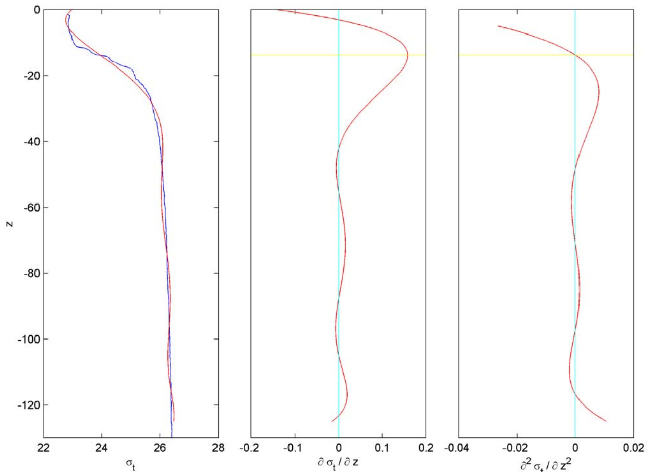
Fig.6. Polynomial regression of the density profile and calculation of the analytical derivatives. The inflection point of the density profile is the depth of maximum gradient. This depth, 13.9m was found by equating the second derivative to zero. The maximum value of the gradient was 0.153 \text{ kg m}^{-4}
