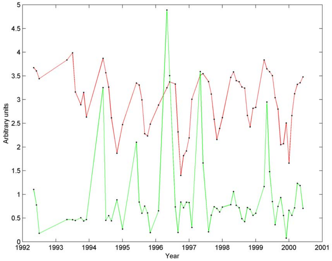
Fig.10. Integrated monthly density (top) and fluorescence, station 27.
