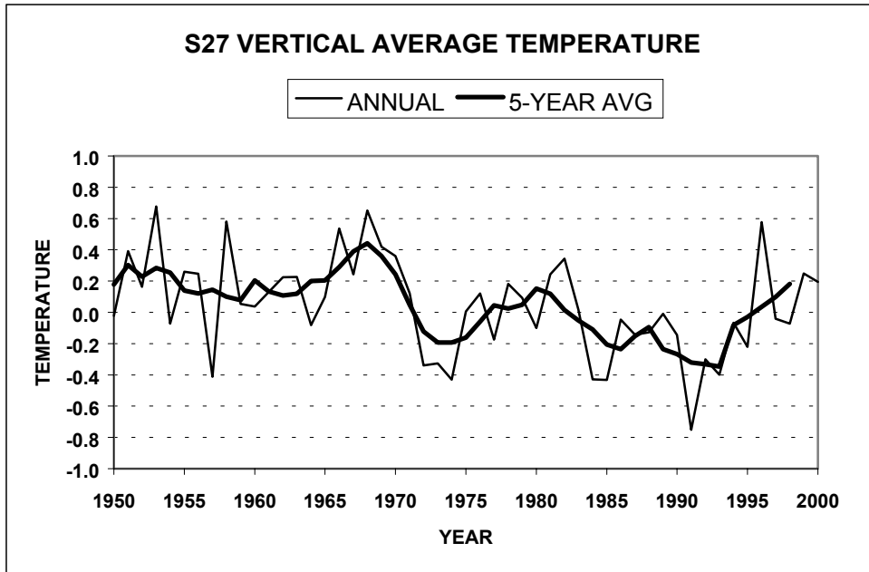
Fig.7. Vertically averaged summer temperature anomaly.
