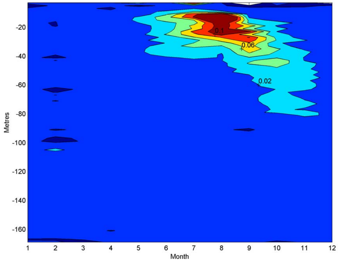
Fig.12.The gradient of density with respect to depth for station 27, 1992-2000.
