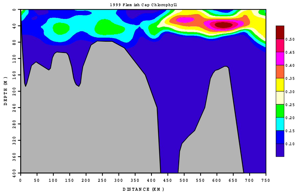
Fig.19. Fluorescence along the Flemish Cap transect.
