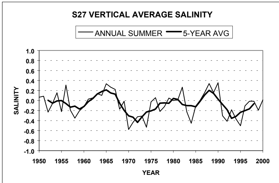
Fig.8. Vertically averaged salinity anomaly.
